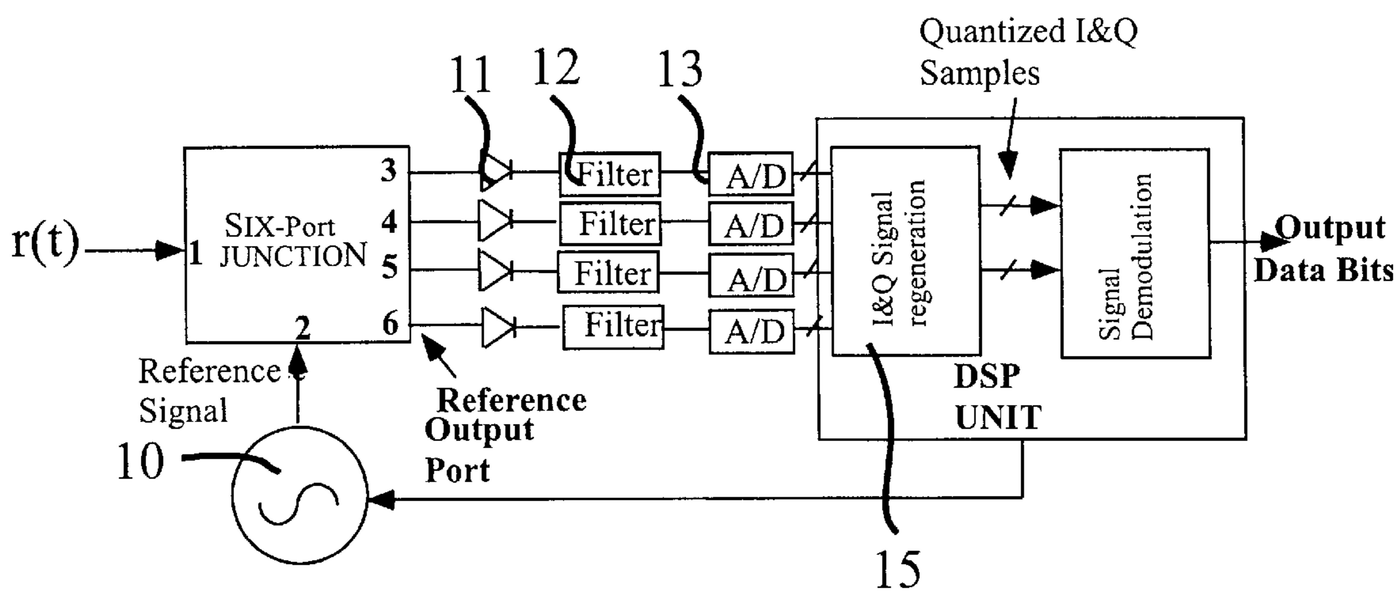
Fig. 2 PRIOR ART
