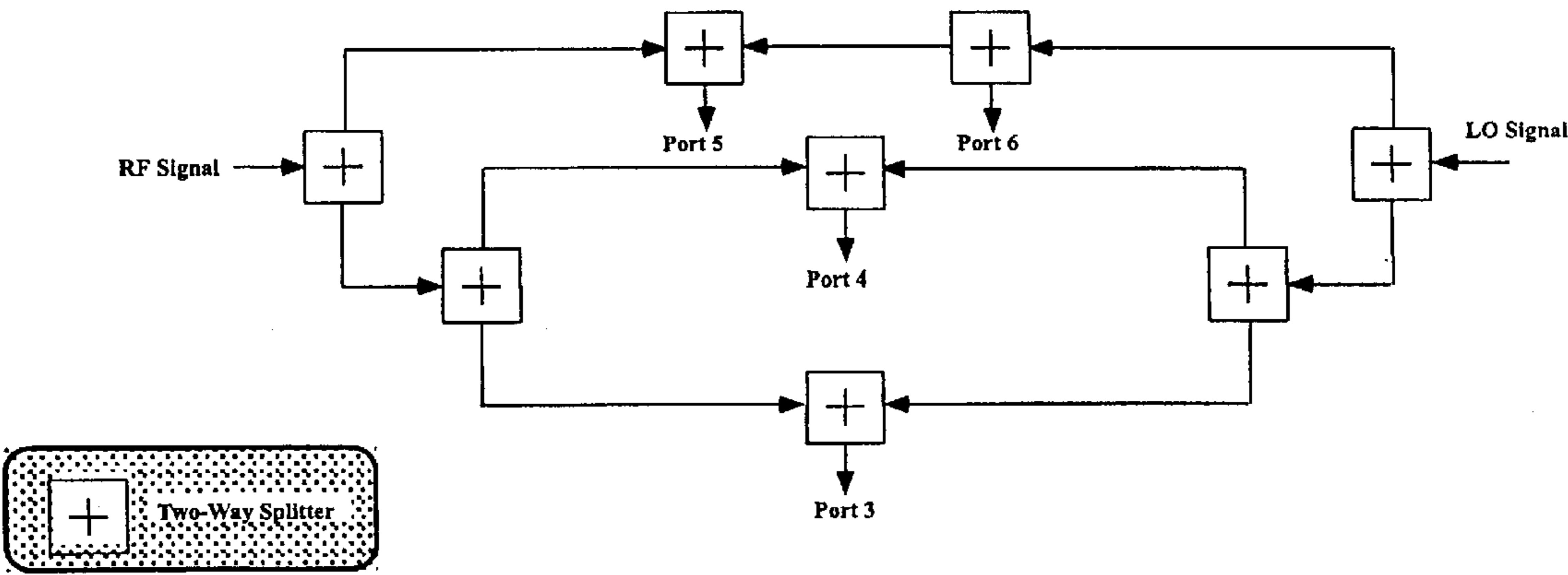
Fig. 3 PRIOR ART
