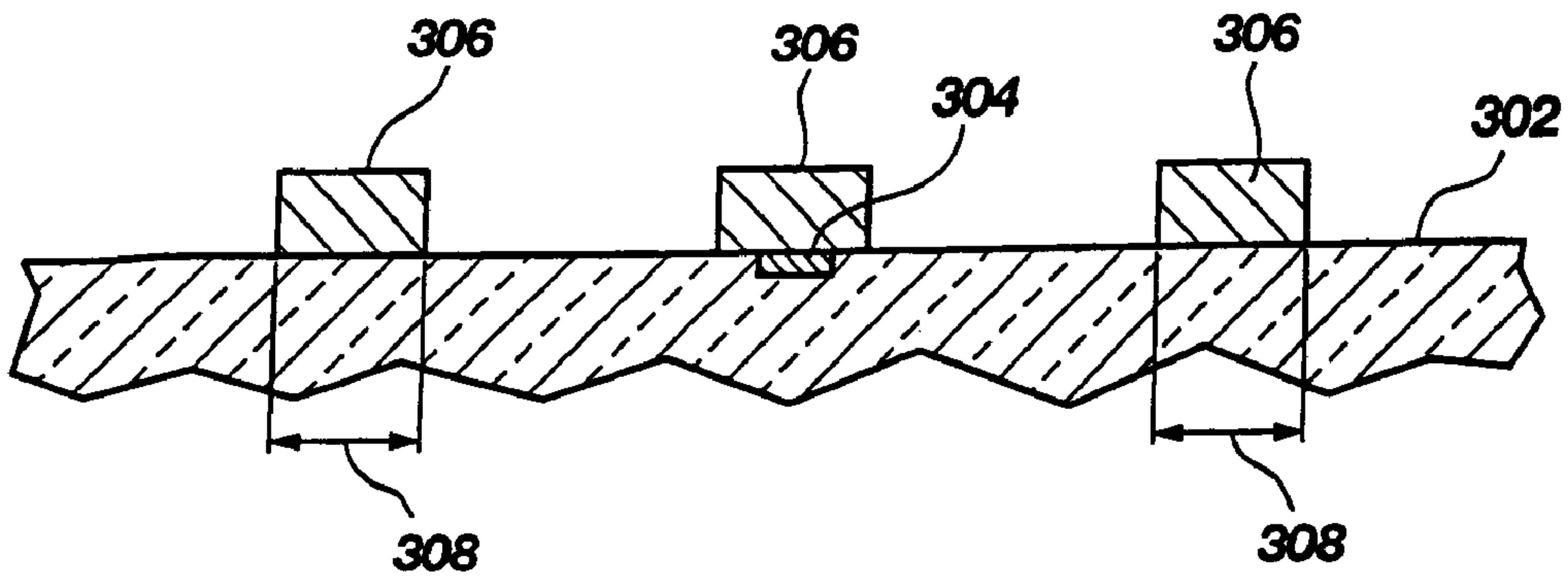
Fig. 23 (PRIOR ART)
