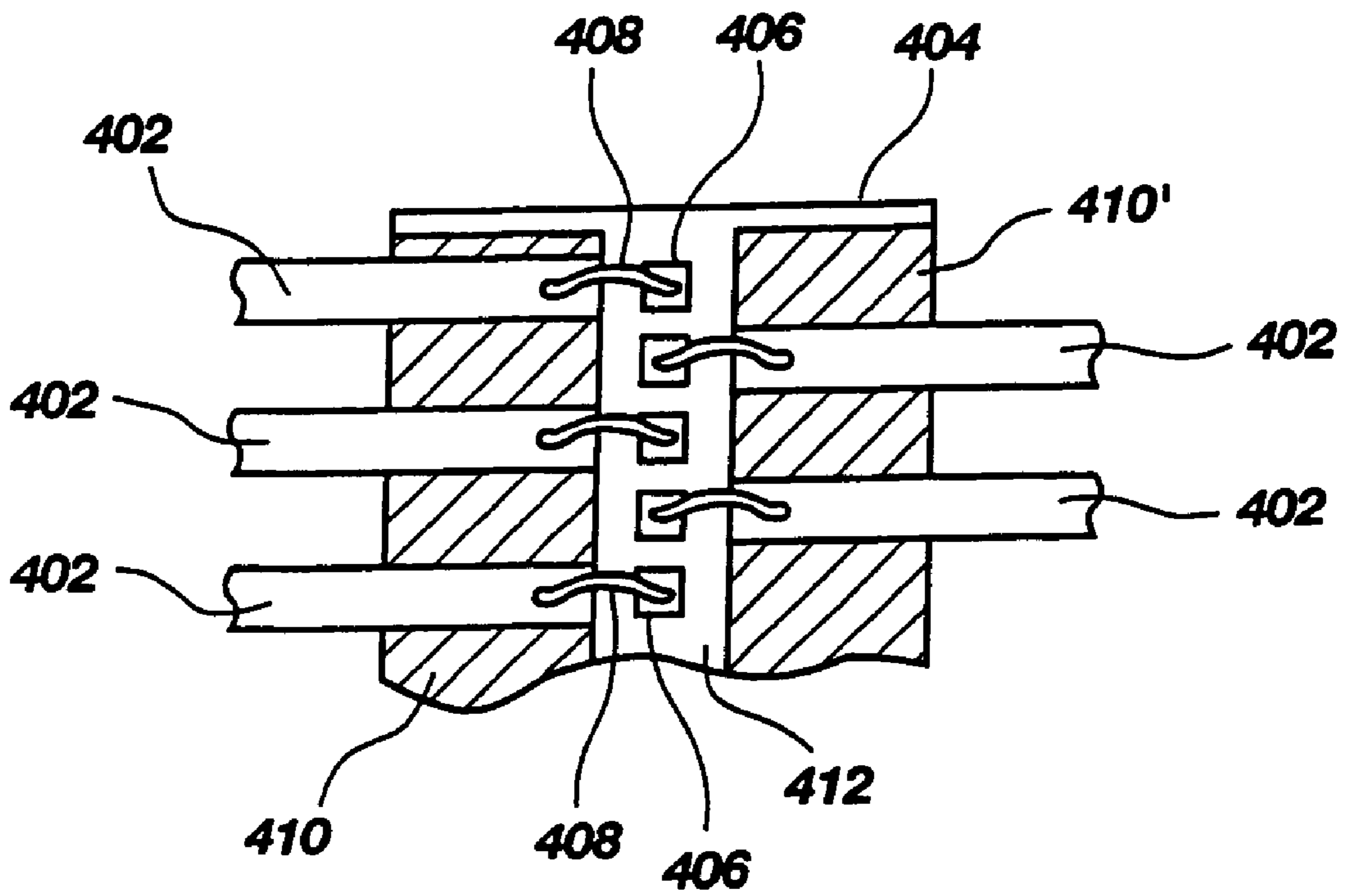
Fig. 30 (PRIOR ART)
