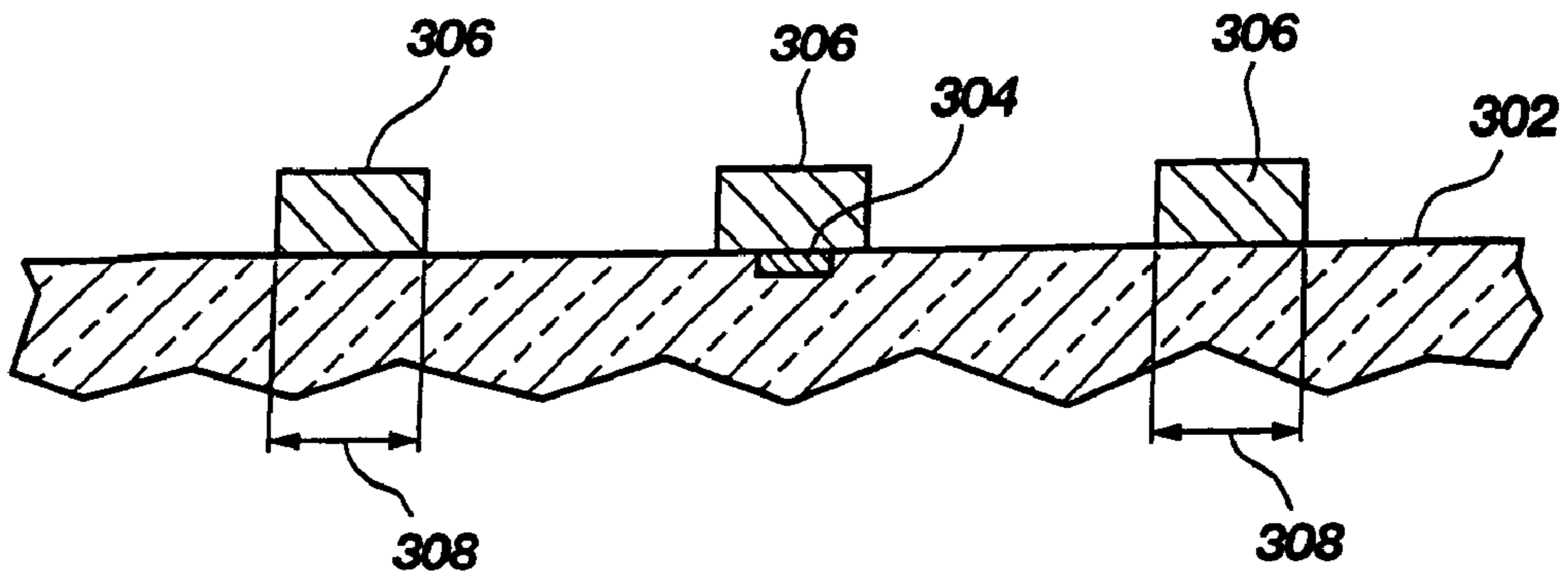
Fig. 23 (PRIOR ART)
