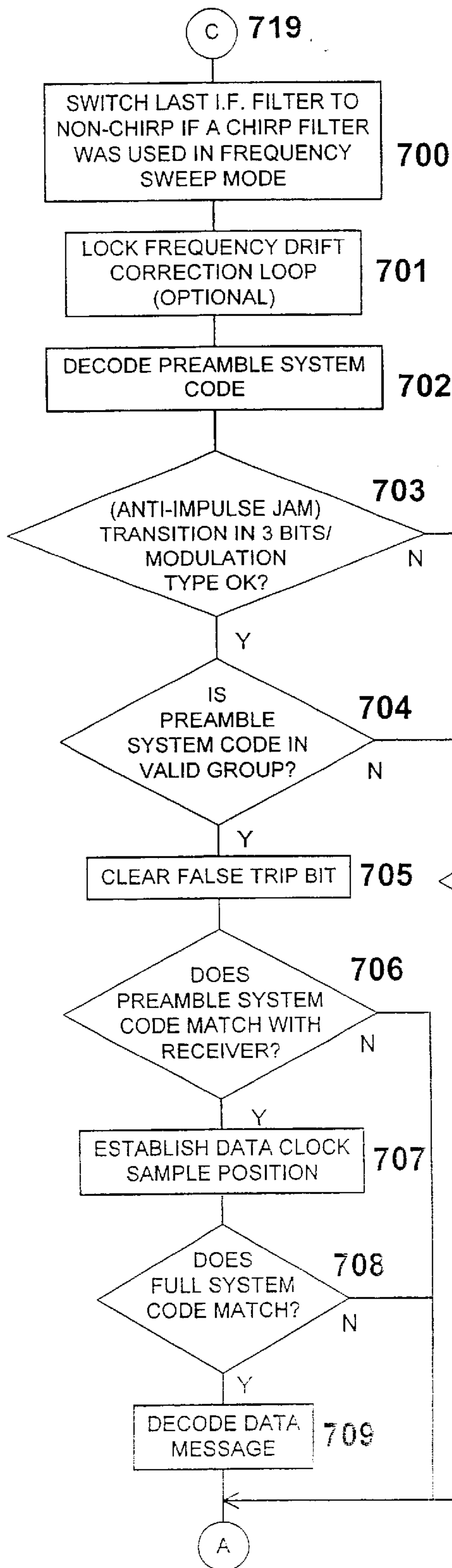
FIGURE 7A TRIP HANDLER
