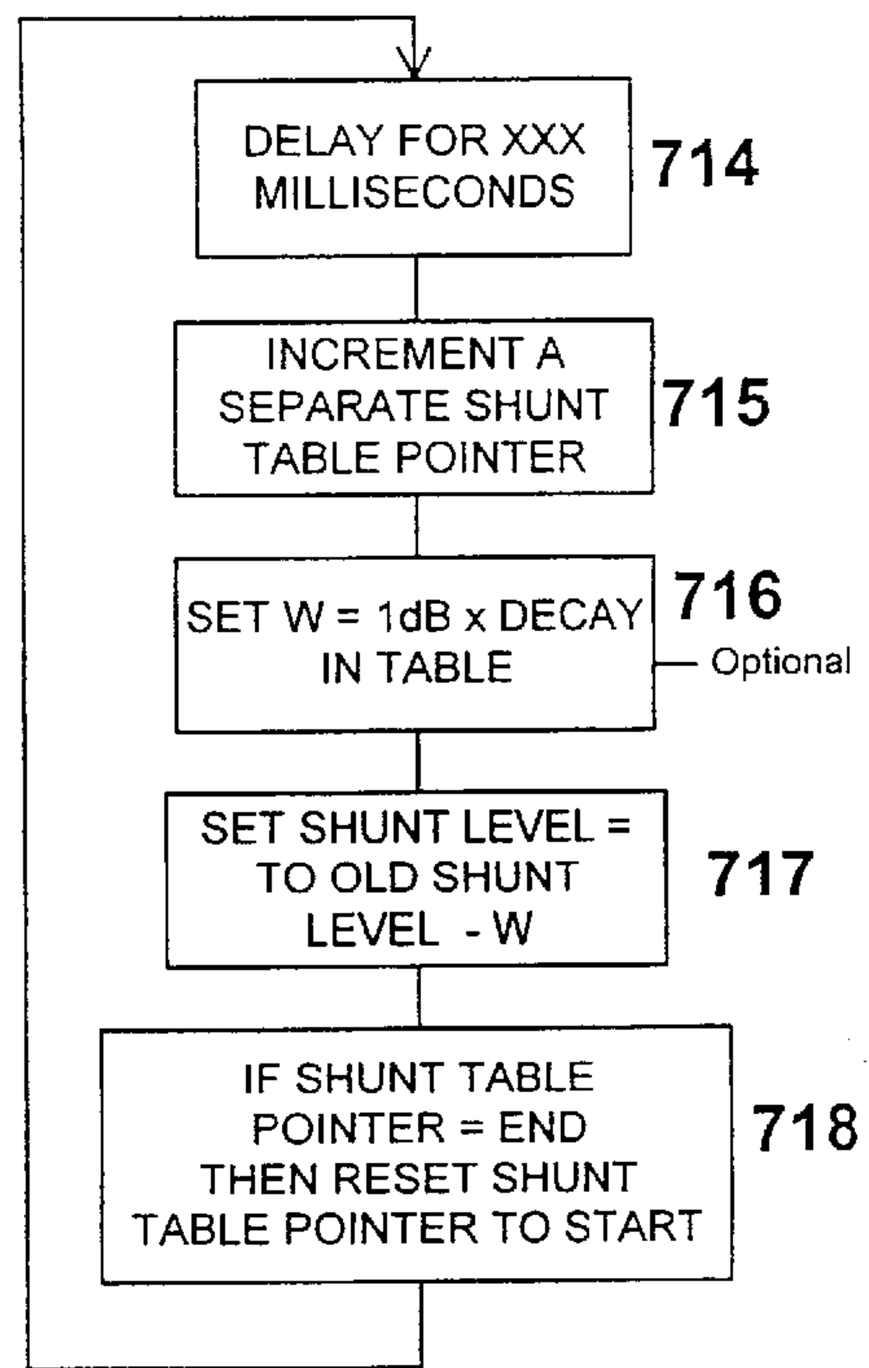
FIGURE 7B TIME BASED SHUNT DECAY
