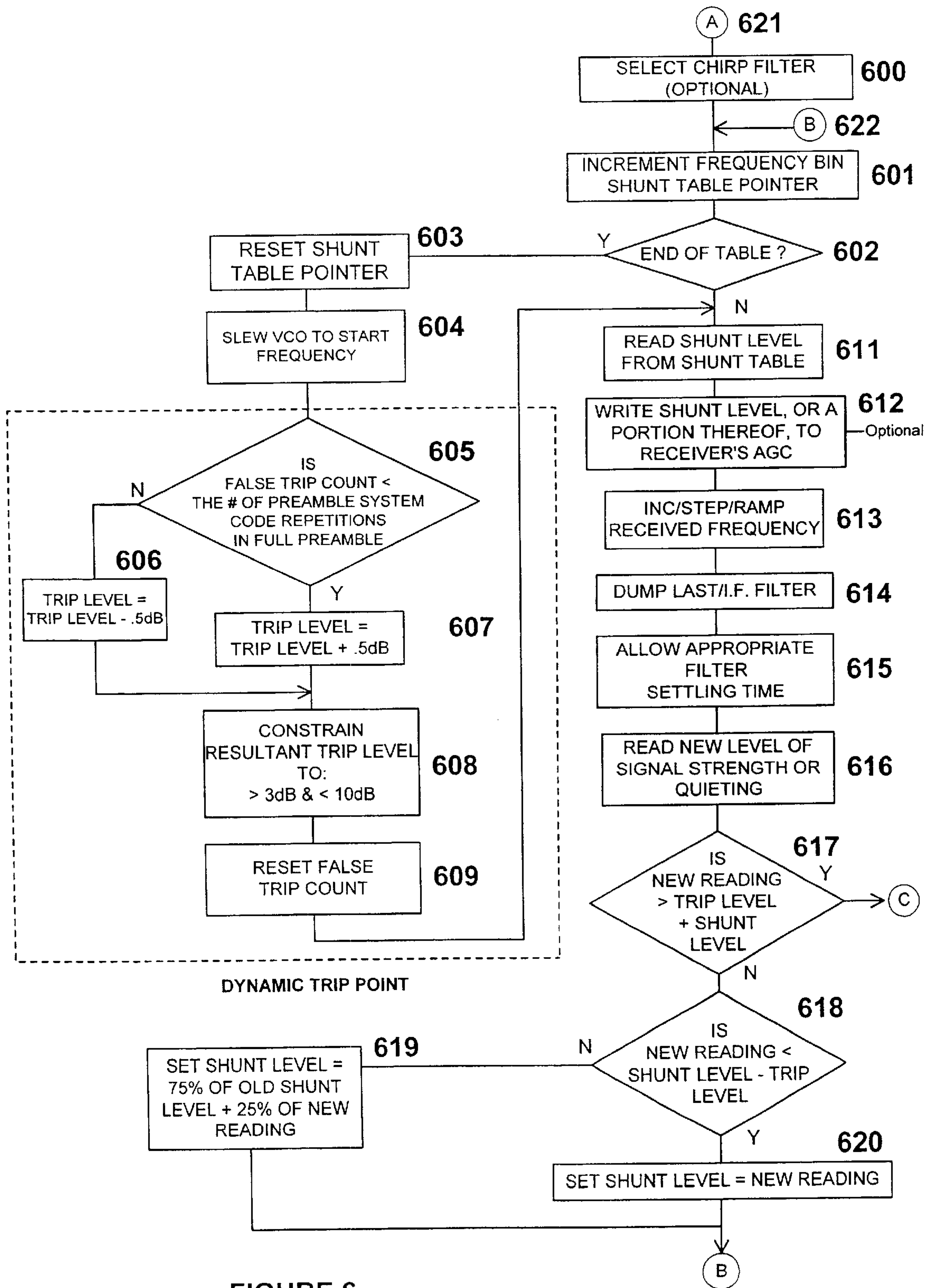
FIGURE 6 FREQUENCY SCAN ALGORITHM
