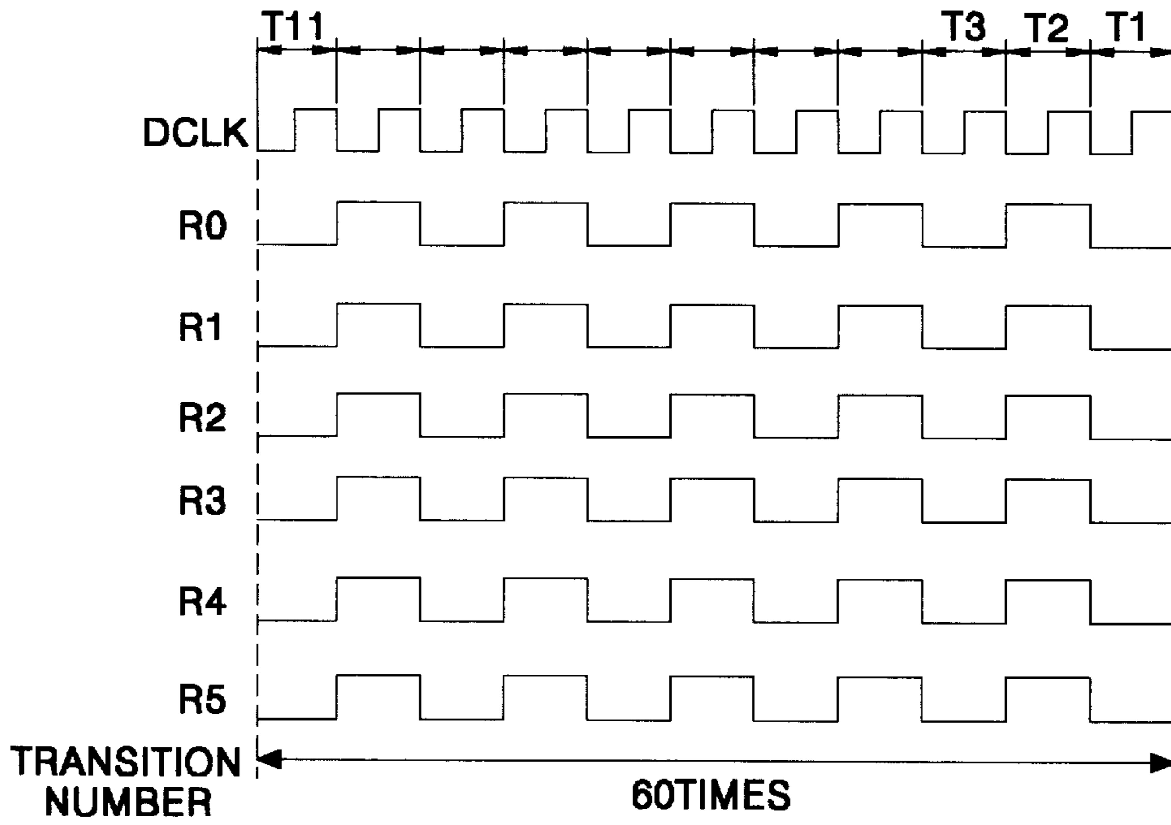
FIG. 2 PRIOR ART
