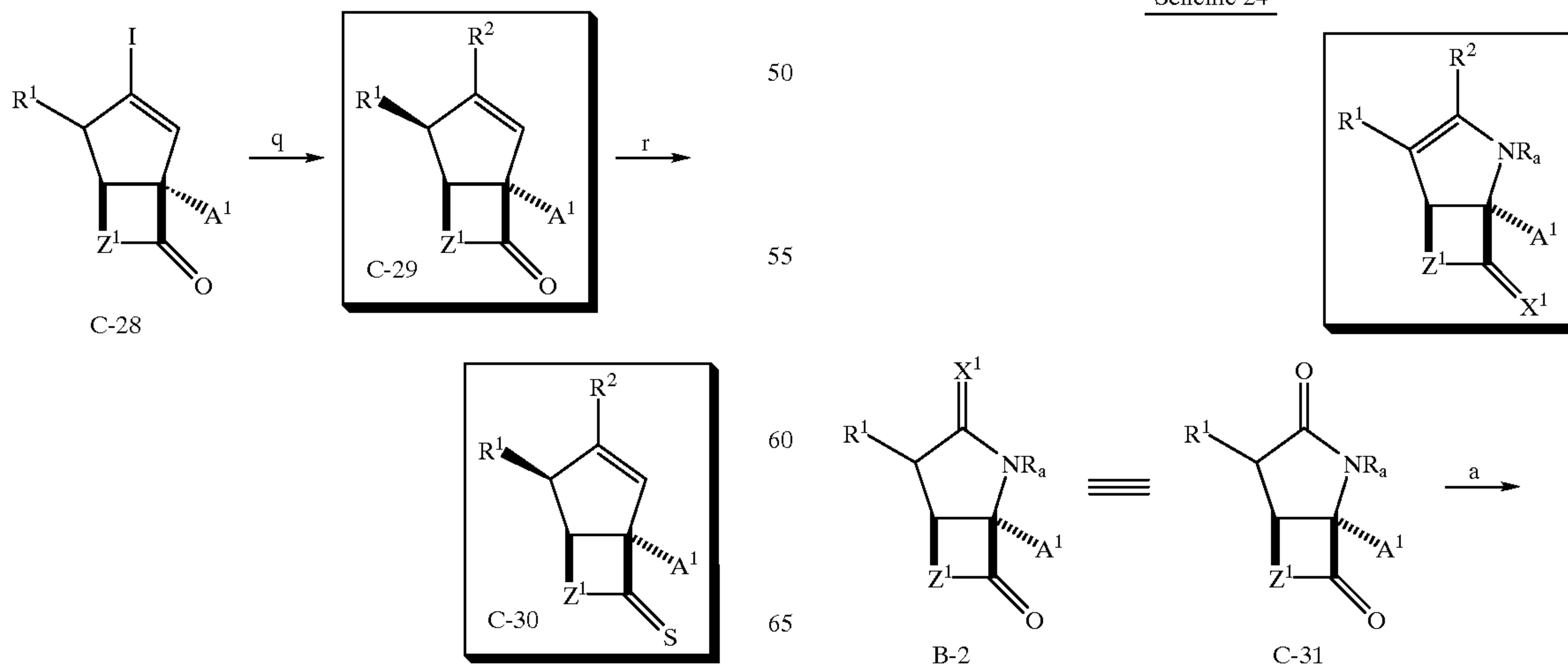
Scheme 24
