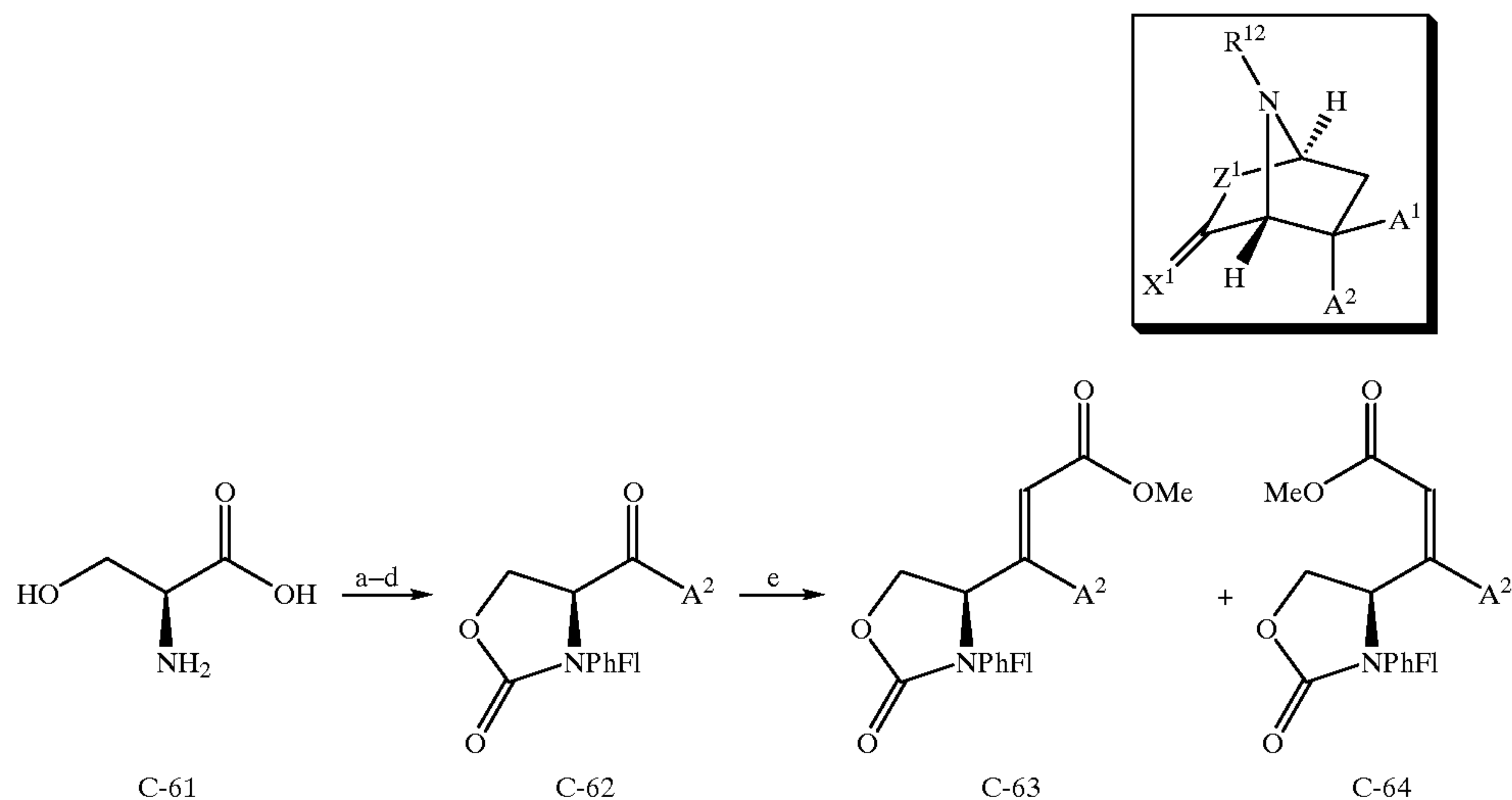
Scheme 27
