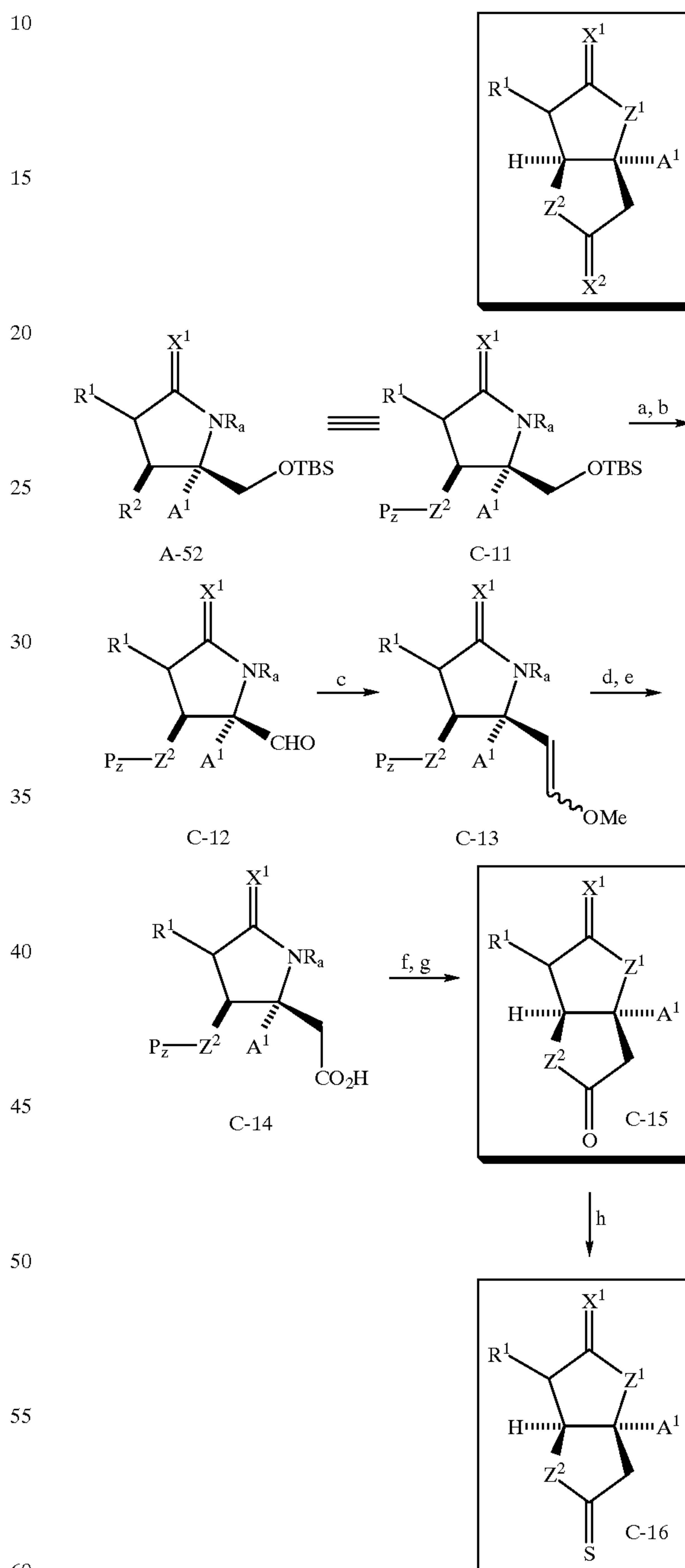
Scheme 22
