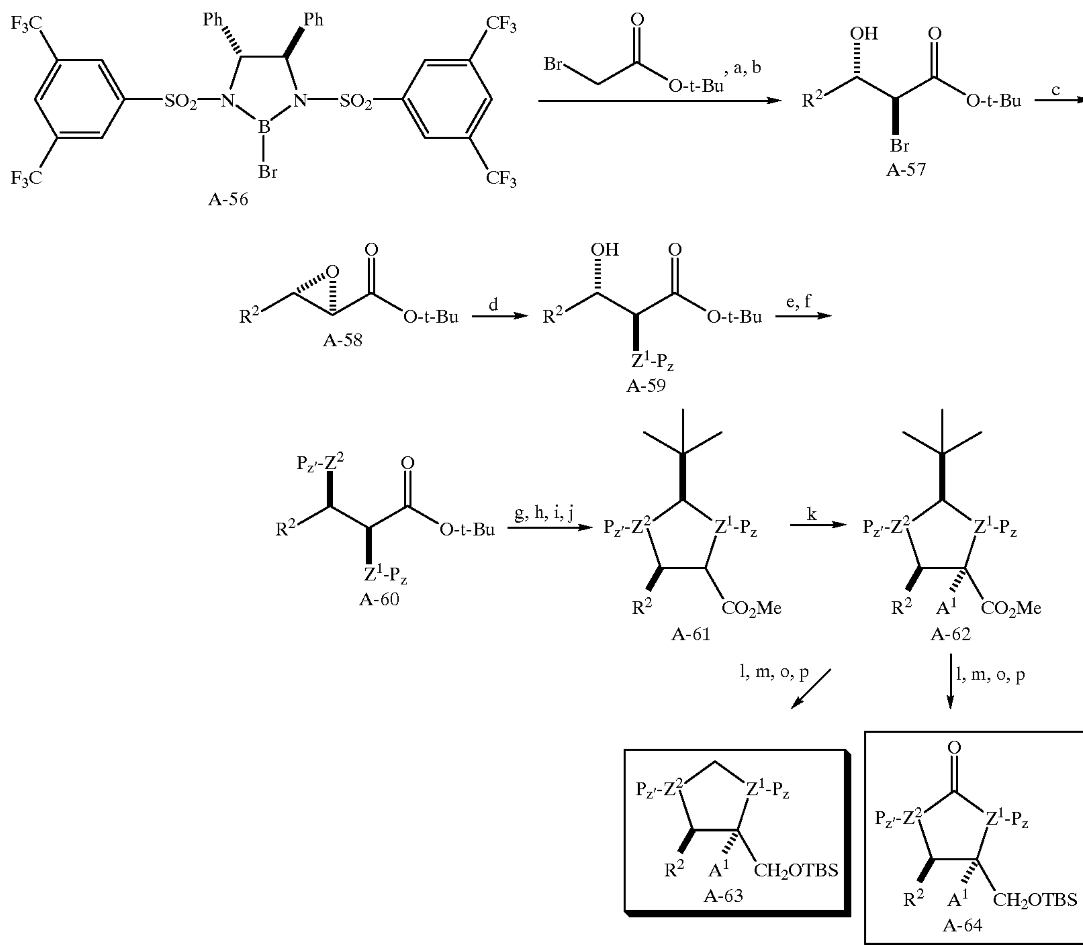
Scheme 10
