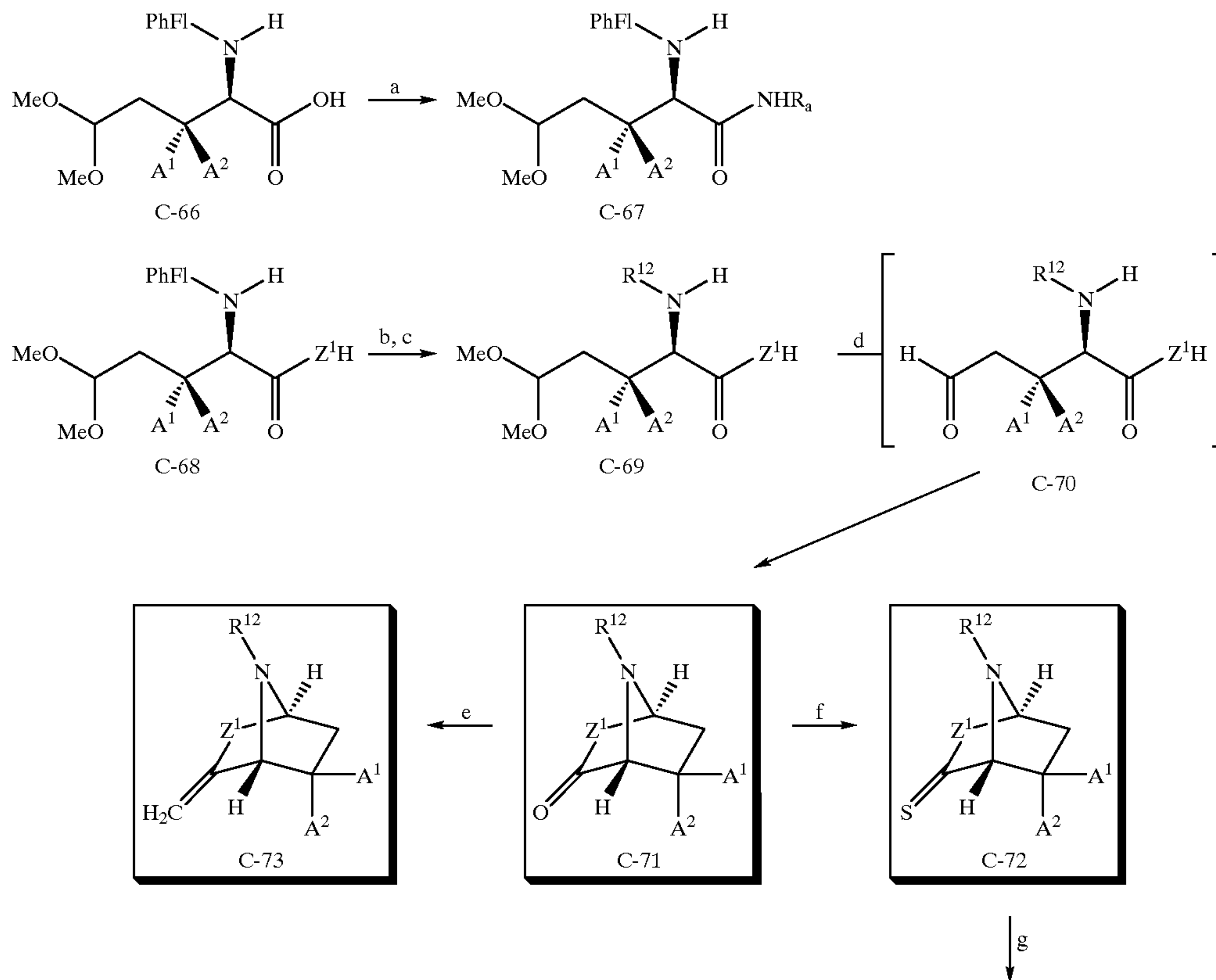
Scheme 28
