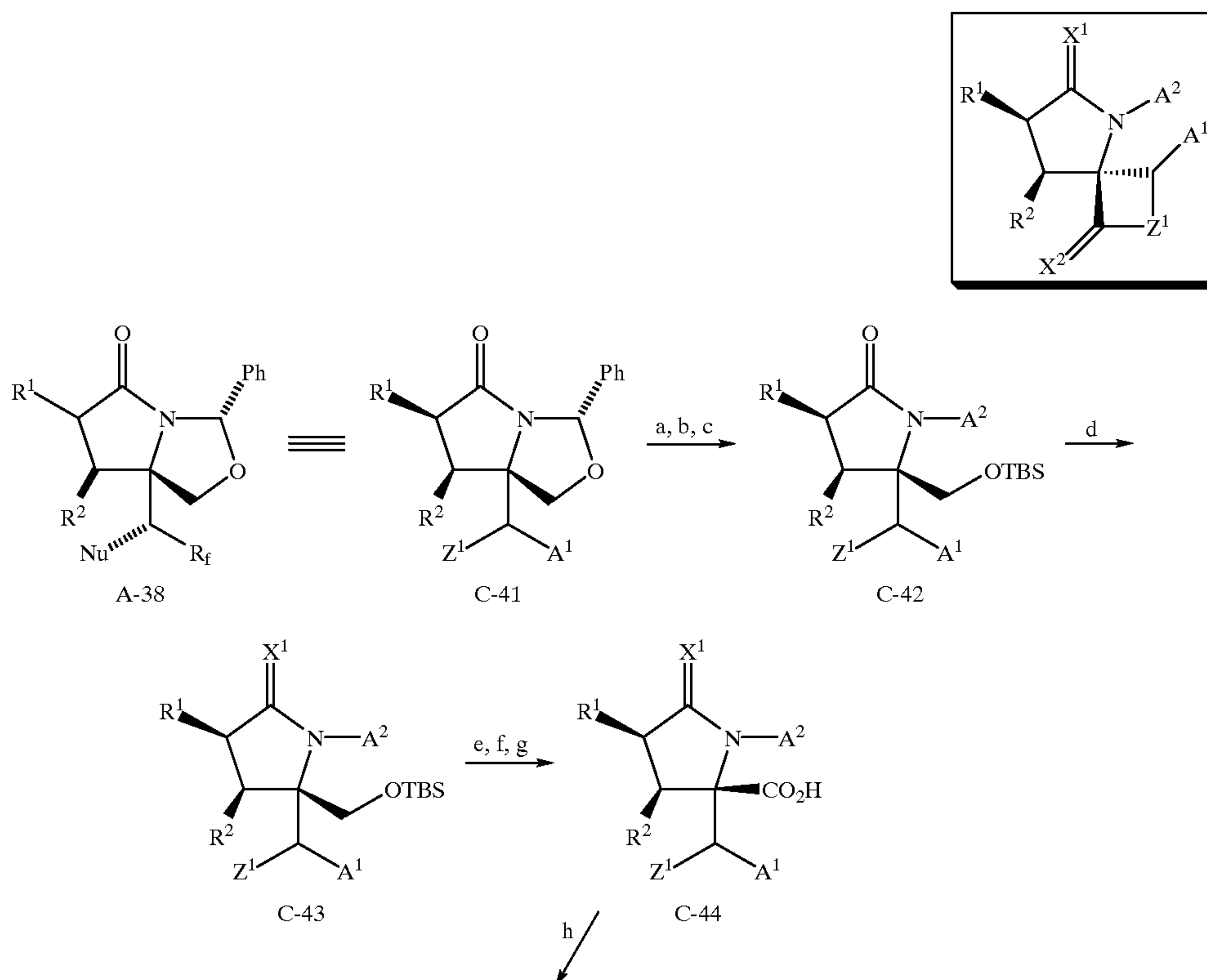
Scheme 25
