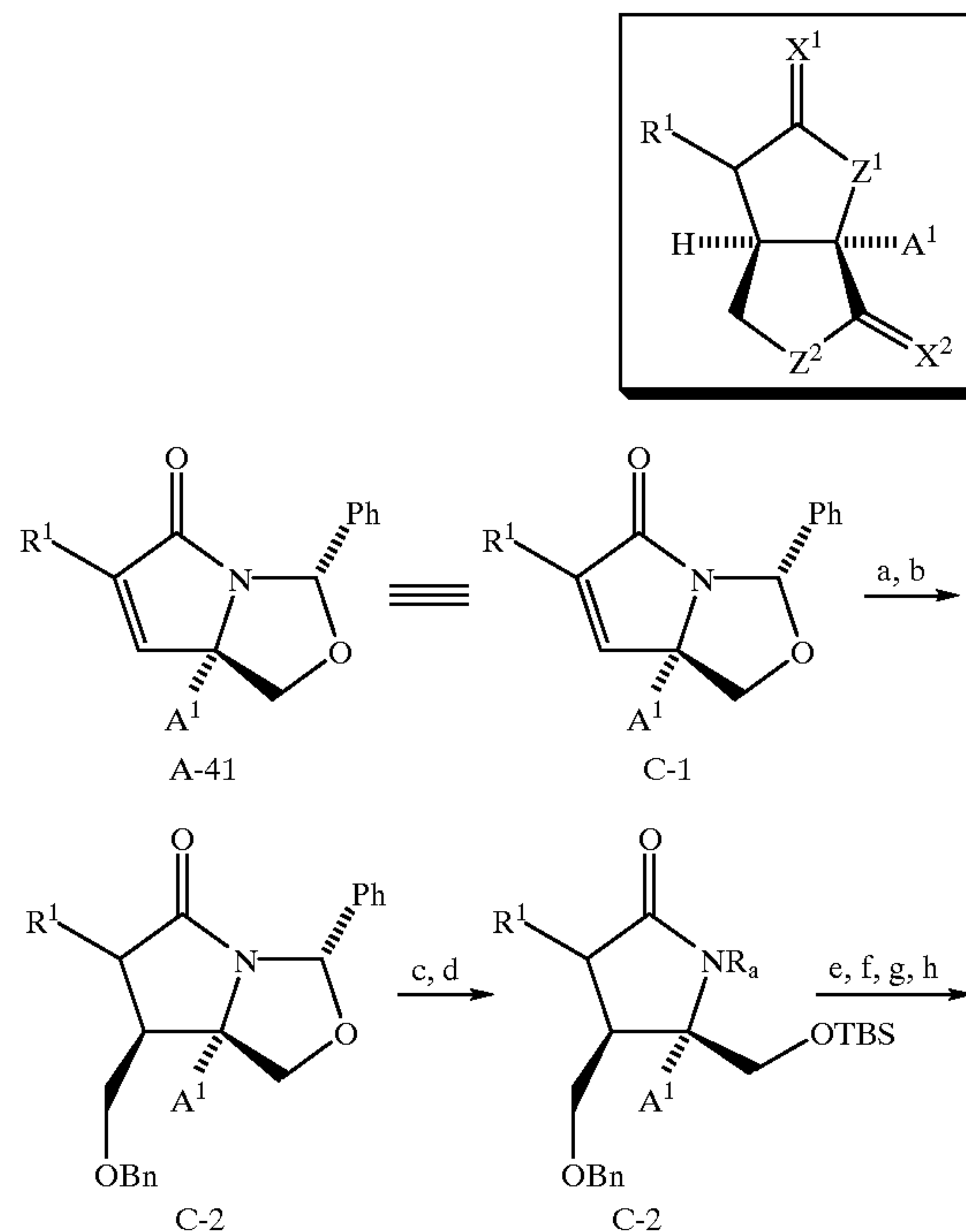
Scheme 21
