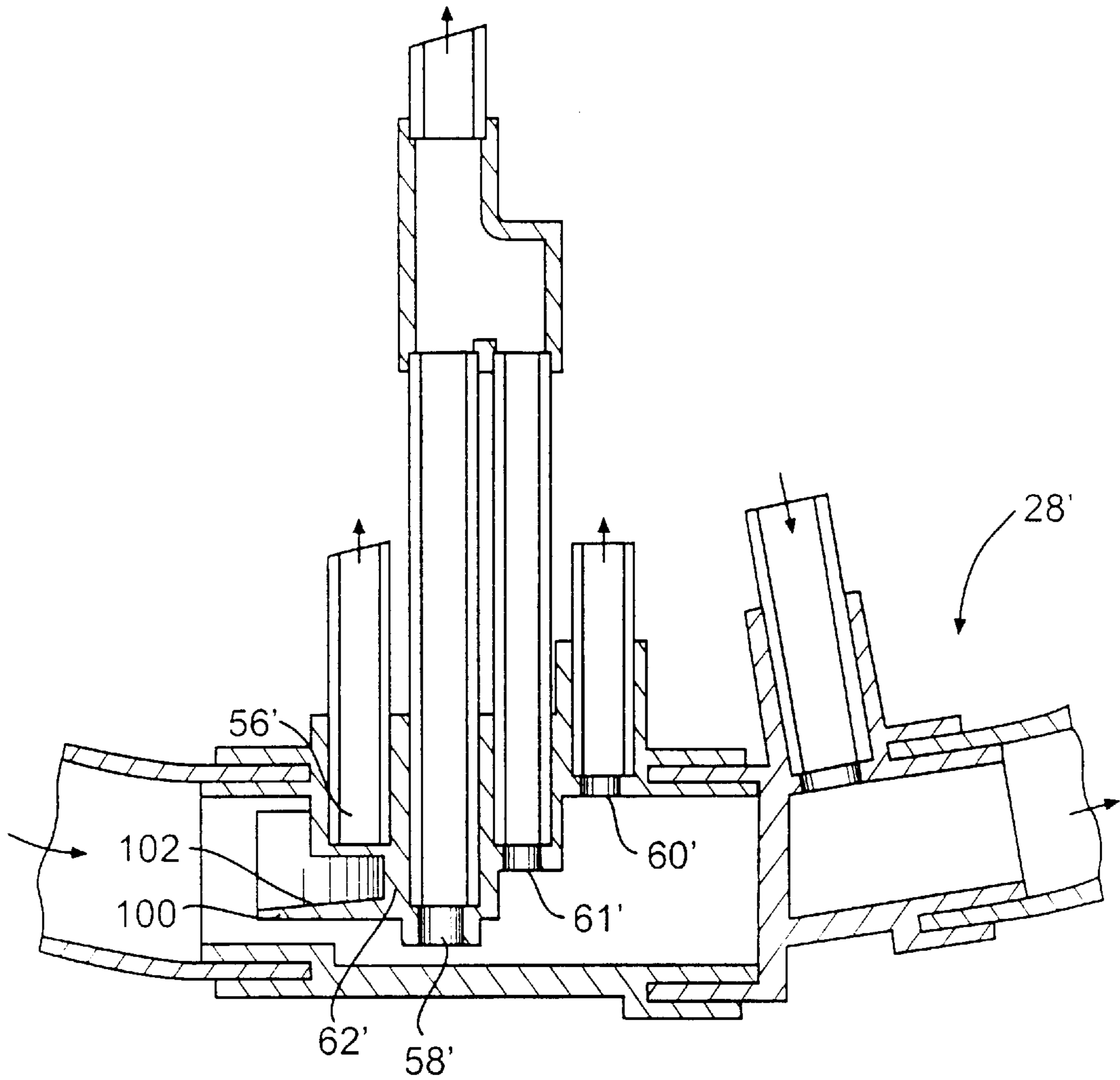
FIG. 3 (PRIOR ART)
