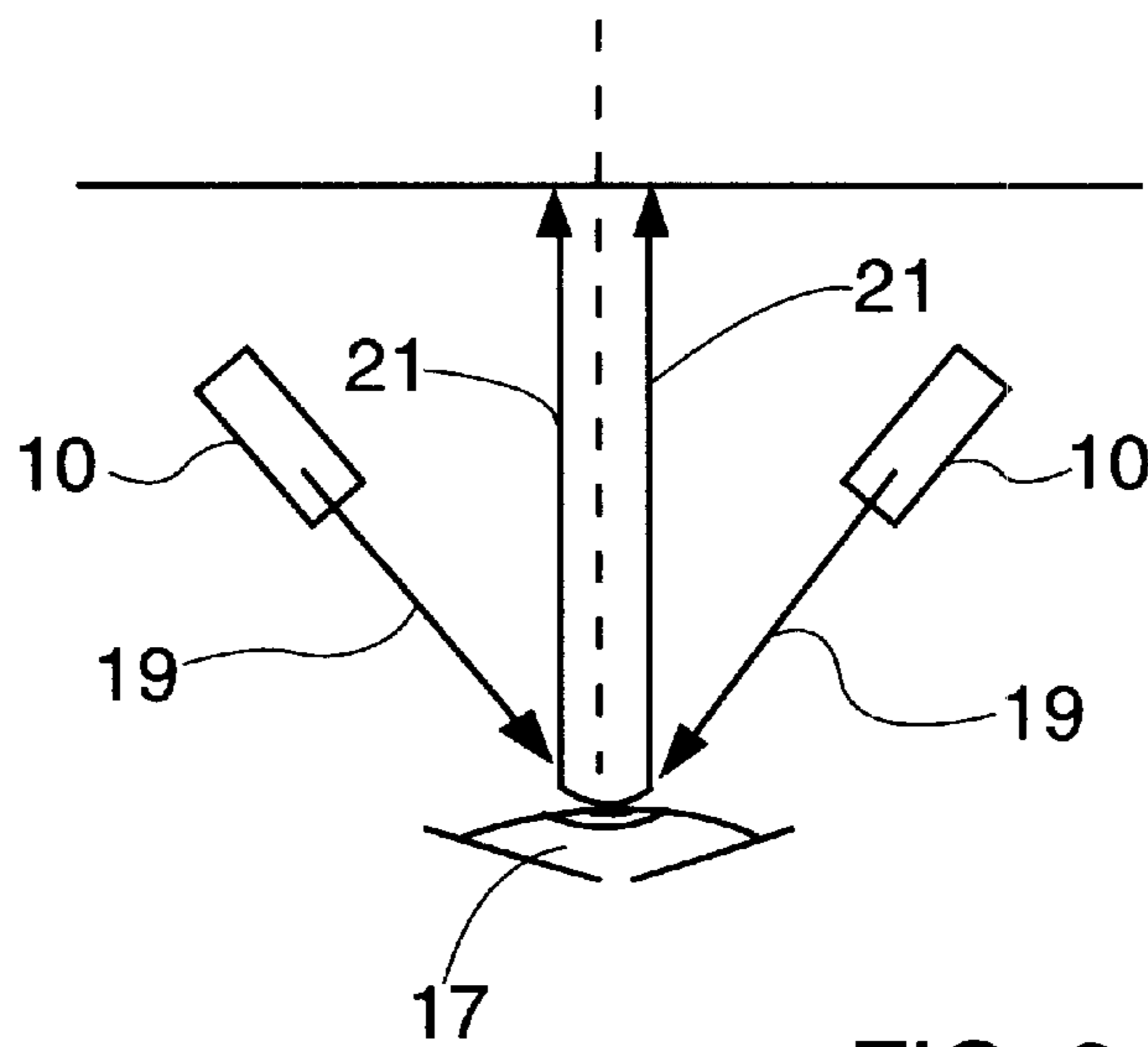
FIG. 3 PRIOR ART
