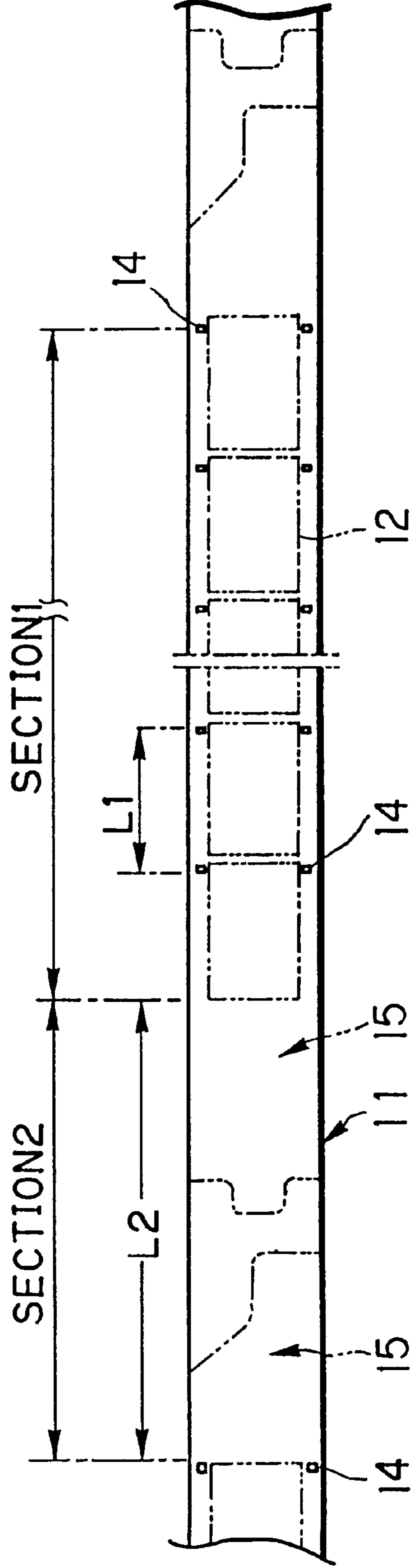
FIG. 26 PRIOR ART
