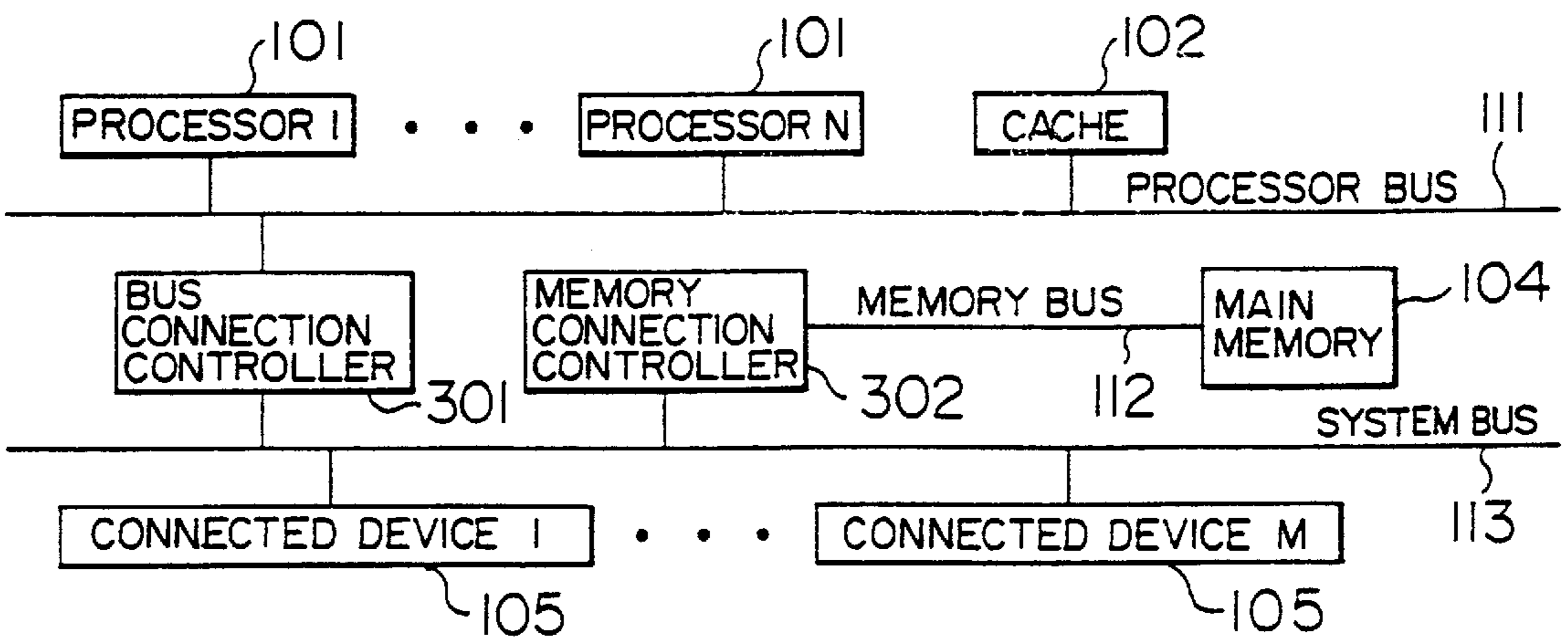
FIG. 3 PRIOR ART
