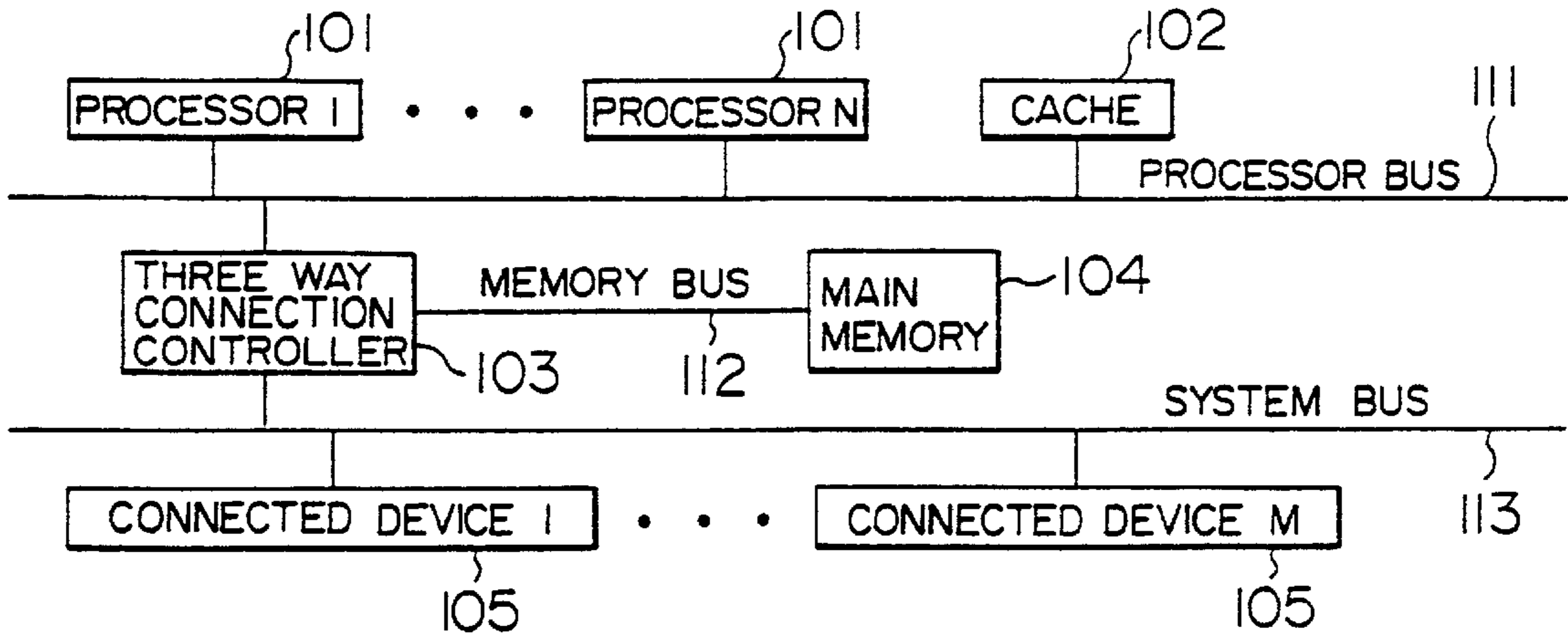
FIG. 2 PRIOR ART
