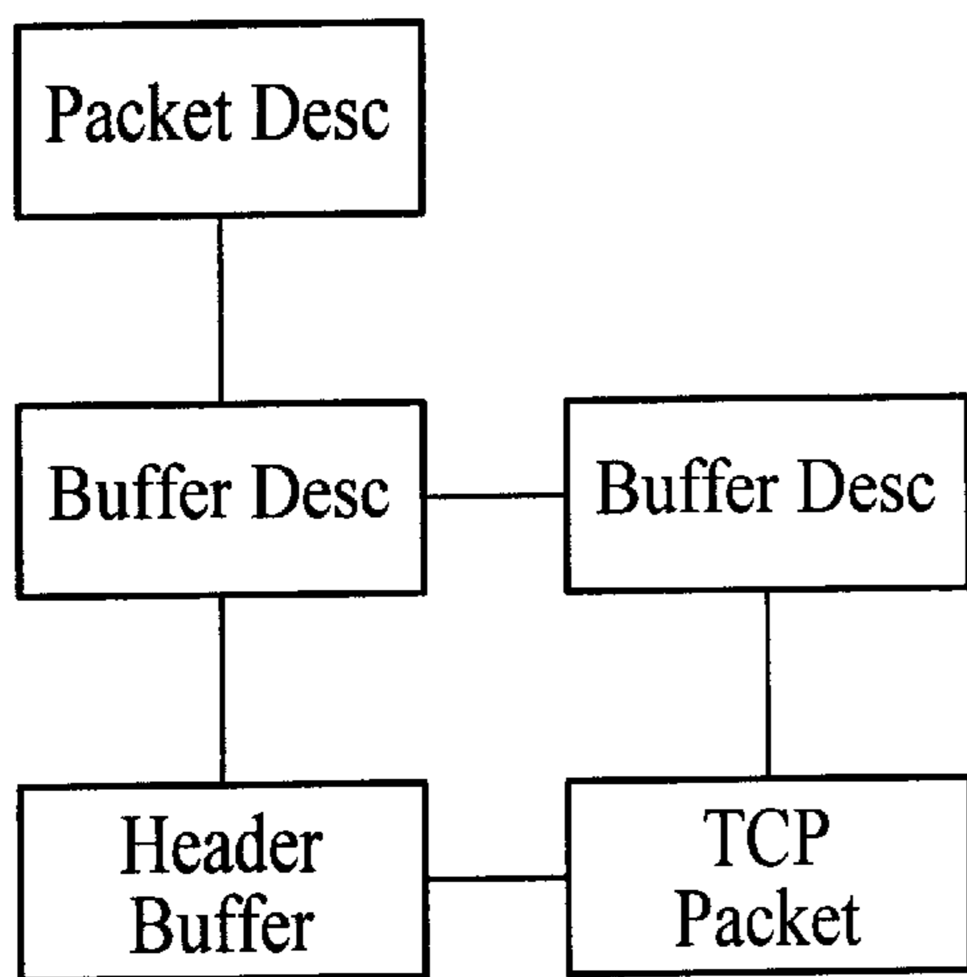
Example of incoming TCP pkt
