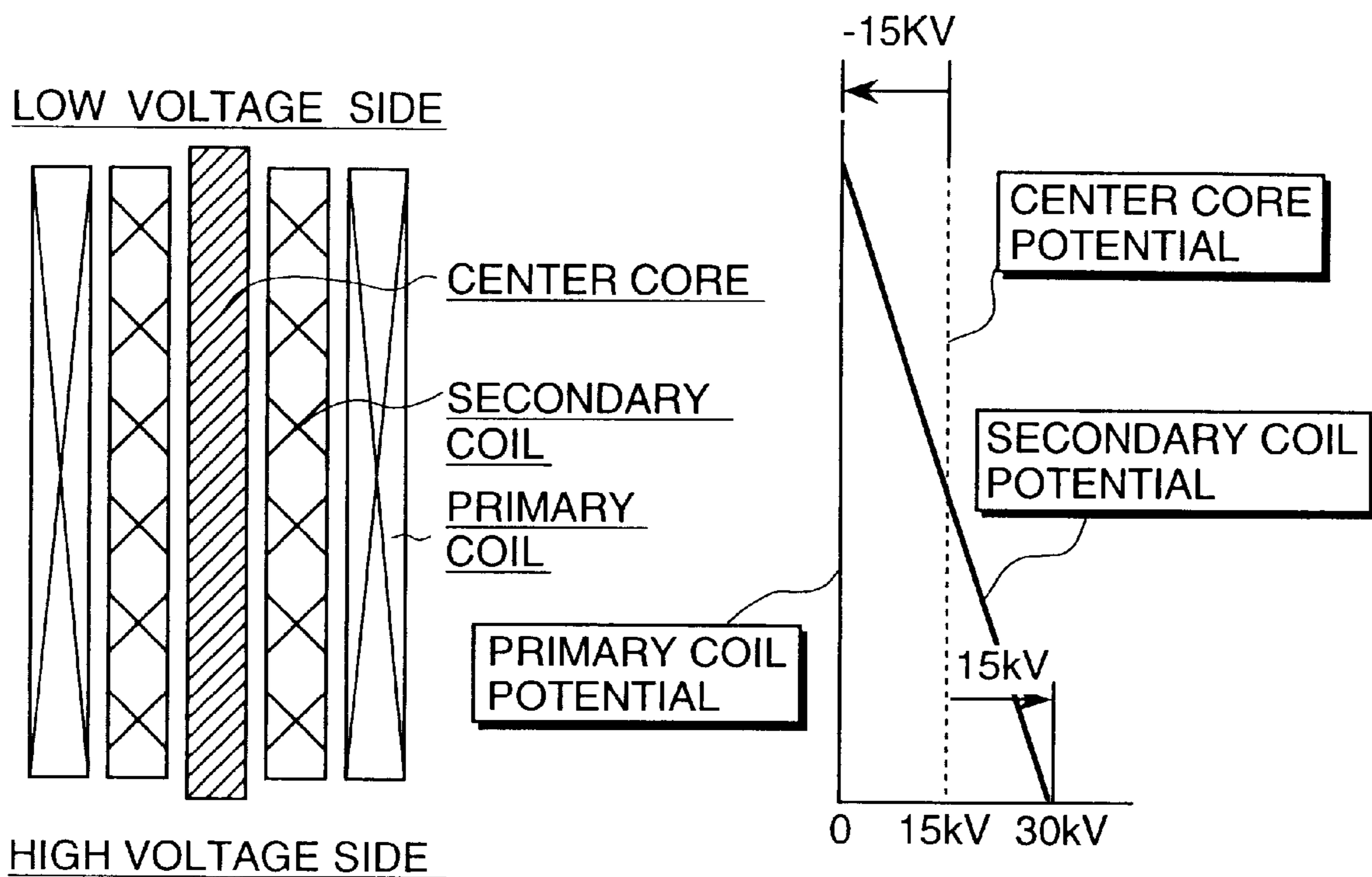
POTENTIALS OF SECONDARY COIL AND CENTER CORE
