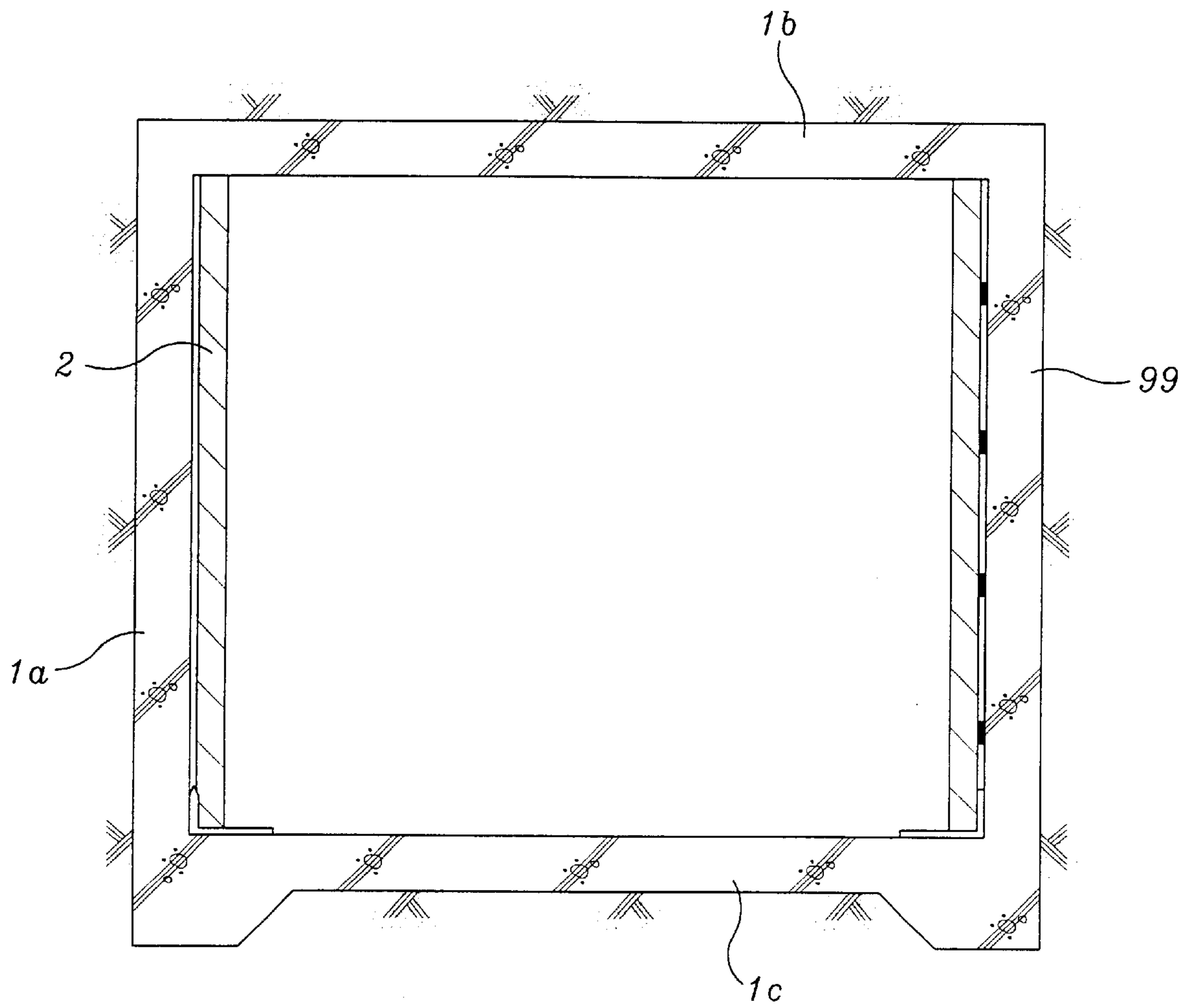
Fig. 2 conventional art
