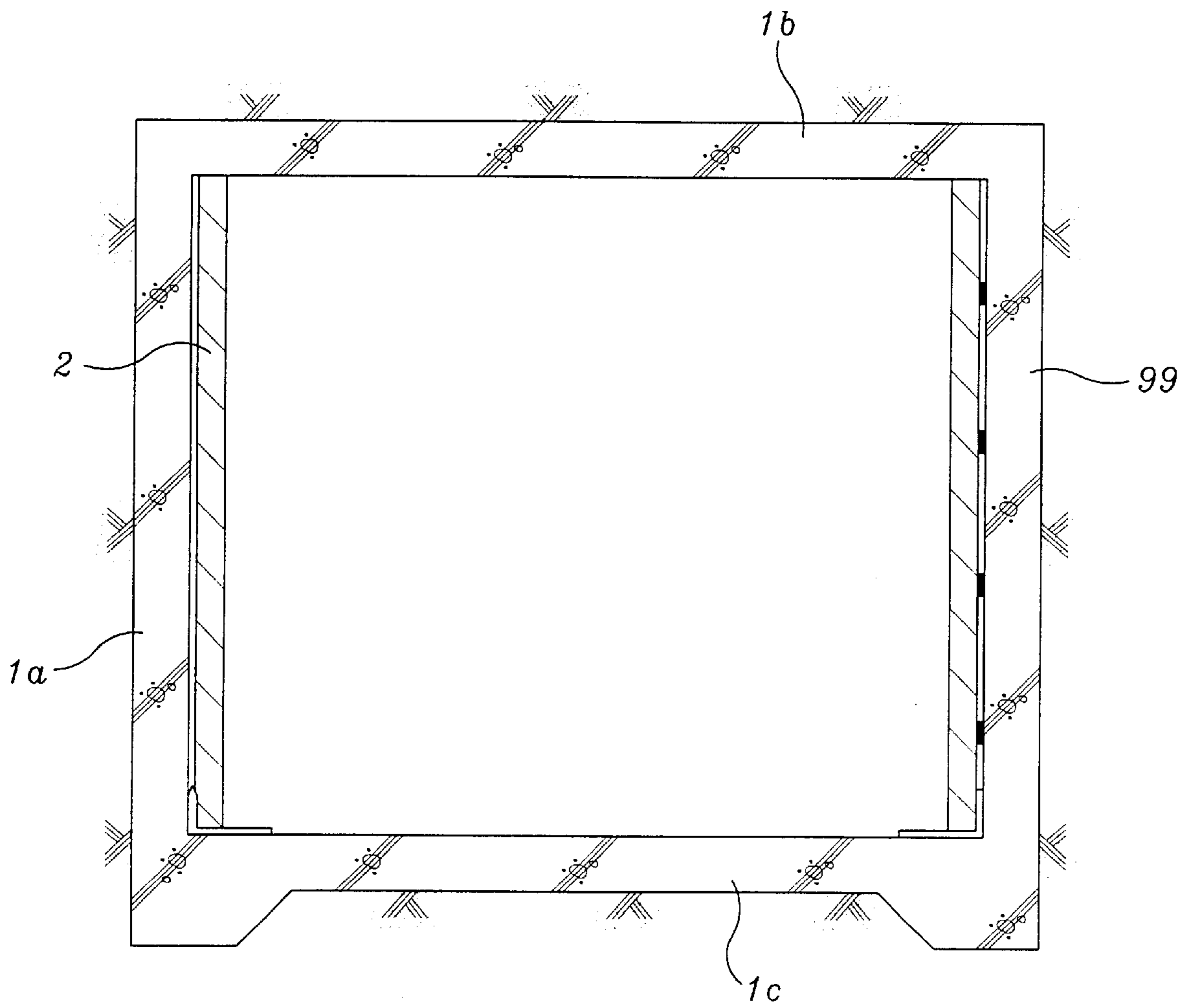
Fig. 2 conventional art
