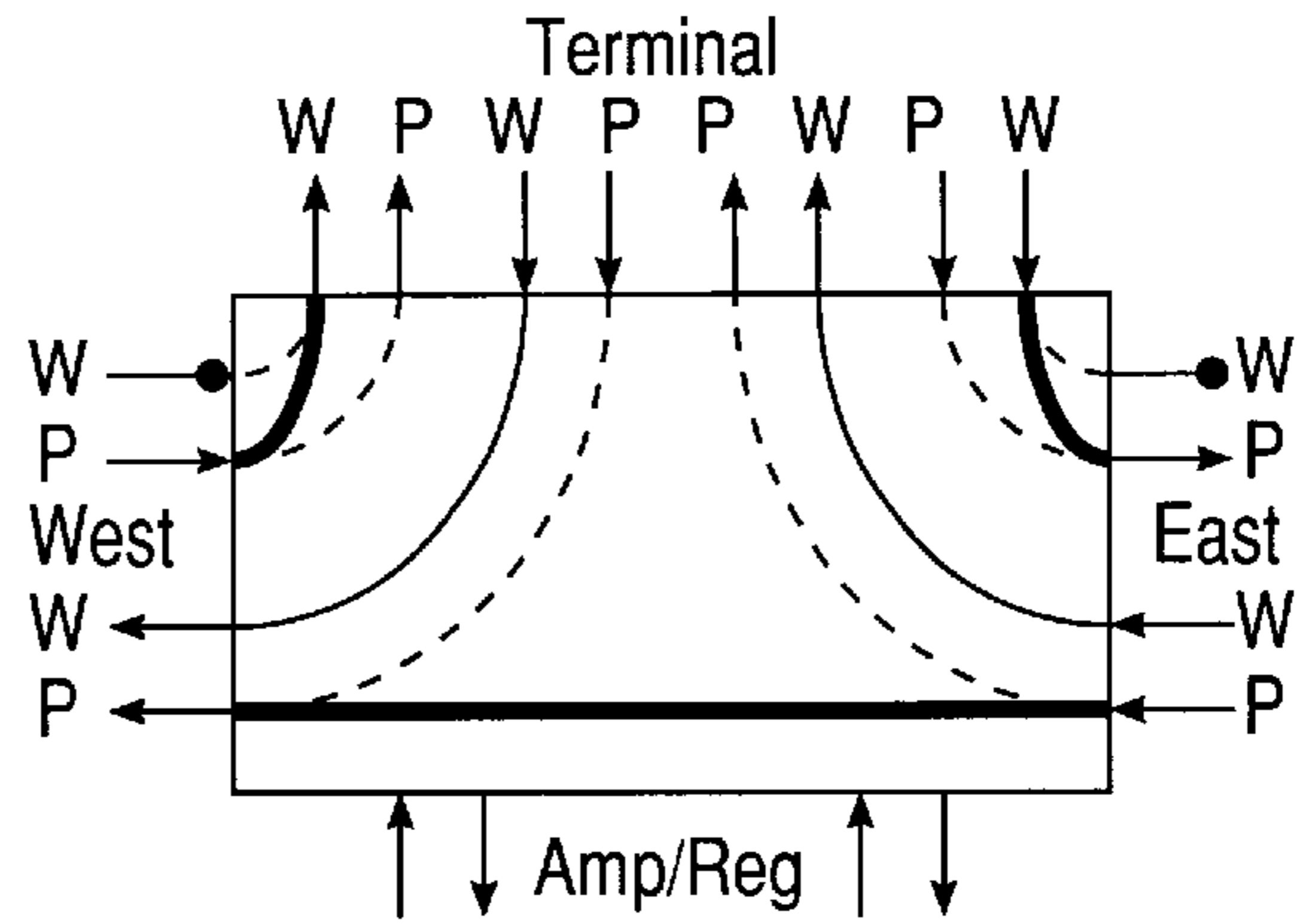
(iv) 8. P-Transit East-to-West. Span Switch West-In, East-Out
