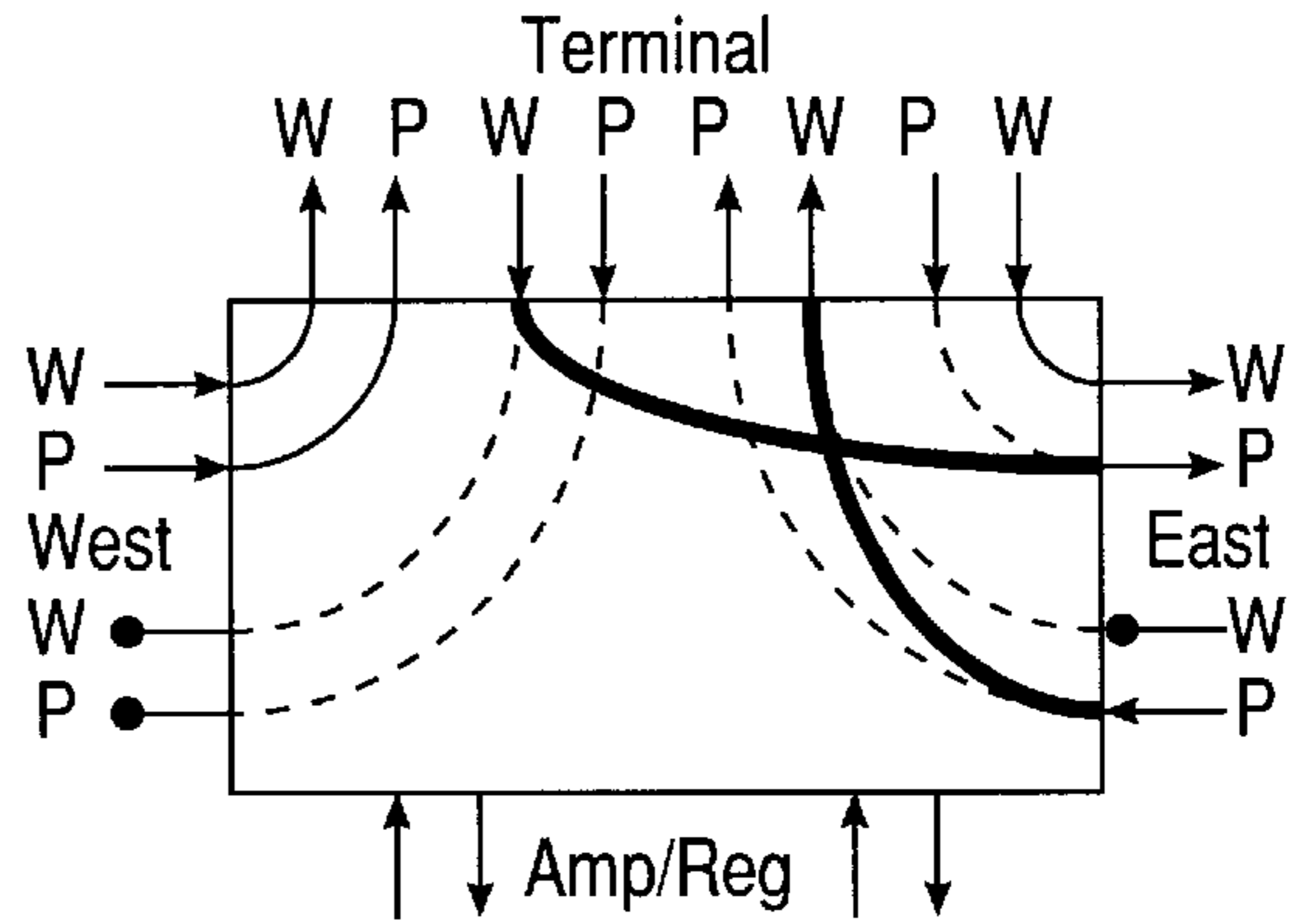
(iii) 18. Ring Switch East-Out. Span Switch East-In
