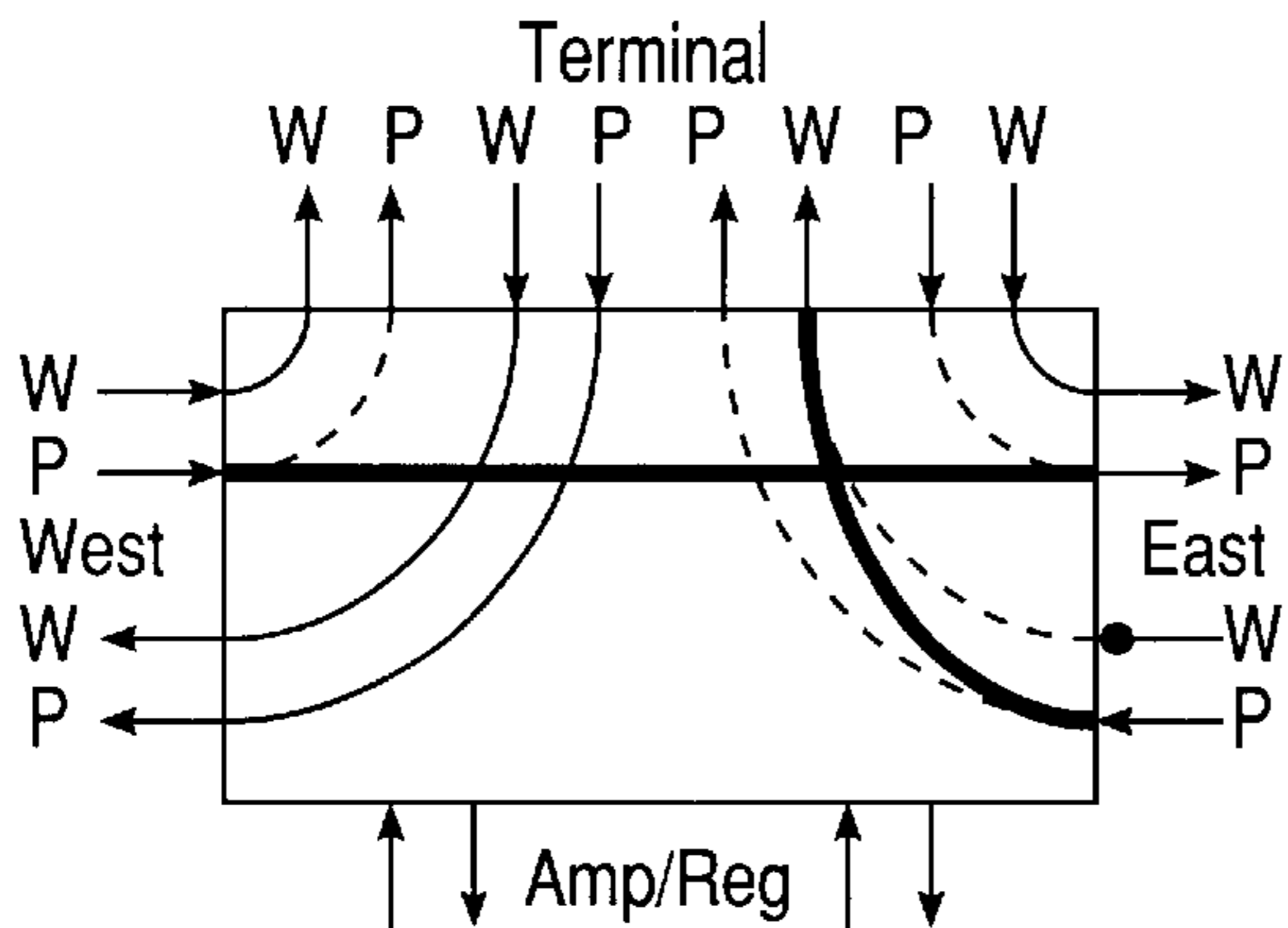
(iv) 3. P-Transit West-to-East, Span Switch East-In
