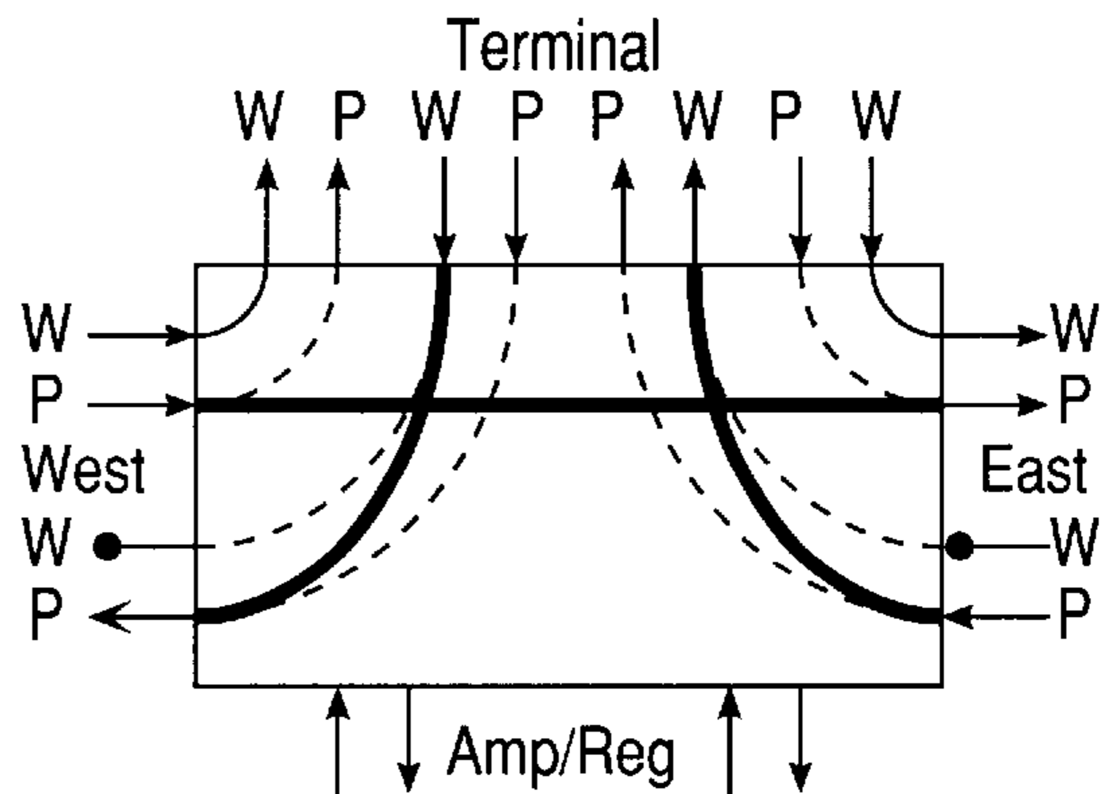
(iv) 4. P-Transit West-to-East, Span Switch West-Out, East-In
