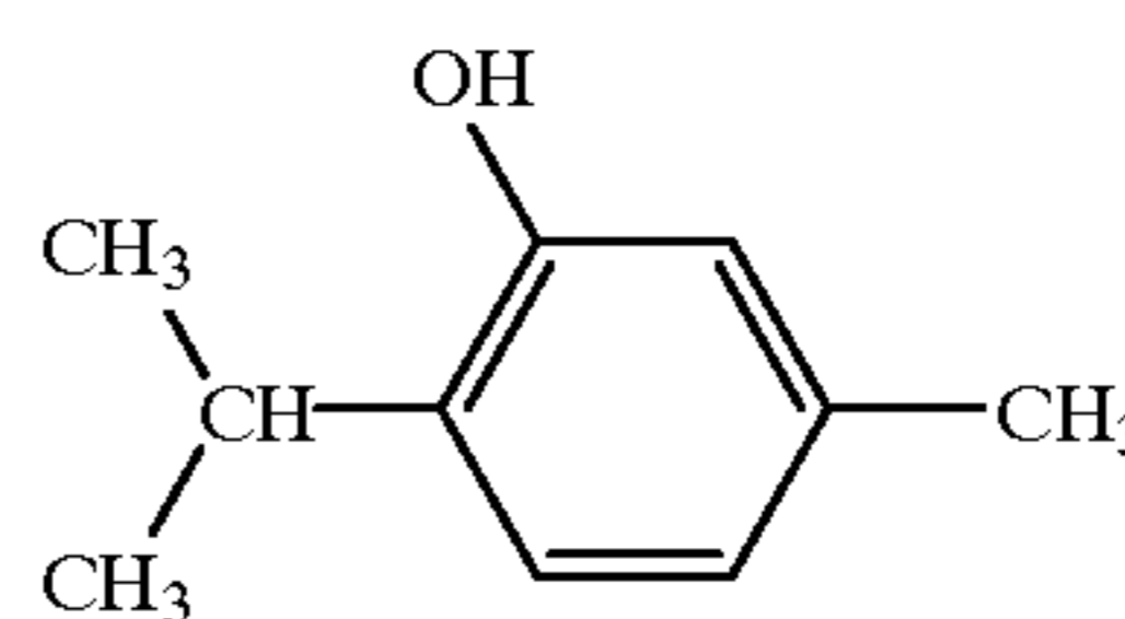
thymol
