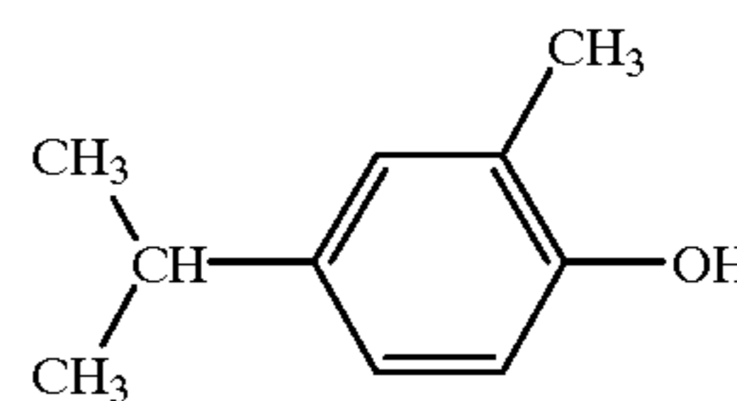
carvacrol
