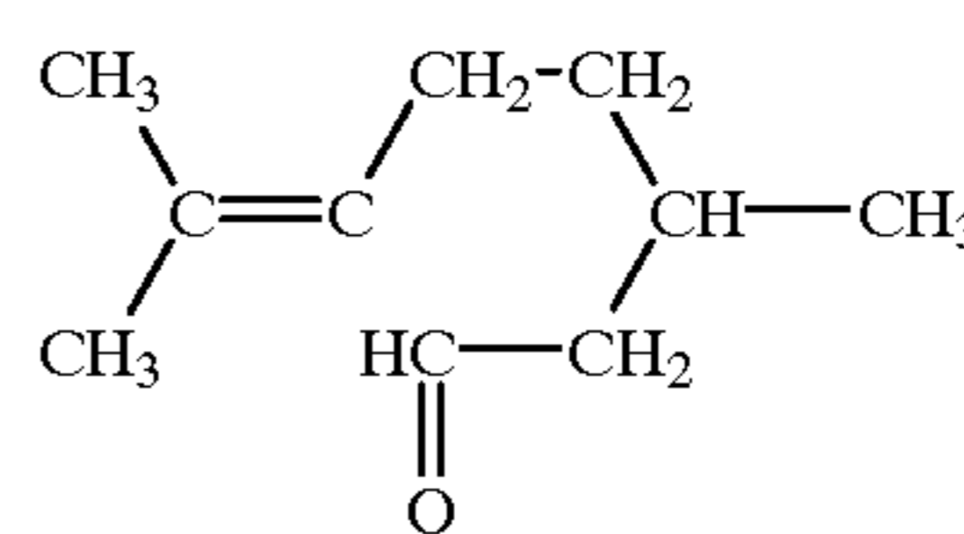
citronellal
