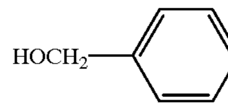
benzyl alcohol
