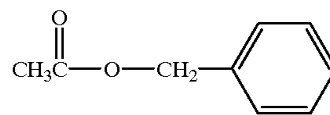
benzyl acetate
