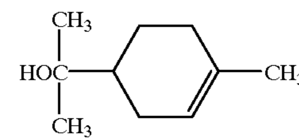
alpha-terpineol
