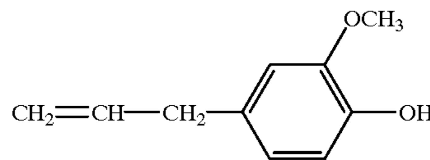
eugenol
