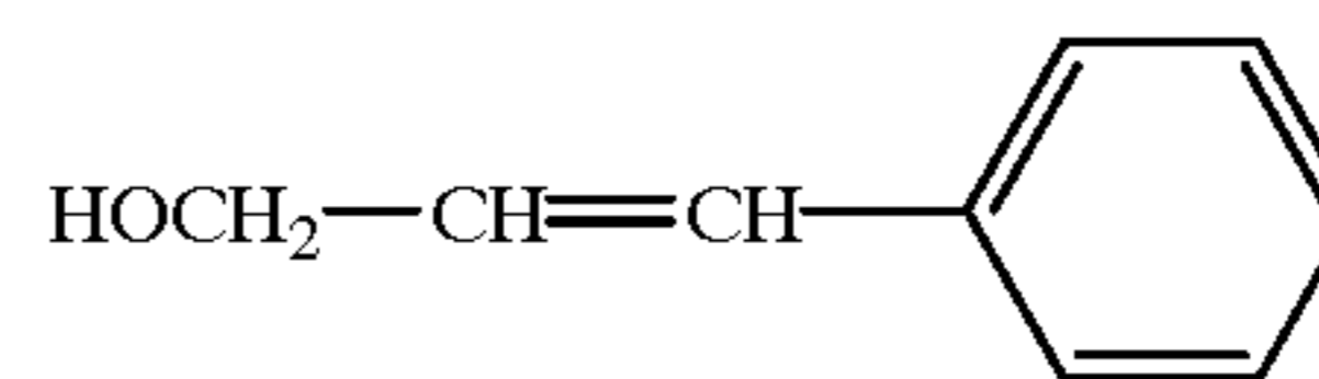
cinnamic alcohol
