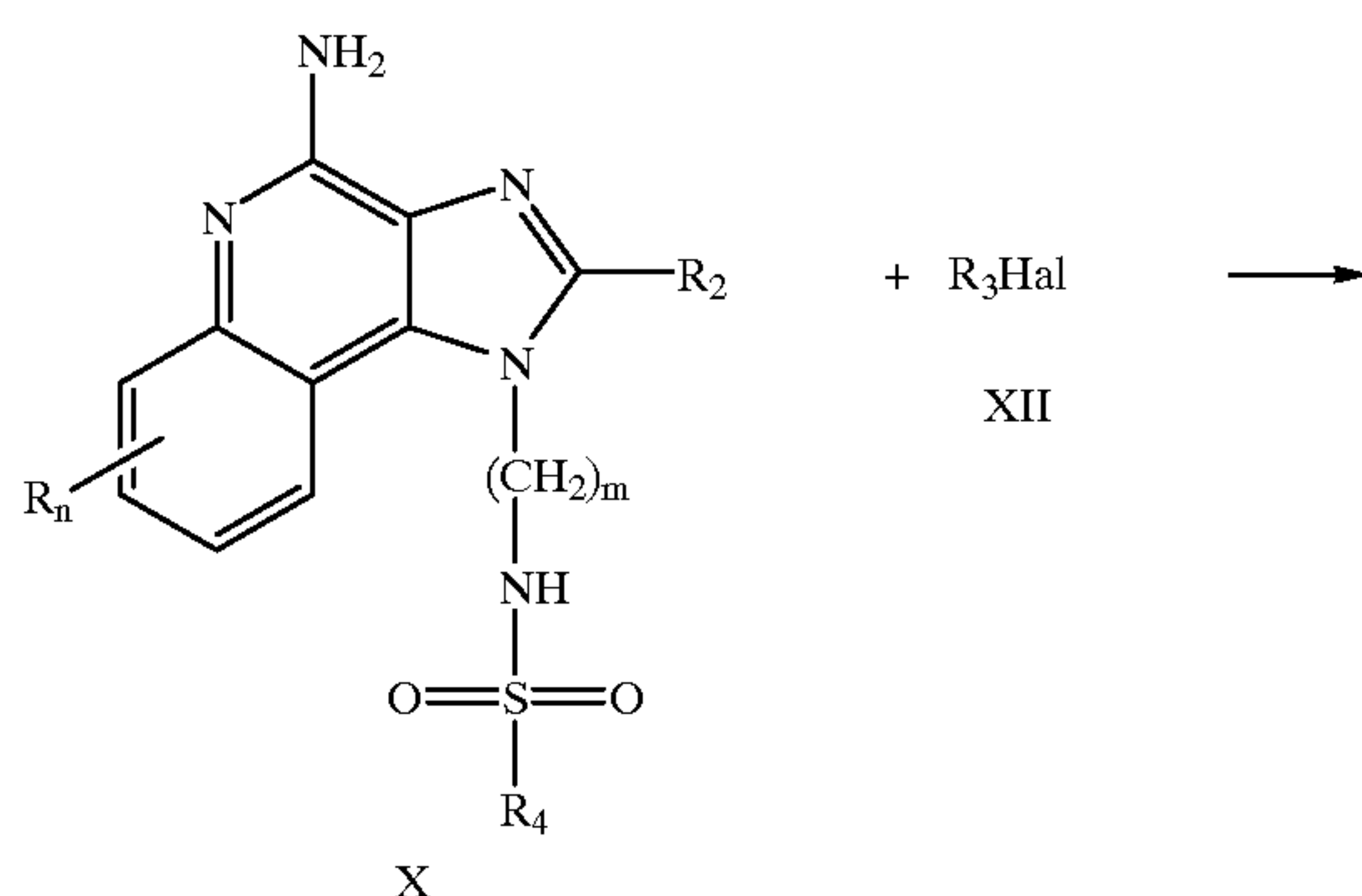
Reaction Scheme IV
