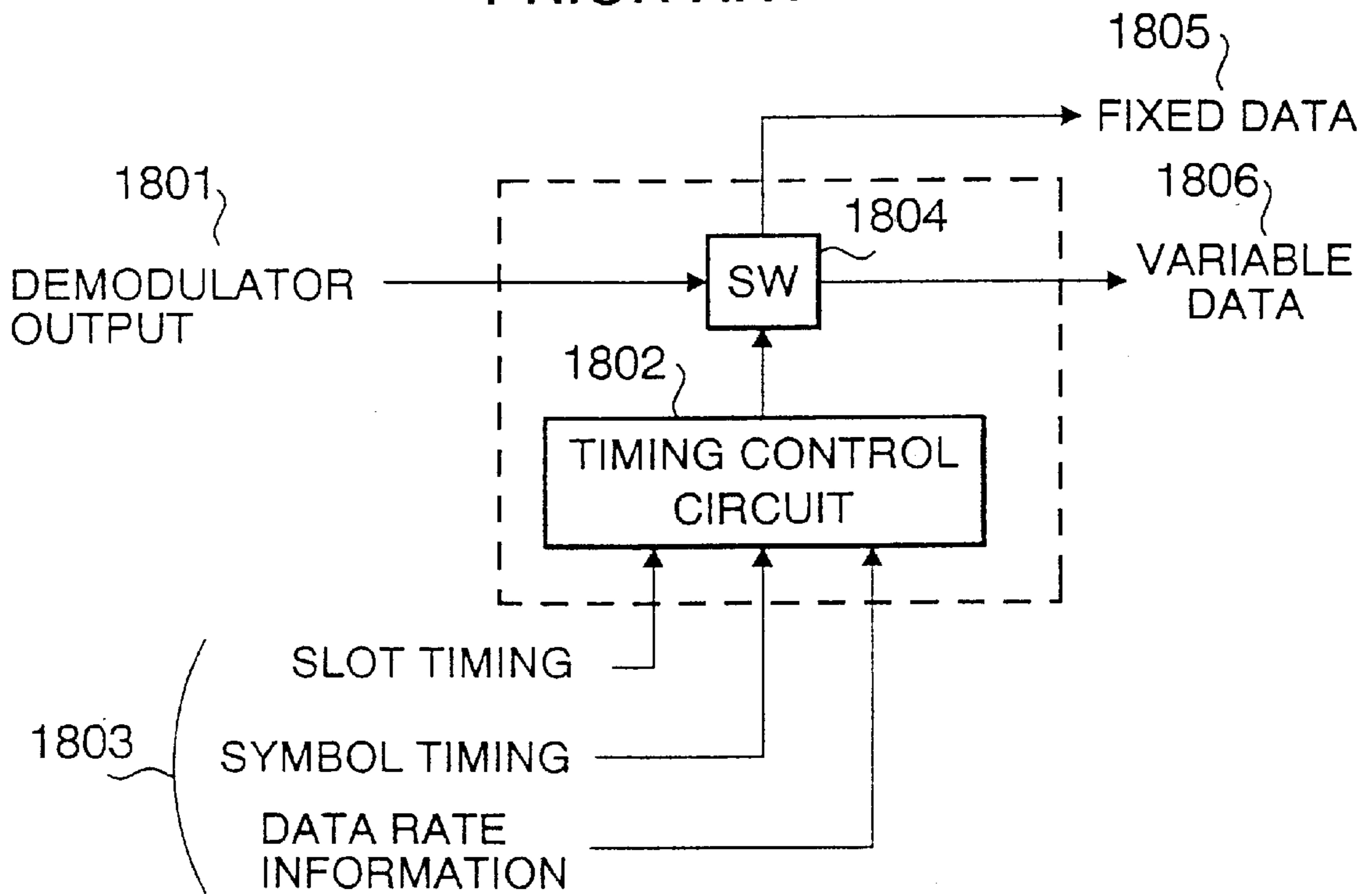
FIG. 7 PRIOR ART
