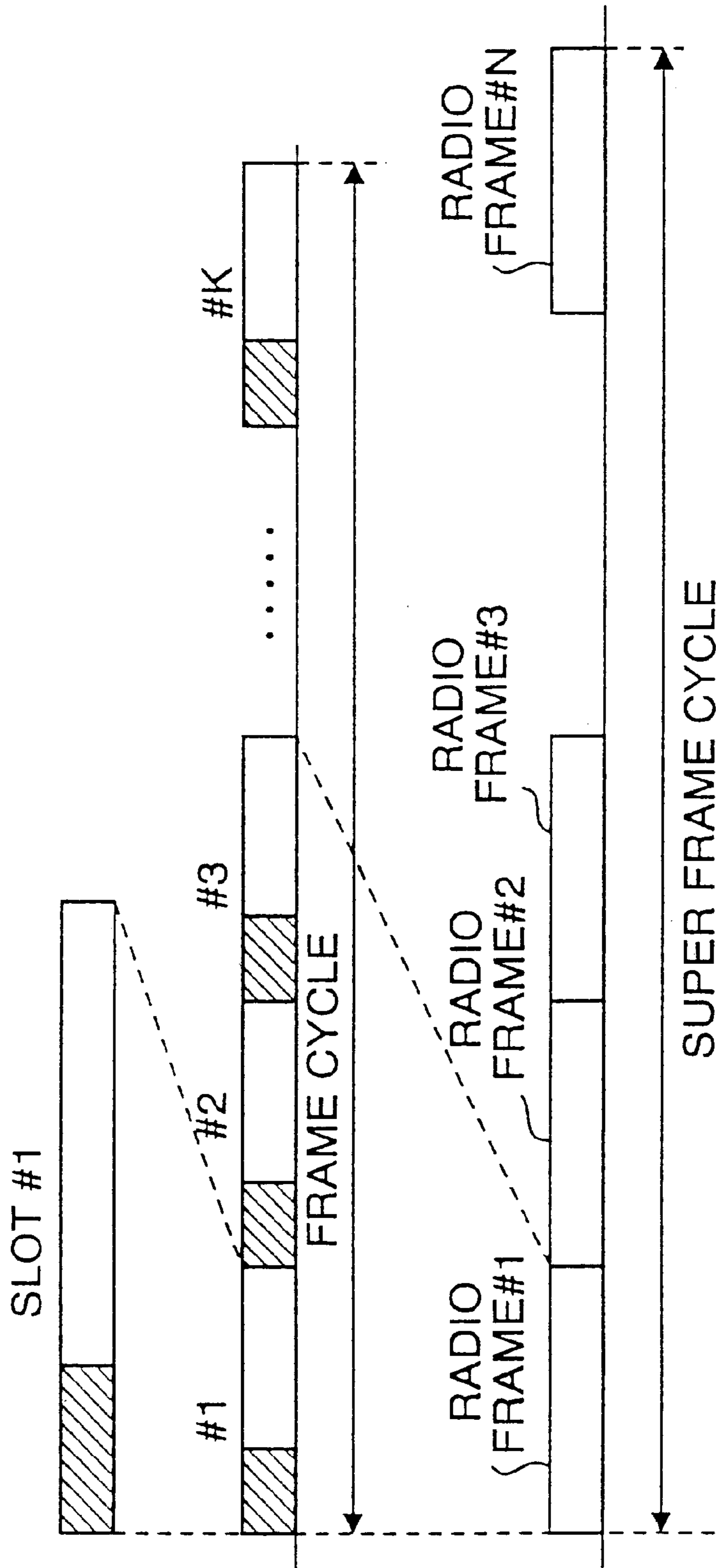
FIG. 3 PRIOR ART
