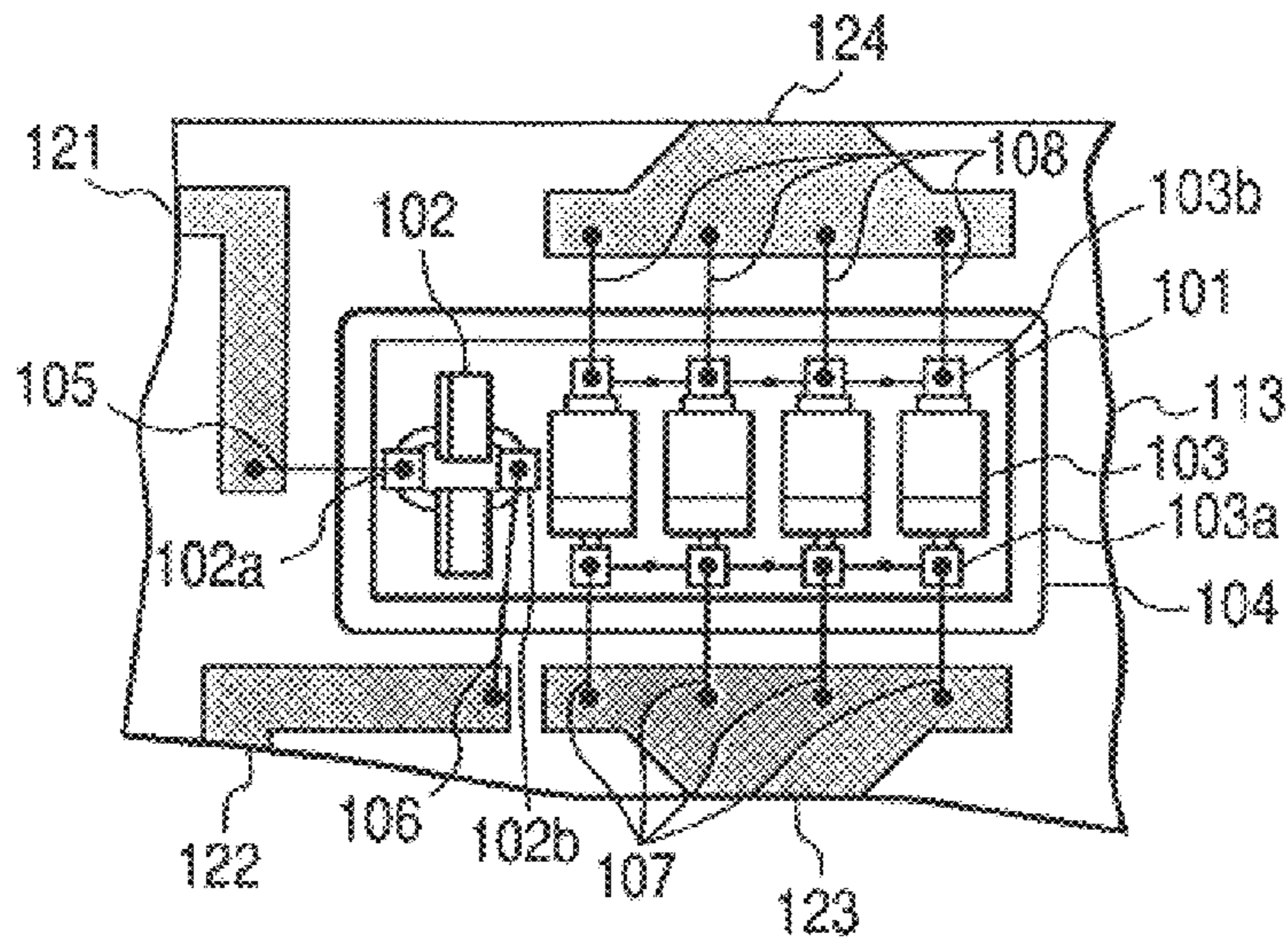
FIG. 21 PRIOR ART
