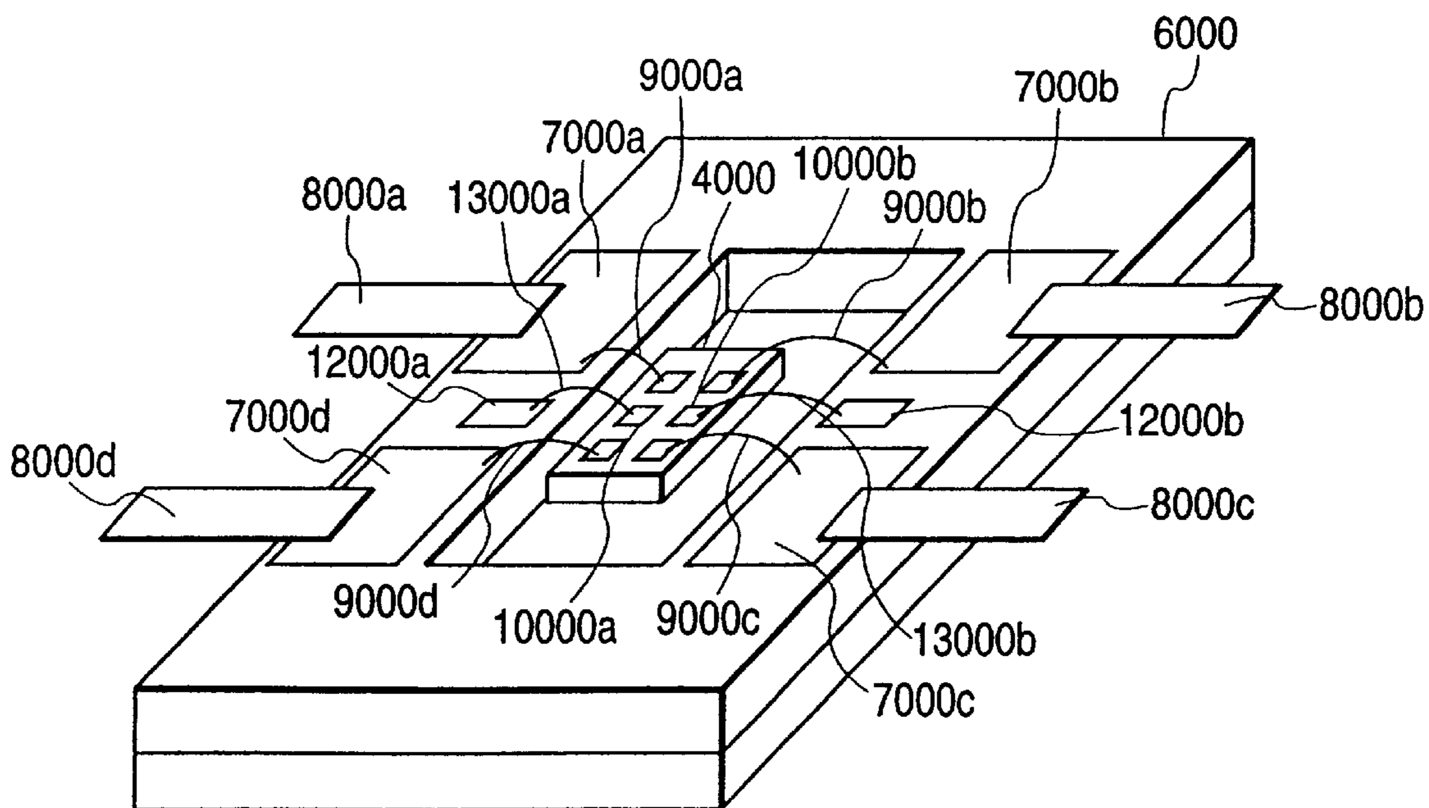
FIG. 22 PRIOR ART
