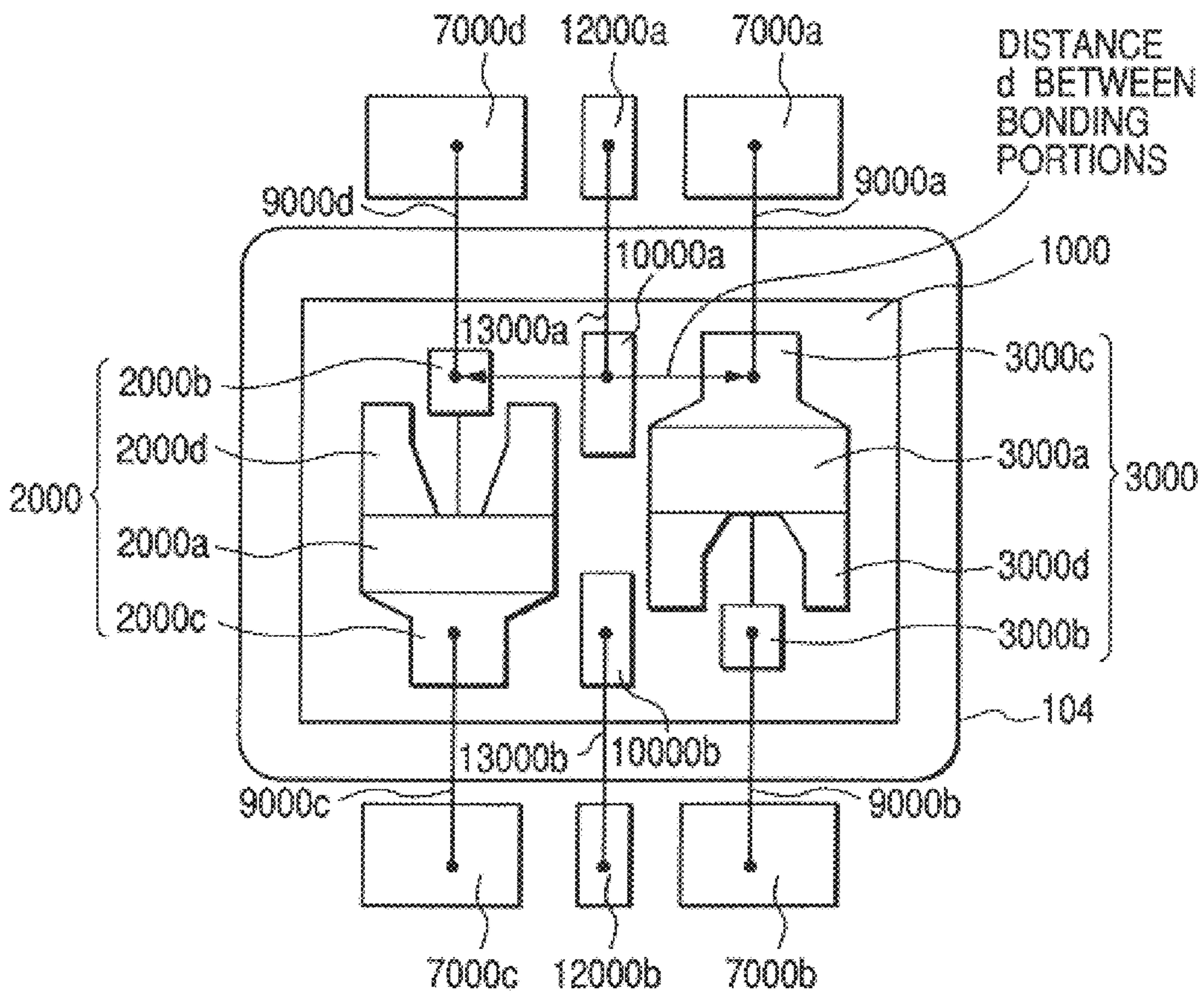
FIG. 21 PRIOR ART
