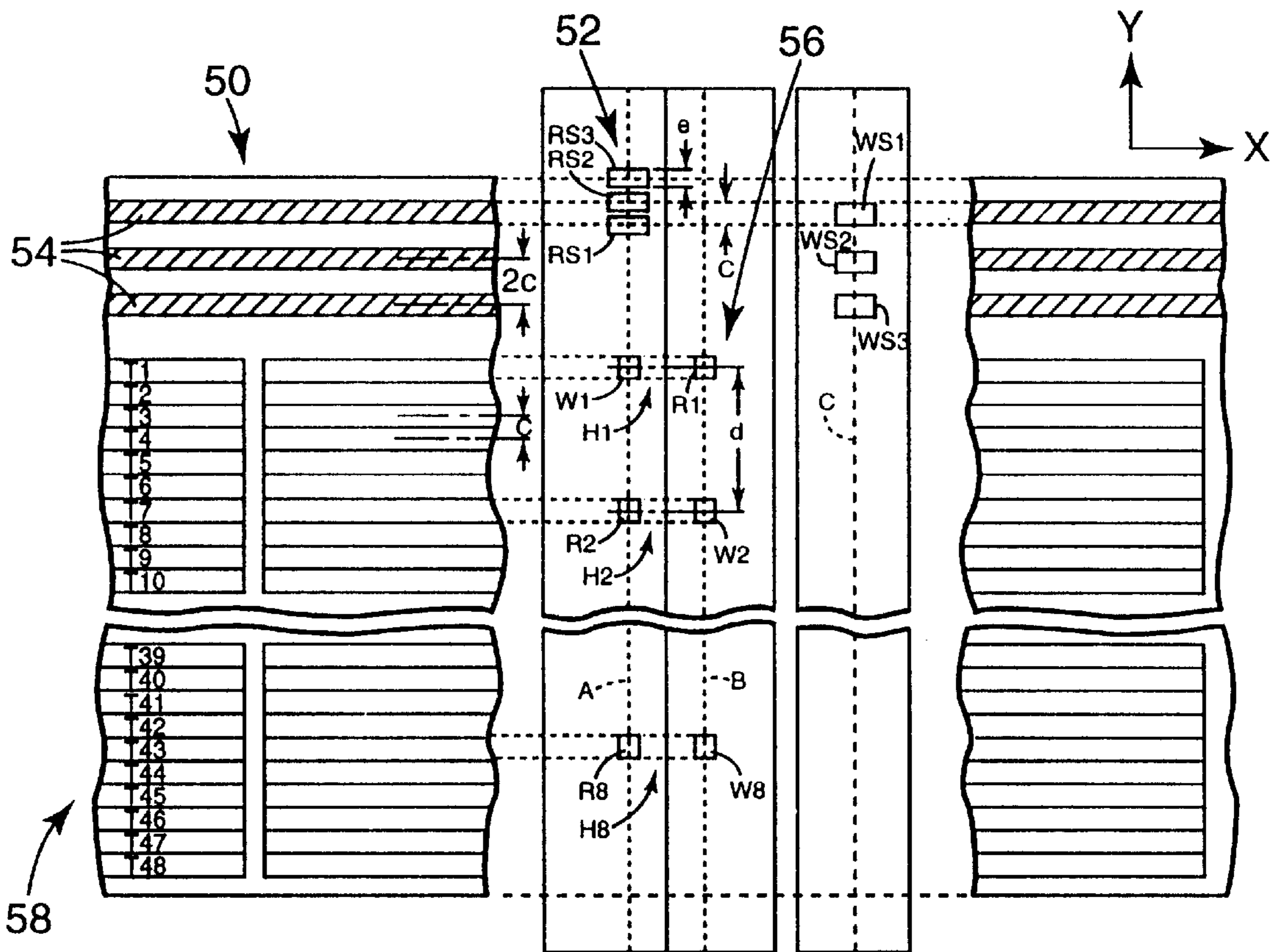
Fig. 5 (PRIOR ART)
