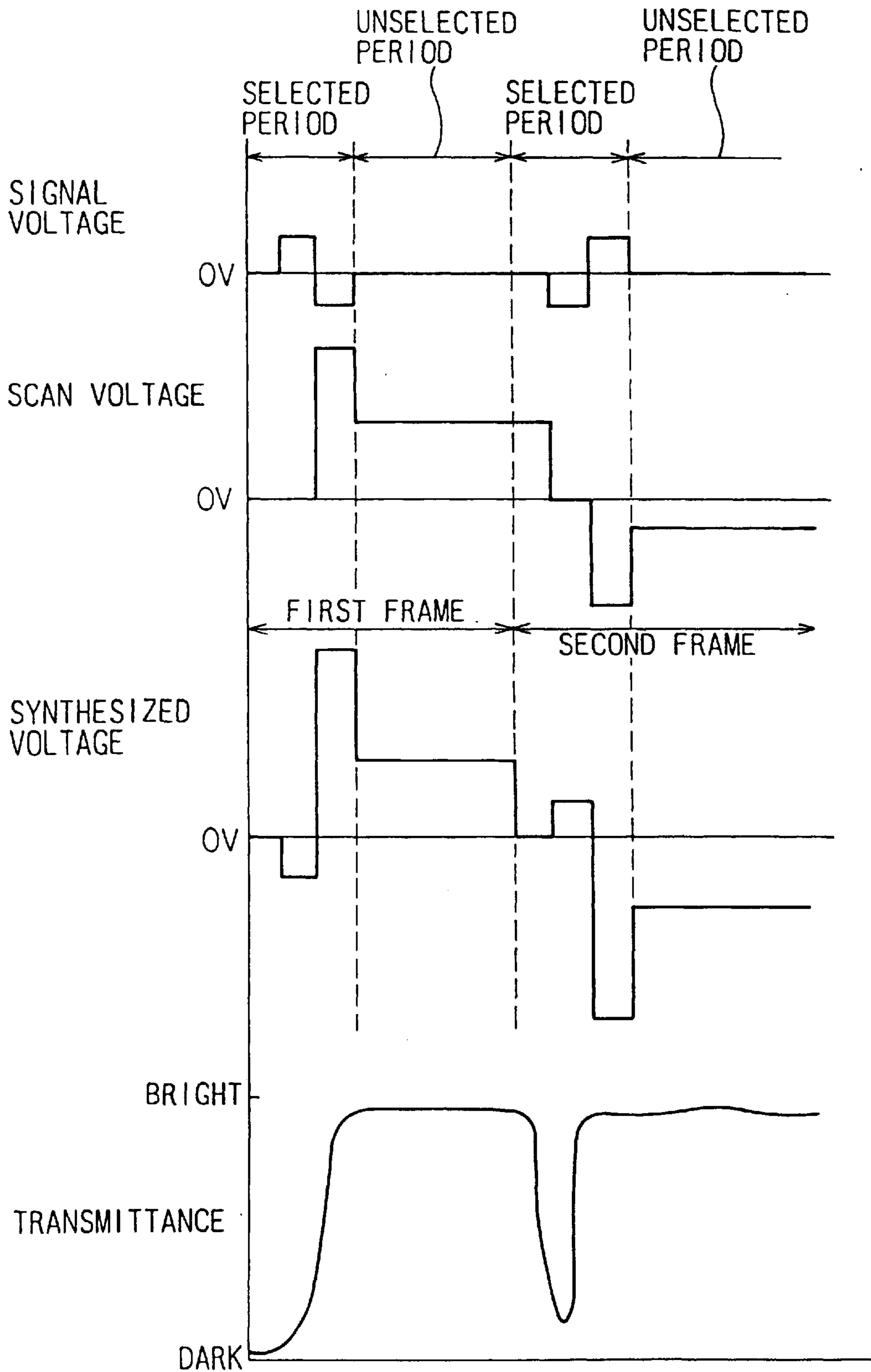
Fig. 6 PRIOR ART
