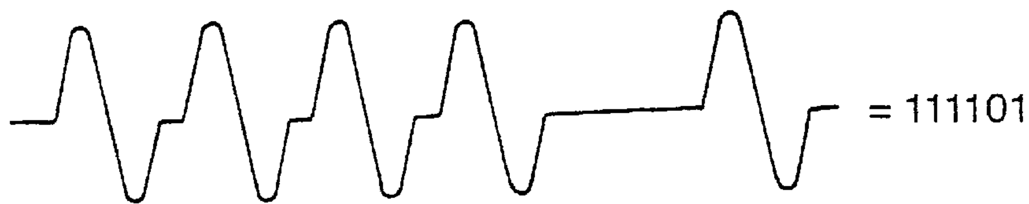
TYPICAL DETECTED OUTPUT FROM READER (ADC INPUT)
