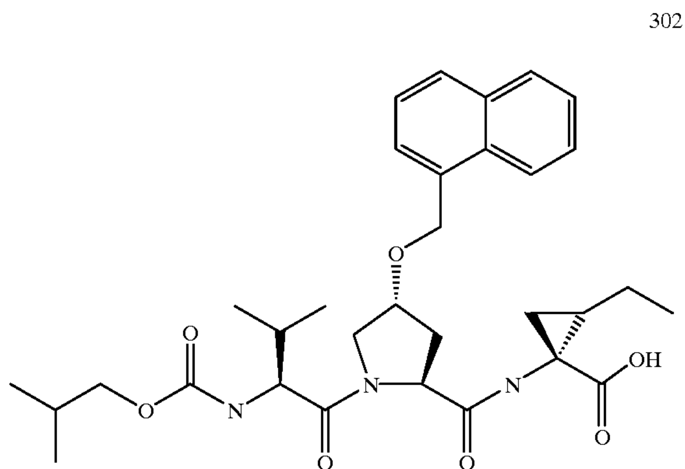
Synthesis of compound 302
