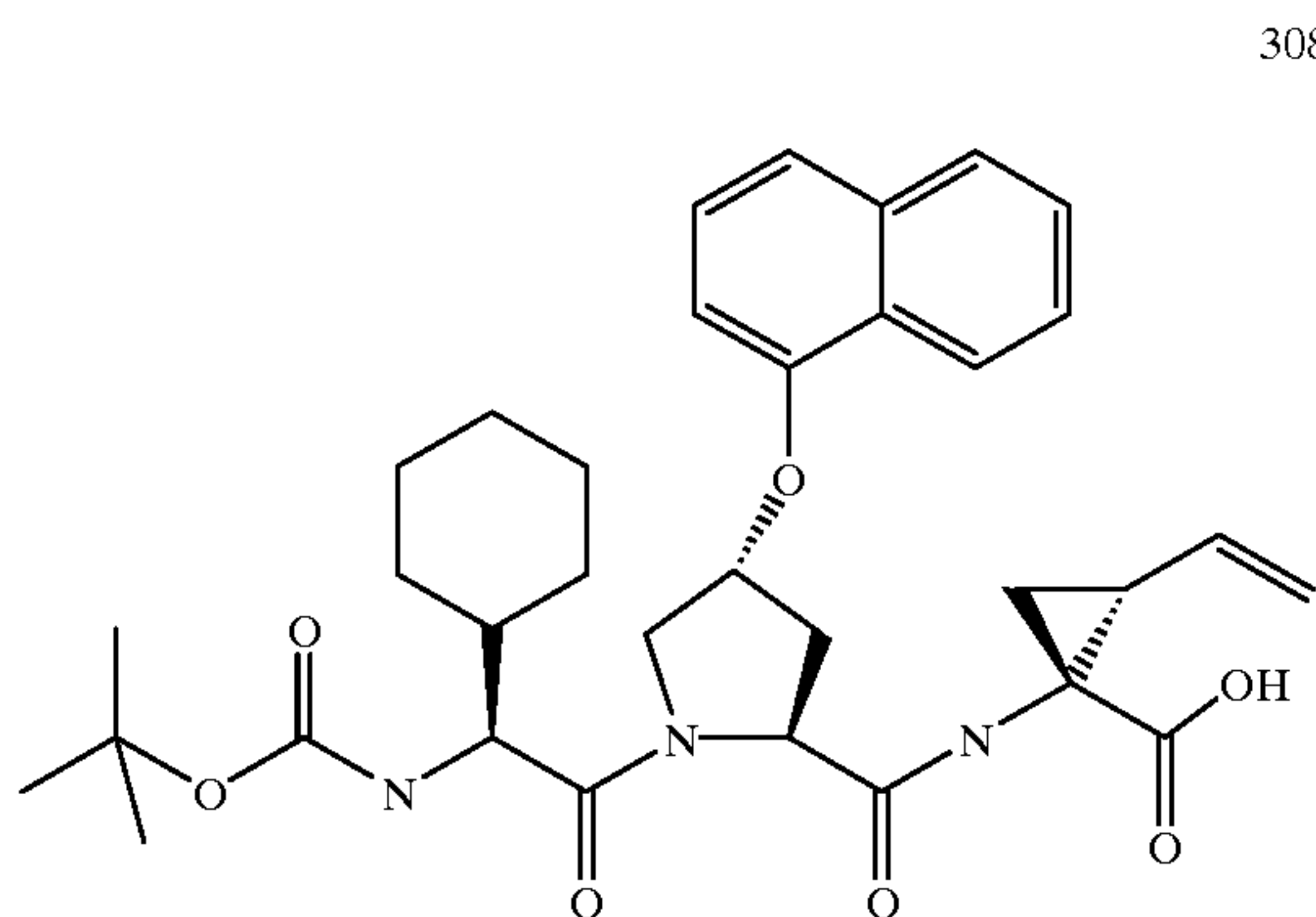
Synthesis of compound 308
