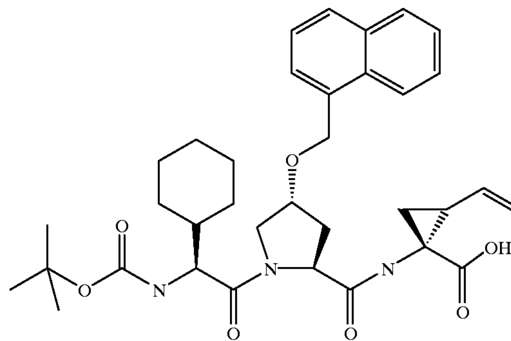
Synthesis of compound 305
