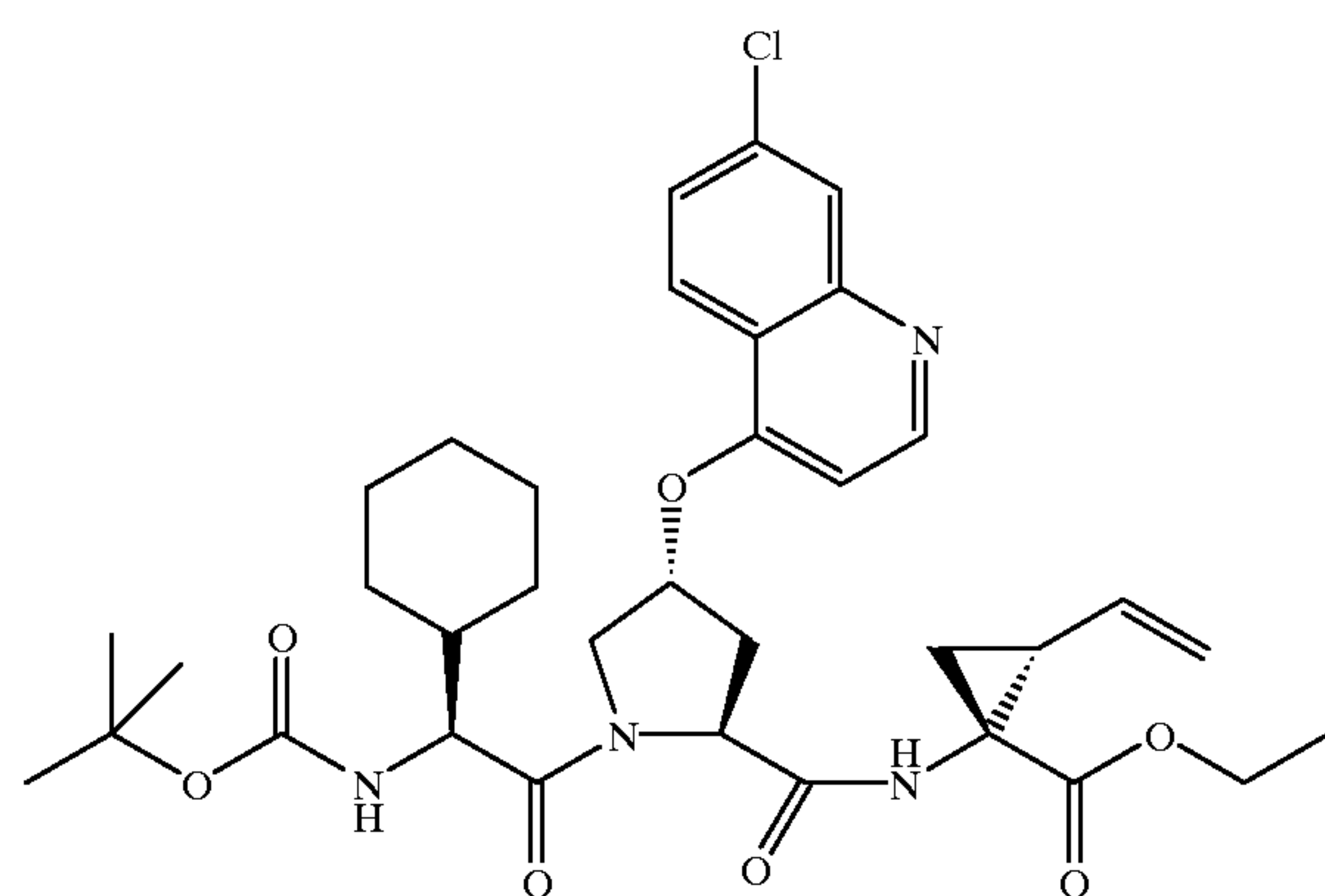
Synthesis of compound 311
