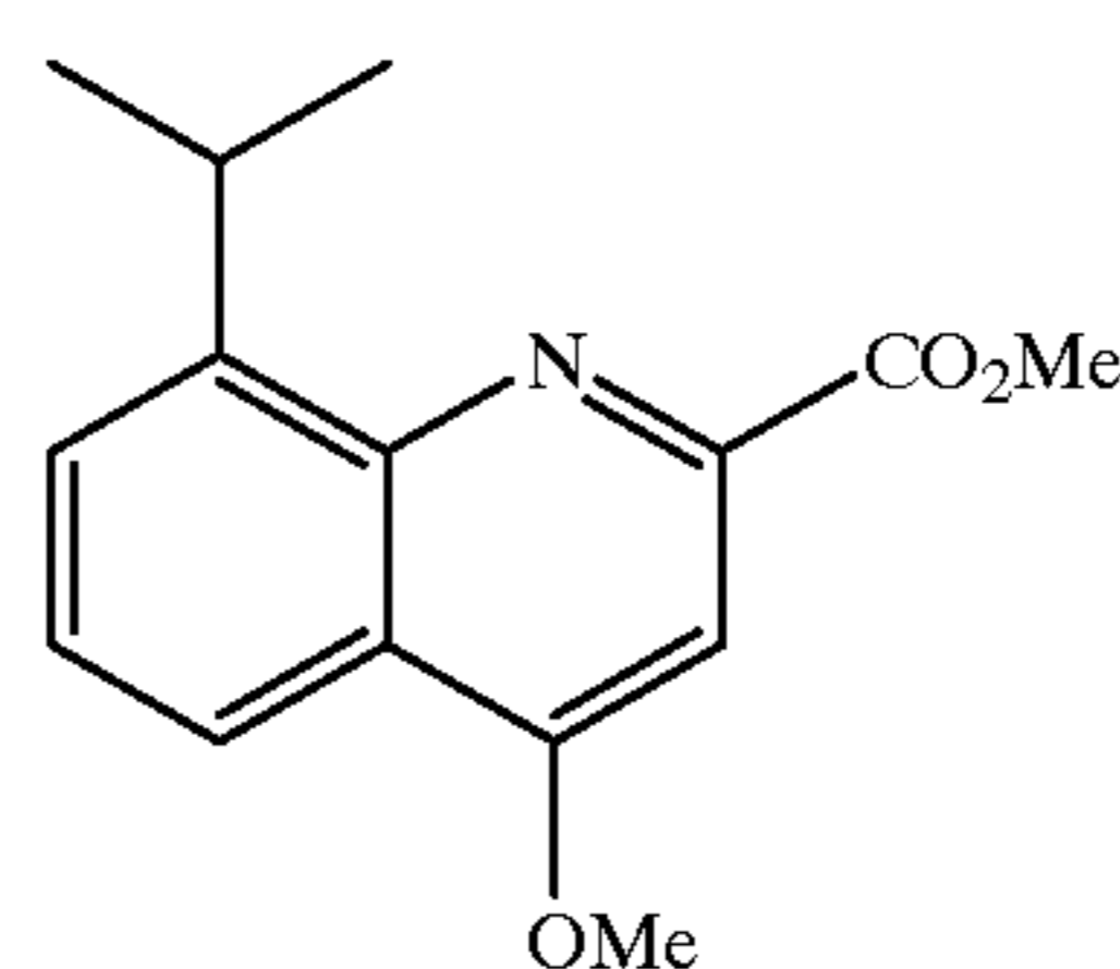
Methyl 8-isopropyl-4-methoxyquinoline-2-carboxylate
