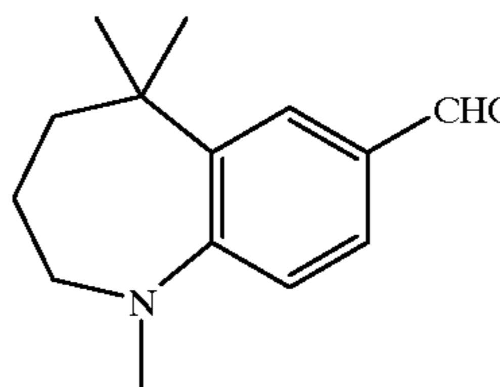
1,5,15-Trimethyl-2,3,4,5-tetrahydro-1H-benzazepine-7-carbaldehyde
