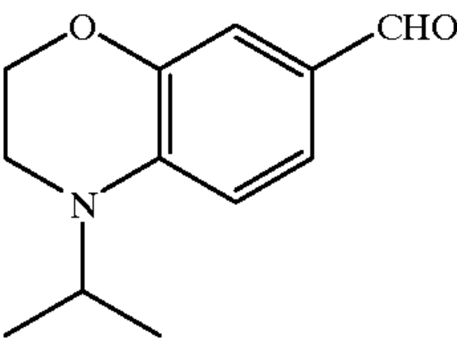
4-Isopropyl-3,4-dihydro-2H-1,4-benzoxazine-7-carbaldehyde
