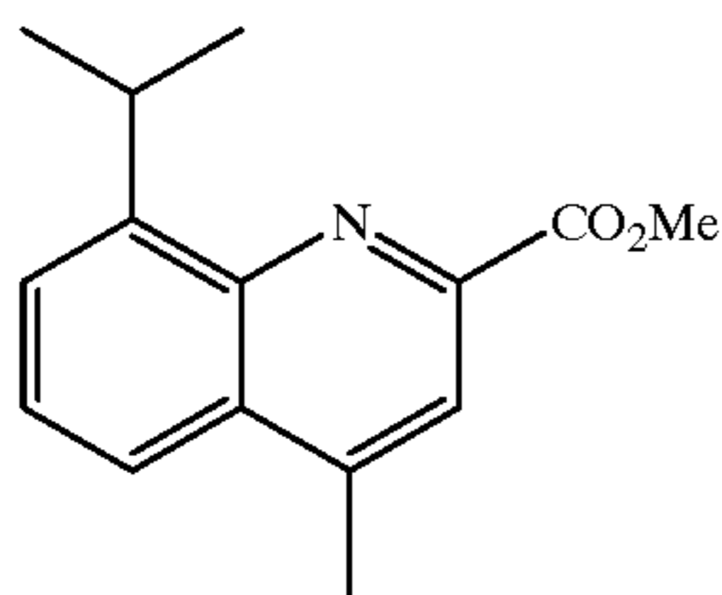
Methyl 8-isopropyl-4-methylquinoline-2-carboxylate
