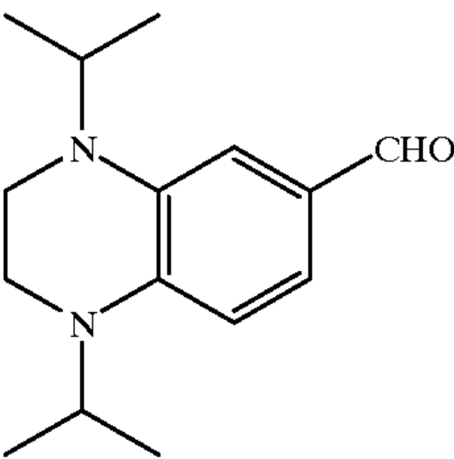
1,4-Diisopropyl-1,2,3,4-tetrahydroquinoxaline-6-carbaldehyde
