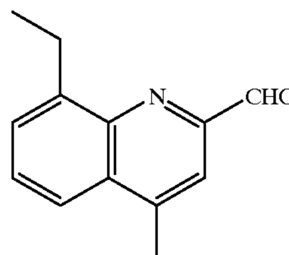
8-Ethyl-4-methylquinoxaline-2-carbaldehyde
