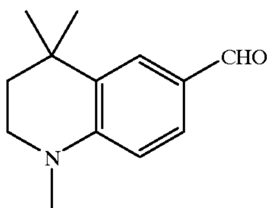
1,4,4-Trimethyl-1,2,3,4-tetrahydroquinoline-6-carbaldehyde
