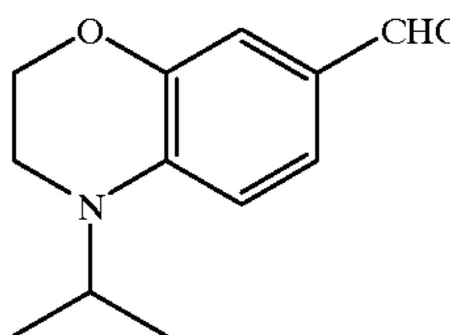
4-Isopropyl-3,4-dihydro-2H-1,4-benzoxazine-7-carbaldehyde
