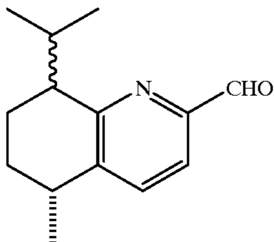
8-Isopropyl-5-methyl-1,5,6,7,8-tetrahydroquinoline-2-carbaldehyde
