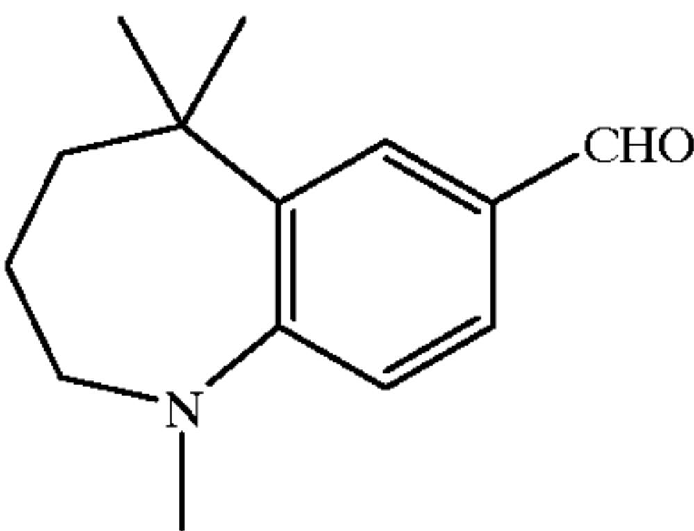
1,515-Trimethyl-2,3,4,5-teatrahydro-1H-benzazepine-7-carbaldehyde
