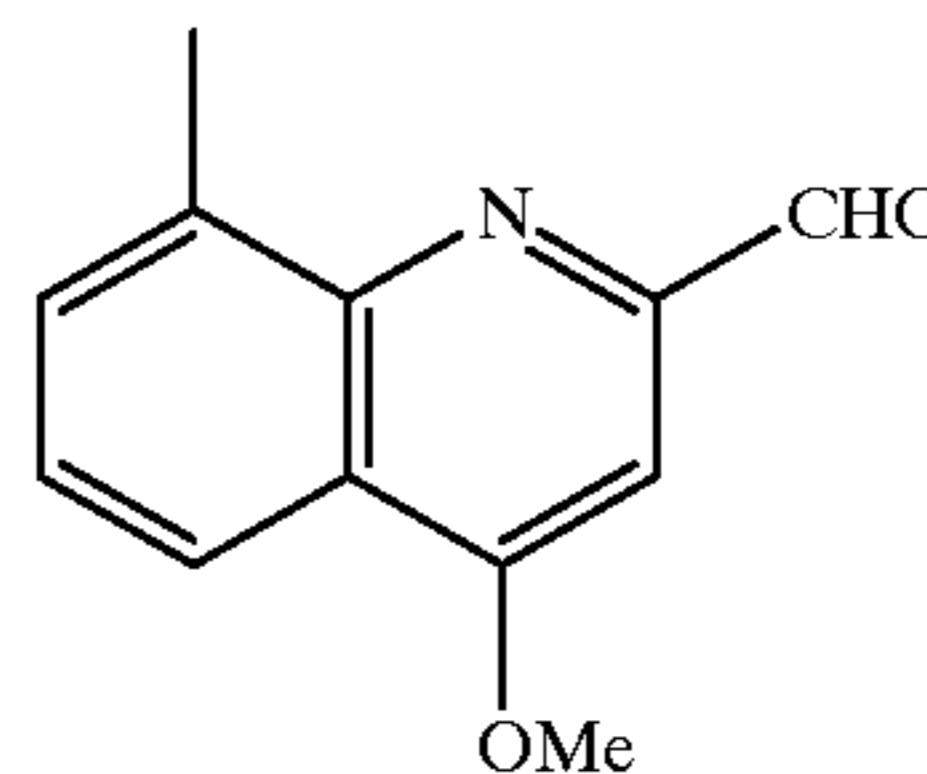
4-Methoxy-8-methylquinoxaline-2-carbaldehyde
