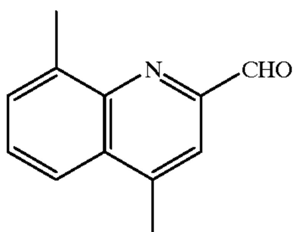
4,8-Dimethylquinoxaline-2-carbaldehyde
