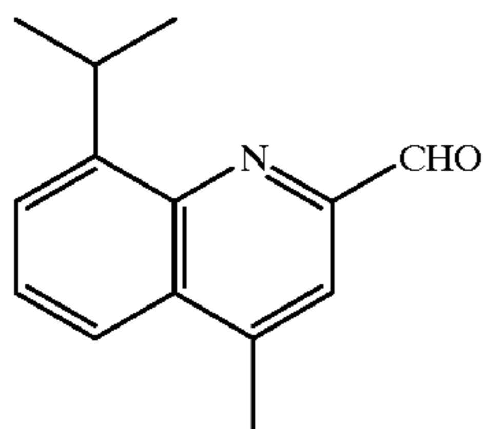
8-Isopropyl-4-methylquinoline-2-carbaldehyde
