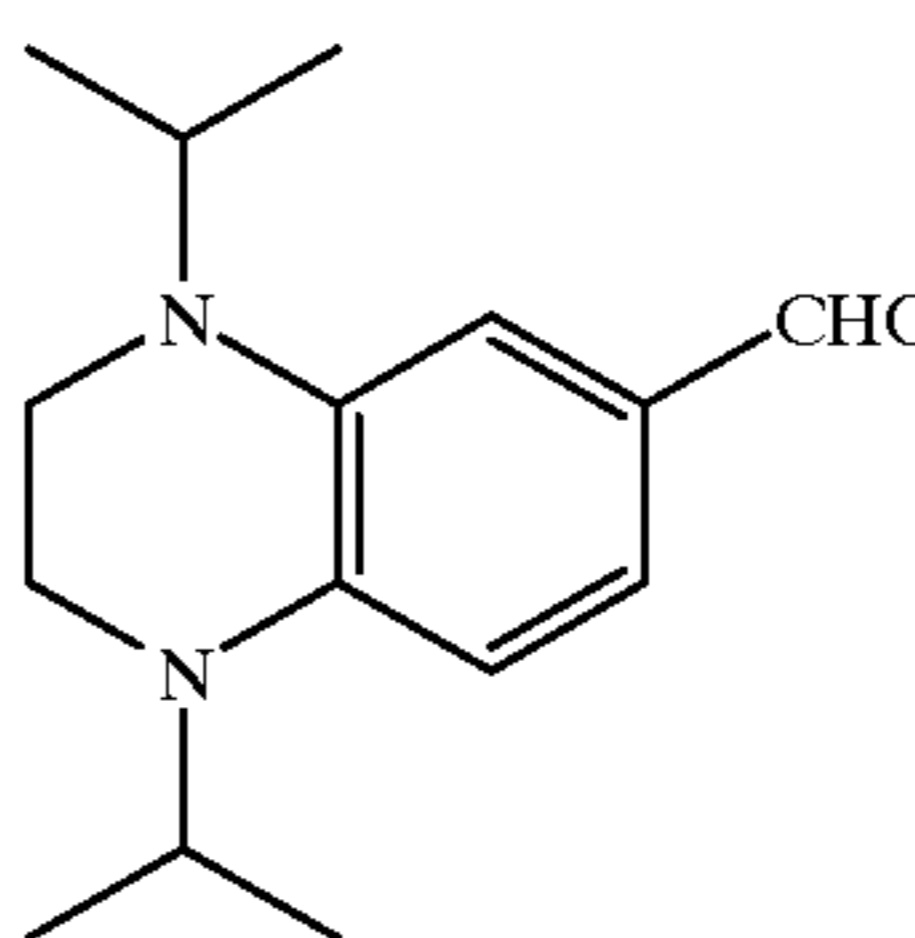
1,4-Diisopropyl-1,2,3,4-tetrahydroquinoxaline-6-carbaldehyde
