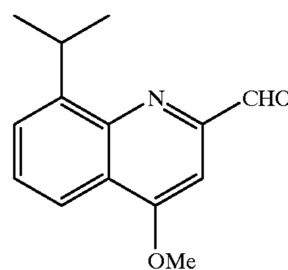
8-Isopropyl-4-methoxyquinoline-2-carbaldehyde
