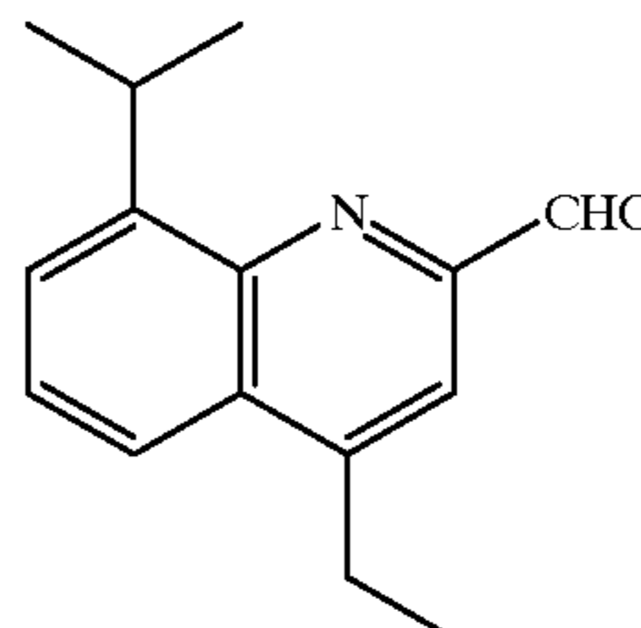
4-Ethyl-8-isopropylquinoxaline-2-carbaldehyde
