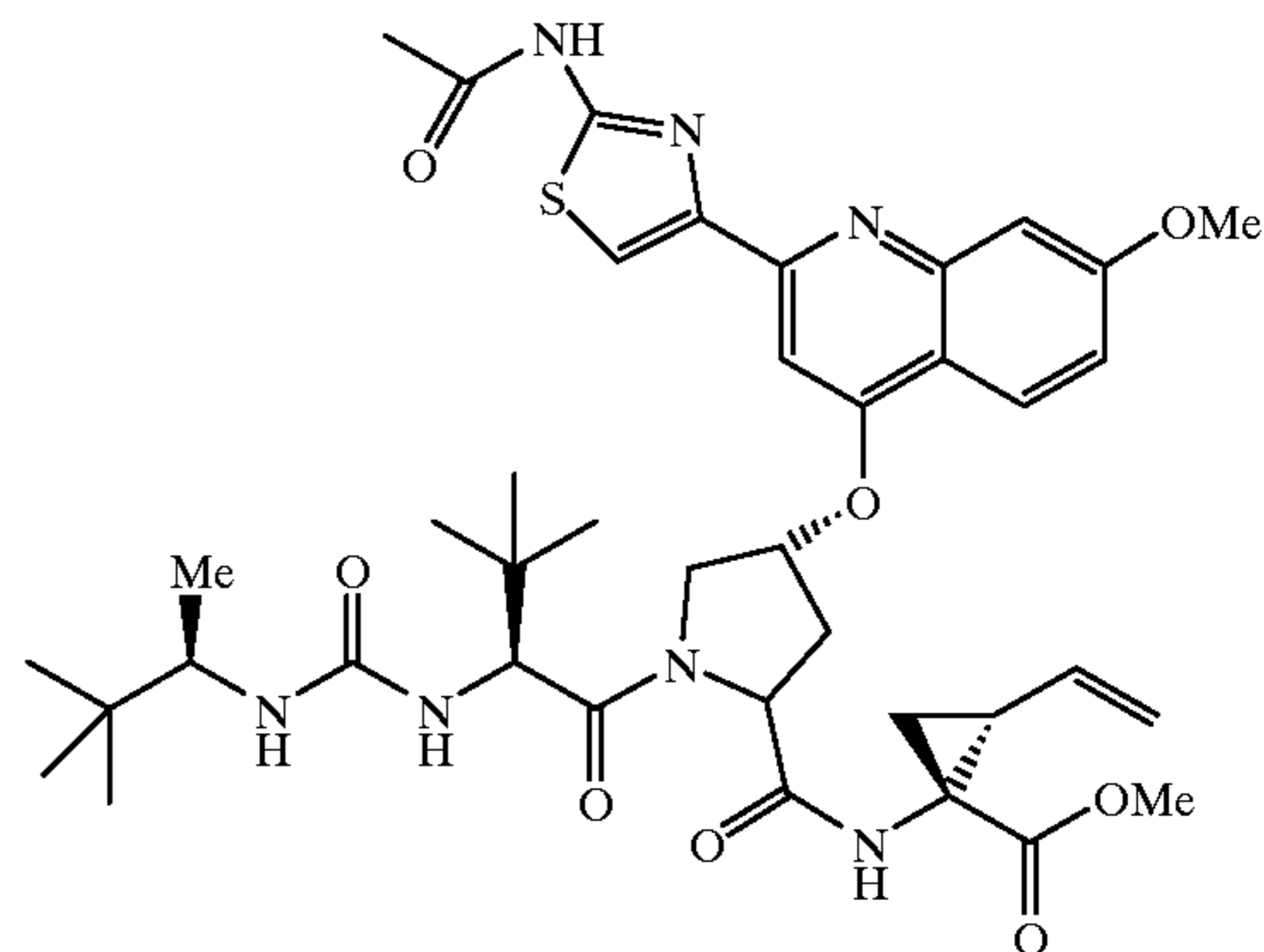
compound 333
