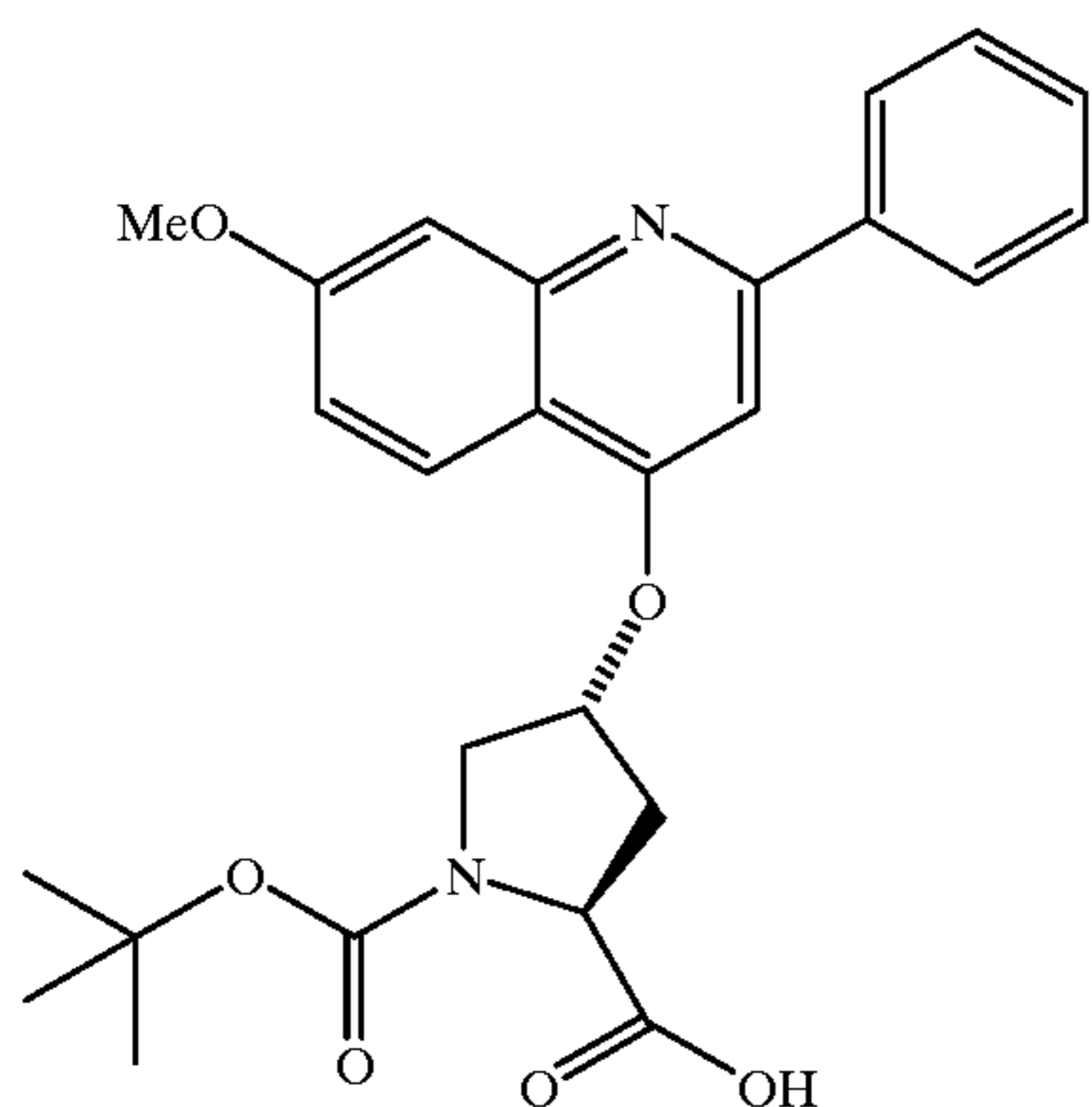
Boc-4(R)-(2-phenyl-7-methoxyquinoline-4-oxo)proline (7)
