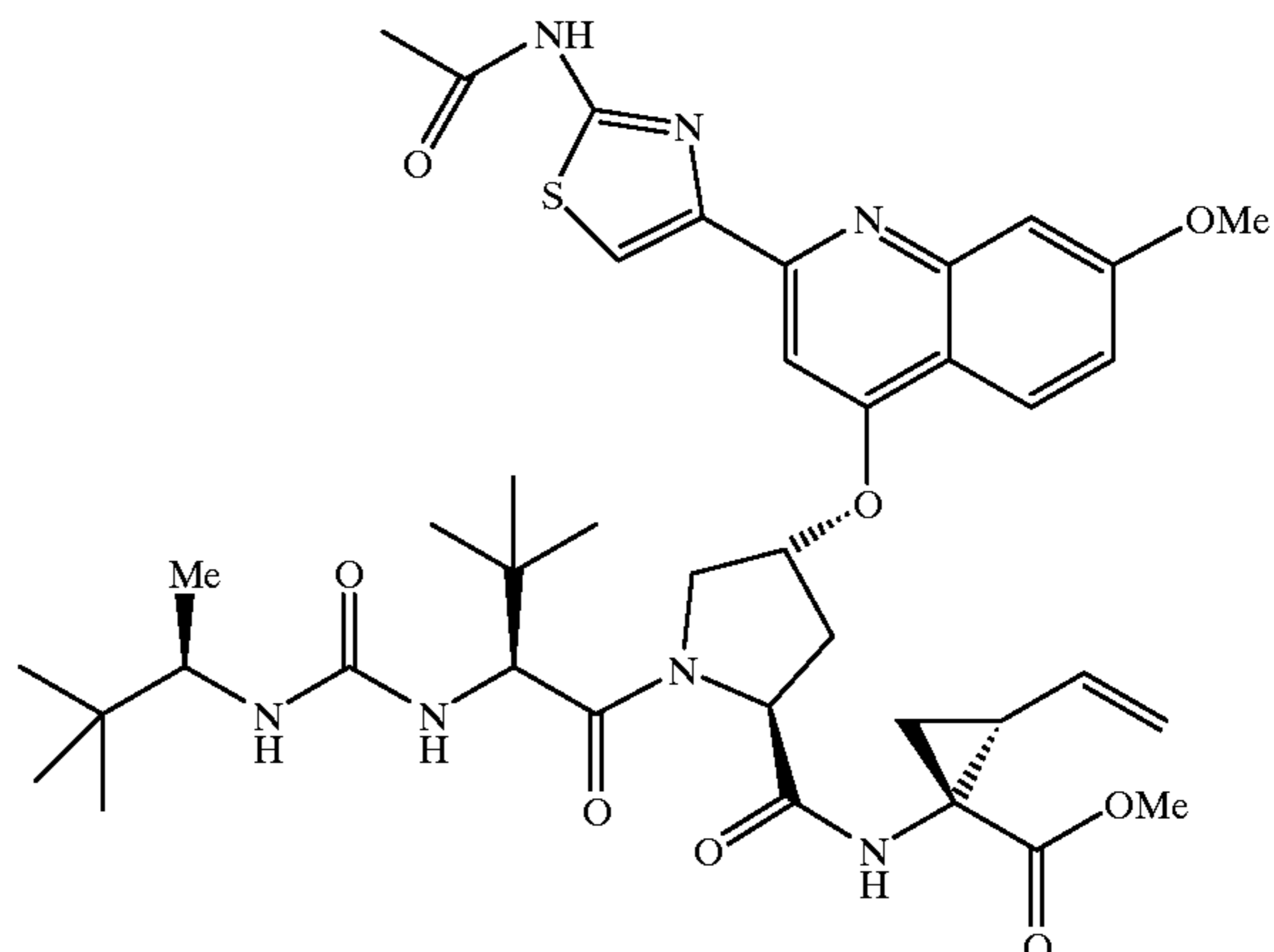
(35q)
