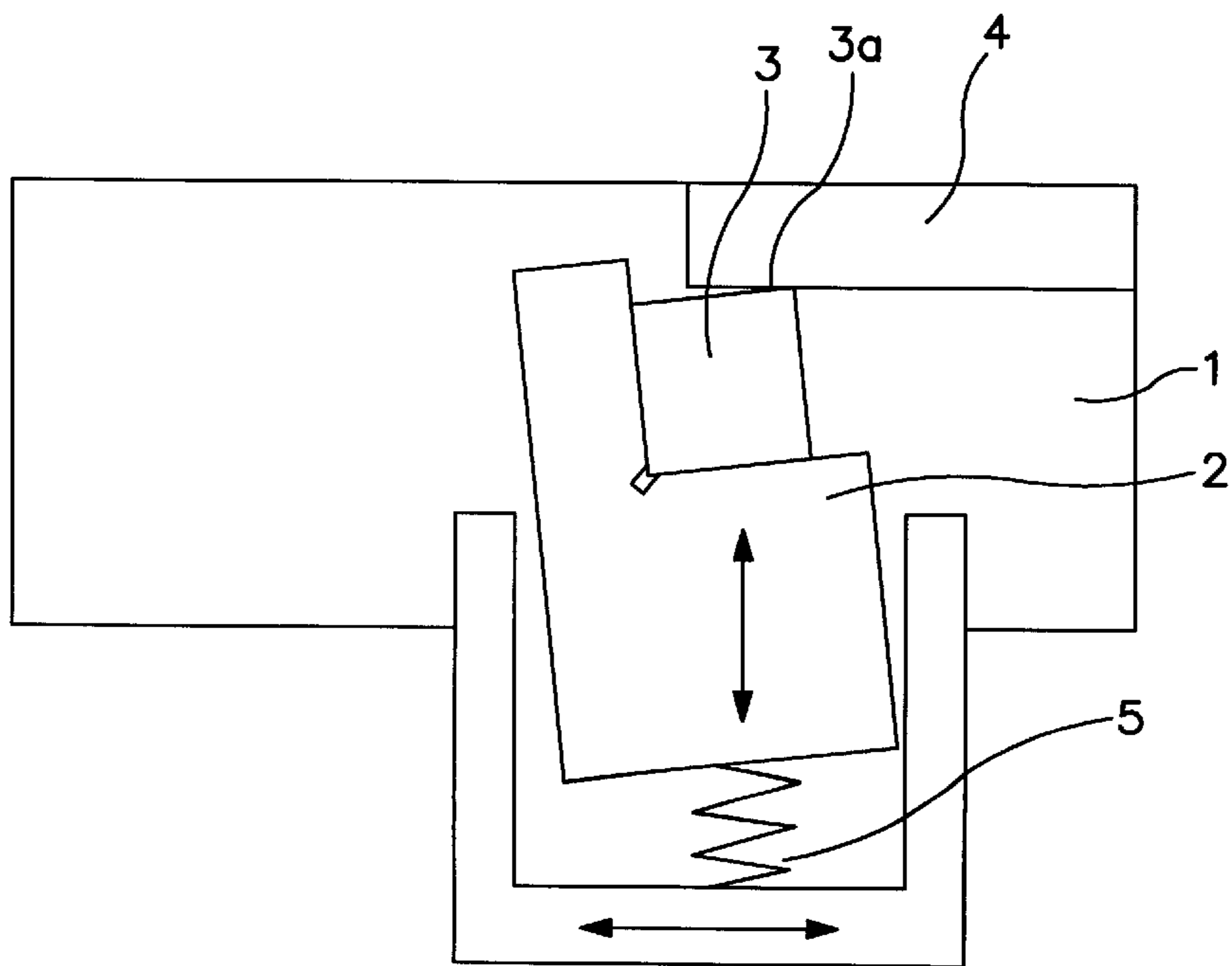
FIG. 9 PRIOR ART
