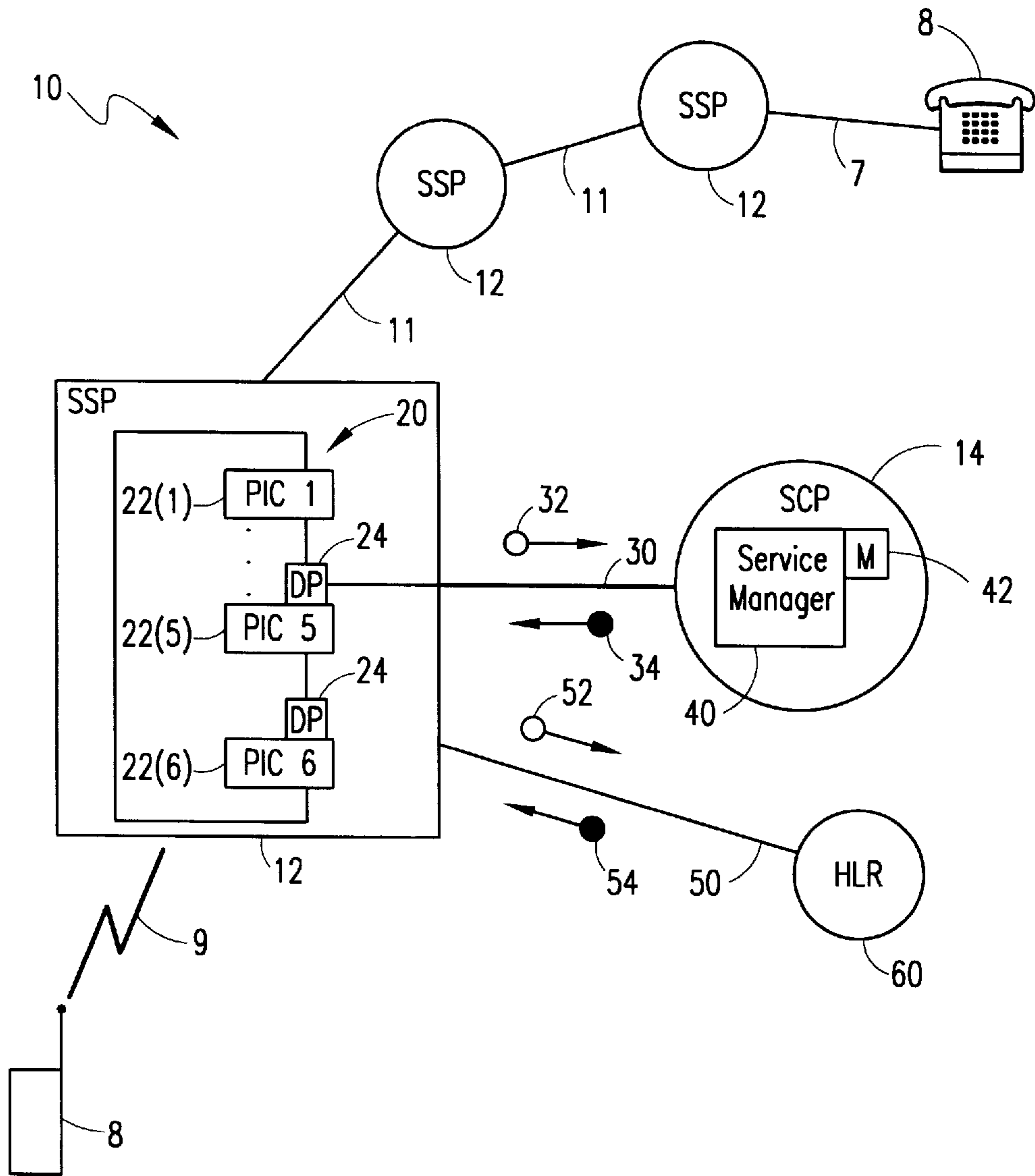
FIG. 1 (PRIOR ART)
