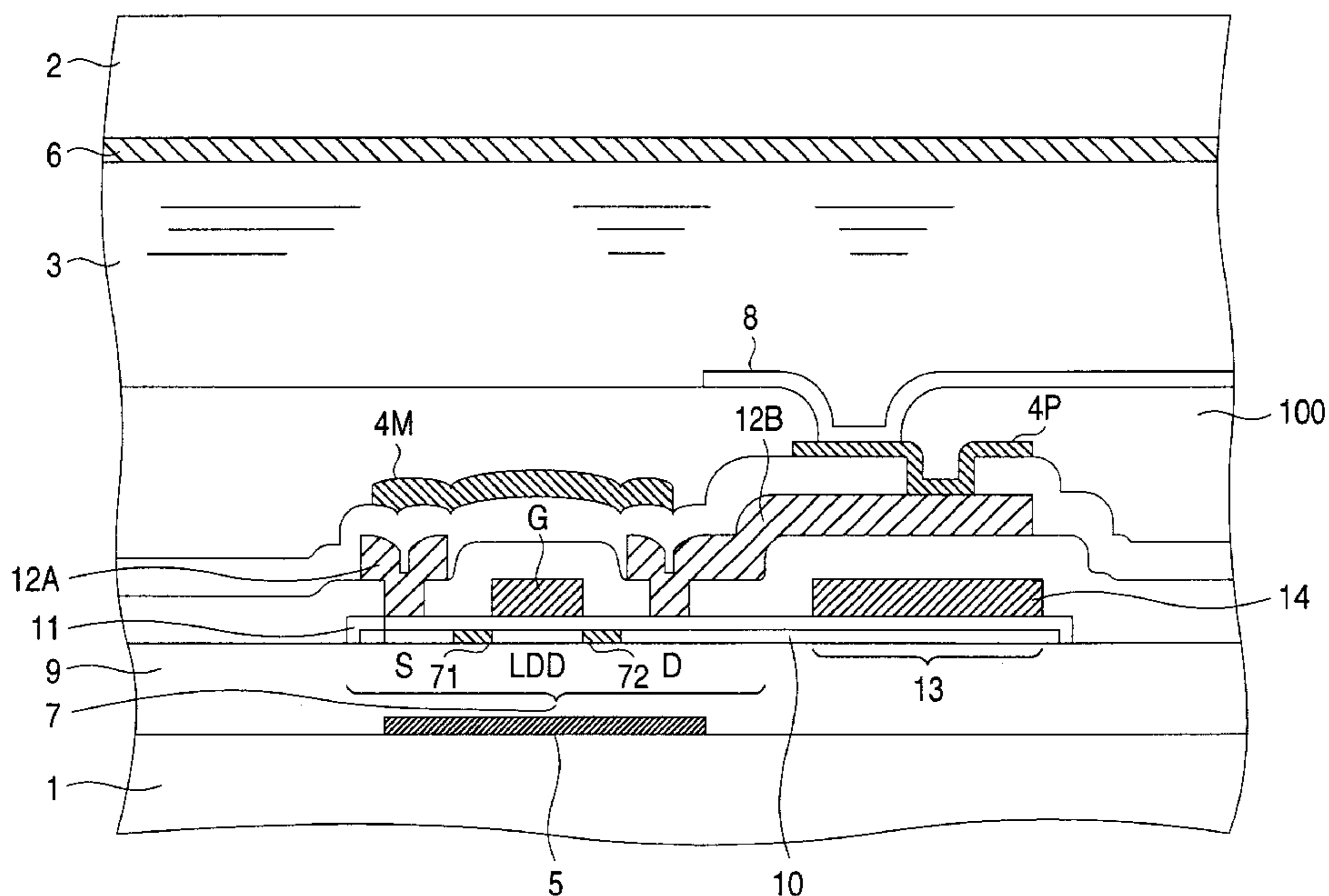
CONSTITUTION OF EMBODIMENT 1 (CROSS SECTION)
