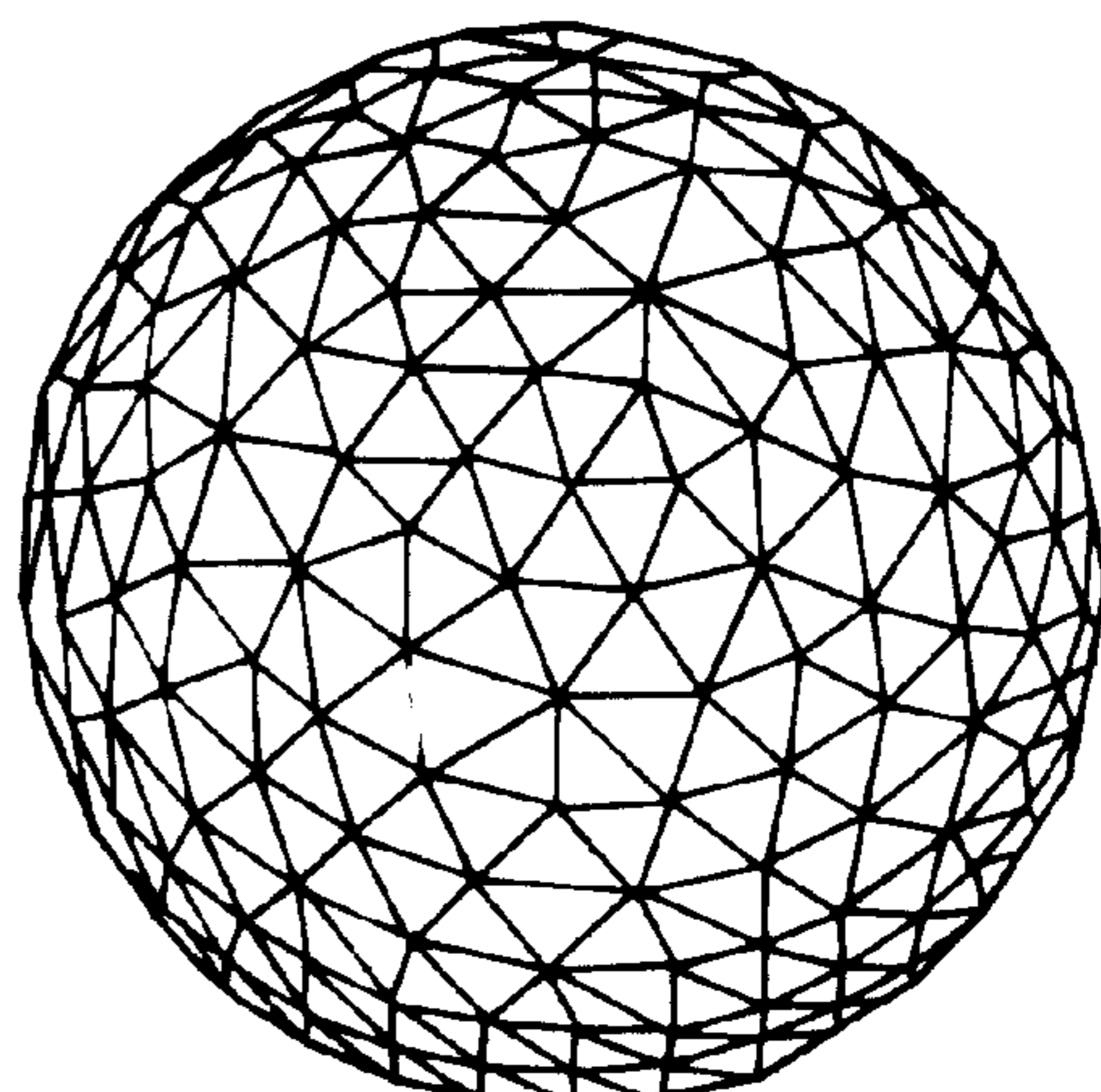
60%: 457 VERTICES
