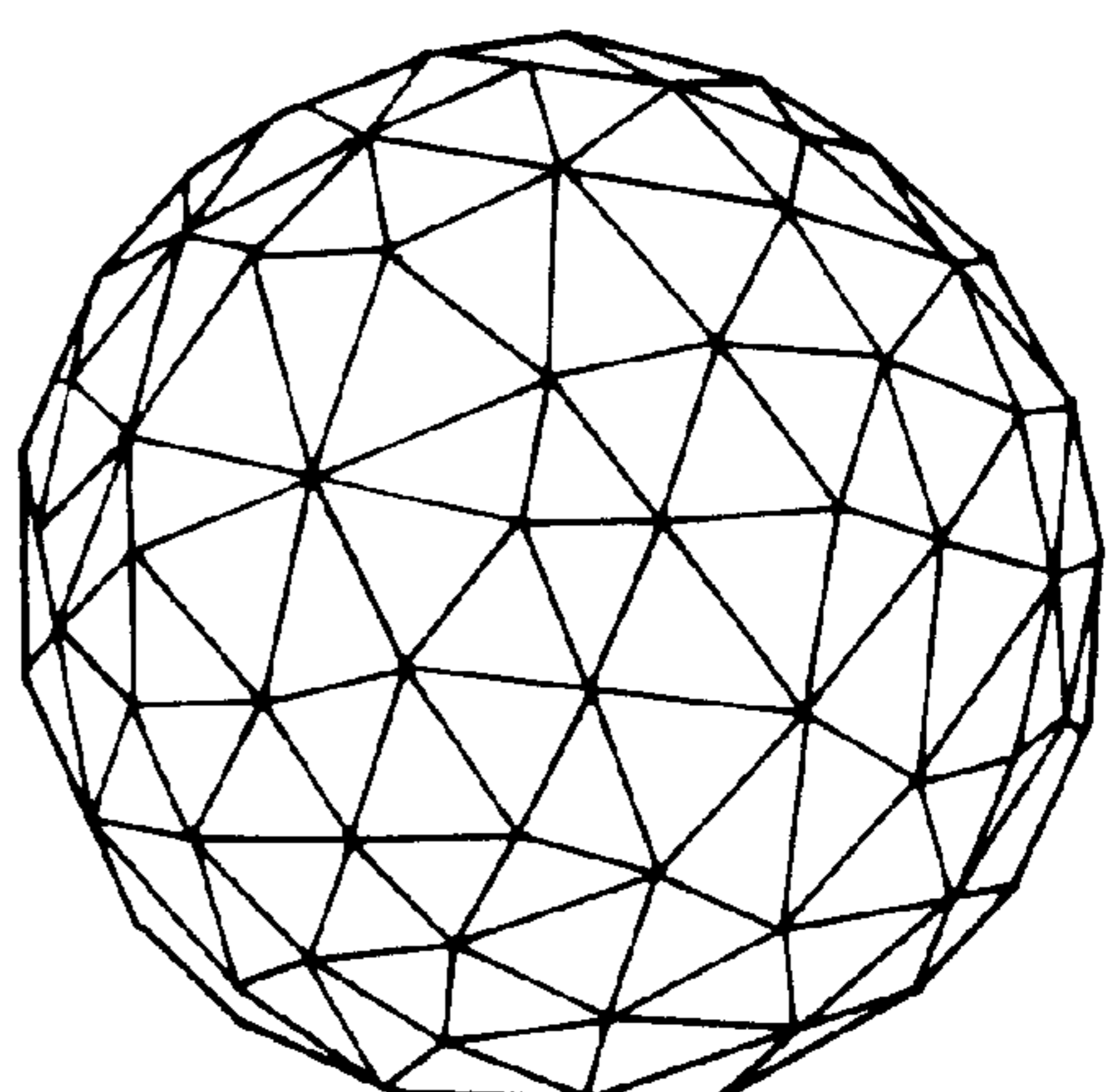
21.6%: 164 VERTICES
