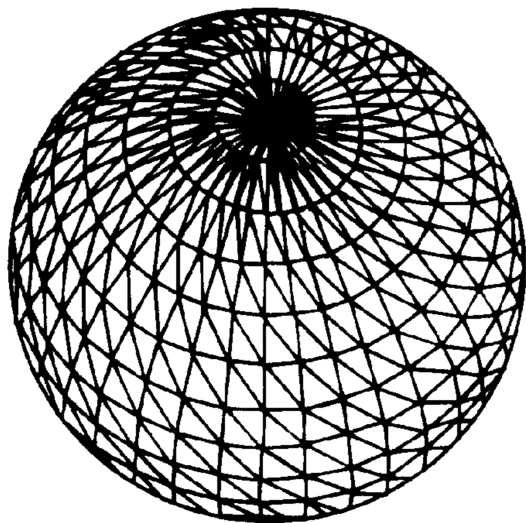
ORIGINAL: 762 VERTICES
