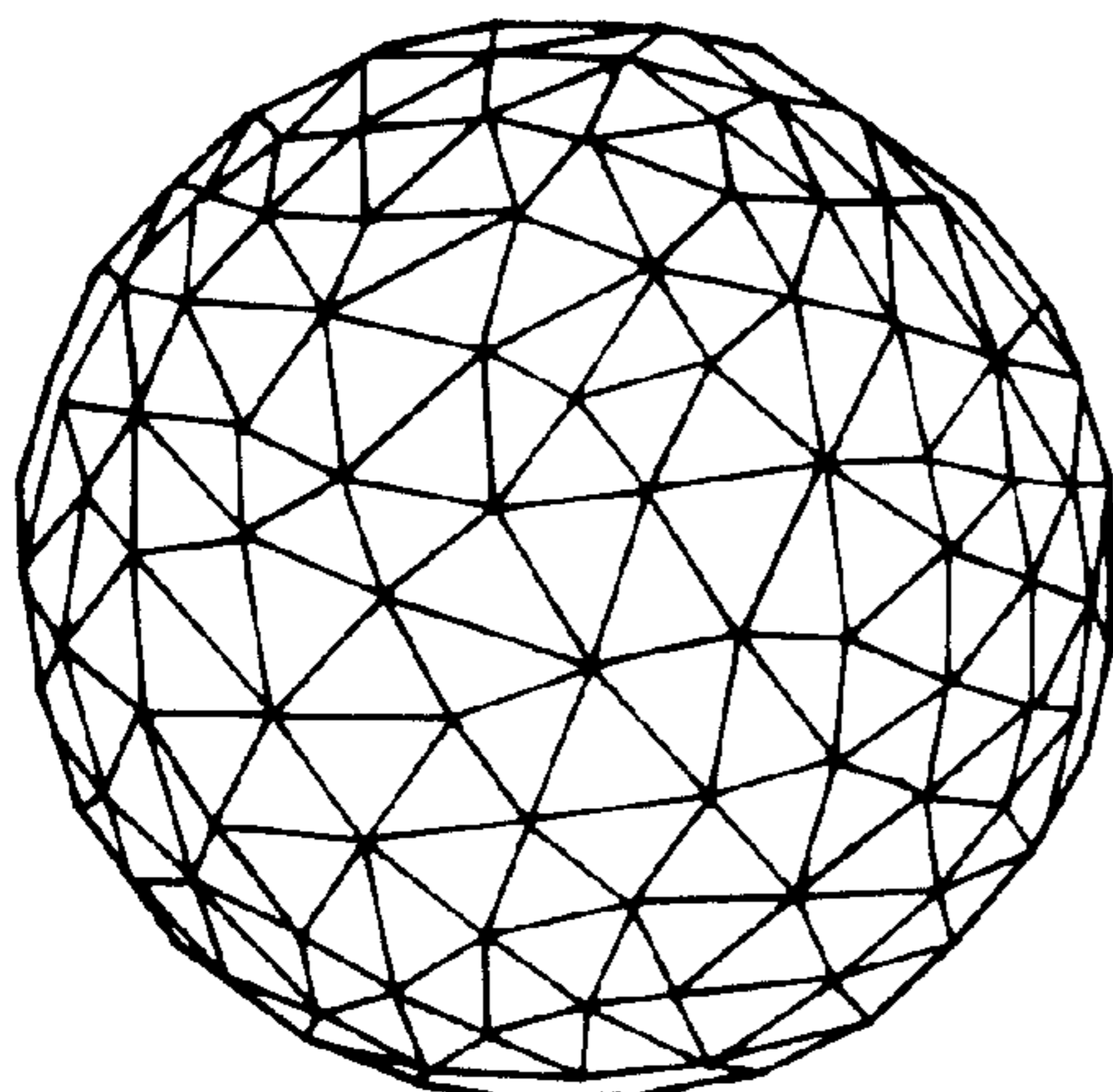
36%: 274 VERTICES
