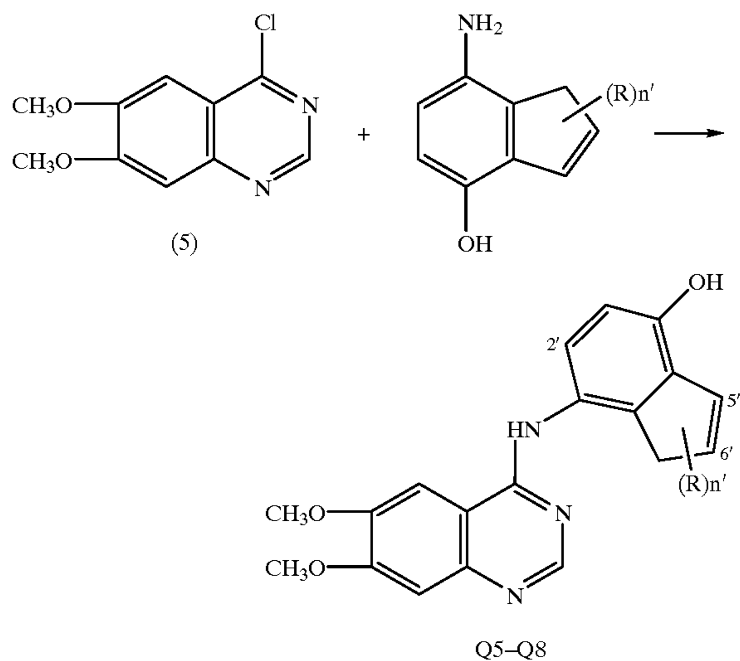
Scheme 3B Synthesis of quinazoline derivatives Q5-Q8
