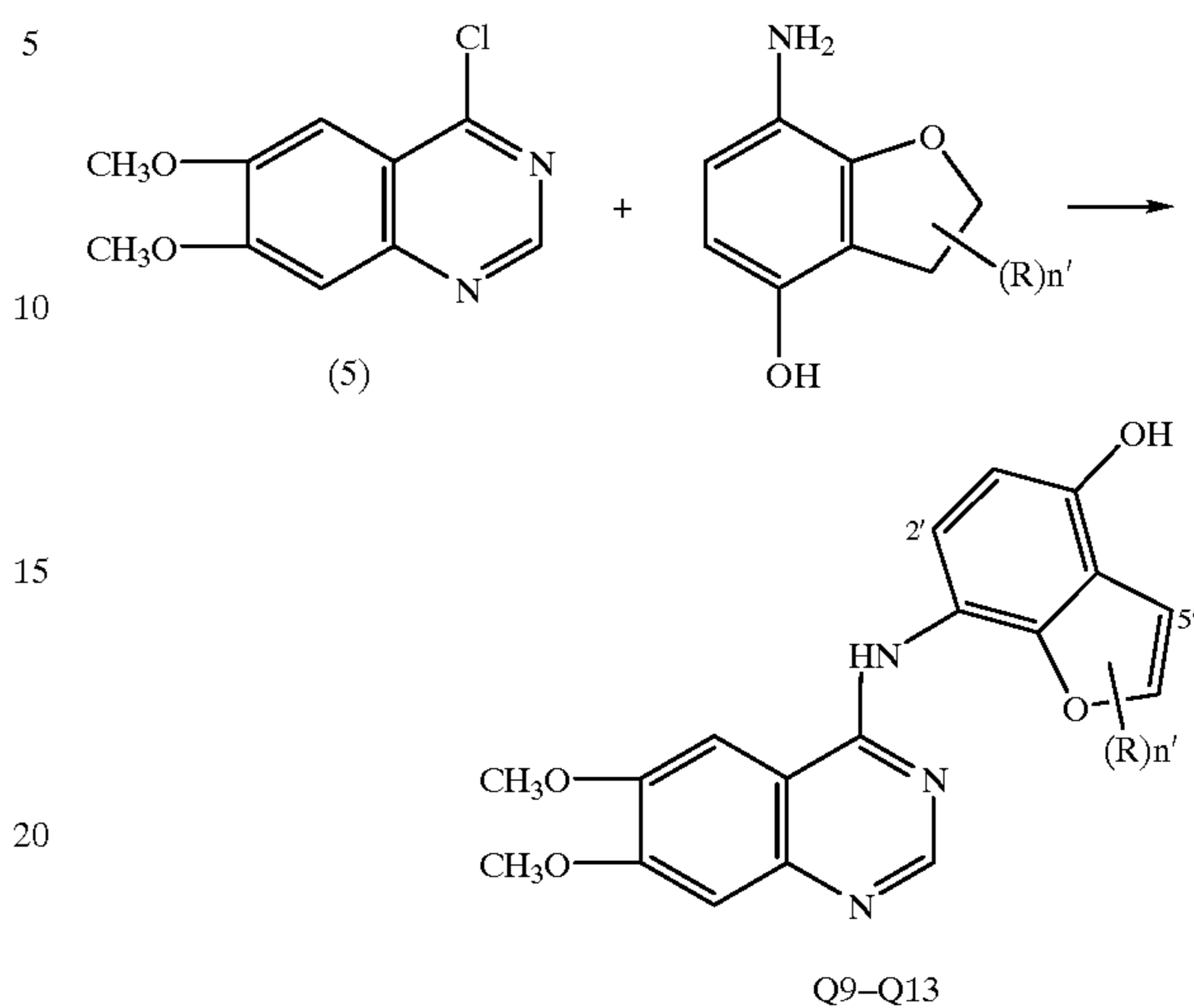
Scheme 3C Synthesis of quinazoline derivatives Q9-Q13
