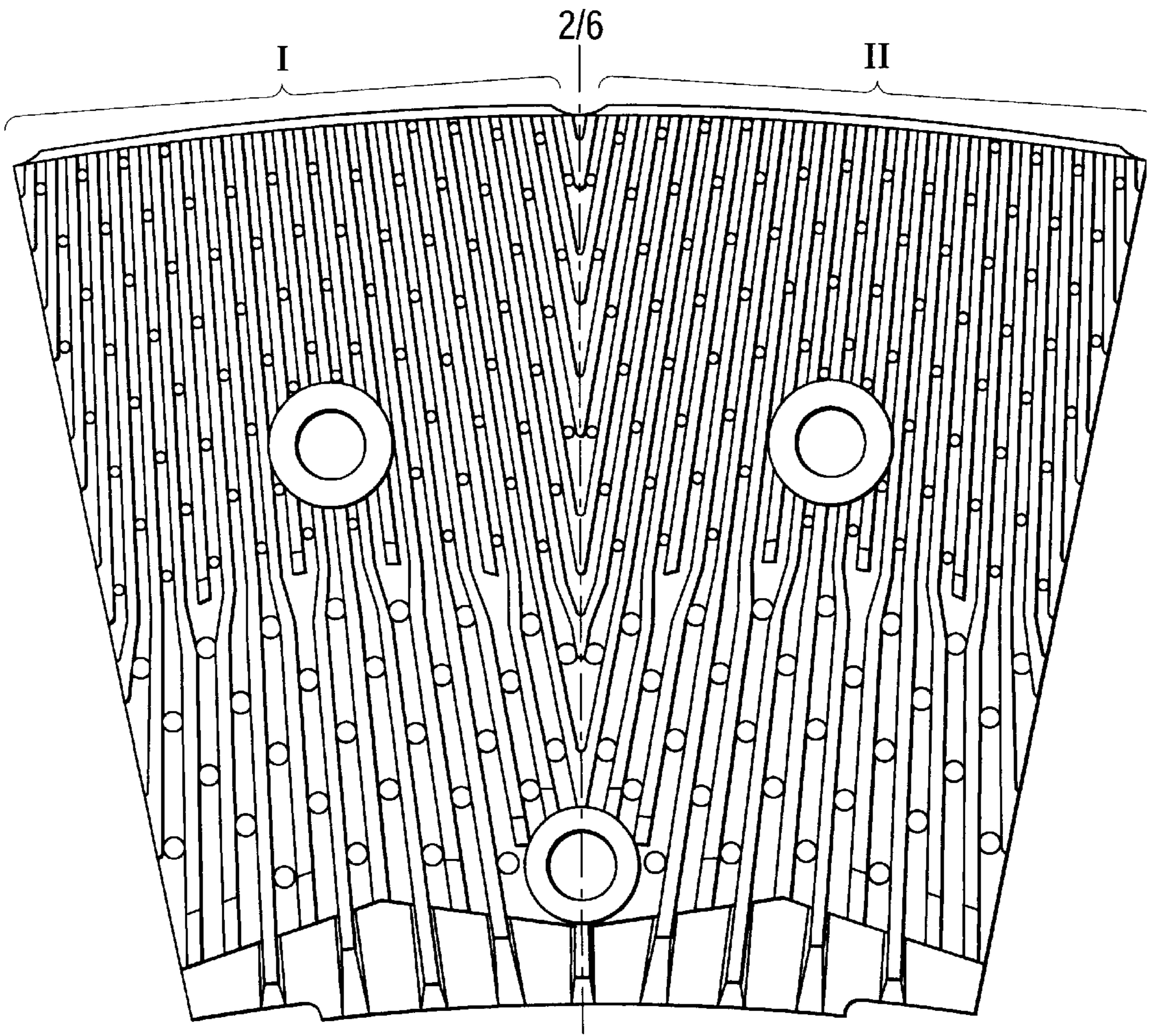
Fig. 2 (PRIOR ART)
