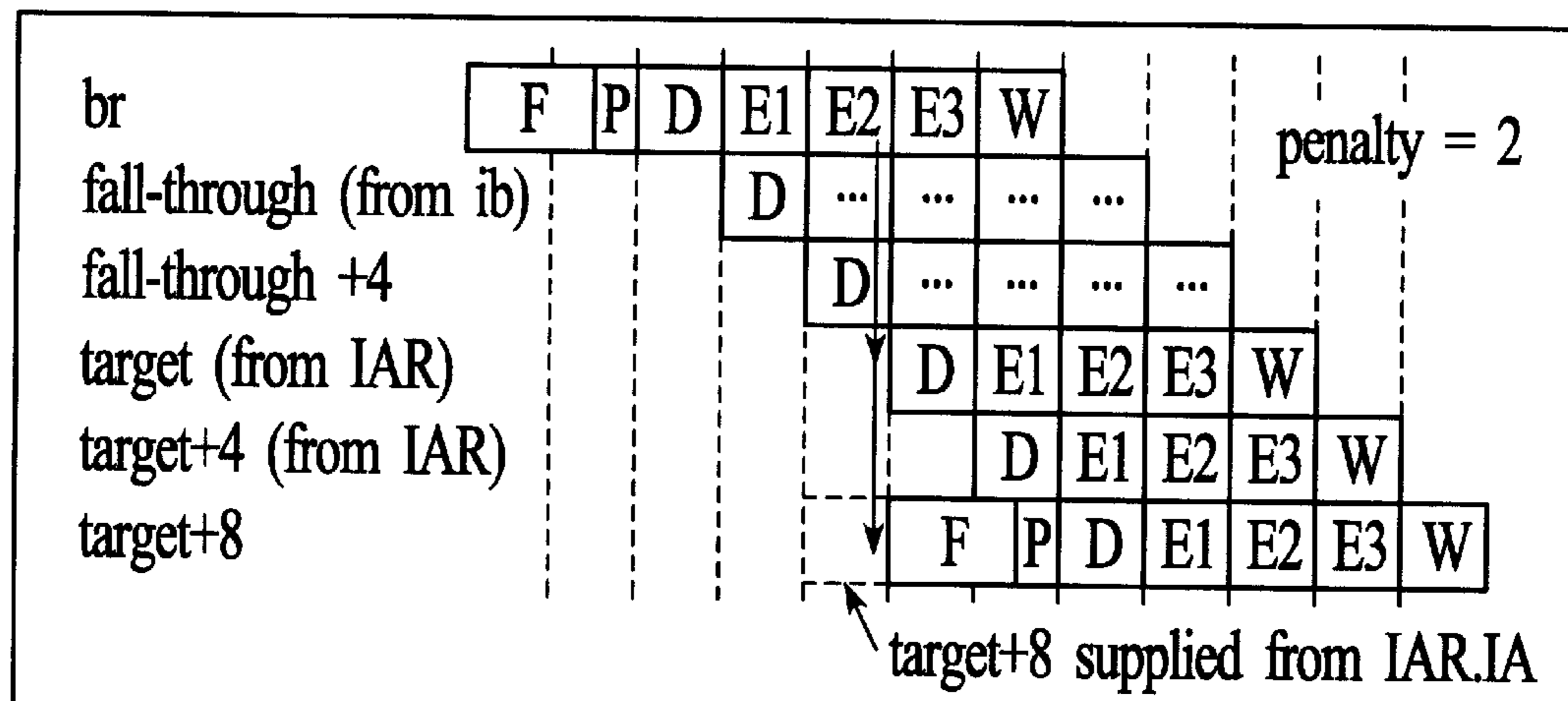
(a) 2 target instructions are ready in IAR.T
