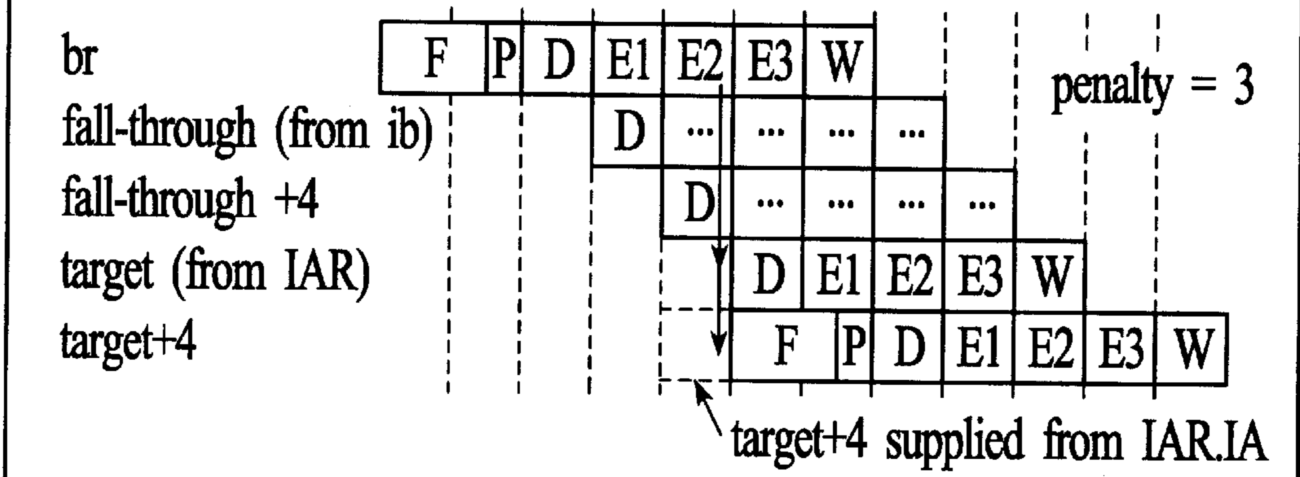
(b) 1 target instruction is ready in IAR.T
