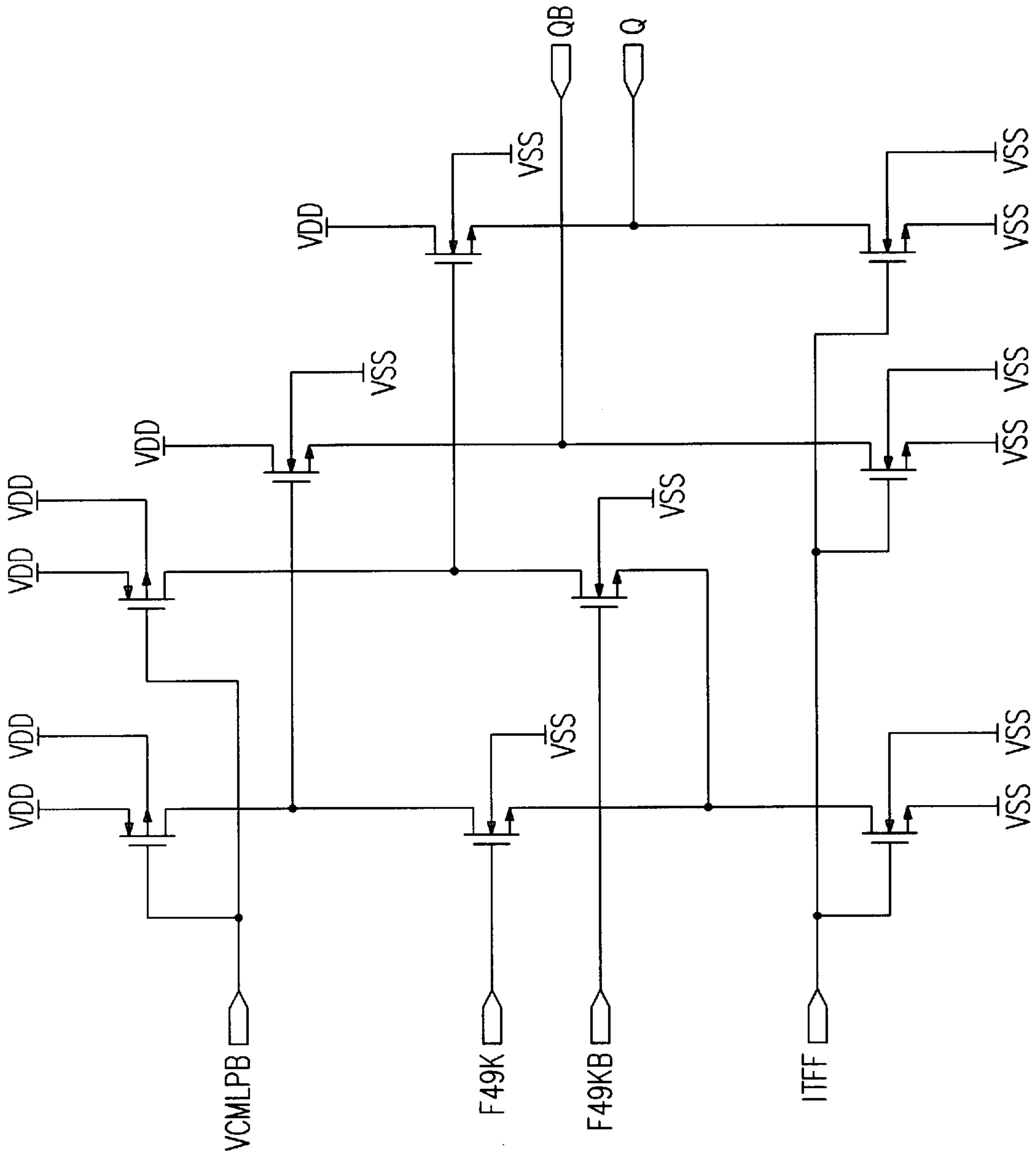
64/65 PRESCALER LEVEL SHIFTER
