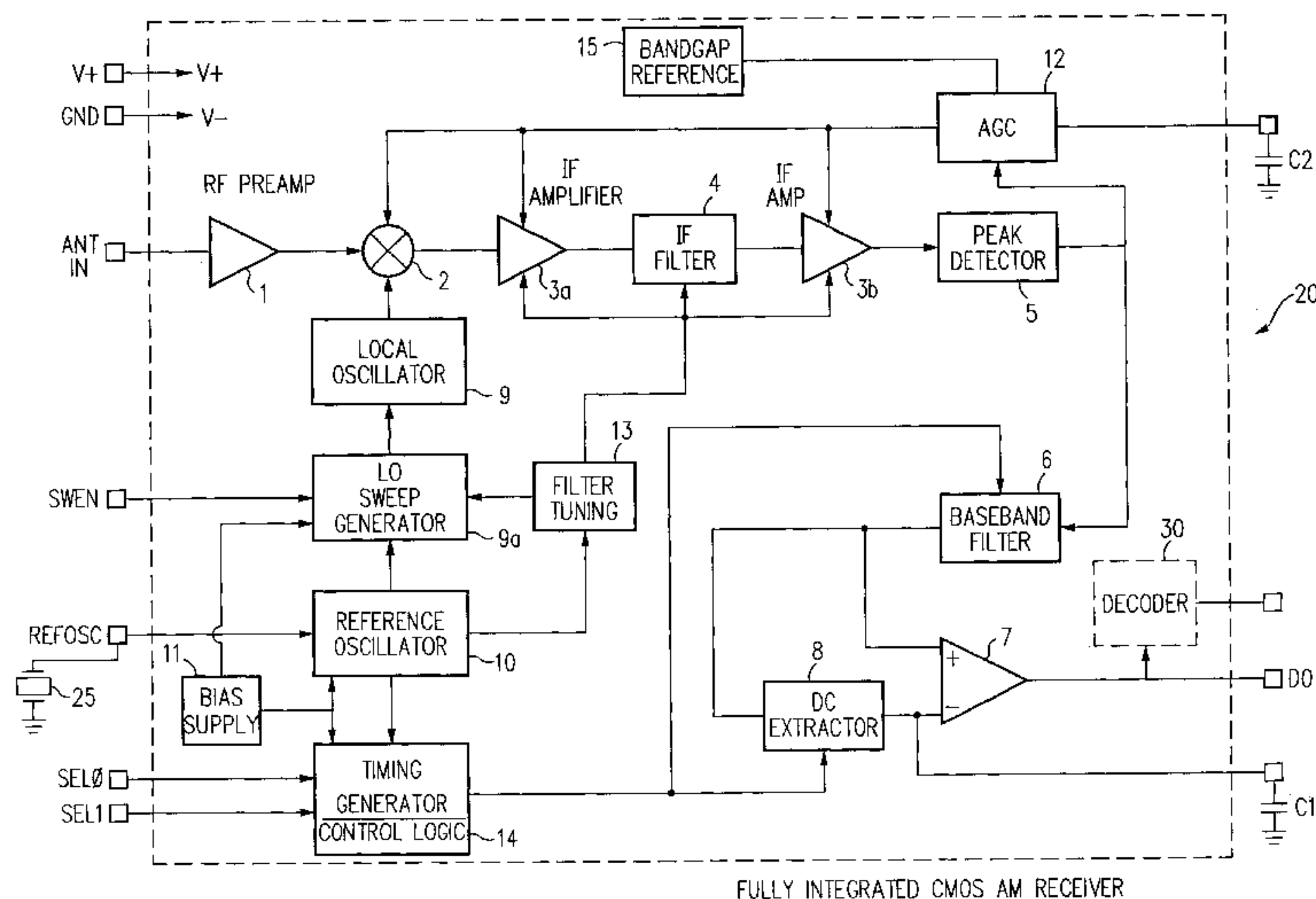
FULLY INTEGRATED CMOS AM RECEIVER
