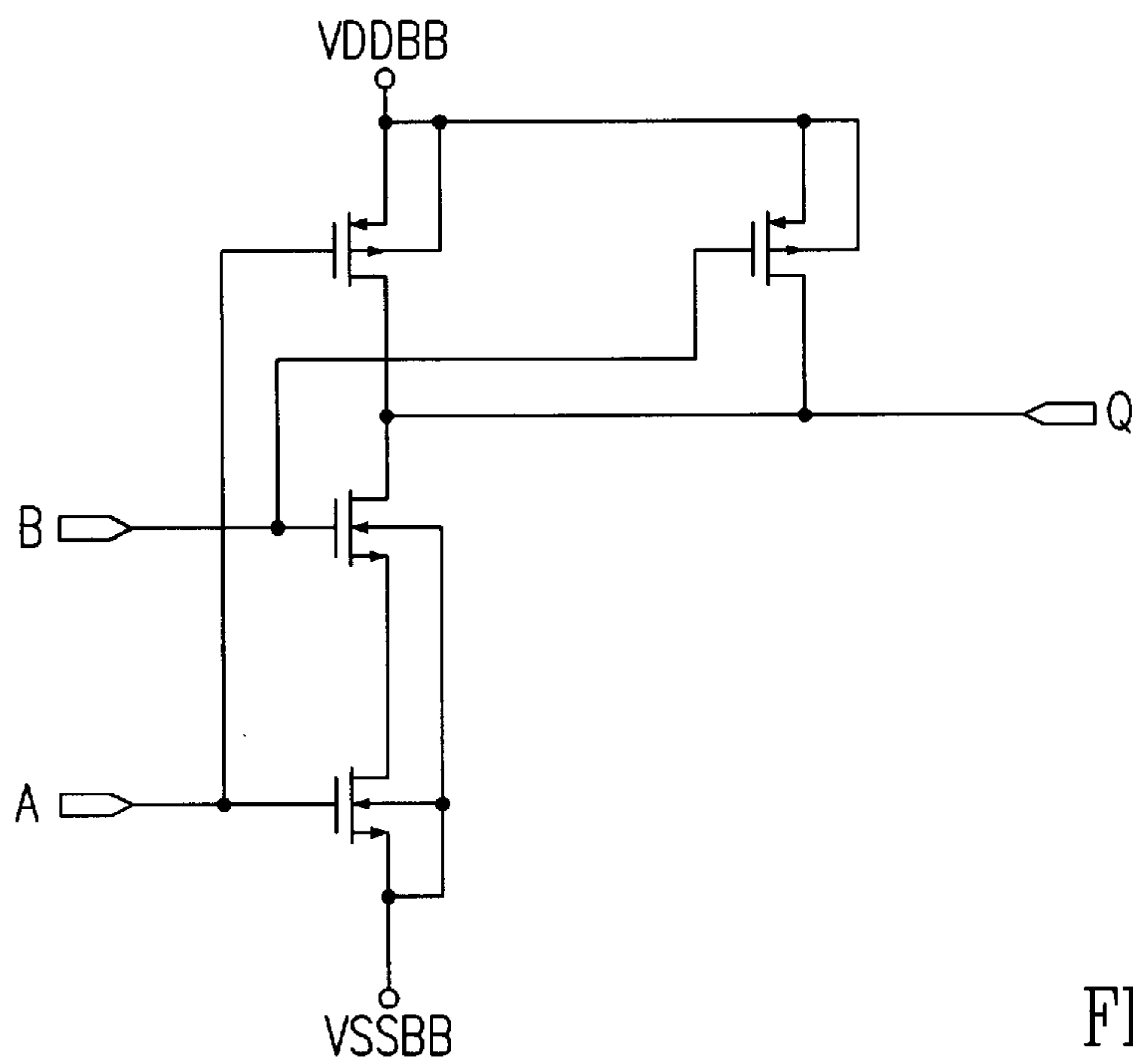
NAND2
