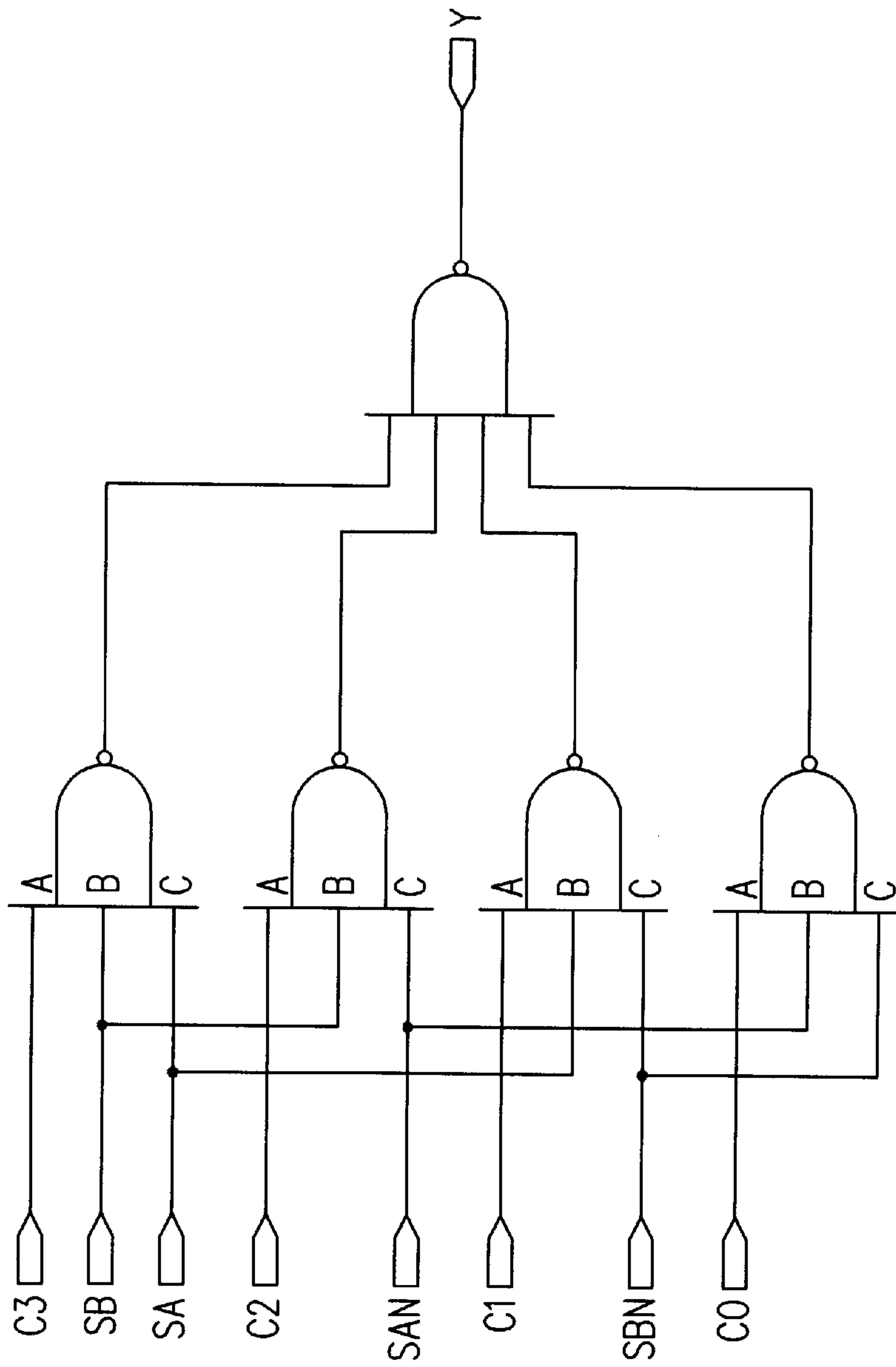
4:1 SELECTOR
