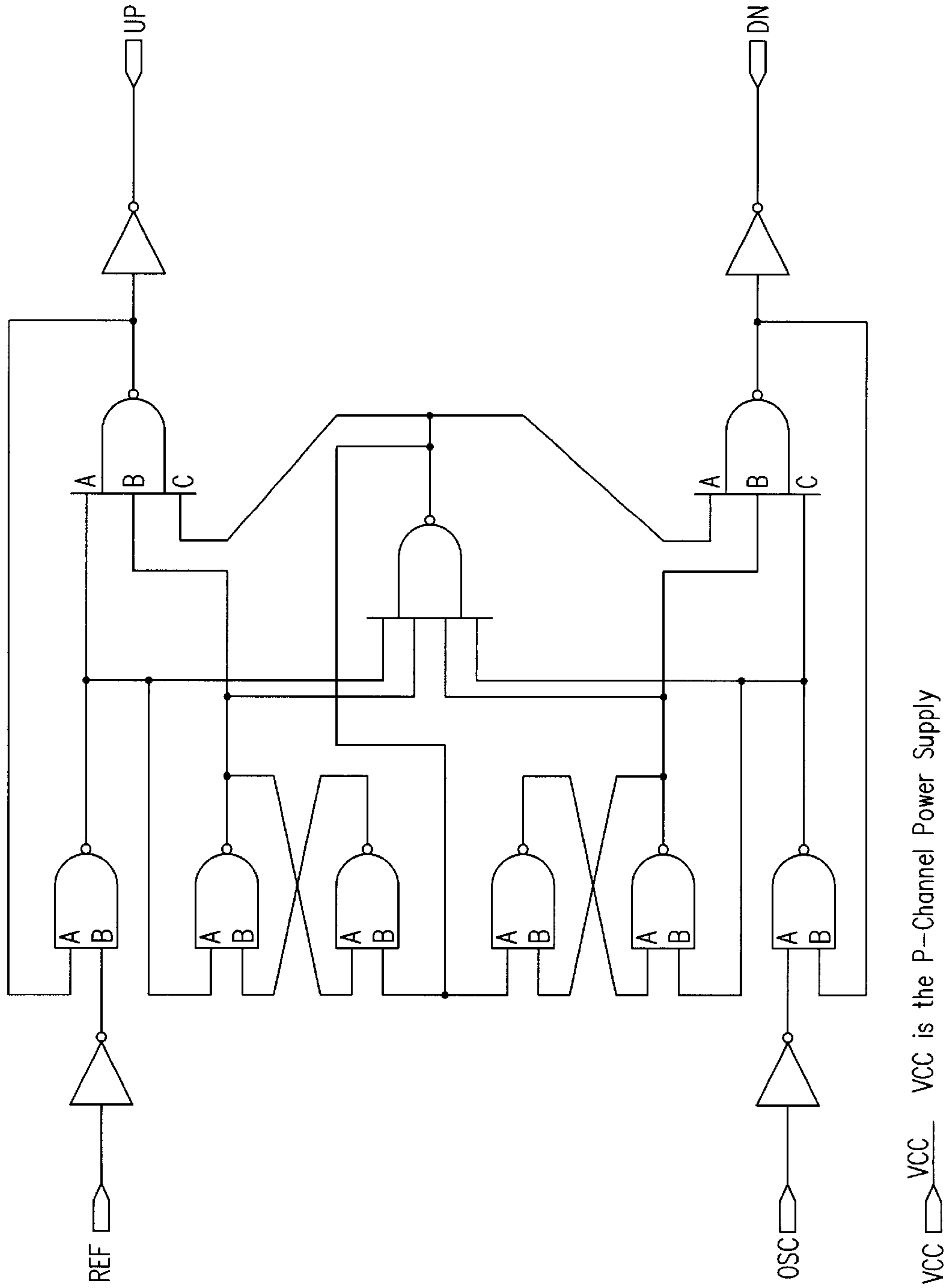
PHASE/FREQUENCY DETECTOR
