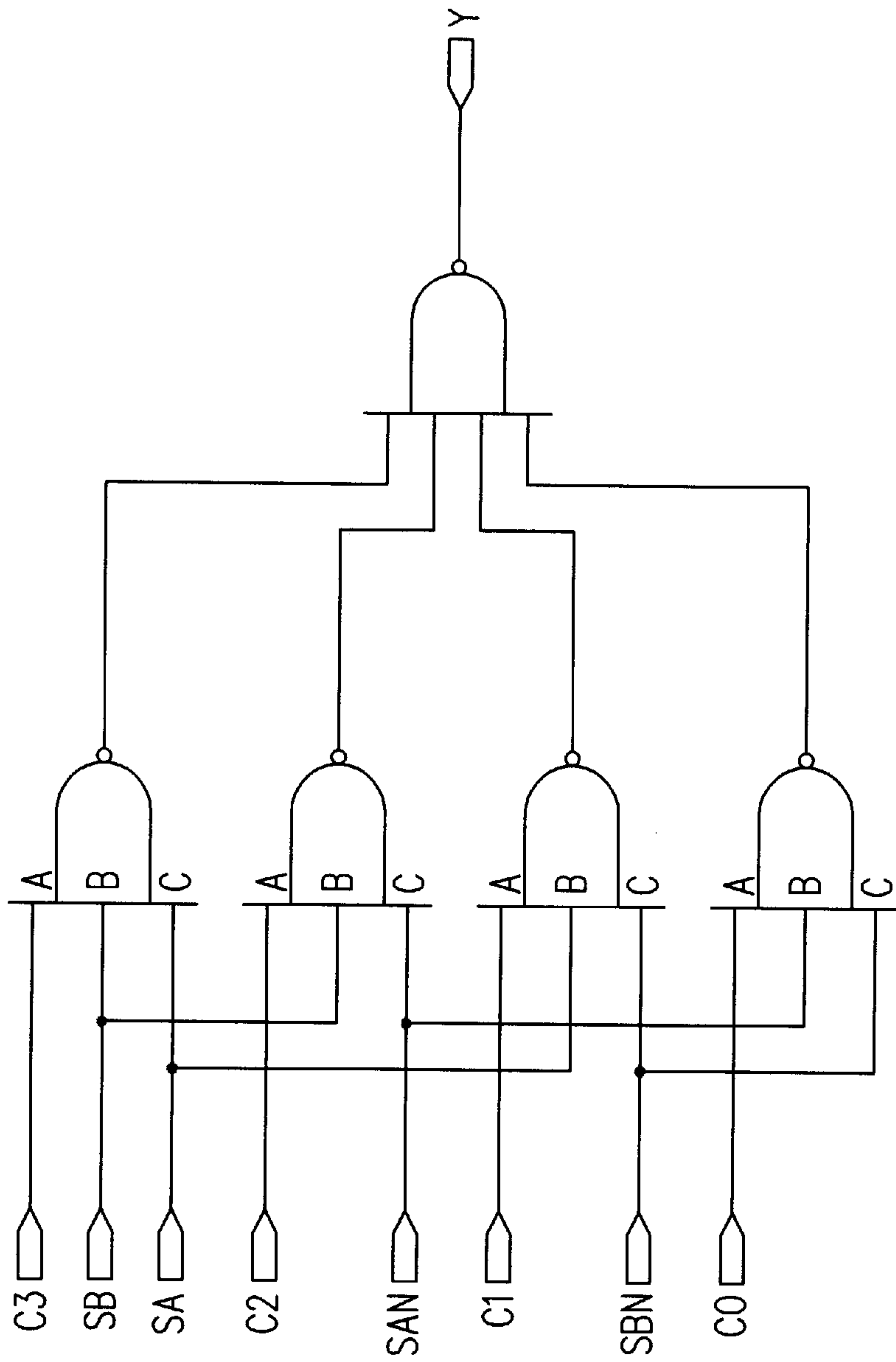
4:1 SELECTOR
