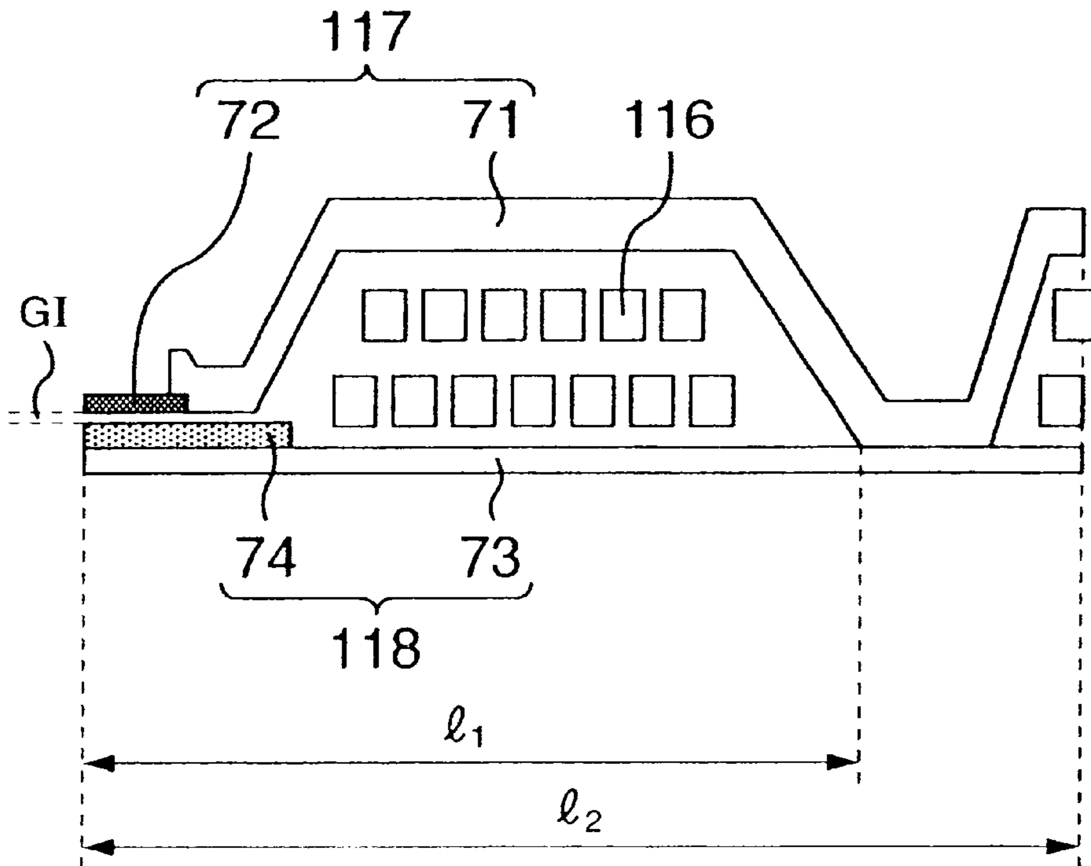
CROSS SECTION
