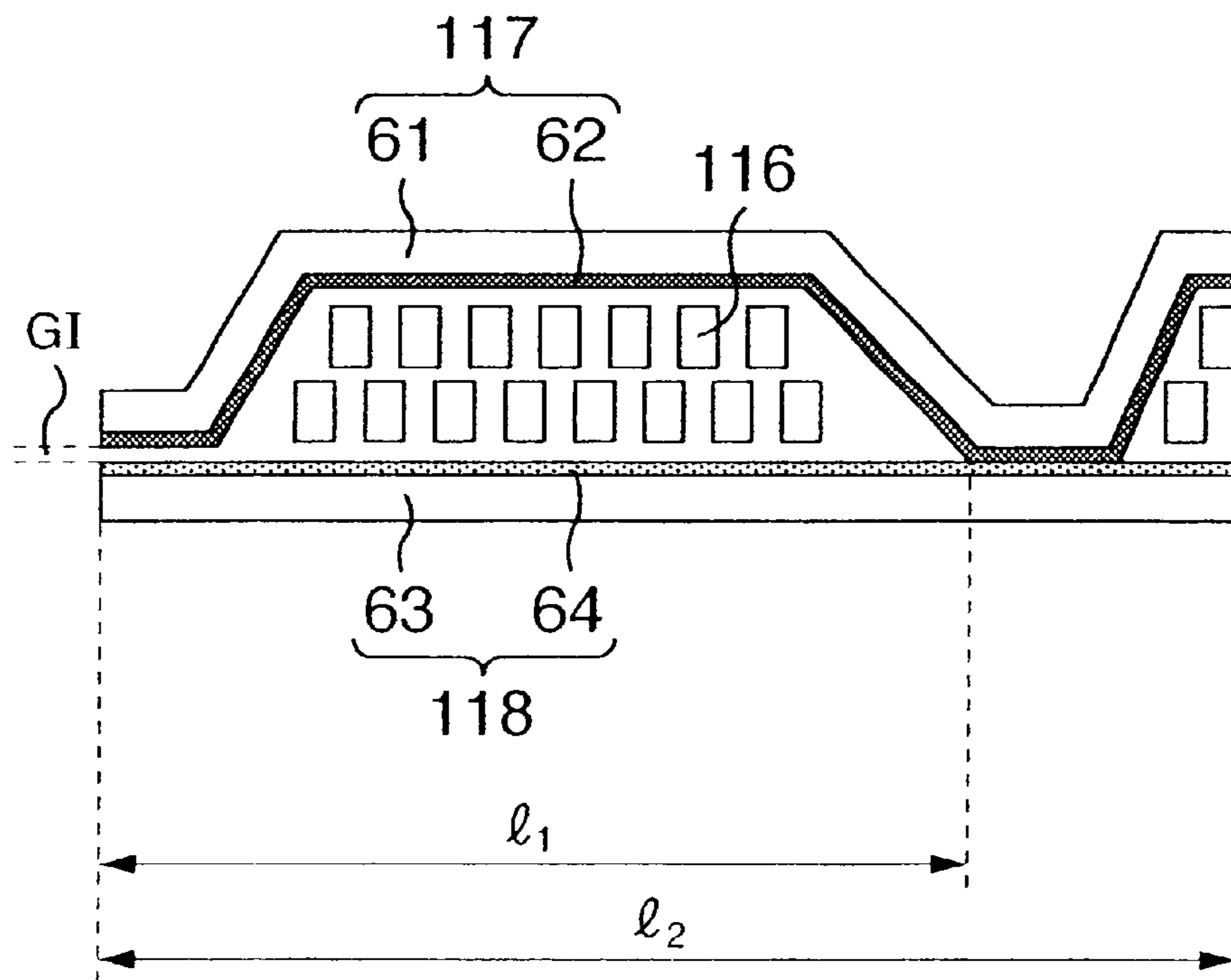
CROSS SECTION
