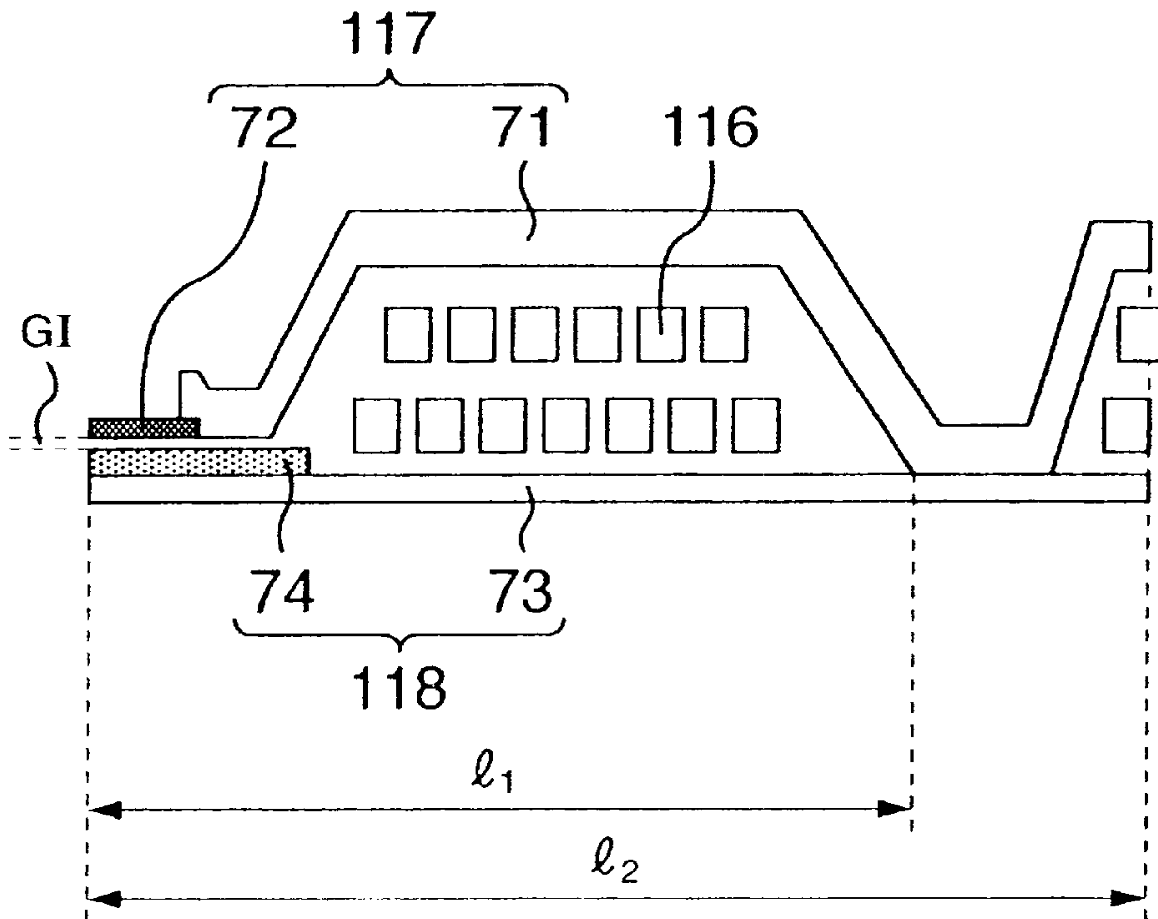
CROSS SECTION
