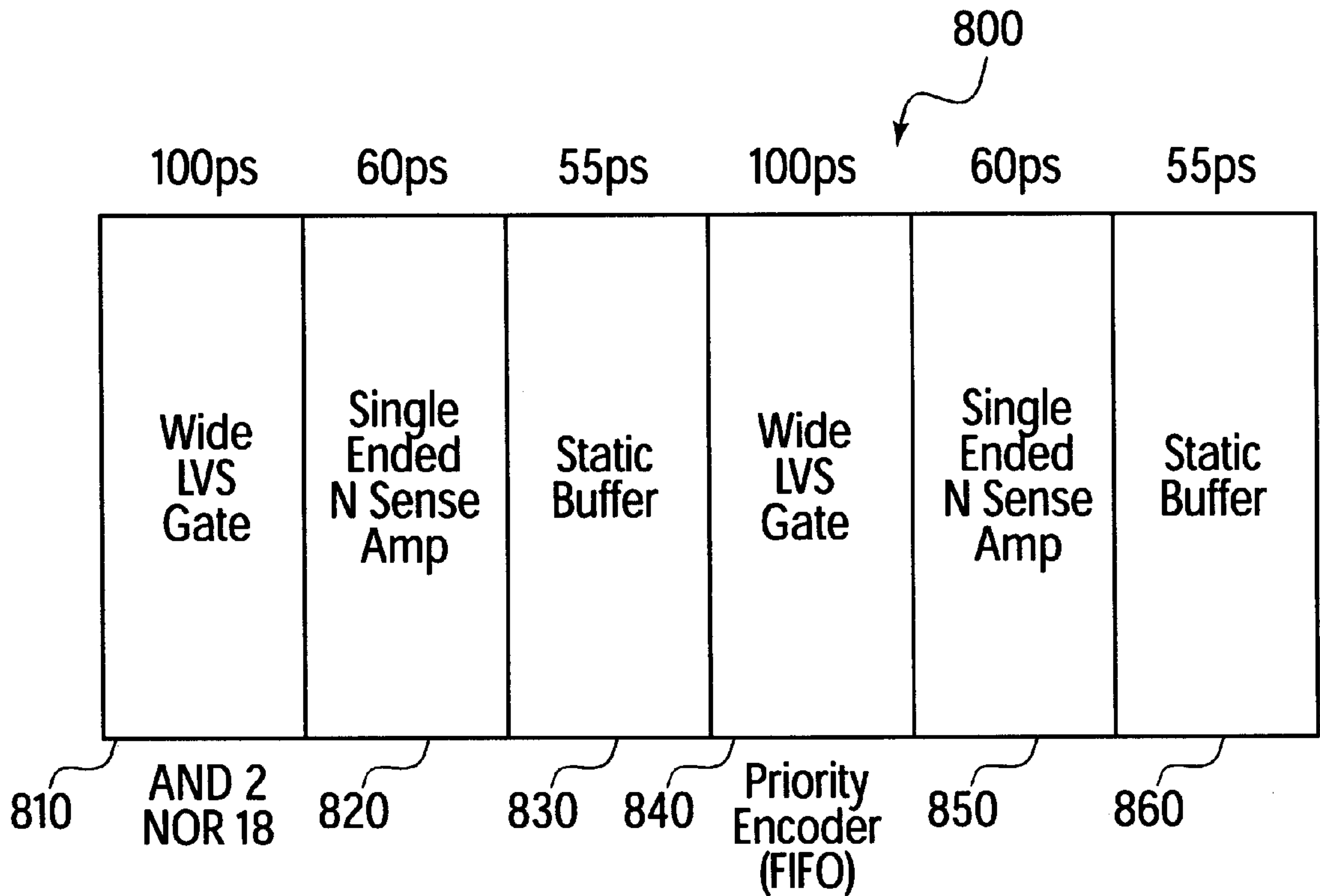
LVS scheduler or PLA circuit topology
