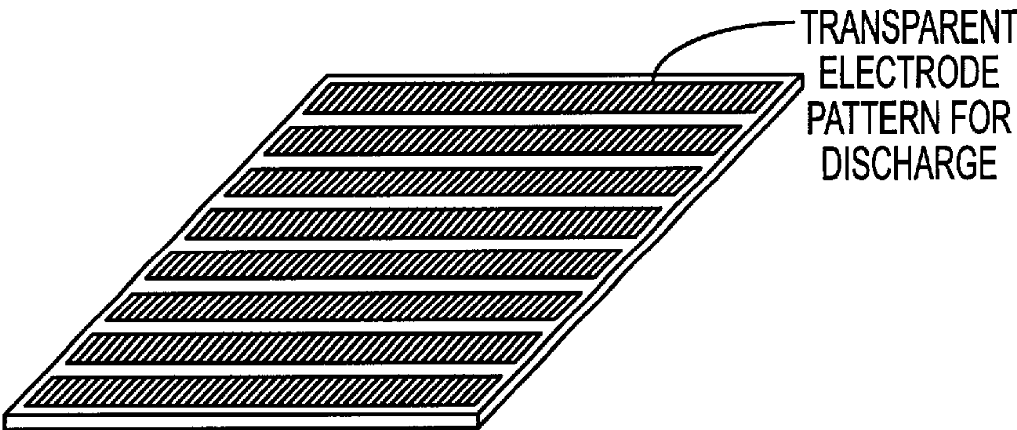
FORMATION OF BUS ELECTRODES (Ag ELECTRODES) (SCREEN PRINTING) FIG. 8B
