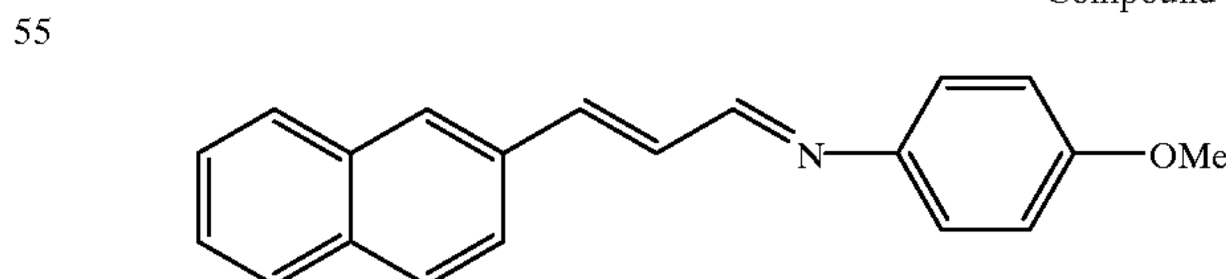
Compound 34
