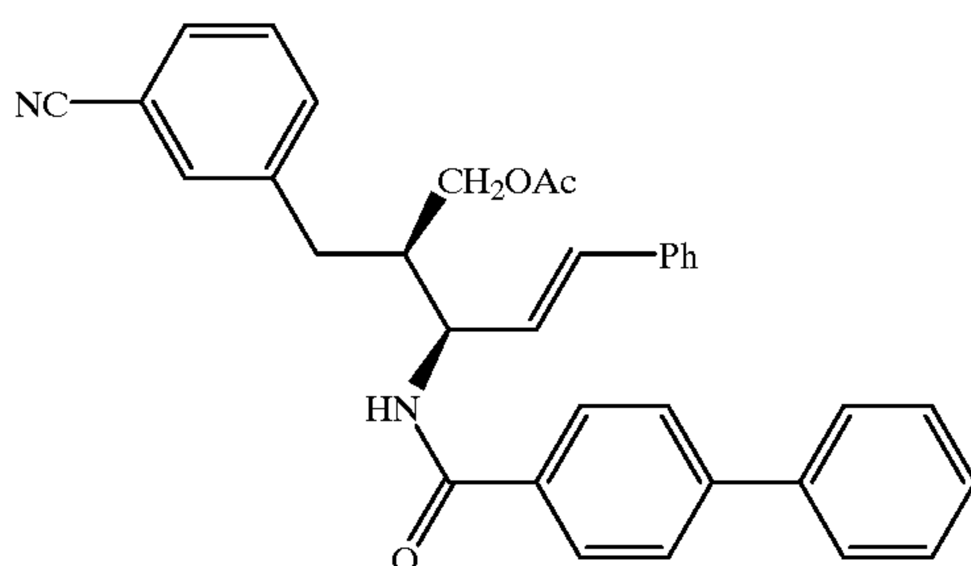
Compound 45
