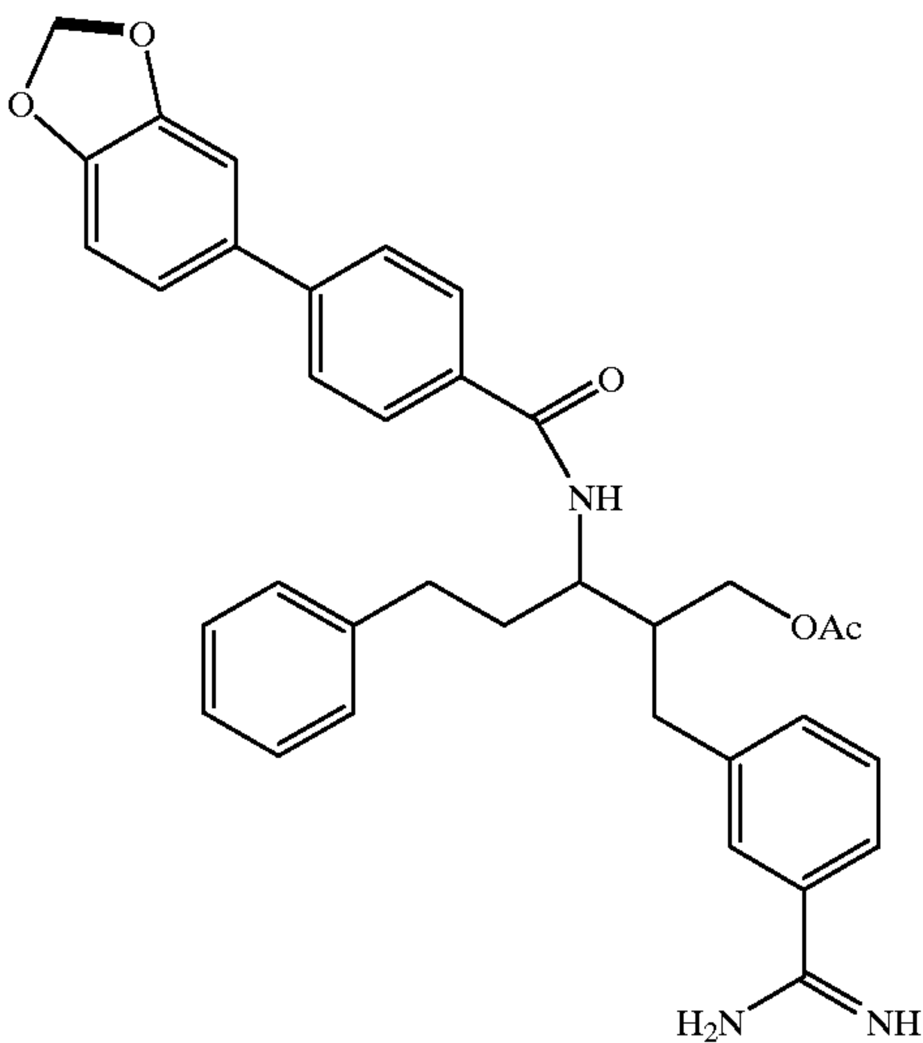
Compound 166
