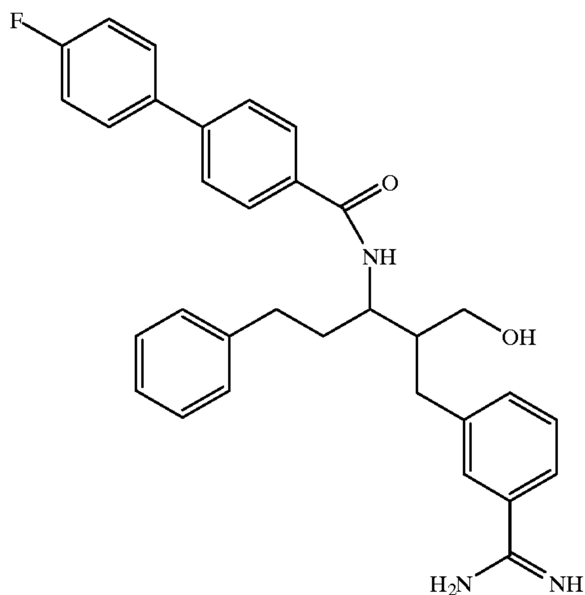
Compound 169
