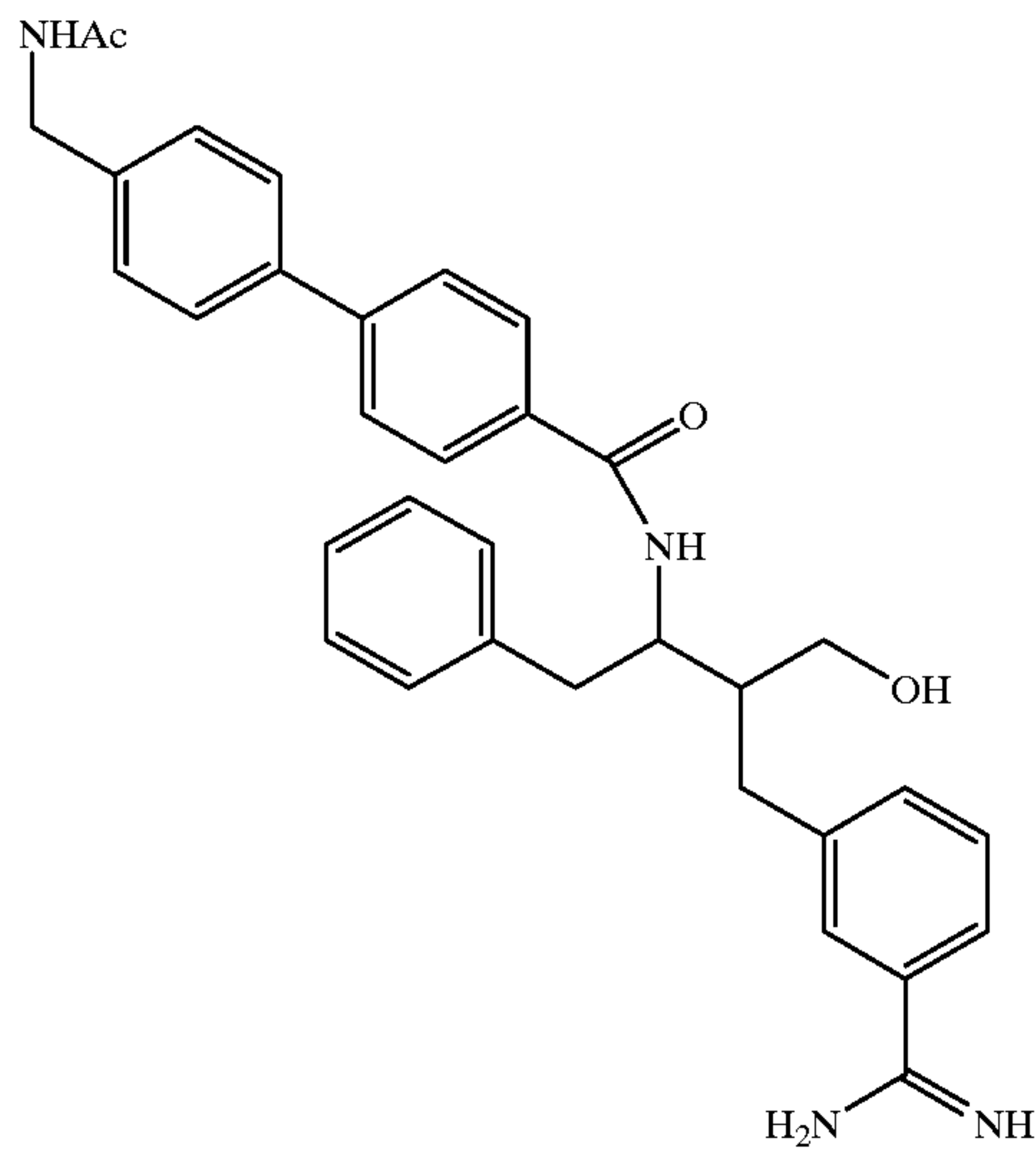
Compound 173
