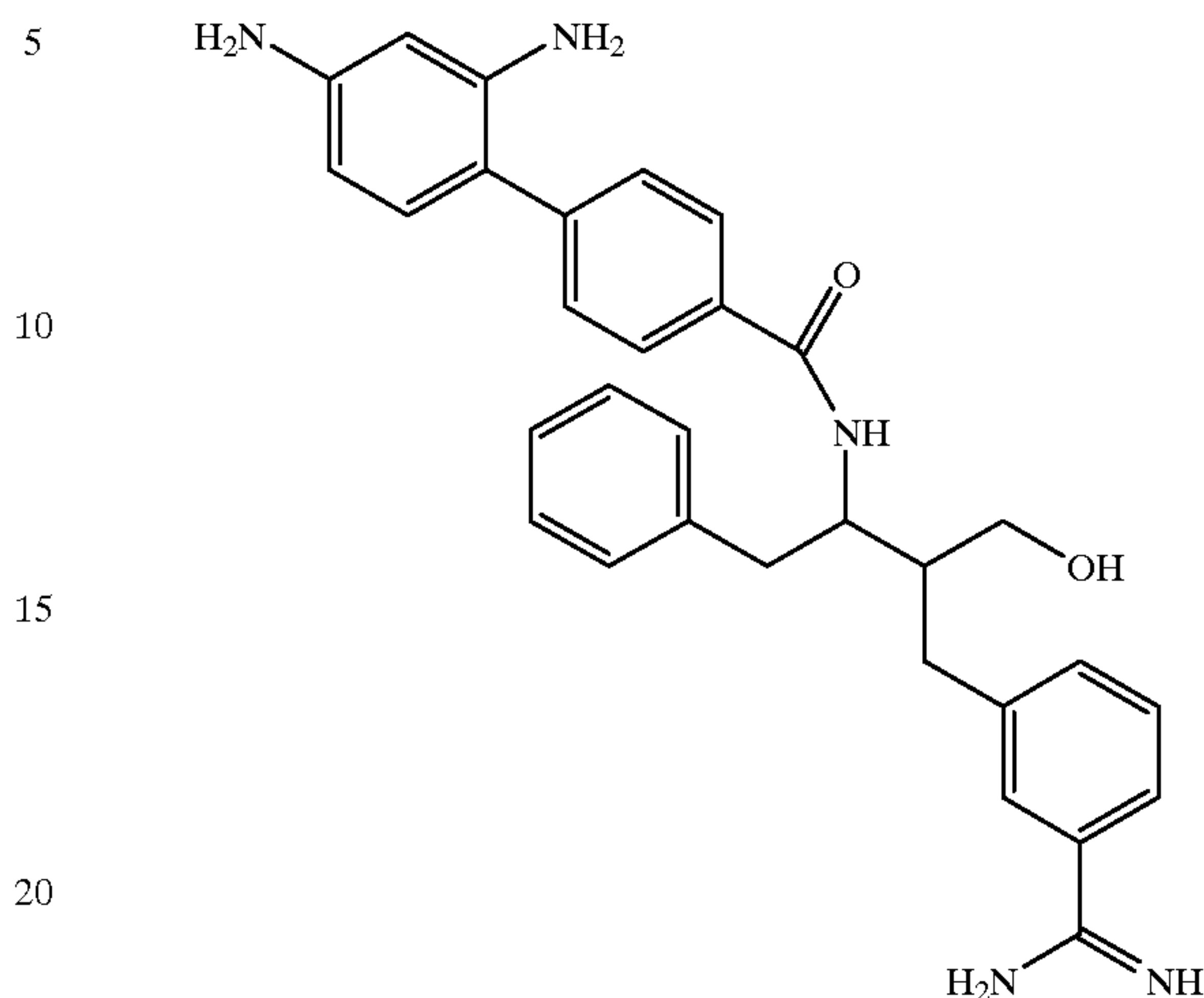
Compound 179
