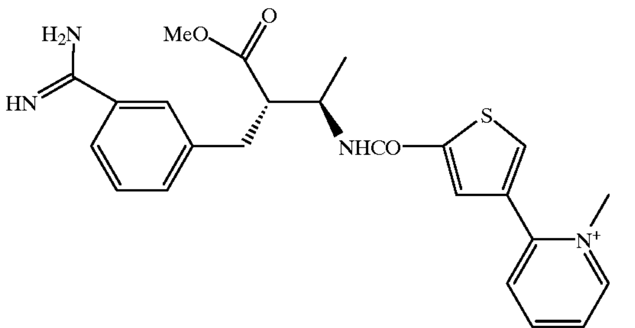
Compound 341
