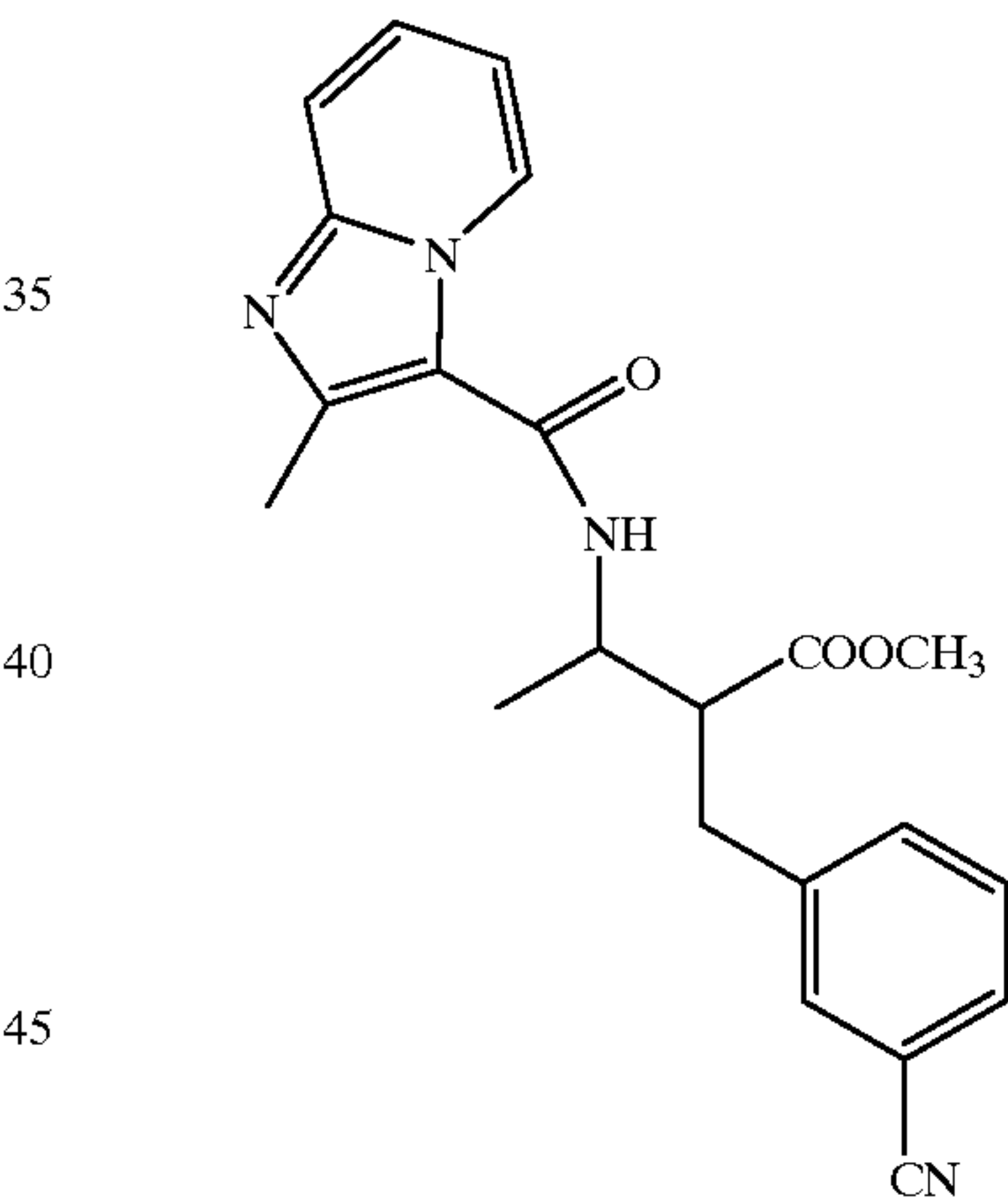
Compound 263
