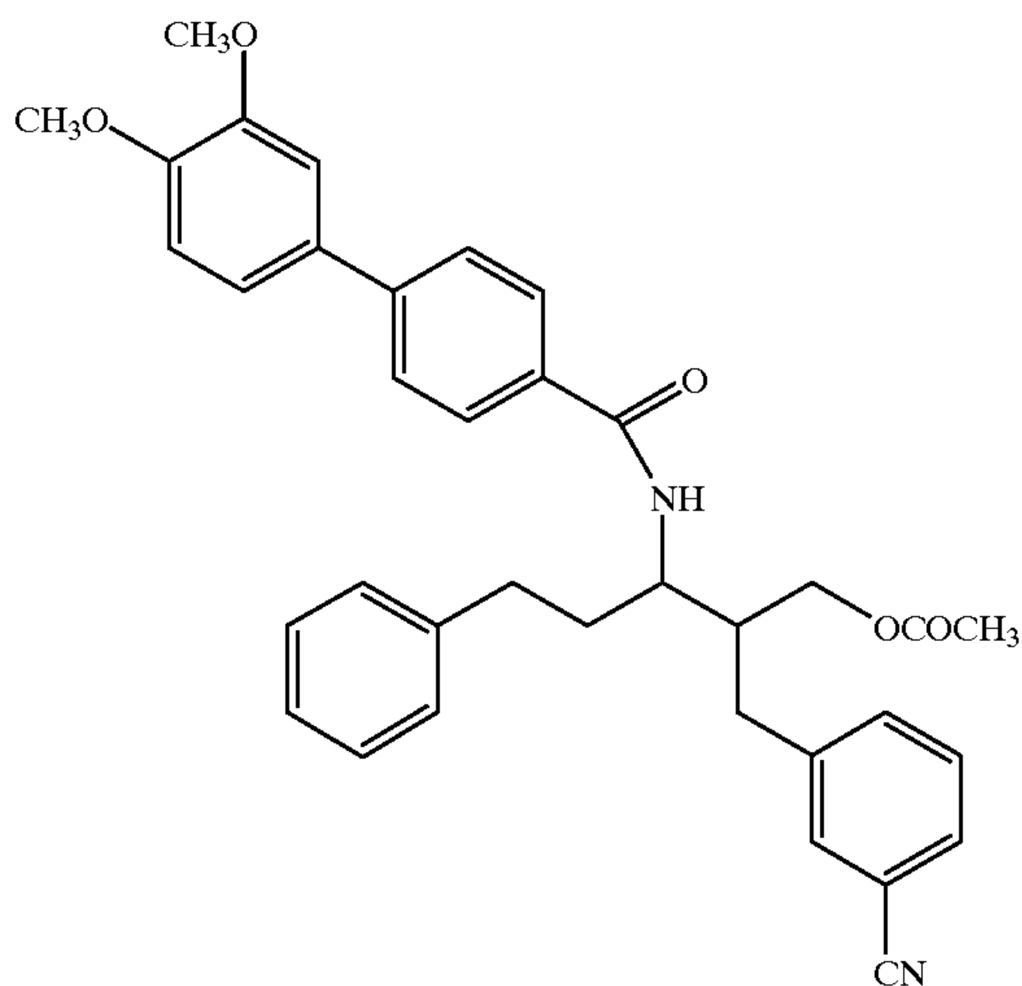
Compound 153
