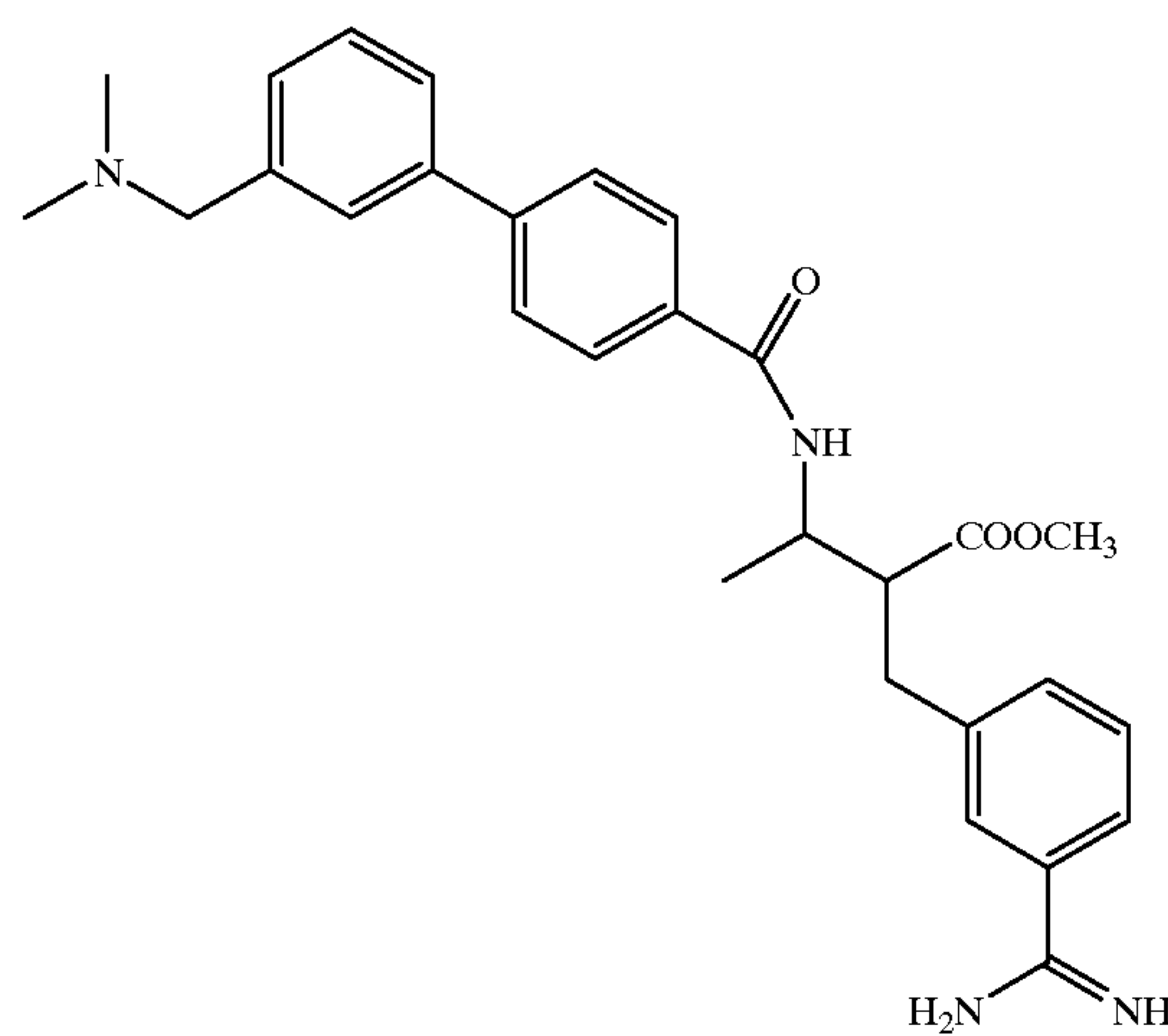
Compound 190
