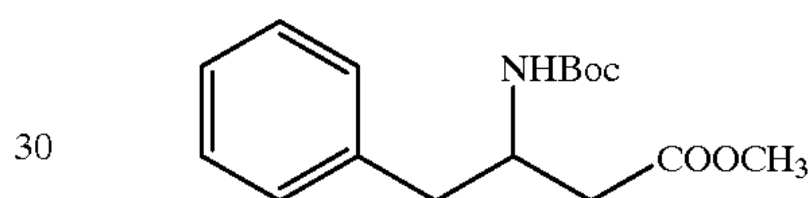
Compound 52
