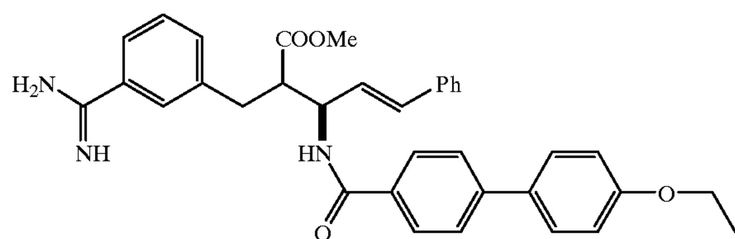
Compound 31
