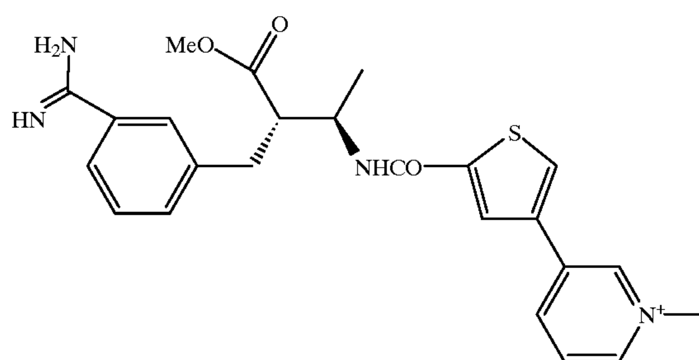
3-{5-[3-(3-Carbamimidoylphenyl)-2-(R)-methoxycarbonyl-1-(R)-methyl-propylcarbamoyl]-thiophen-3-yl}-1-methylpyridinium ditrifluoroacetate.
