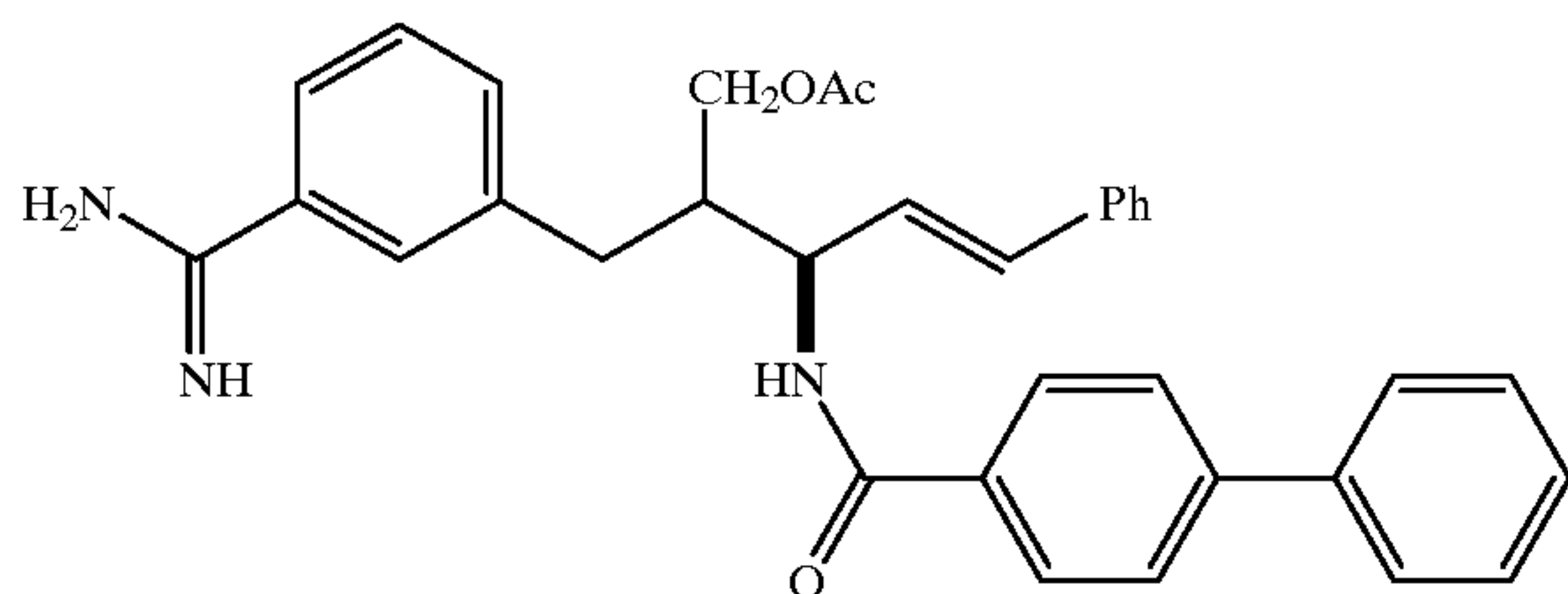
Compound 46
