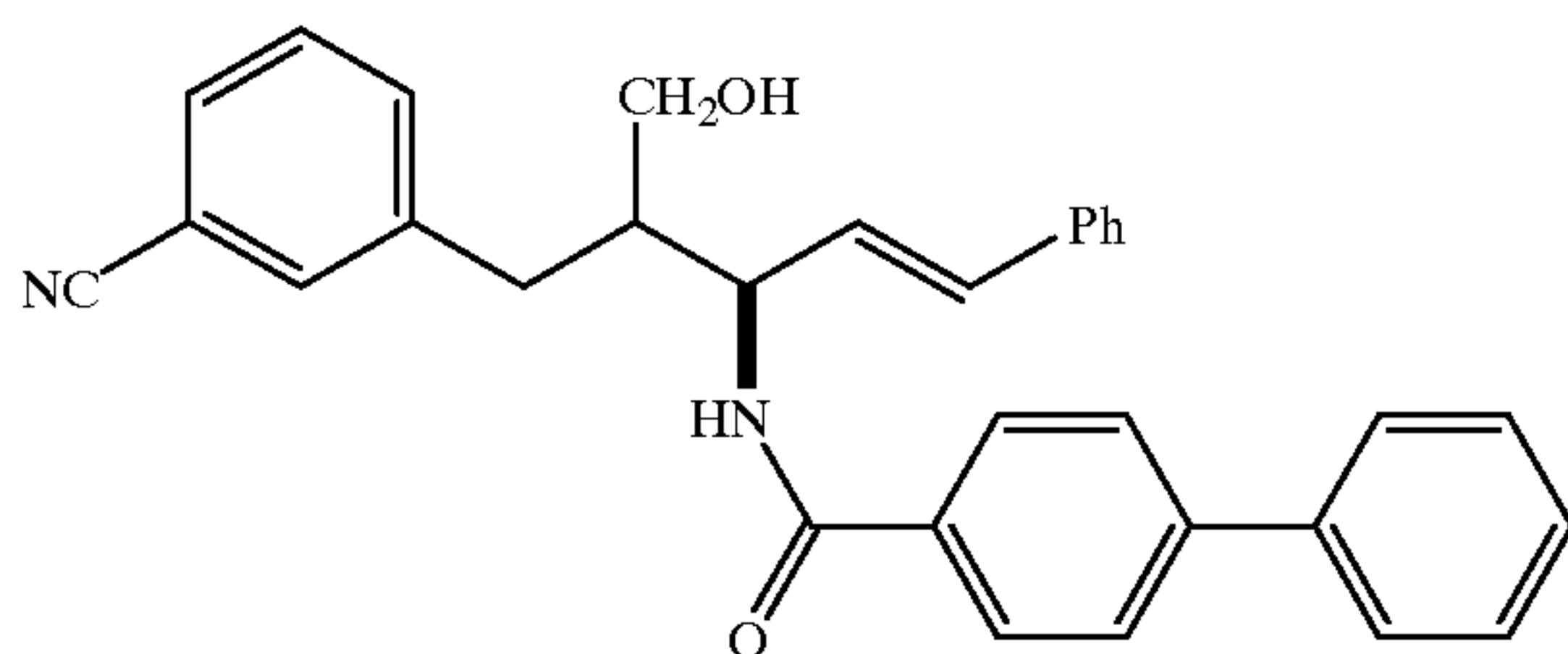
Compound 41
