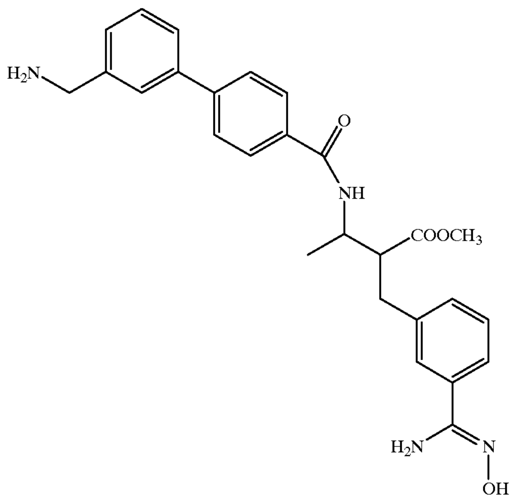
Compound 189
