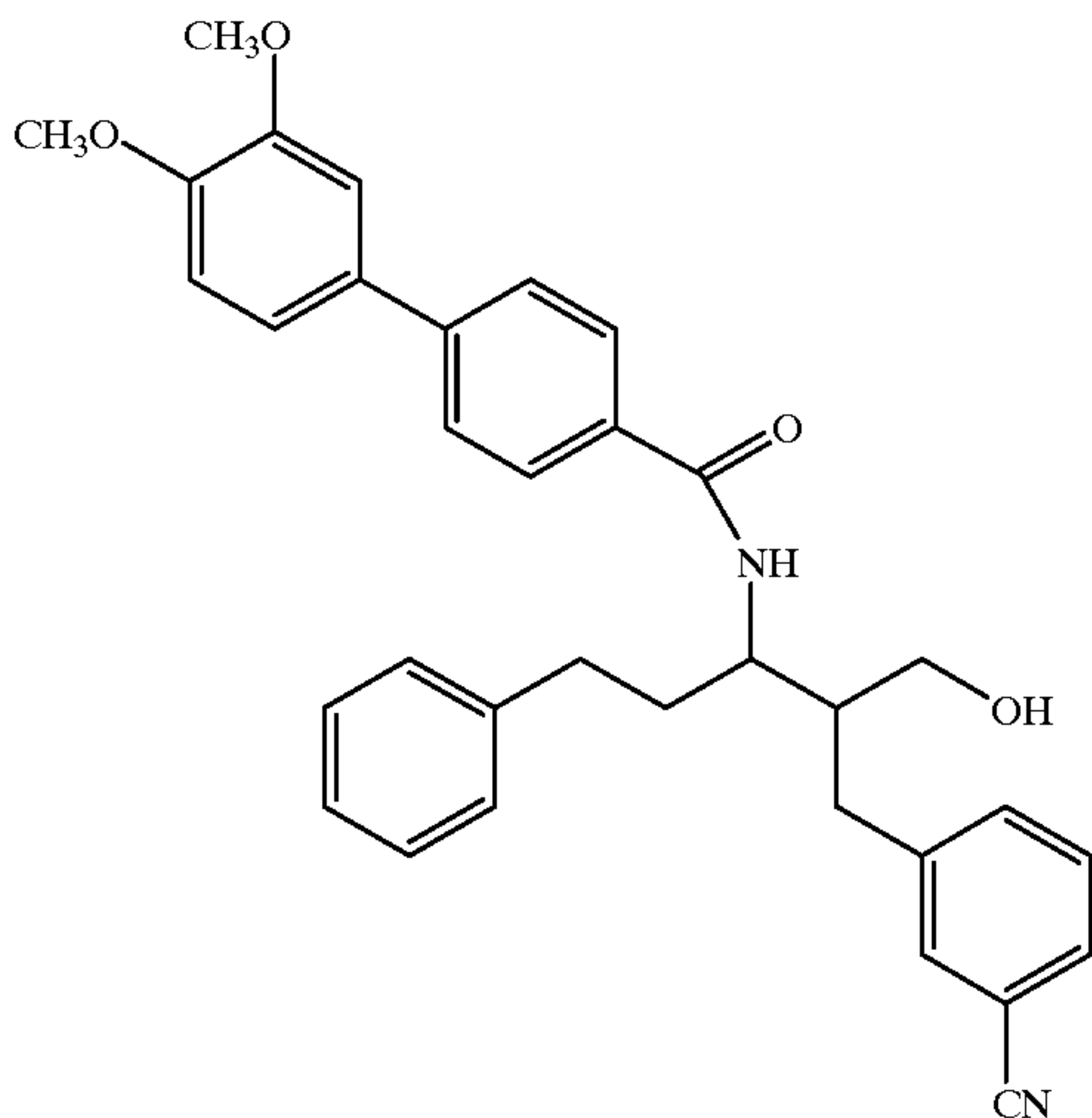
Compound 134
