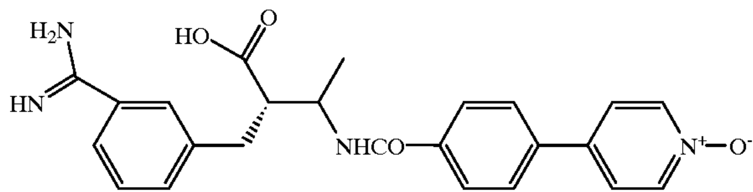
2-(3-Carbamimidoyl-benzyl)-3-[4-(1-oxy-pyridin-4-yl)-benzoylamino]-butyric acid trifluoroacetate.
