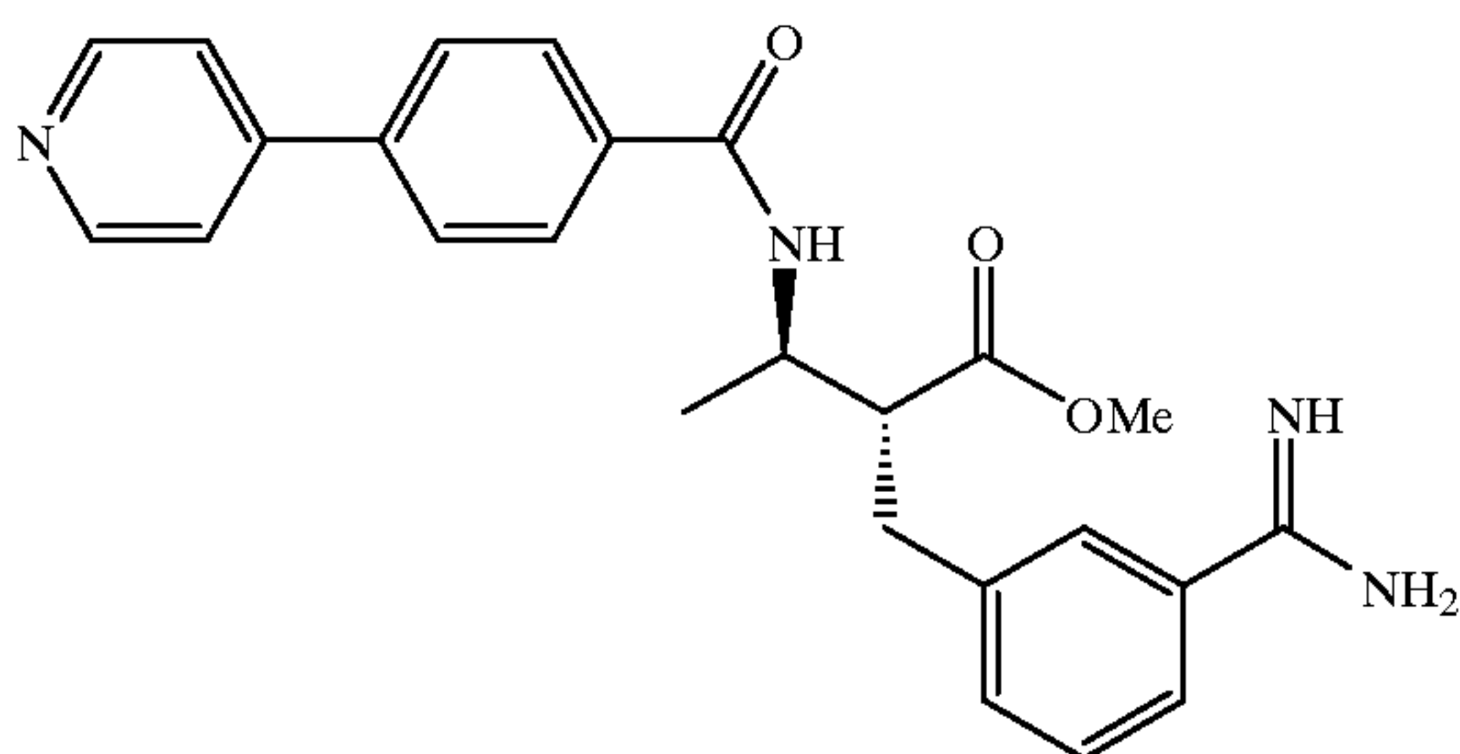
Compound 211
