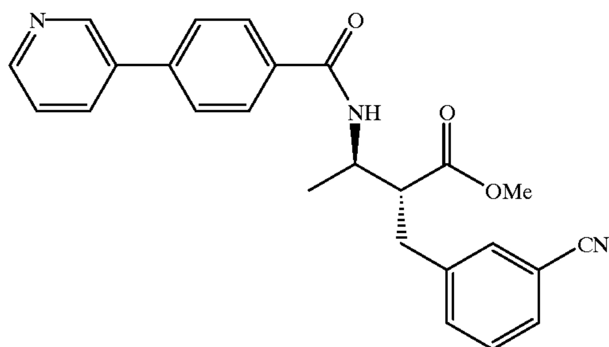
Compound 203
