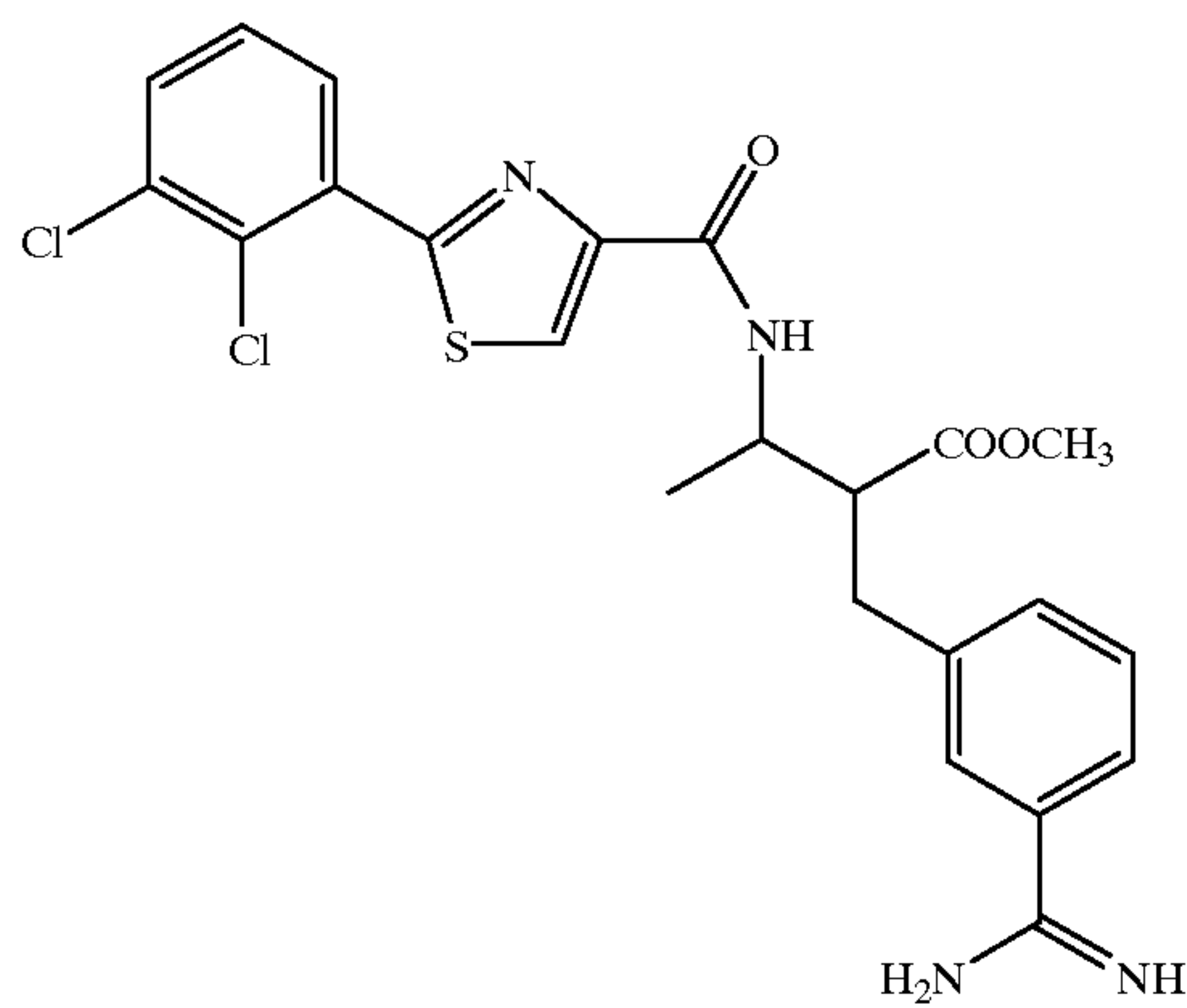
Compound 293
