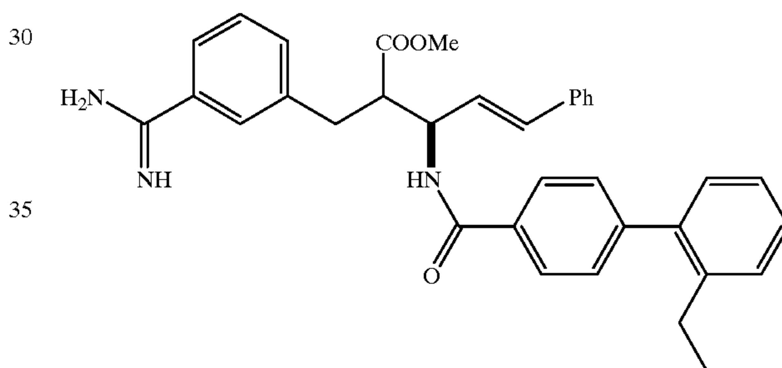
Compound 28
