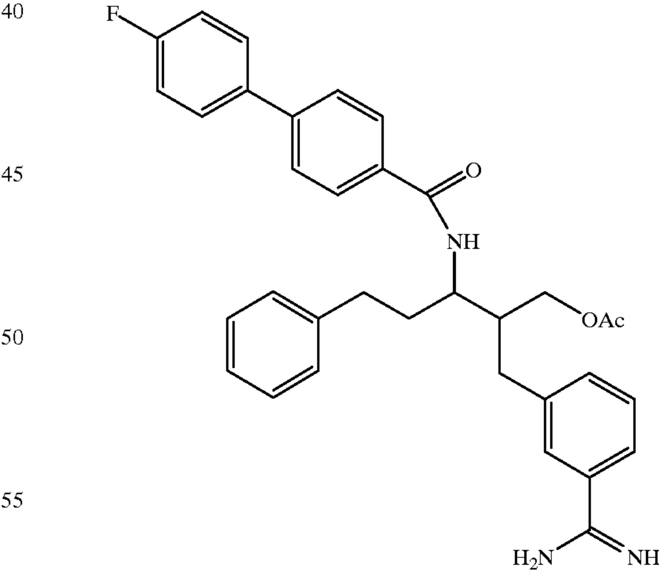
Compound 164
