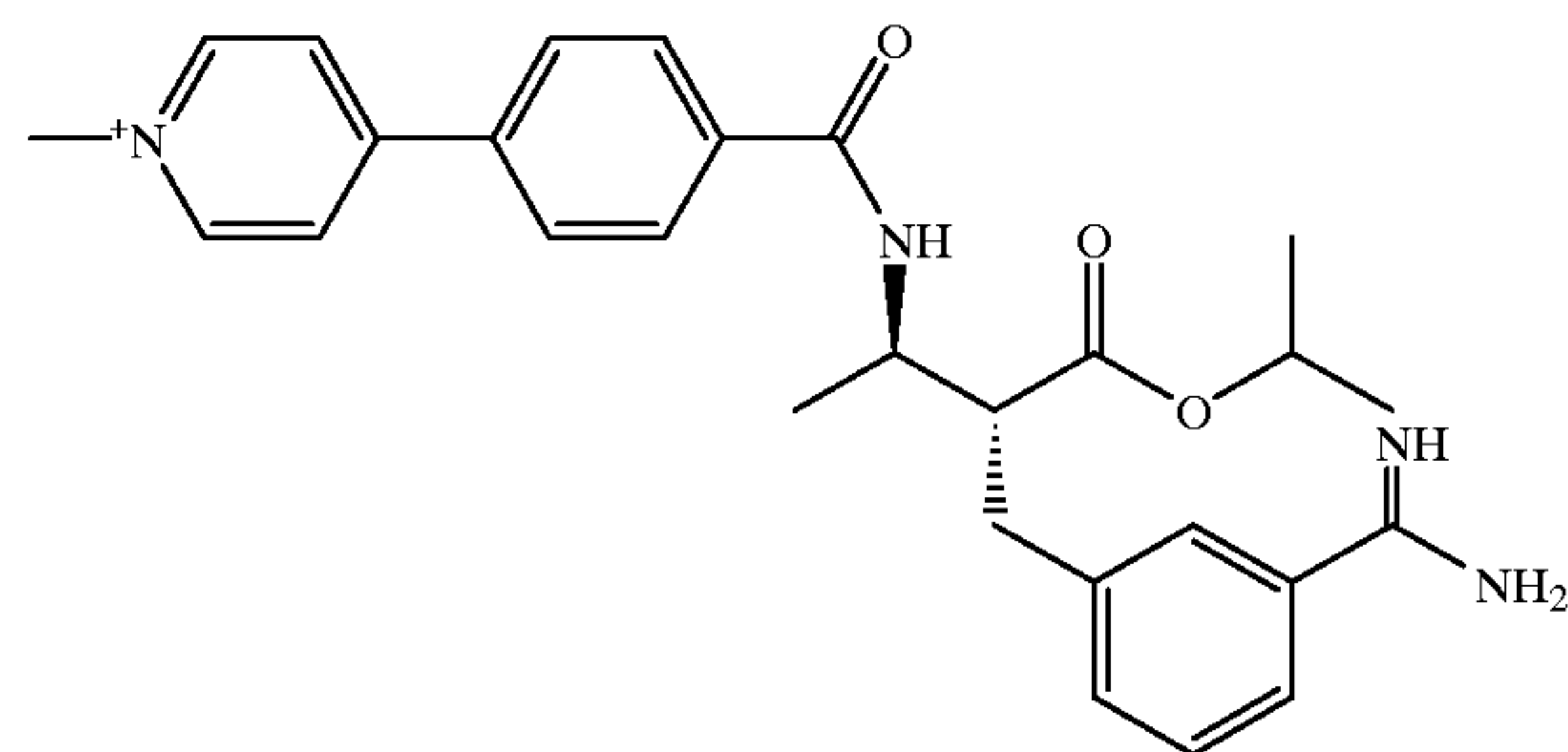
Compound 221
