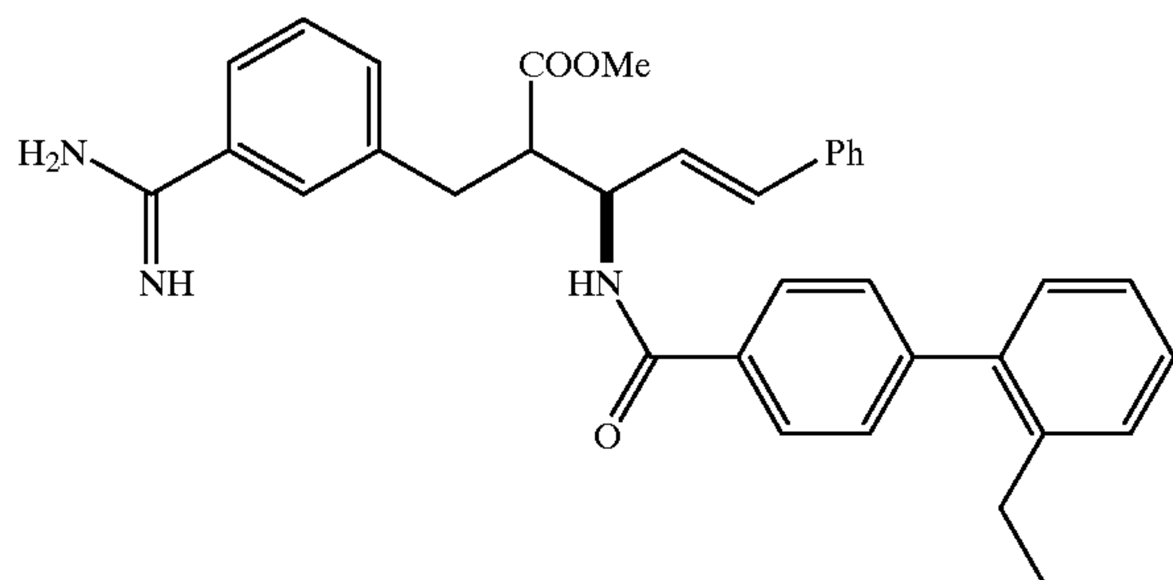
Compound 25
