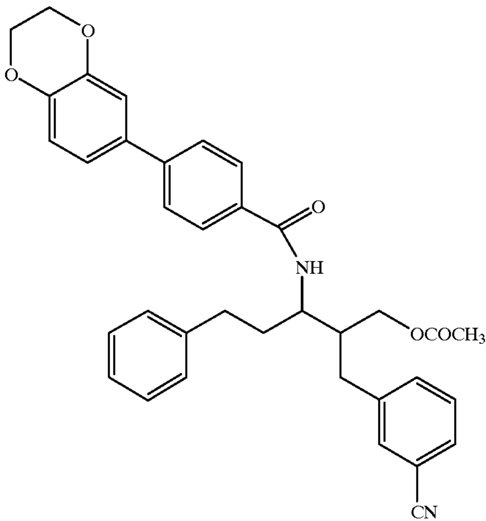
Compound 148
