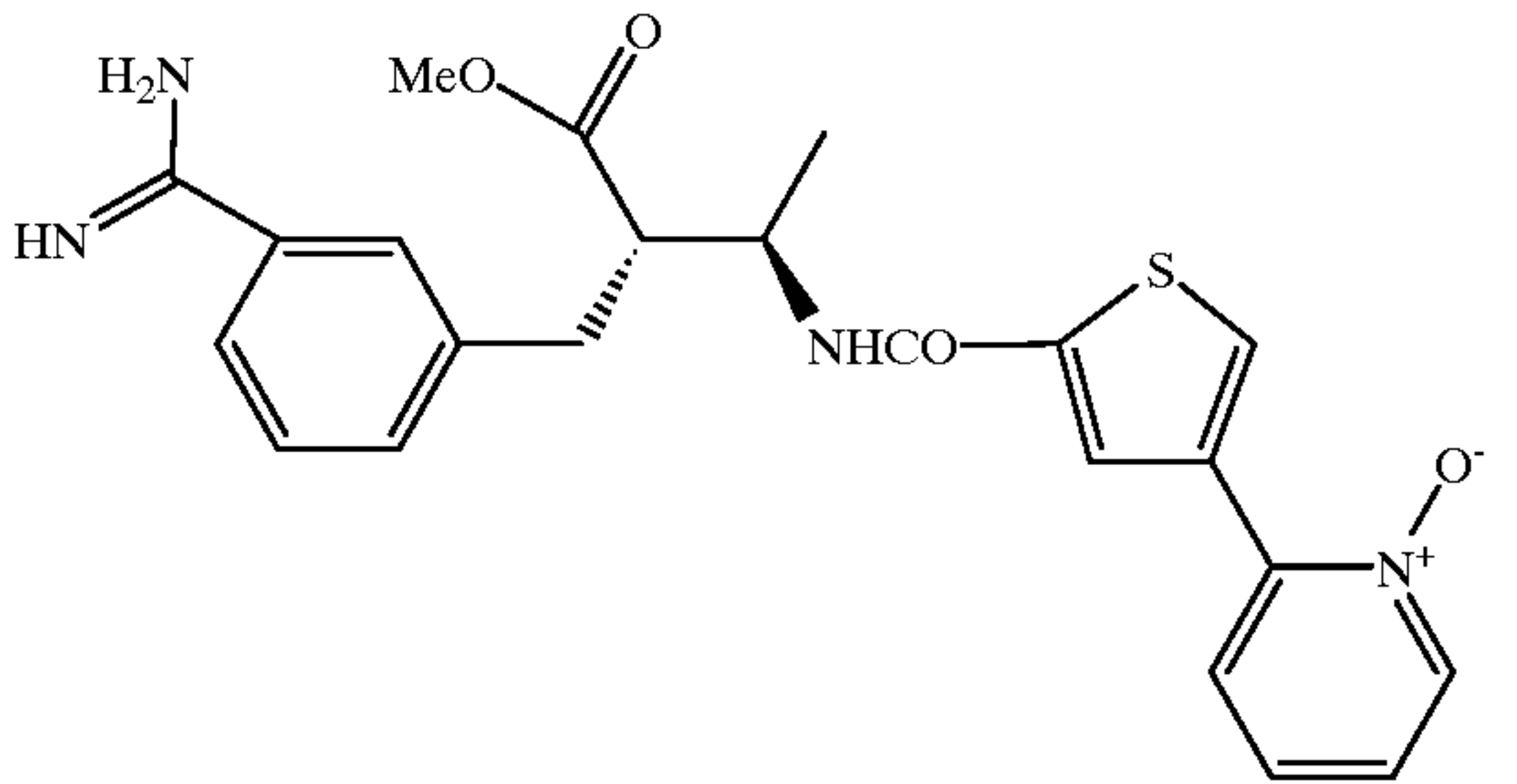
Compound 340
