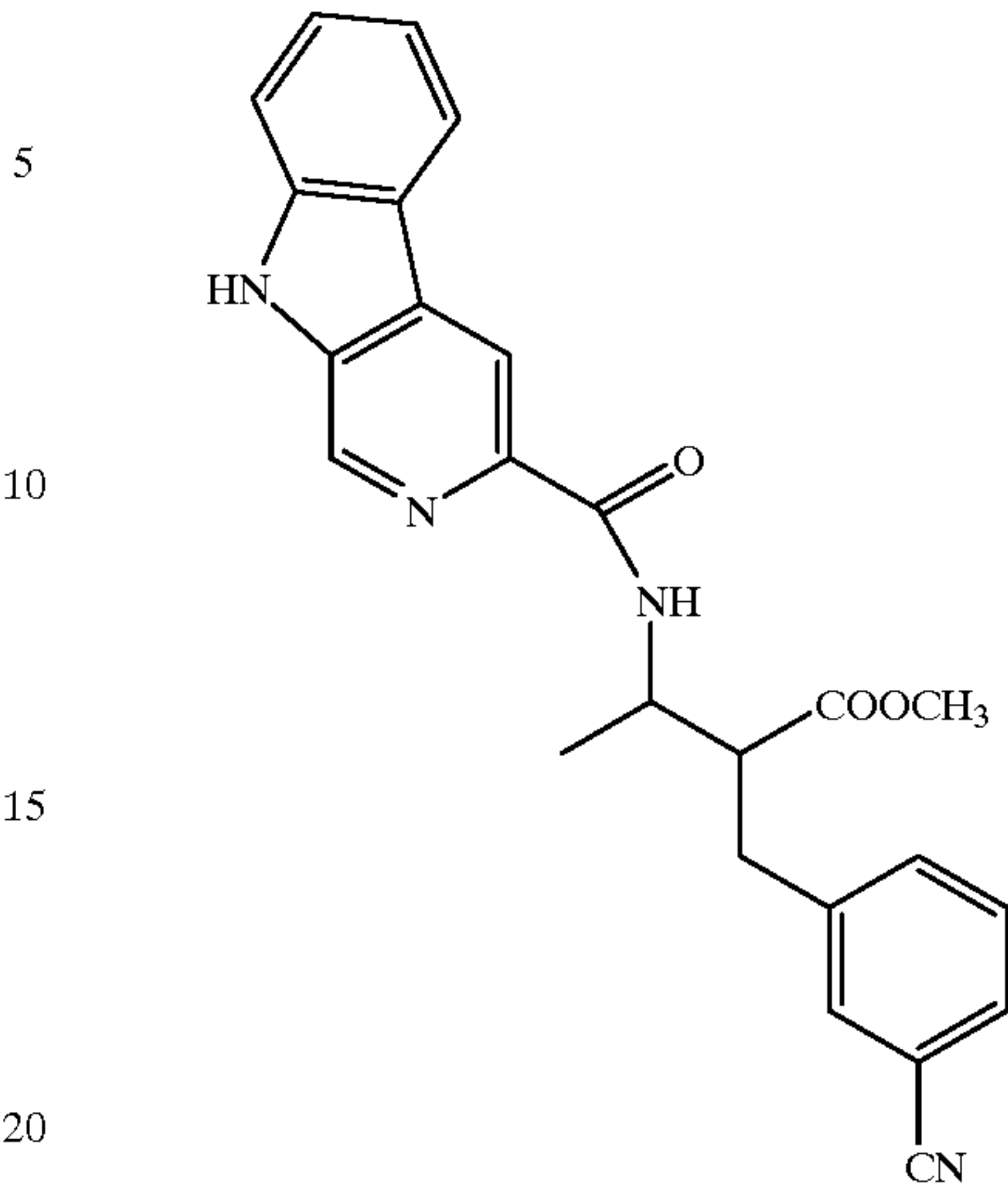
Compound 261
