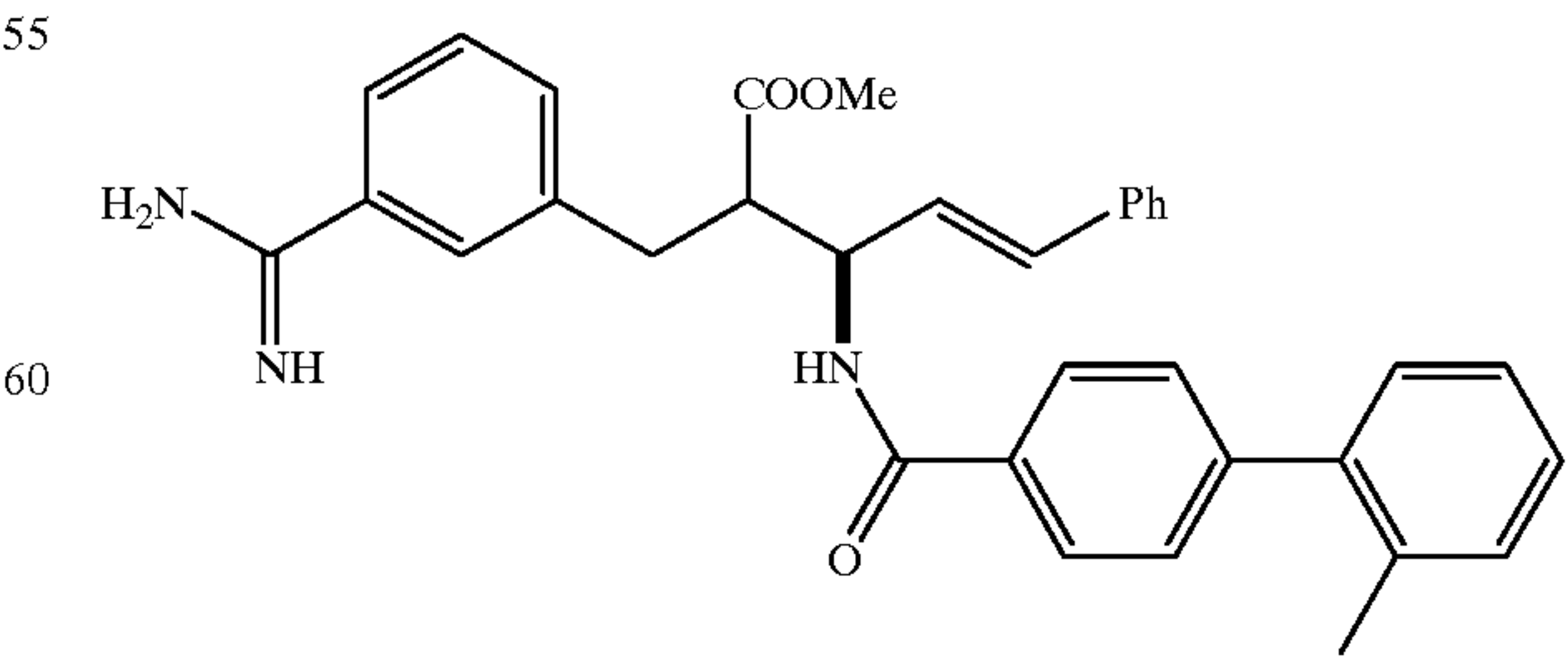
Compound 19
