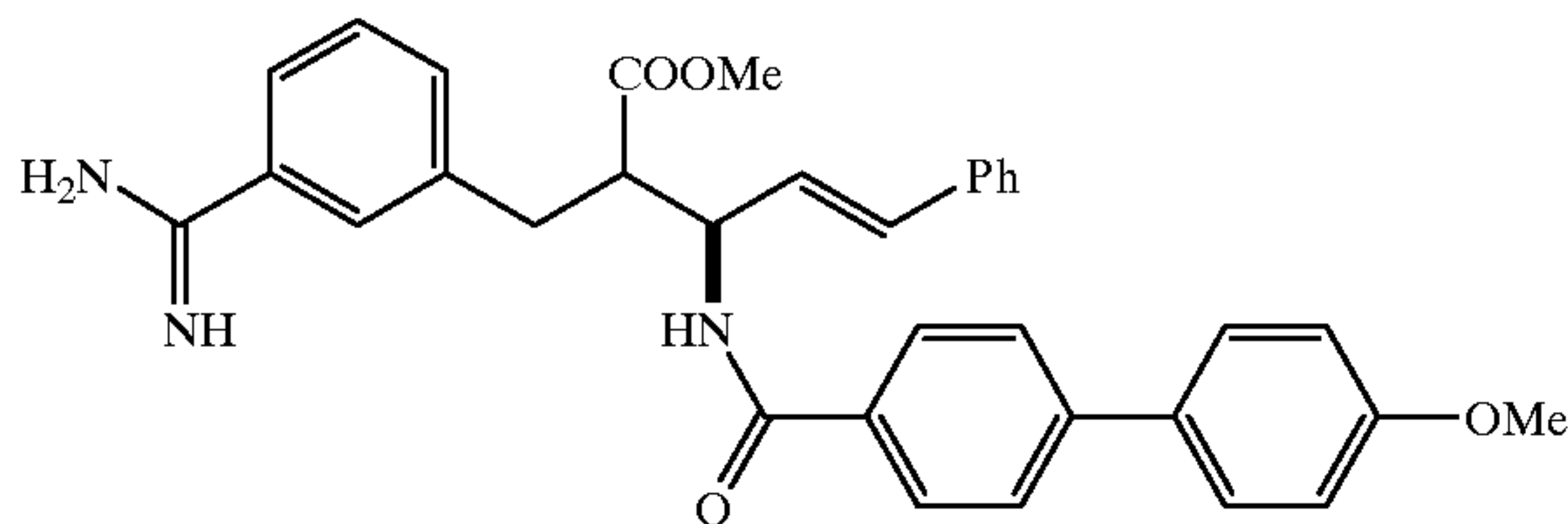
Compound 26
