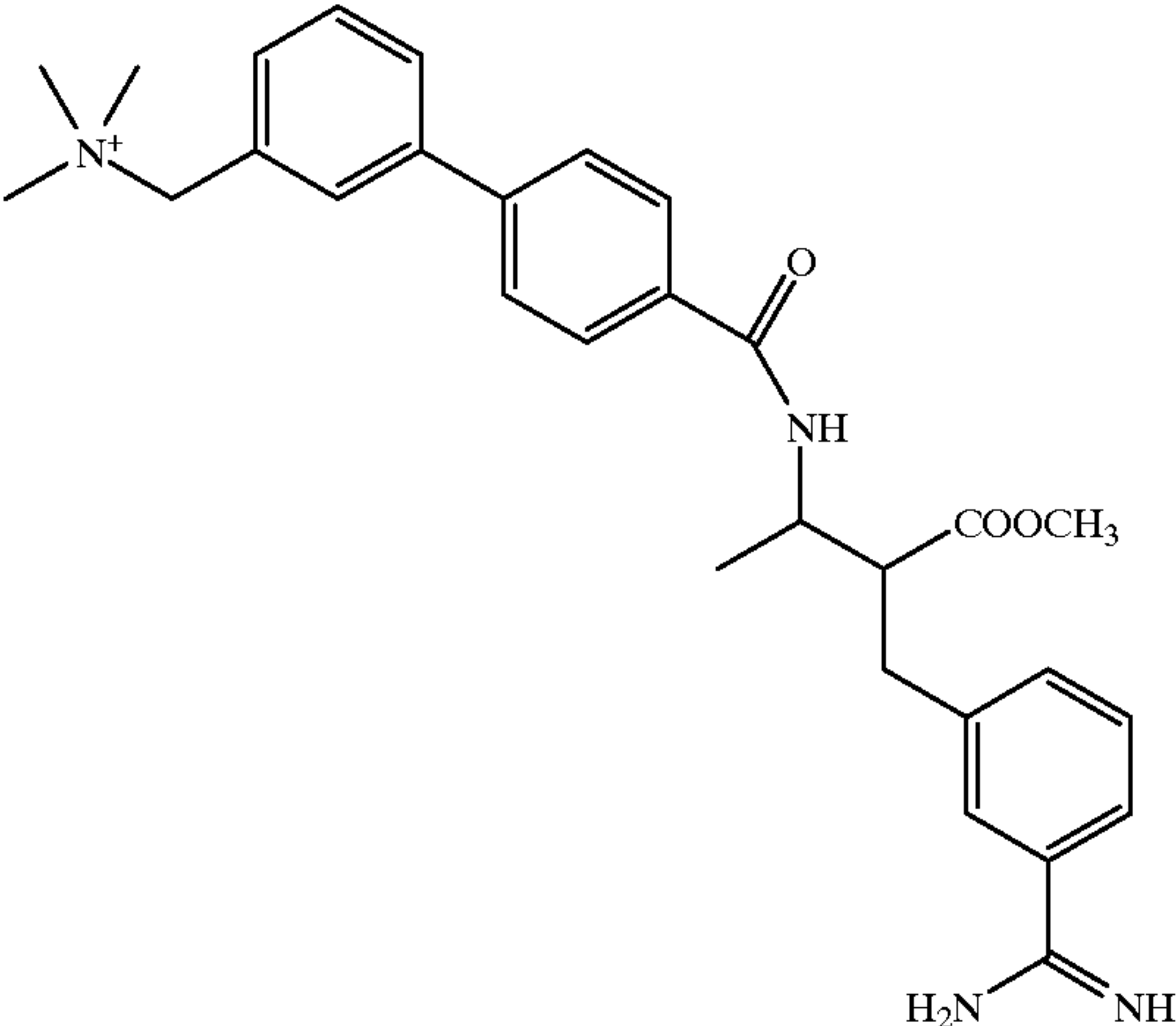
Compound 191
