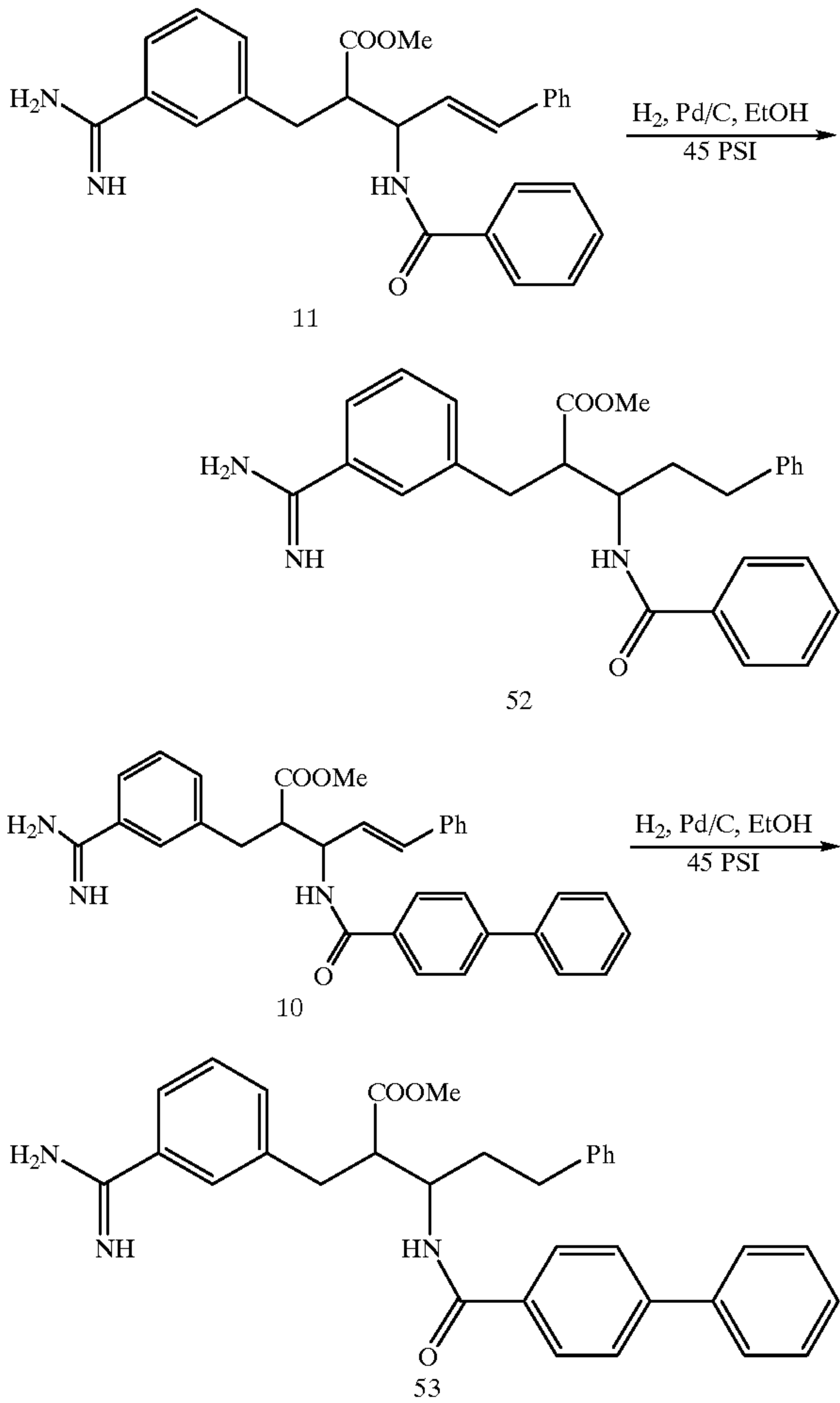
SCHEME E
