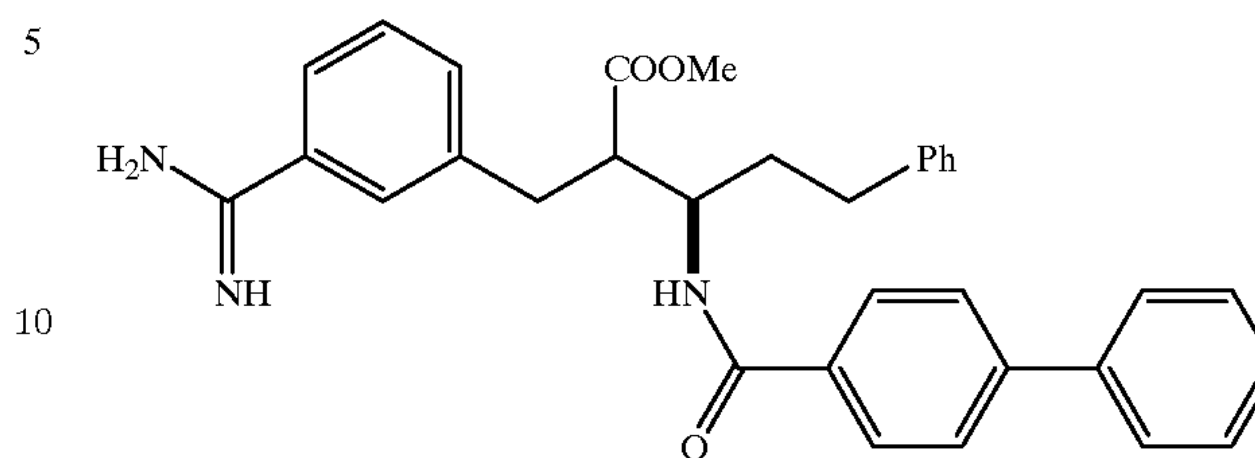
Compound 55
