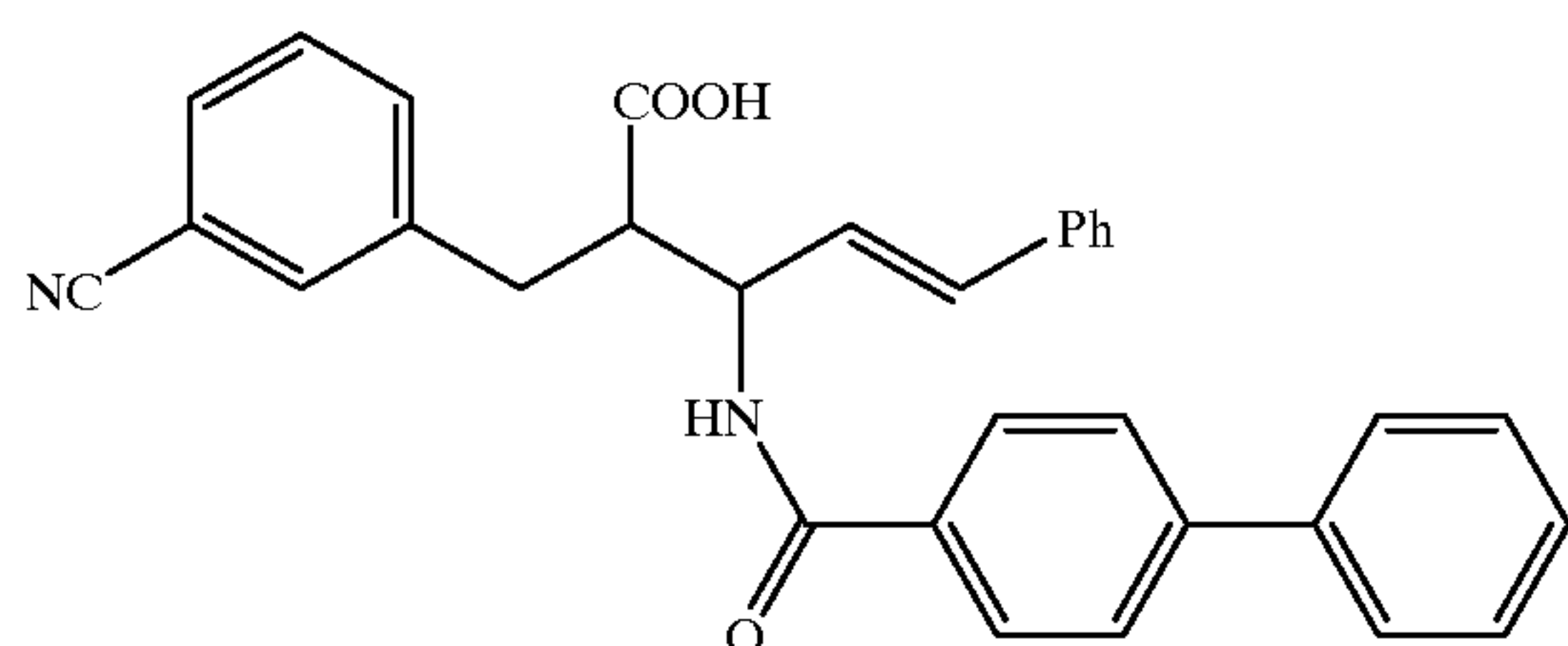
Compound 9
