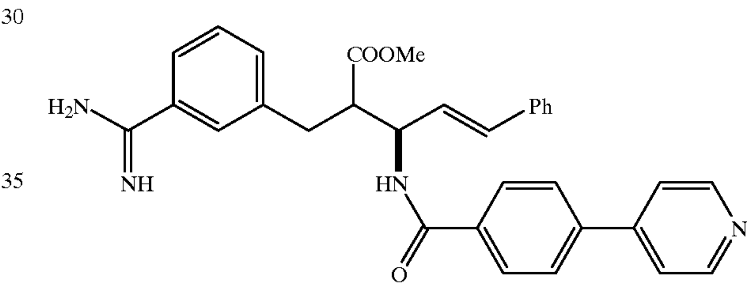
Compound 18
