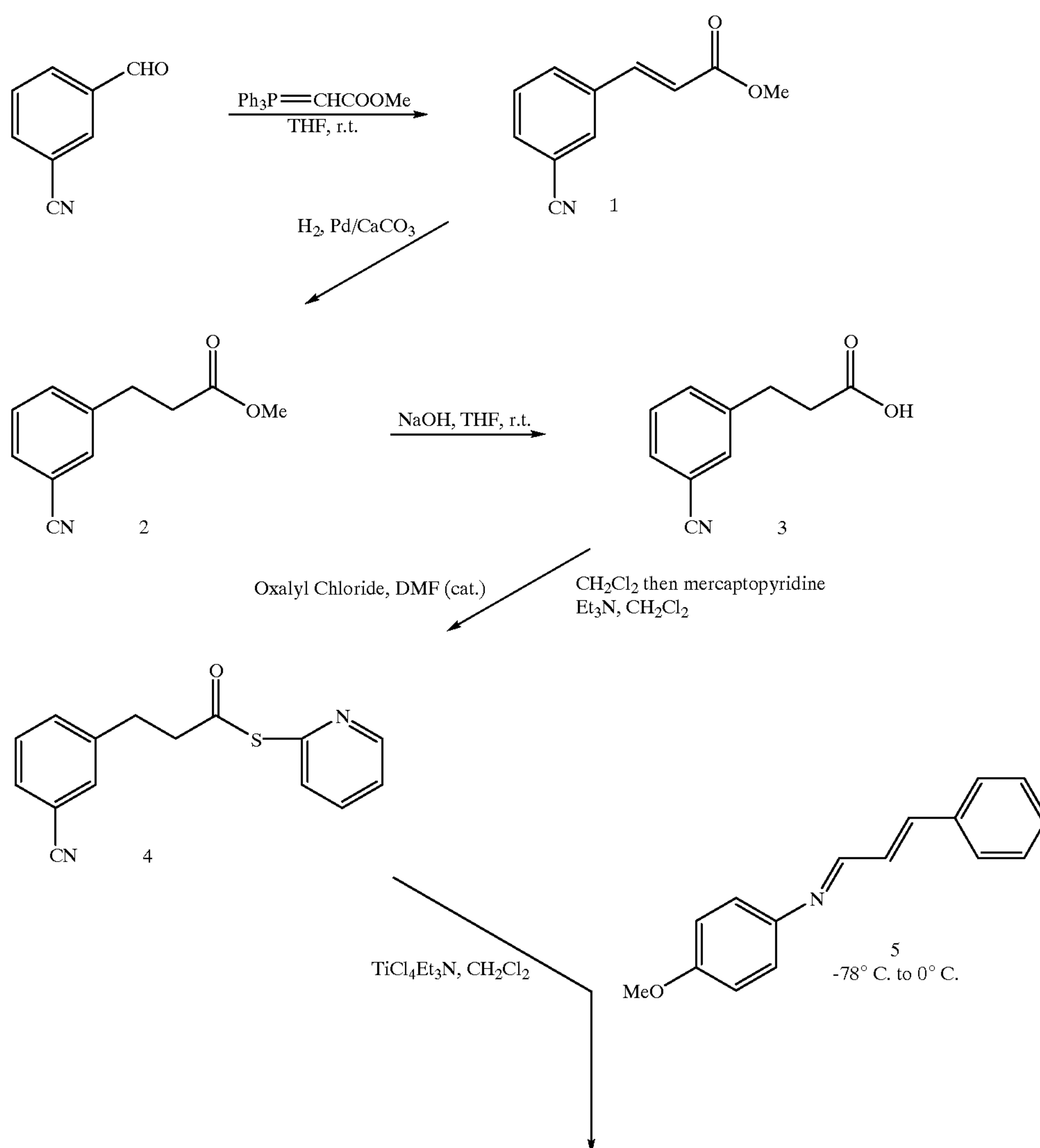
SCHEME A
