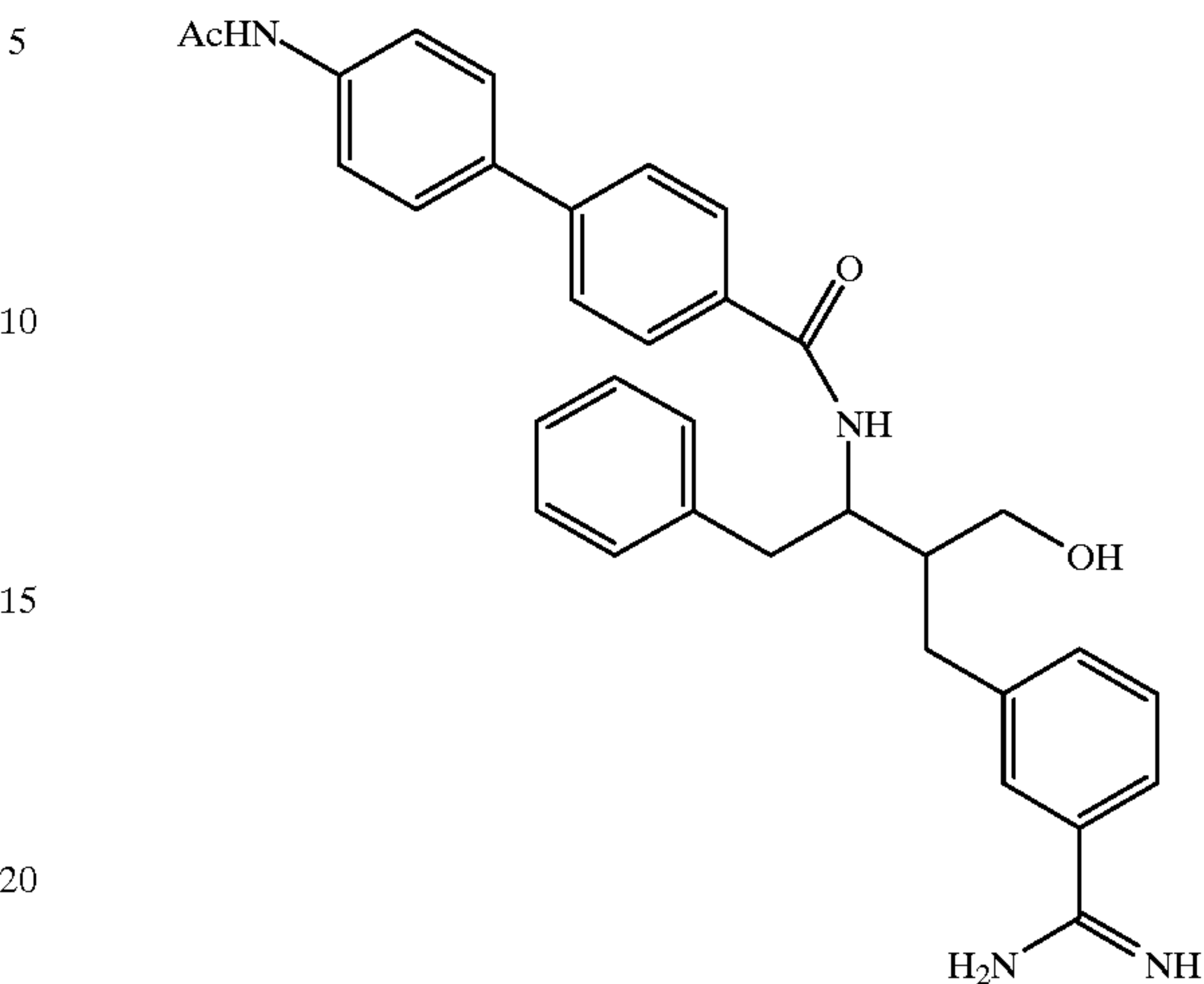
Compound 183
