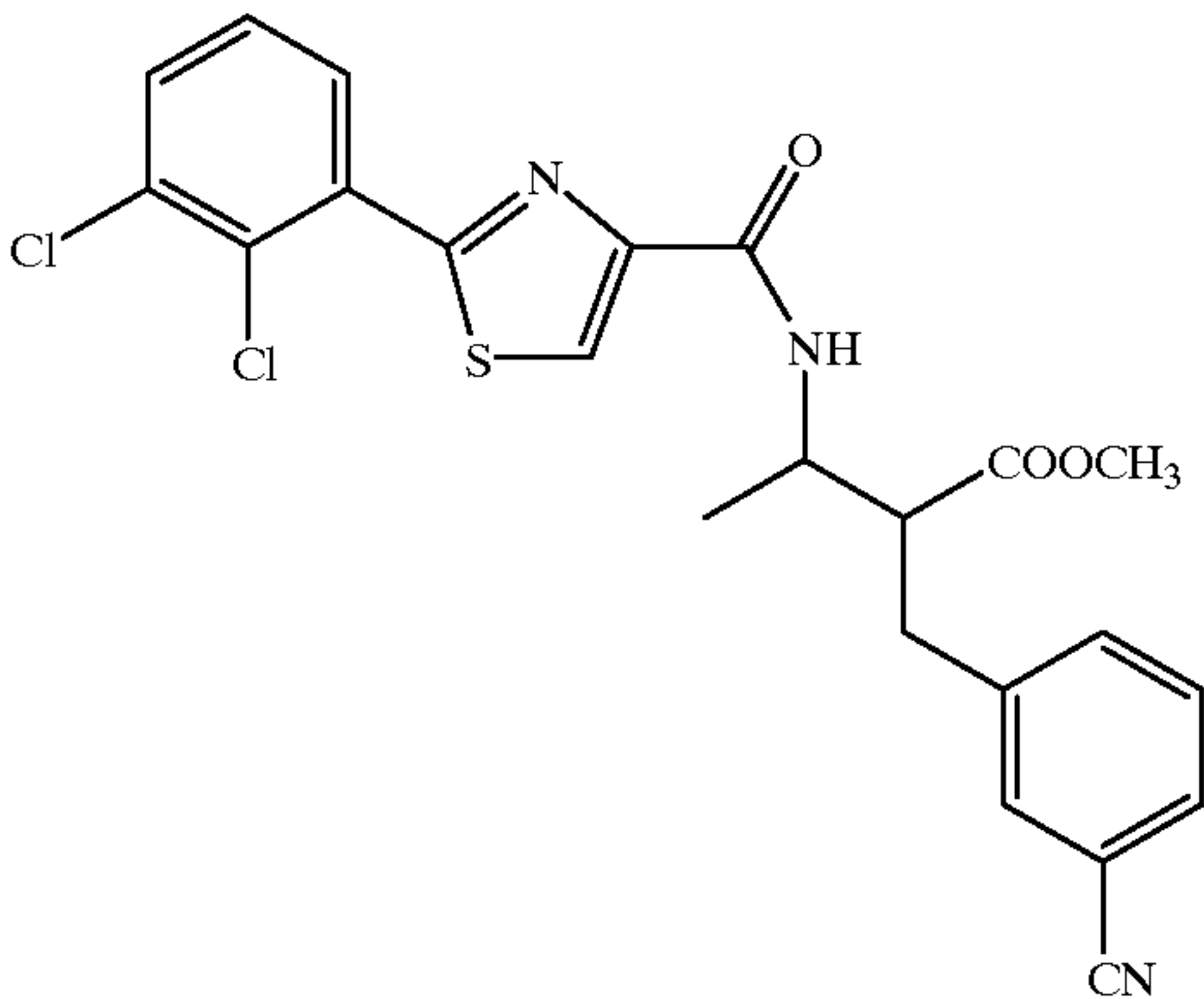
Compound 261
