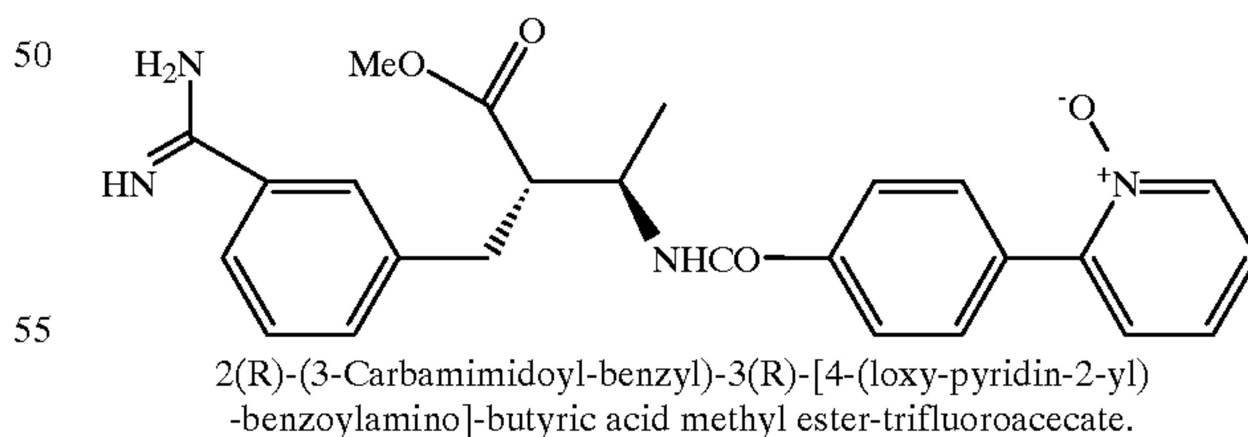
2-(3-Carbamimidoyl-benzyl)-3-[4-(1-oxy-pyridin-4-yl)-benzoylamino]-butyric acid trifluoroacetate.
