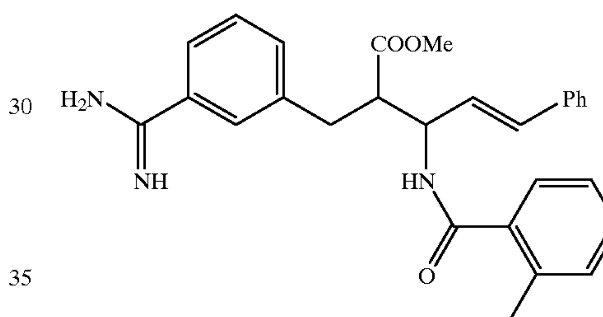
Compound 10
