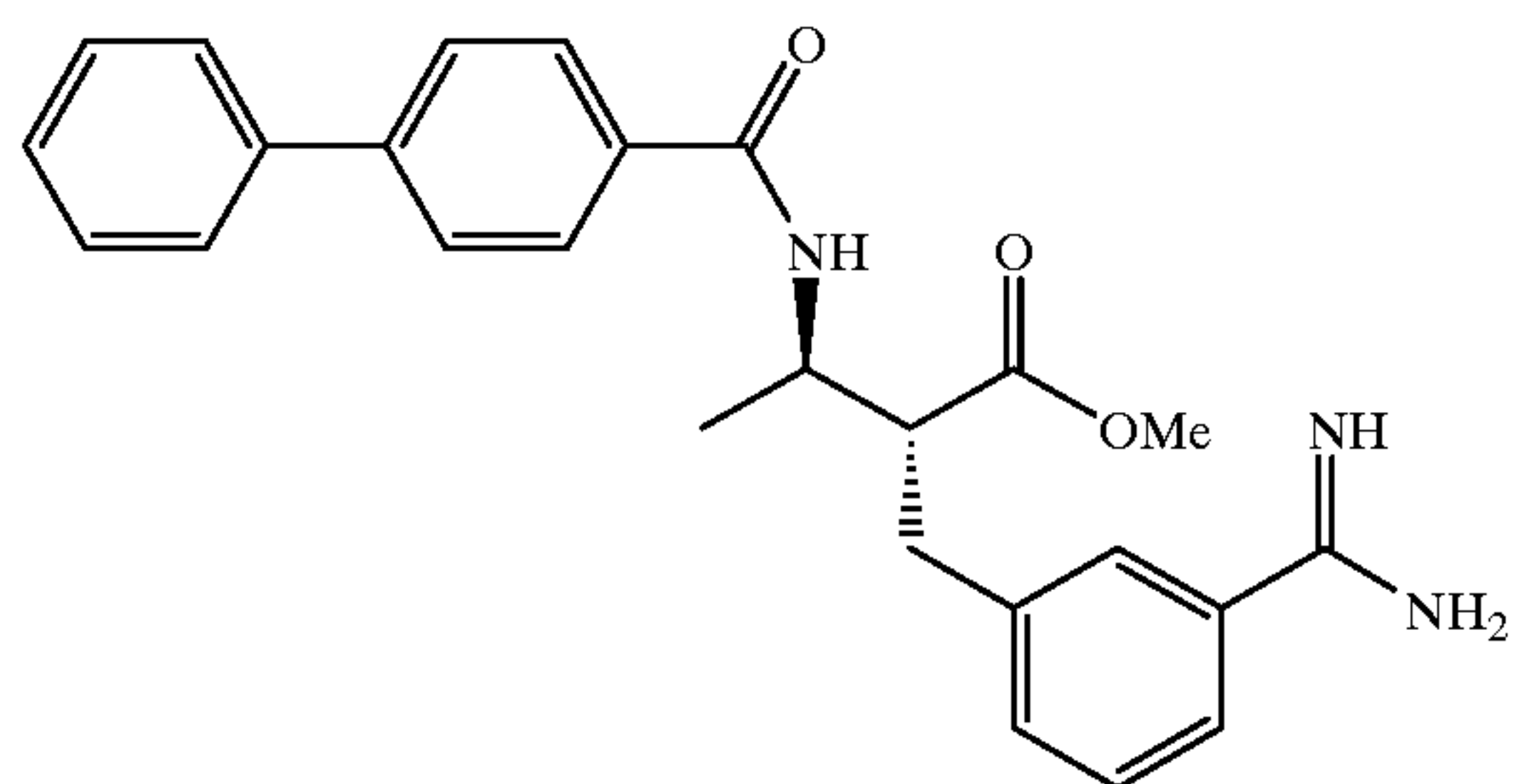
Compound 212
