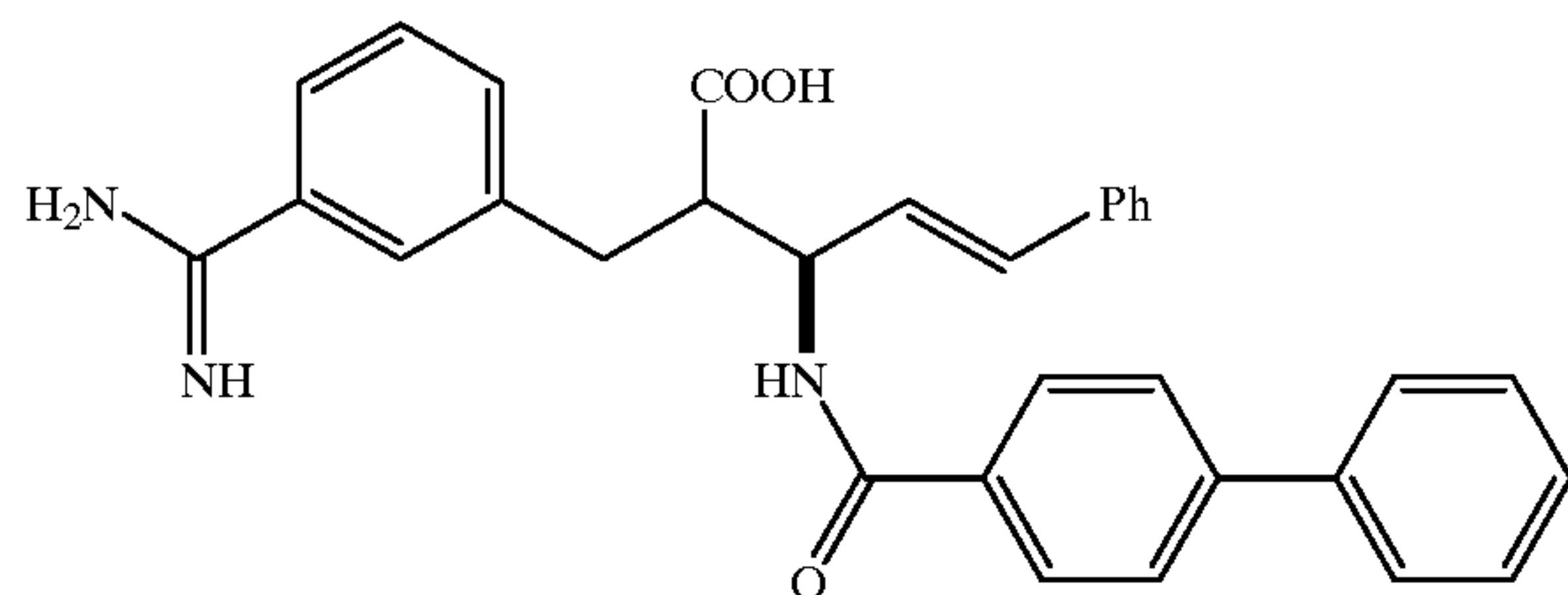
Compound 47
