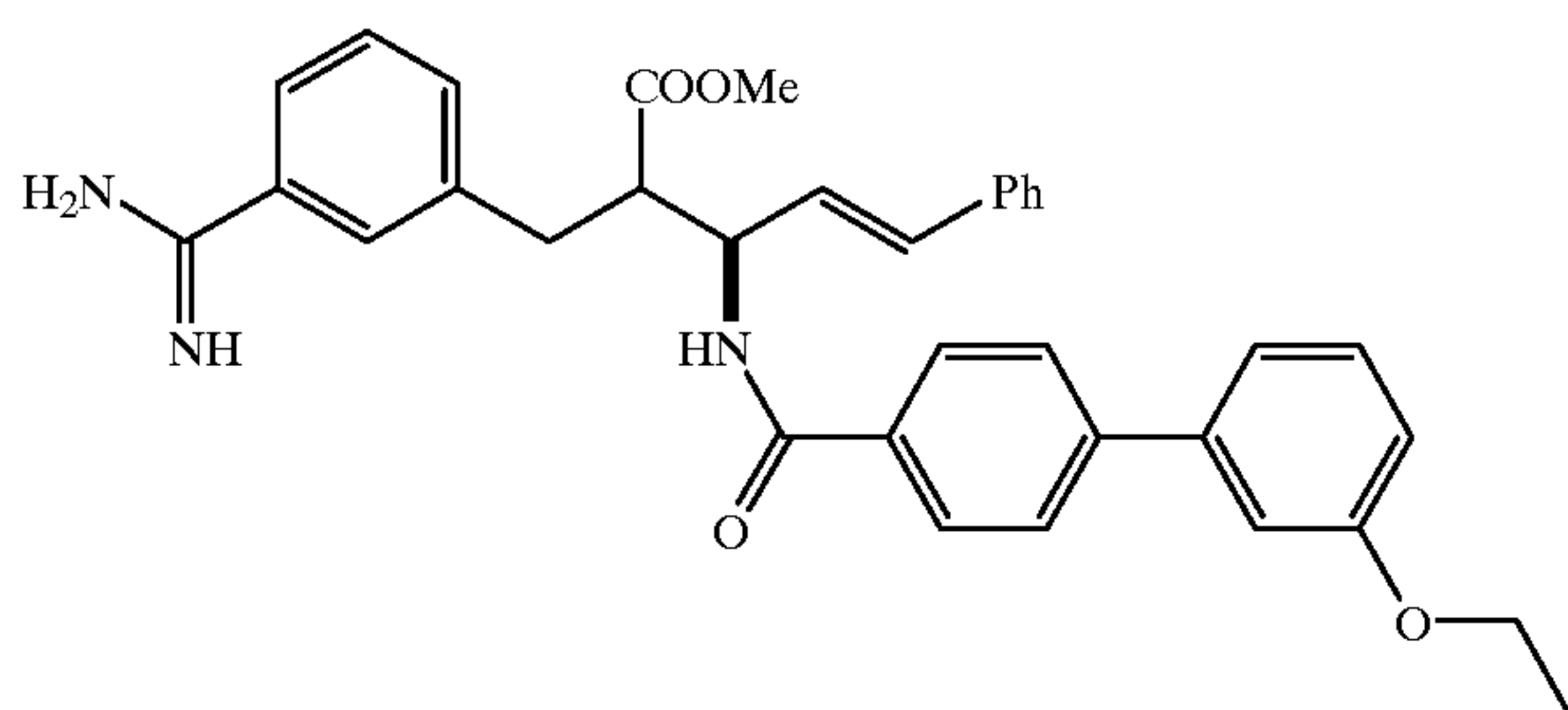
Compound 30
