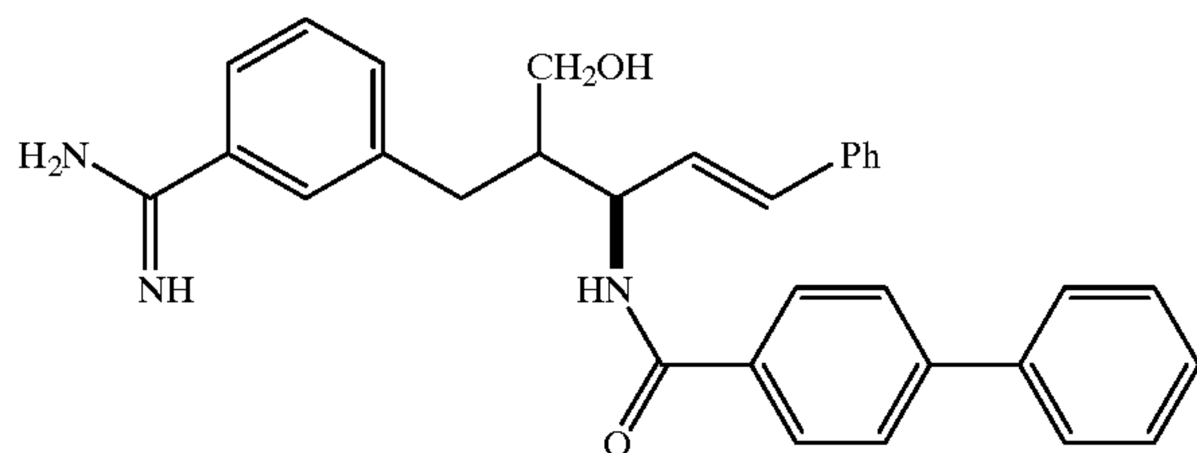
Compound 42
