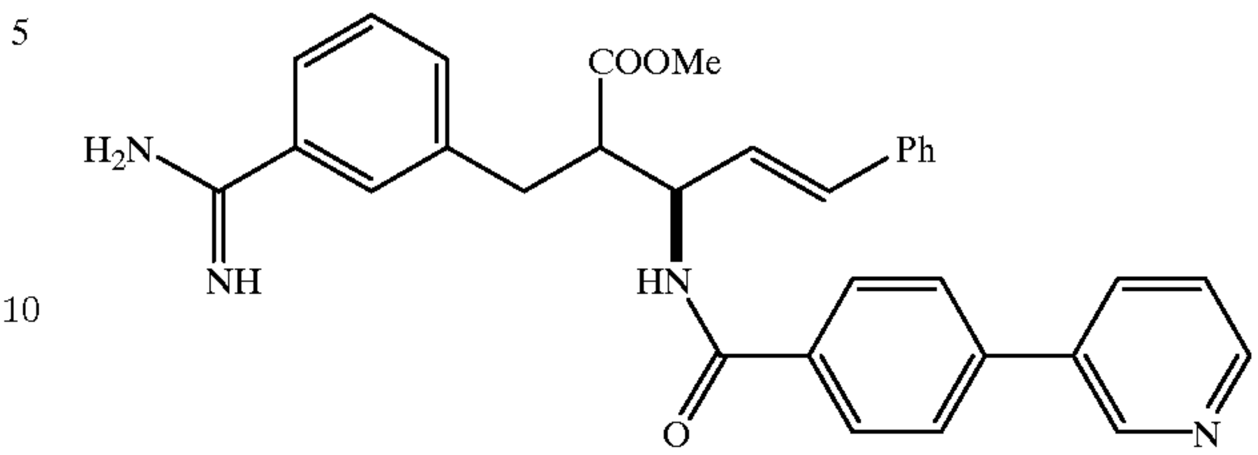
Compound 17
