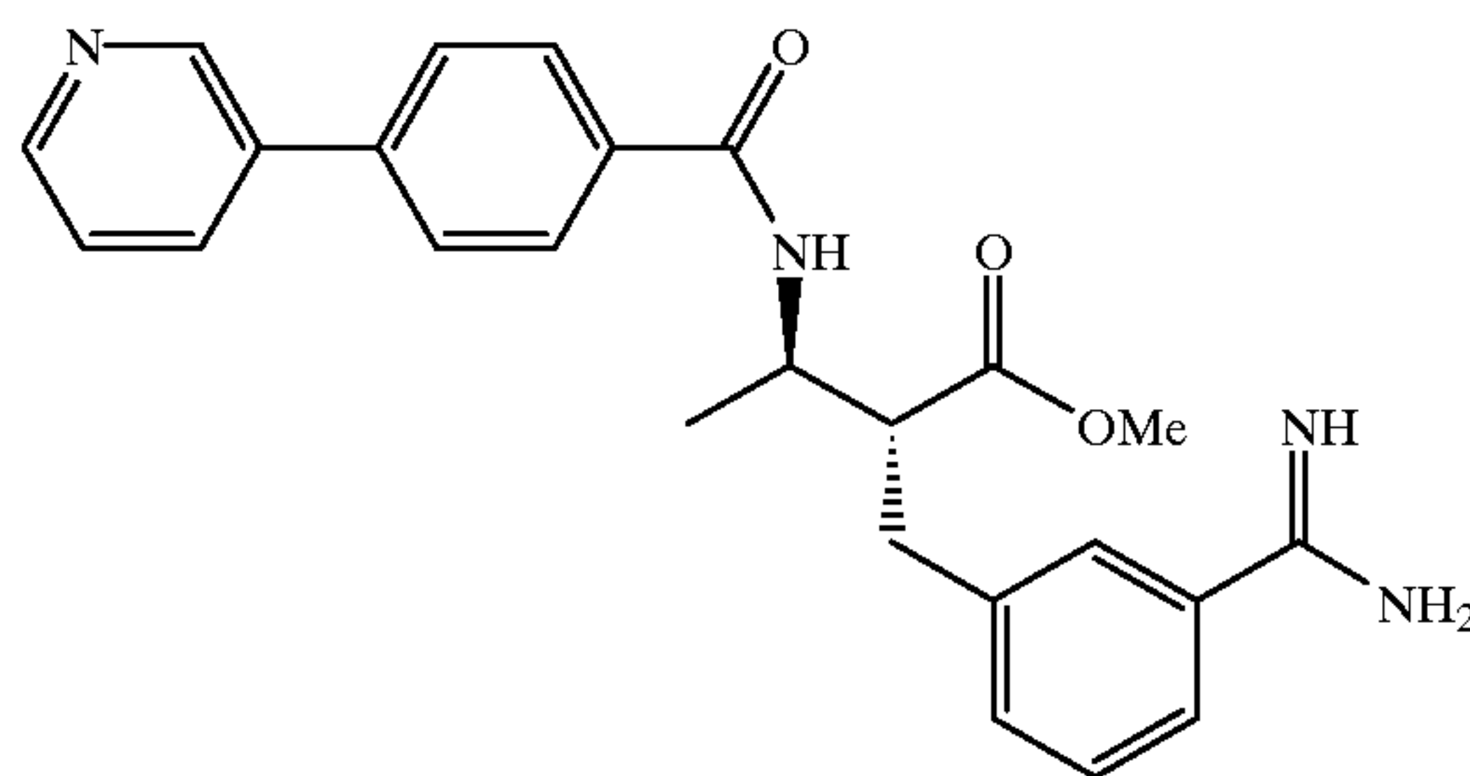
Compound 210
