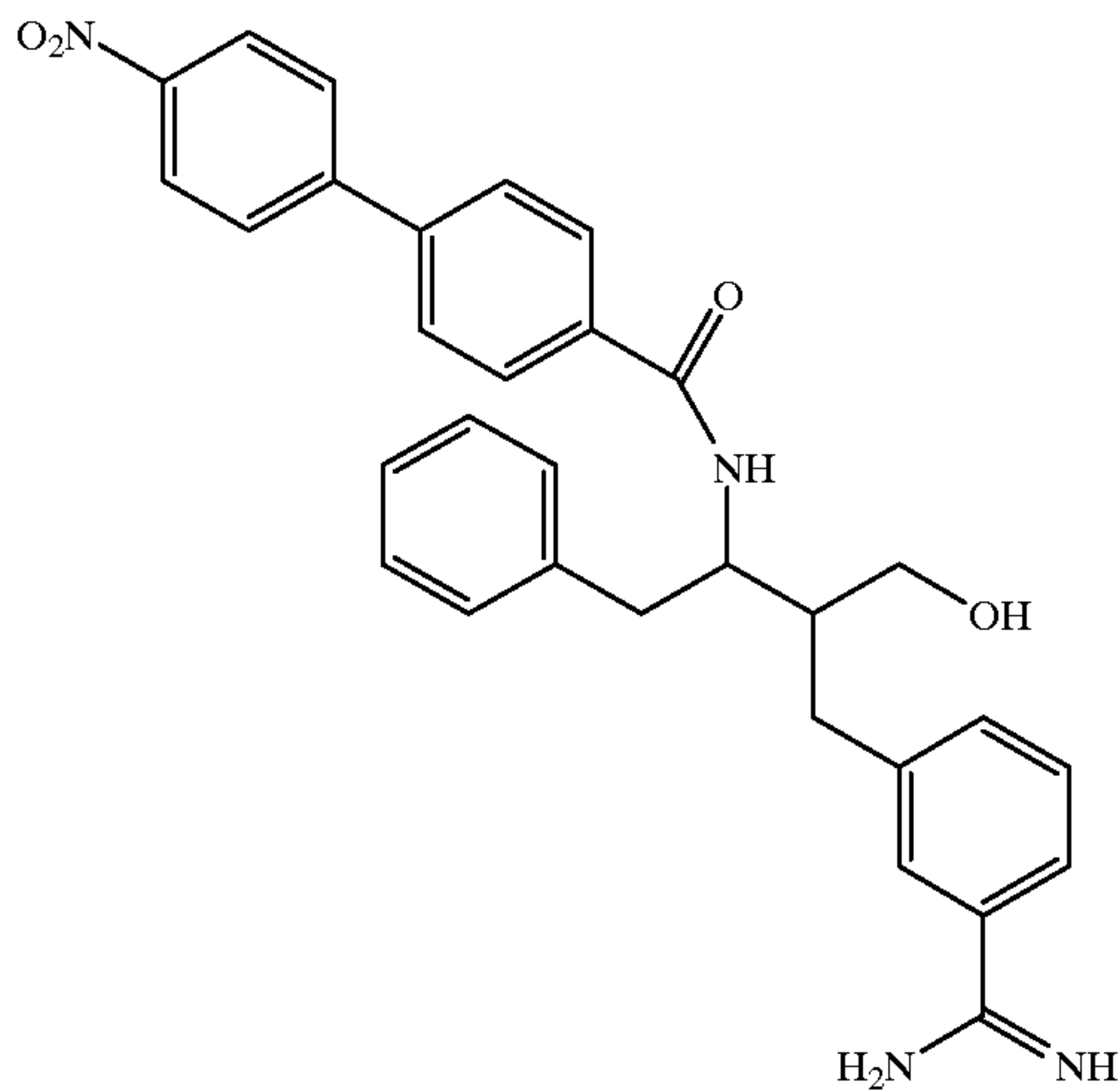
Compound 177
