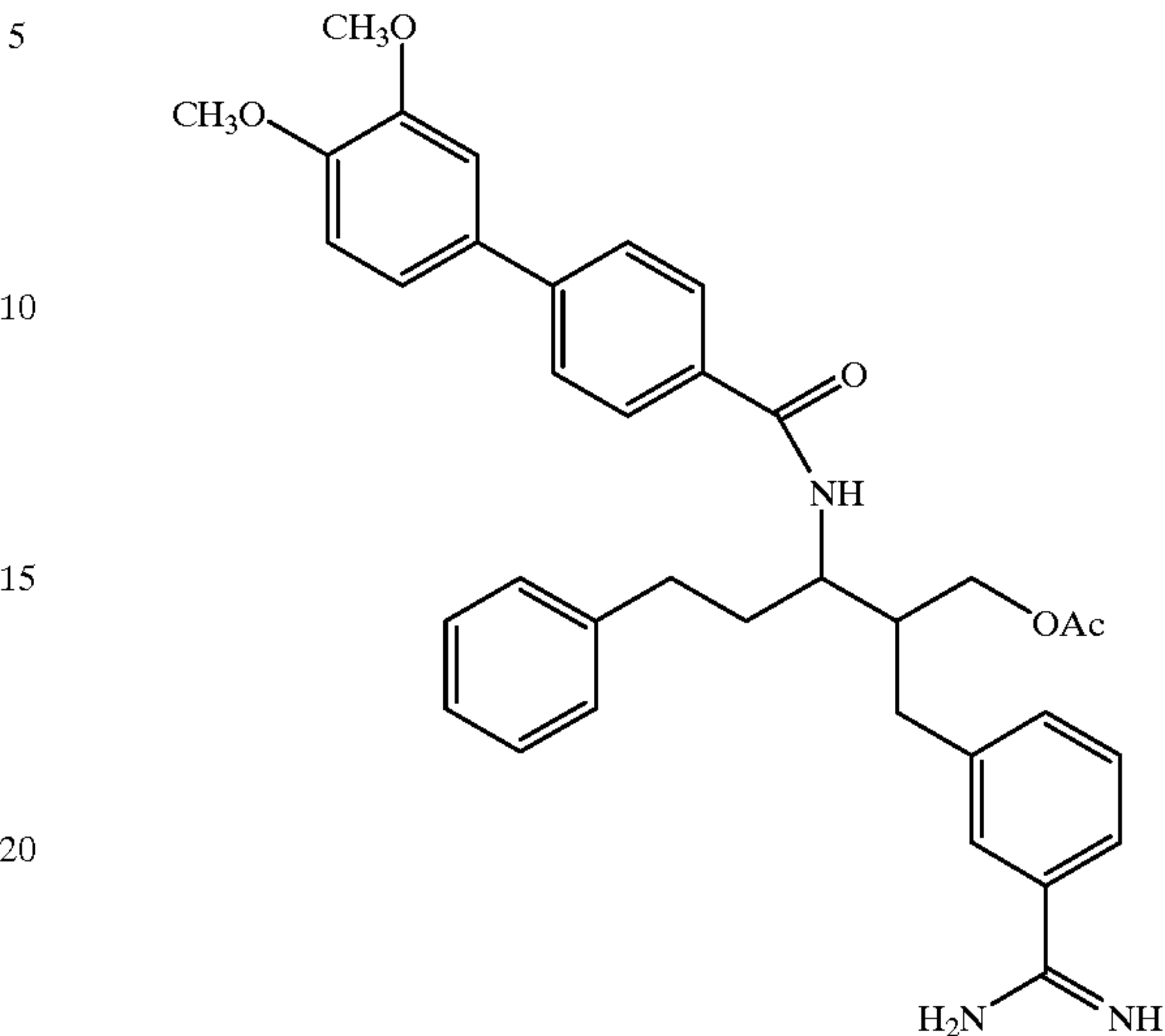
Compound 167
