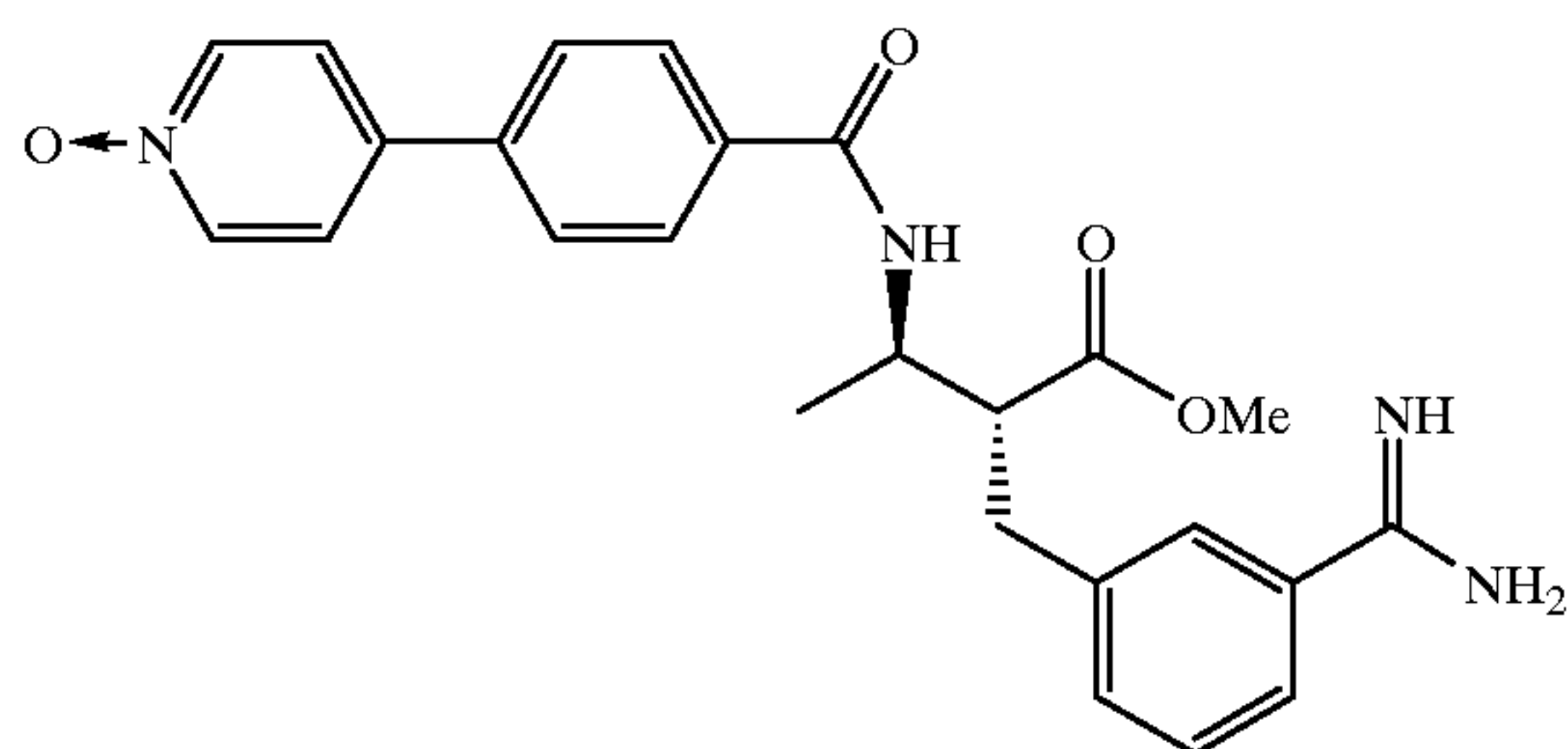
Compound 209
