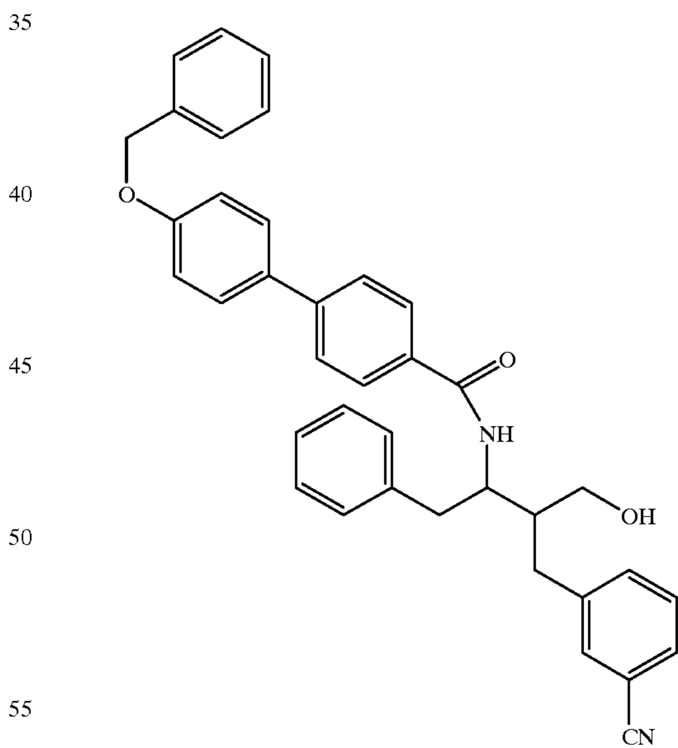
Compound 141
