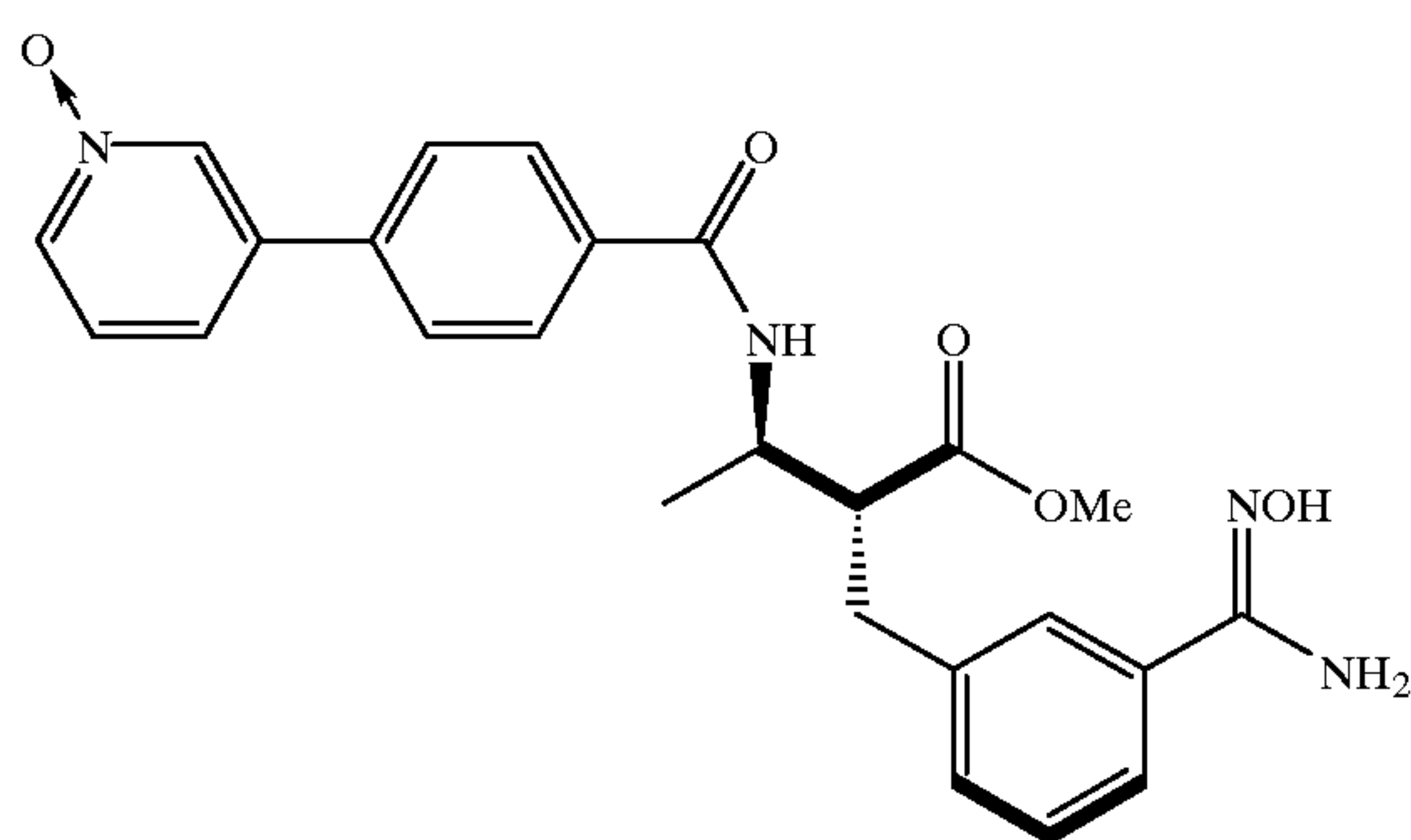
Compound 218
