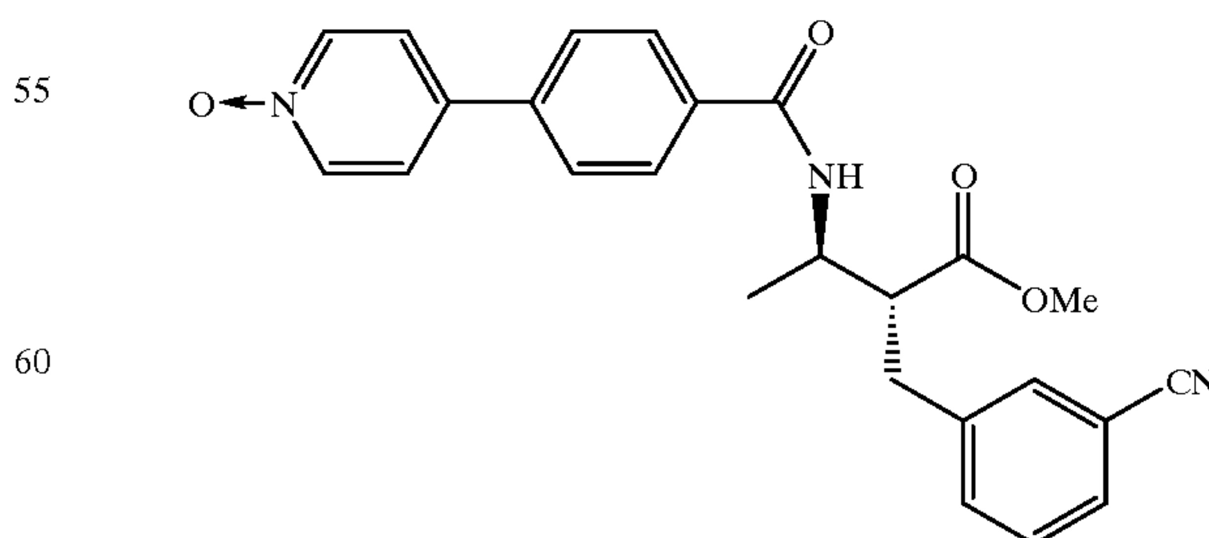
Compound 207
