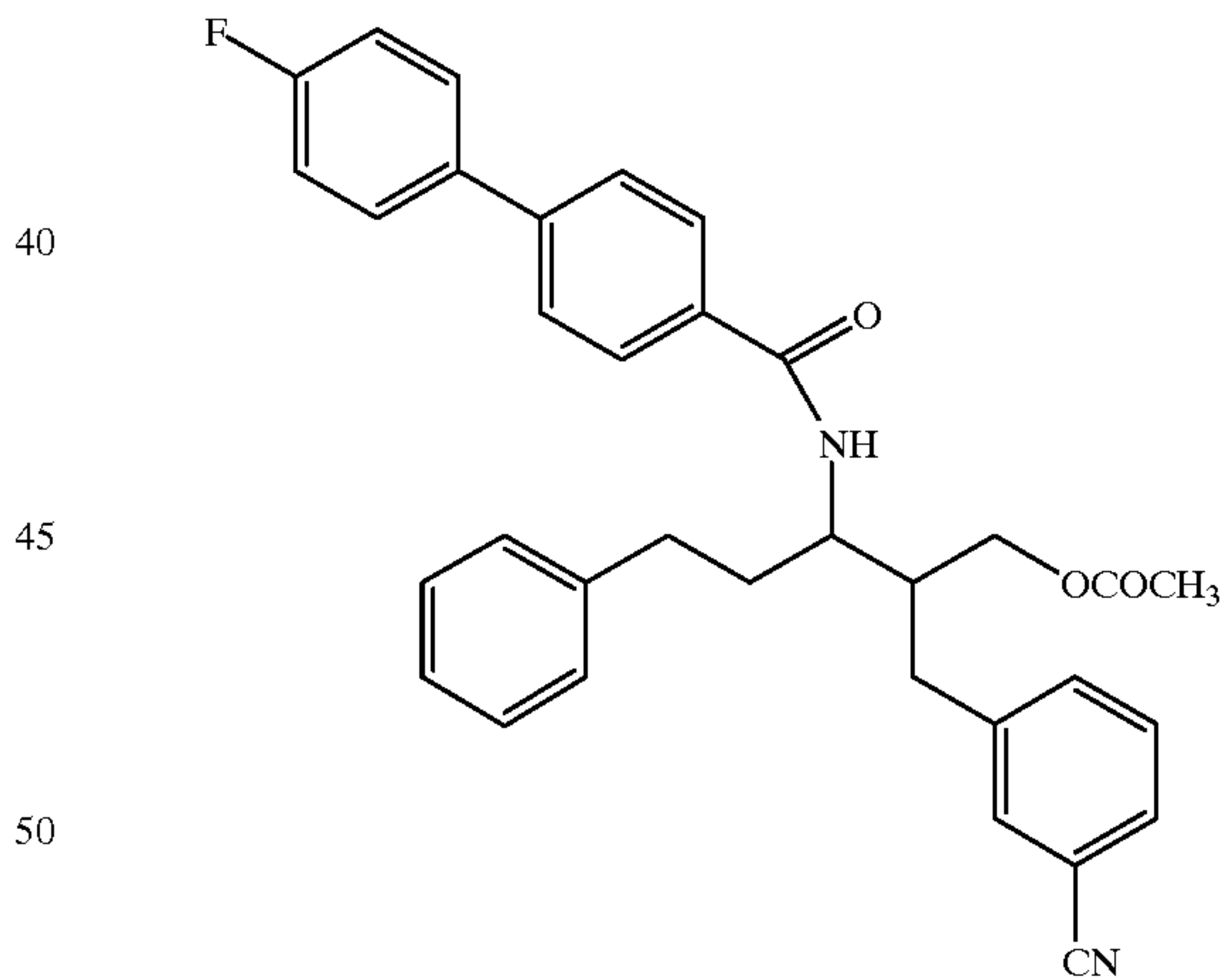
Compound 151
