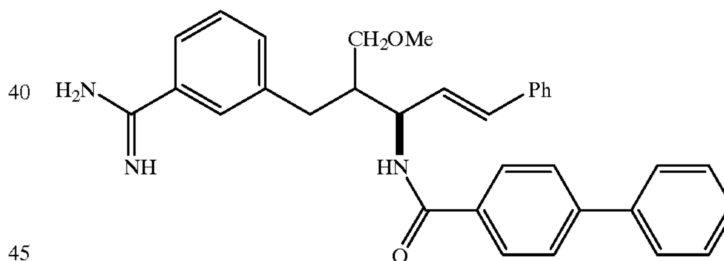
Compound 42
