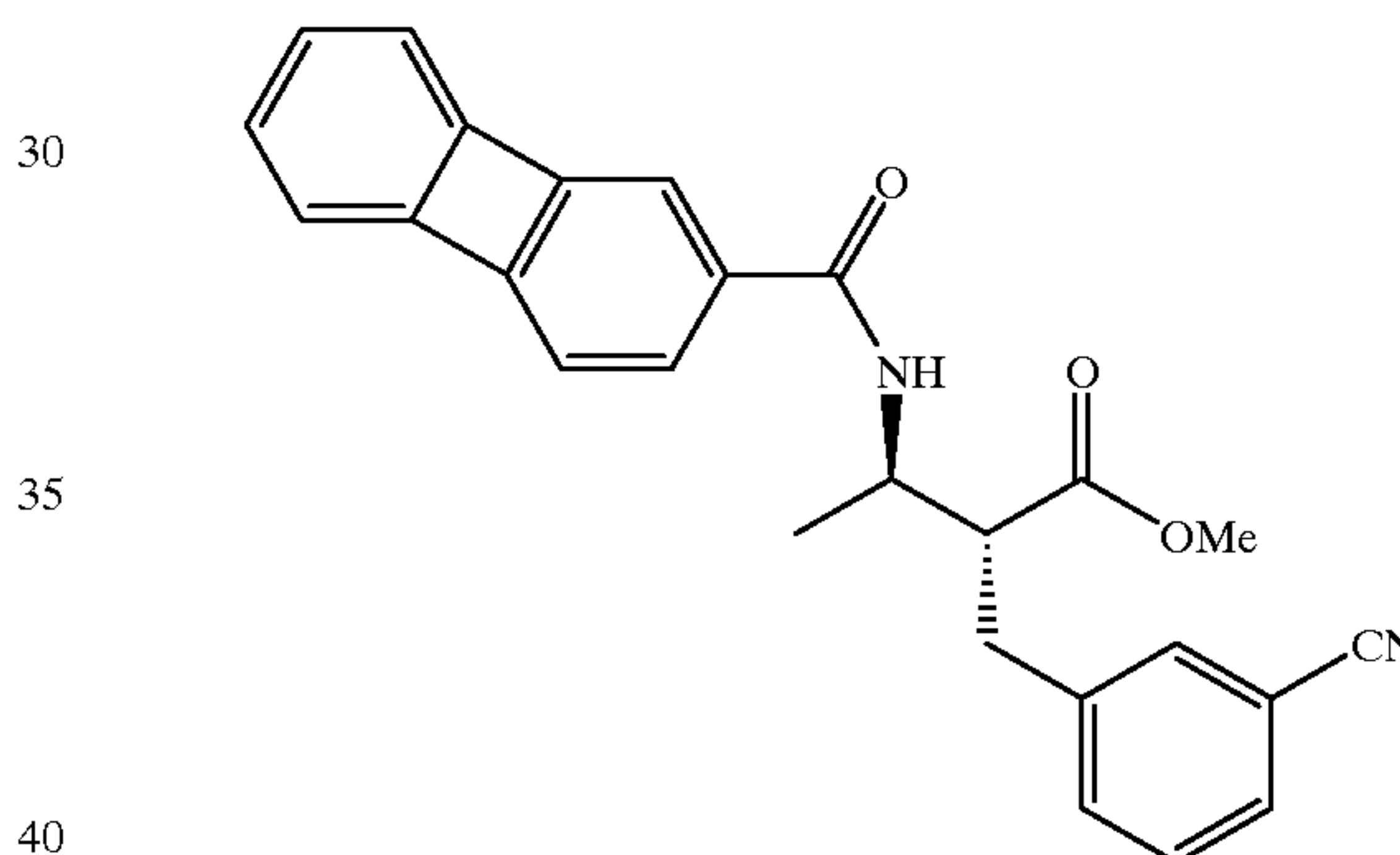
Compound 206
