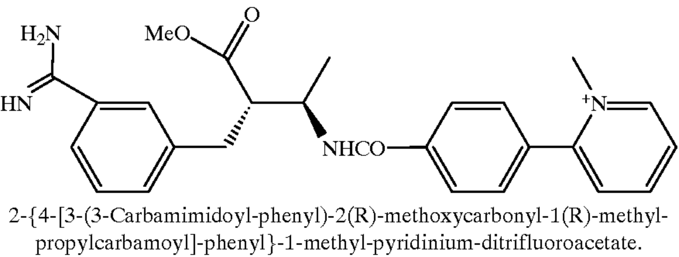
Compound 338
