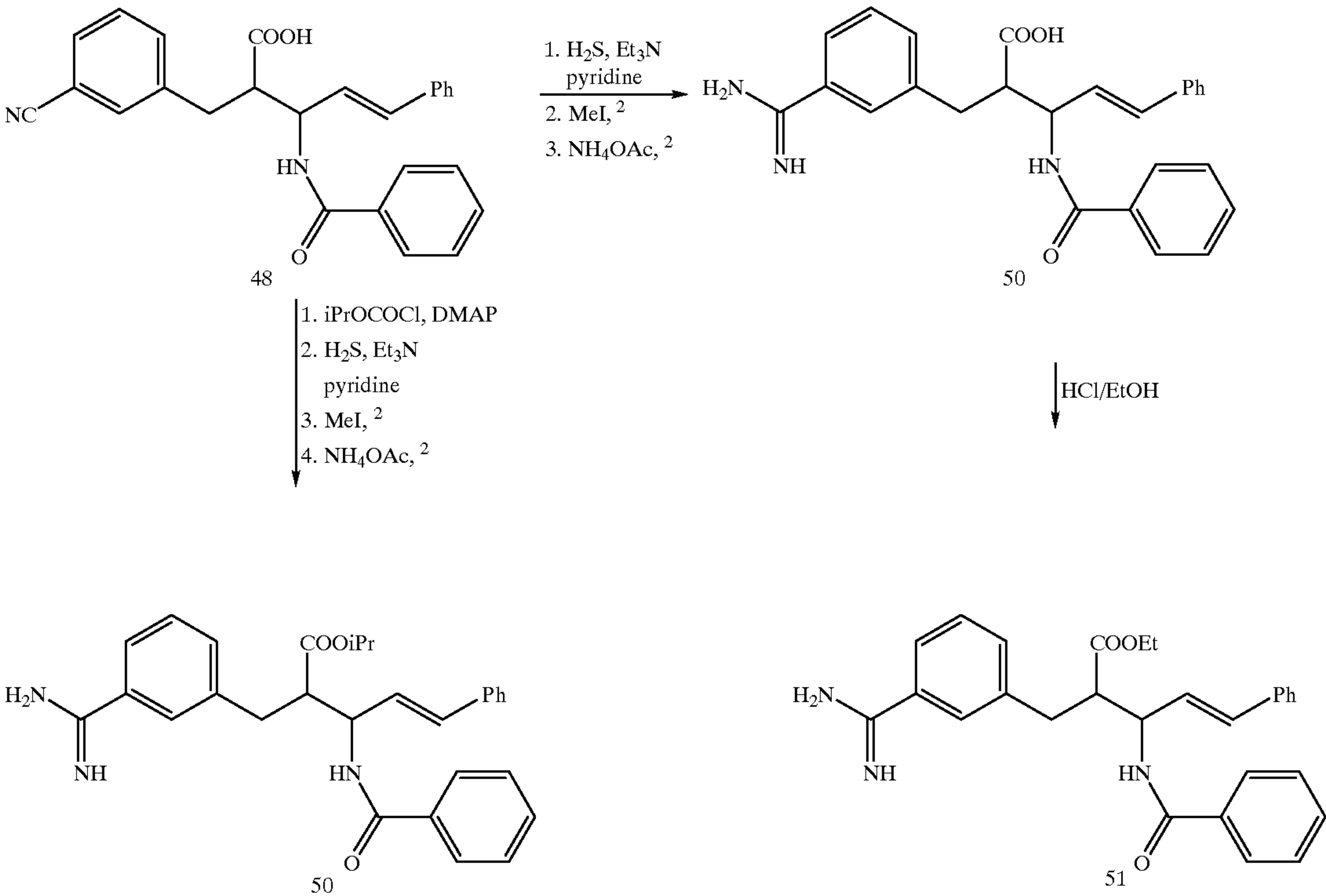
SCHEME D
