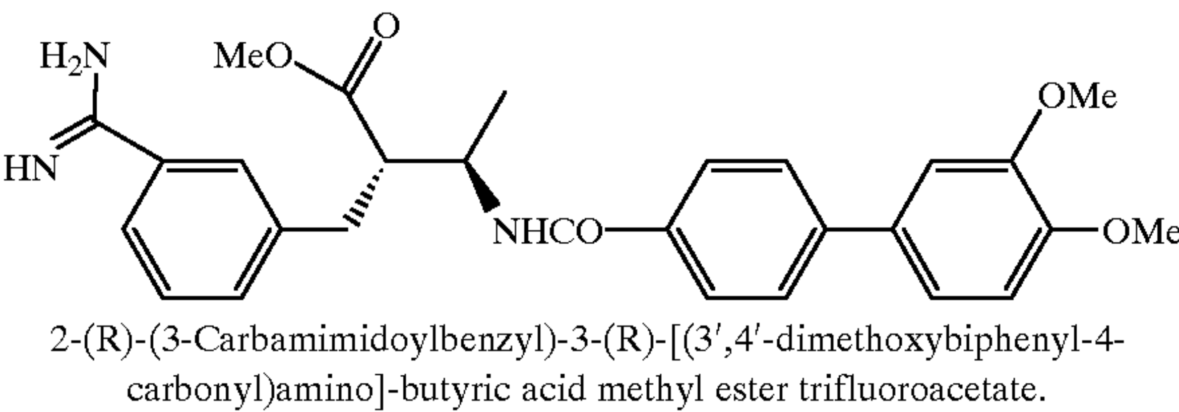
Compound 339
