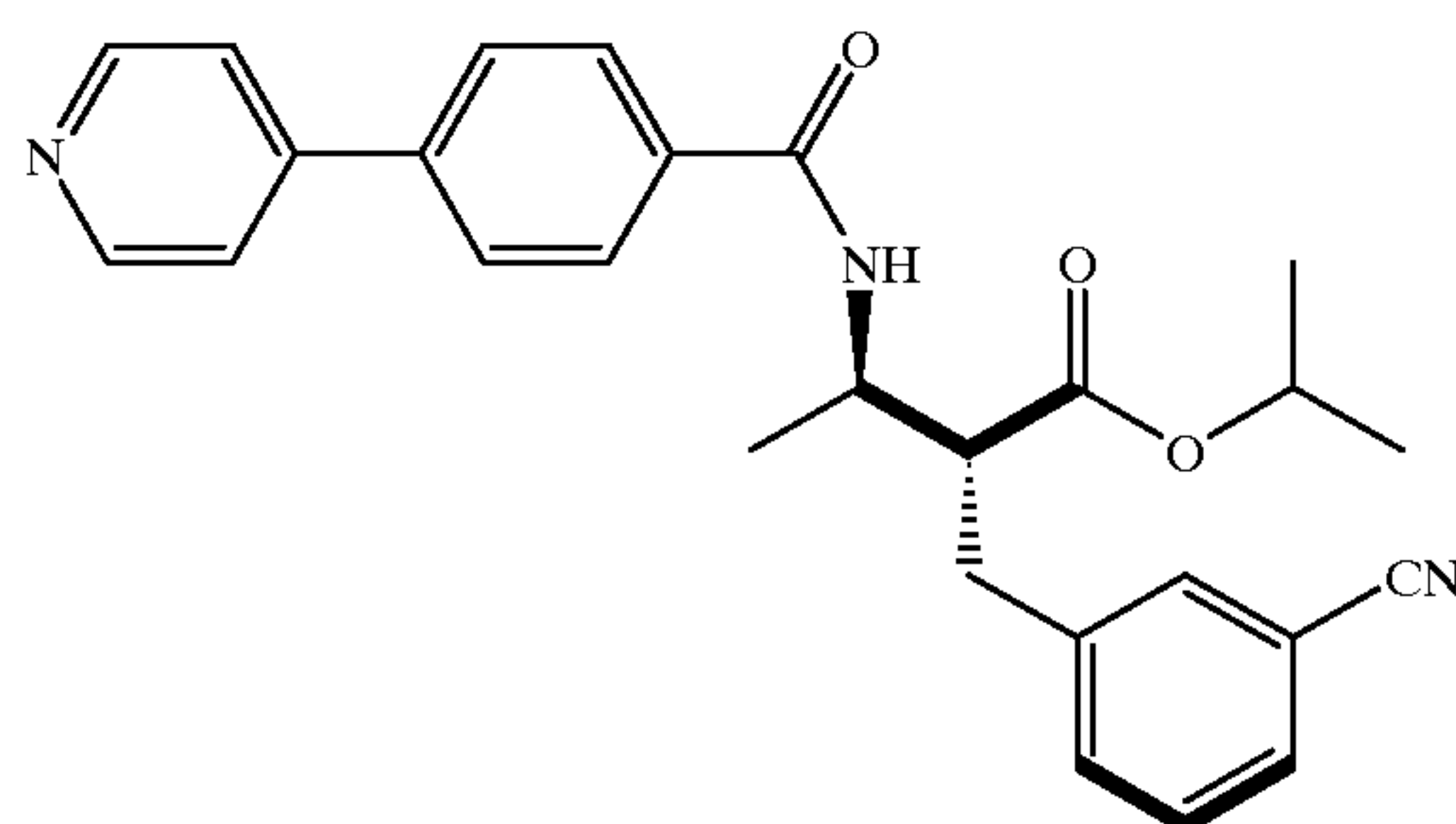
Compound 220
