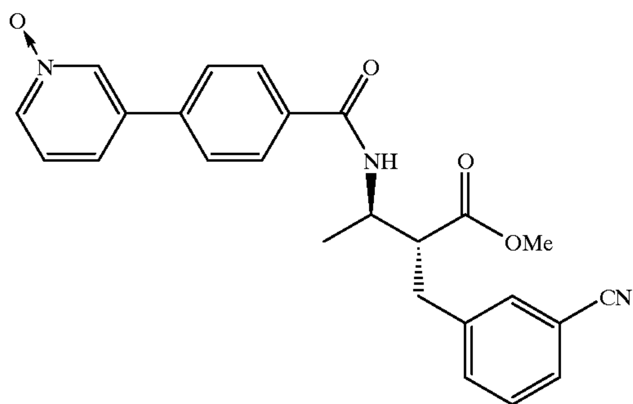
Compound 208
