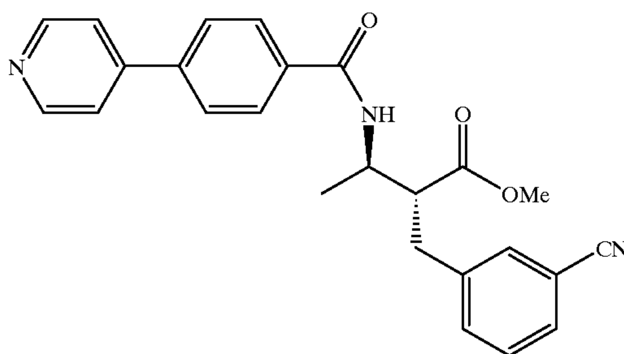
Compound 204
