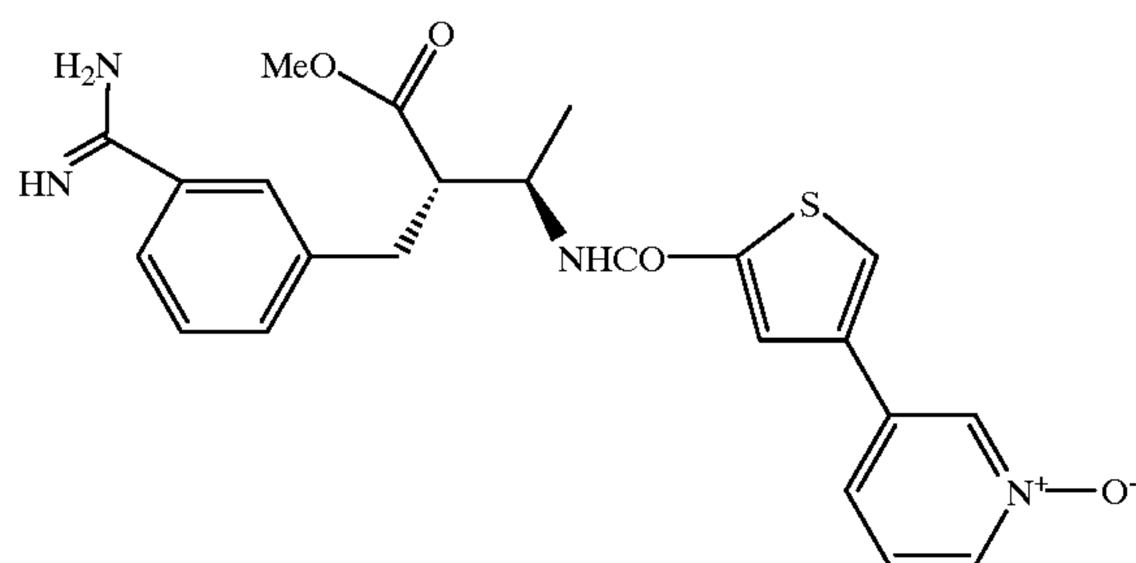
2-(R)-(3-Carbamimidoylbenzyl)-3-(R)-{oxypyridin-3yl}-thiophene-2-carbonyl}-amino}butyric acid methyl ester trifluoroacetate.
