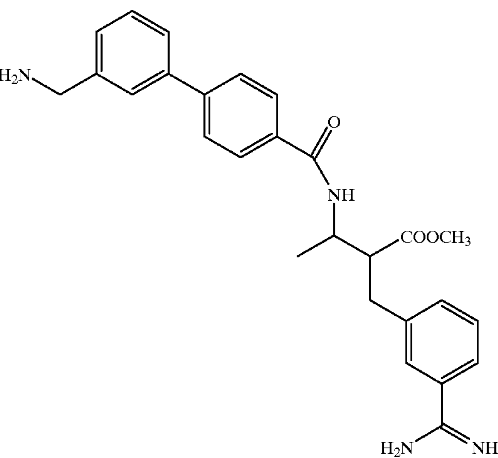
Compound 188
