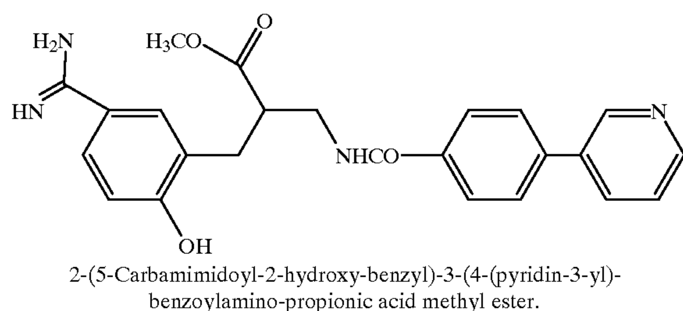
Compound 345
