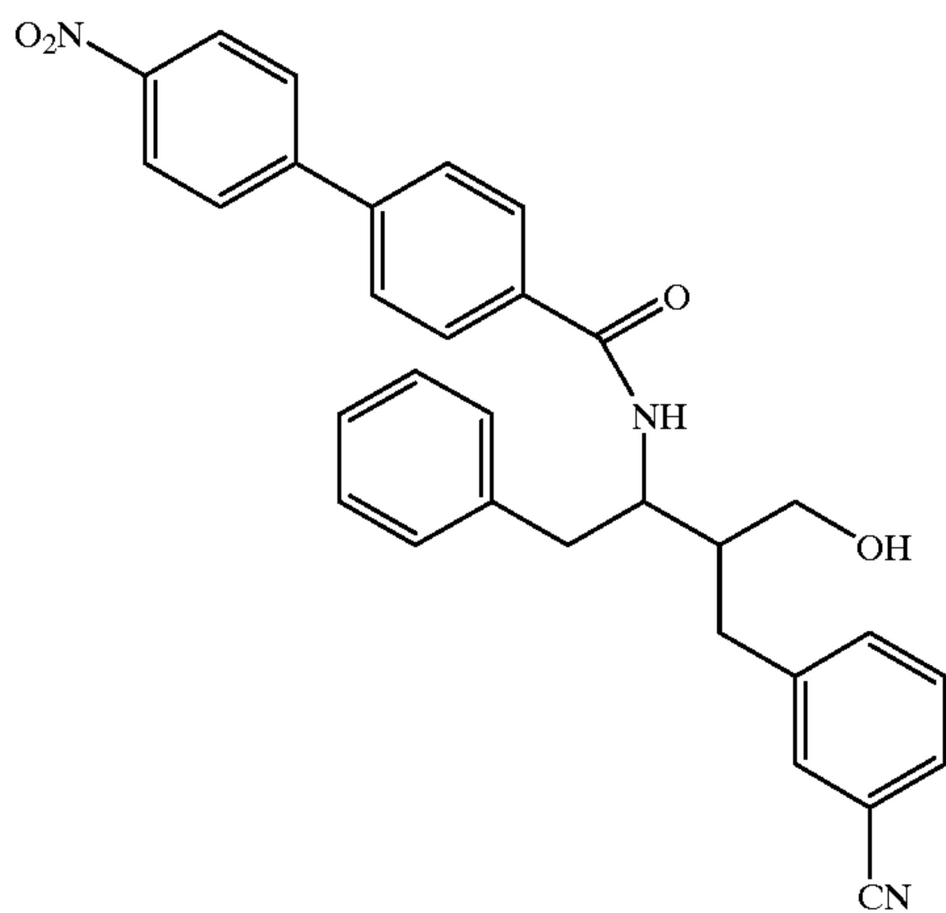
Compound 140
