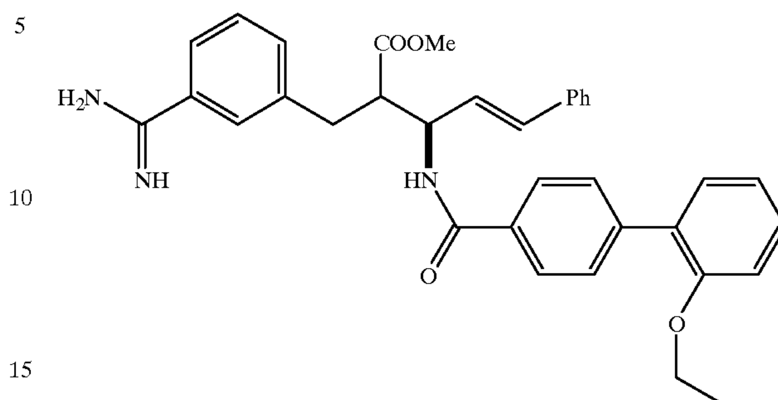
Compound 30
