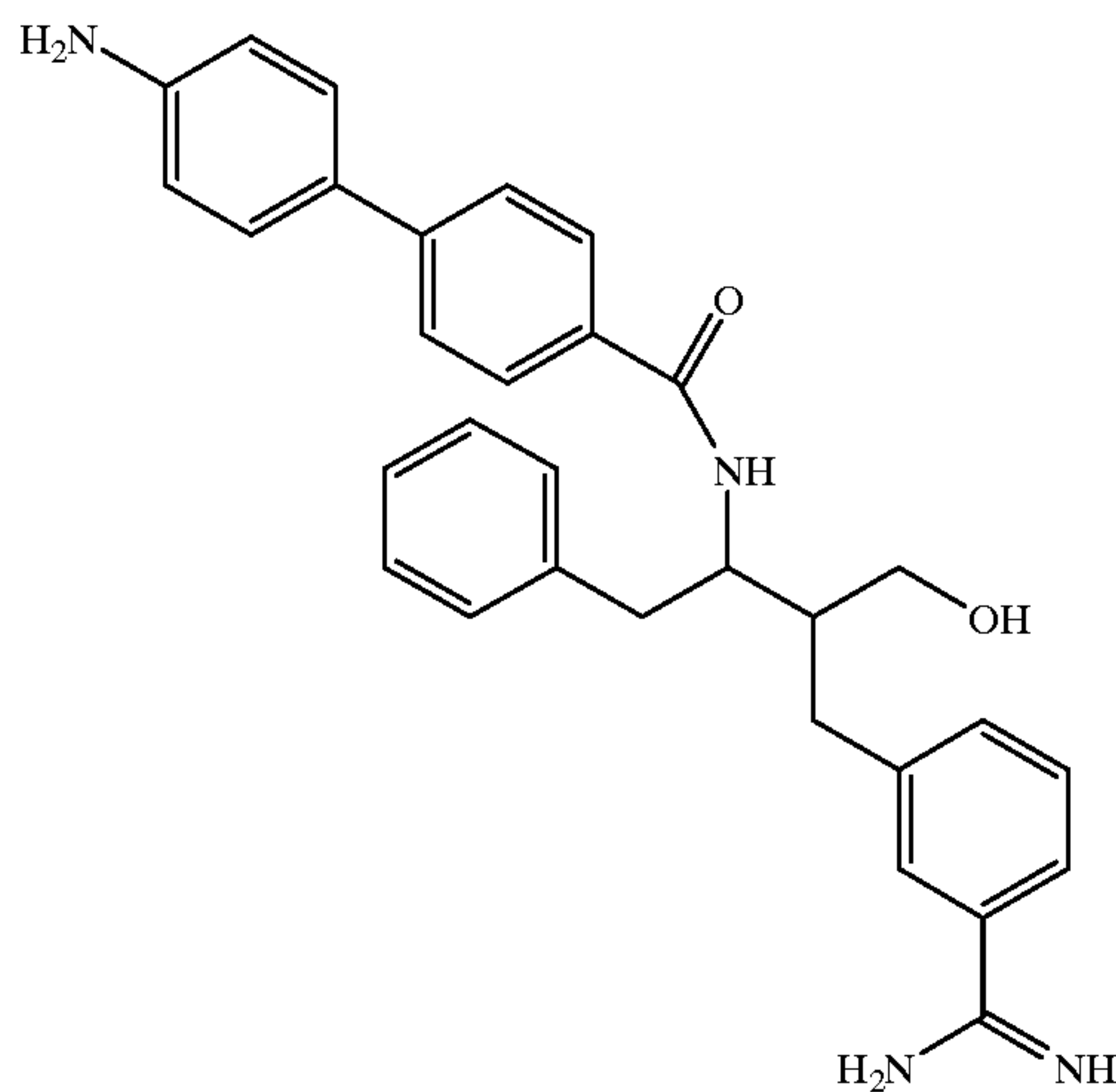
Compound 178
