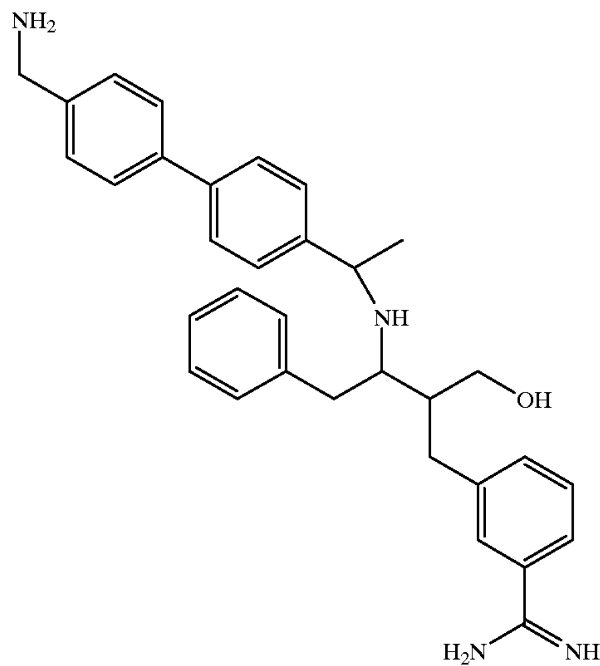
Compound 174
