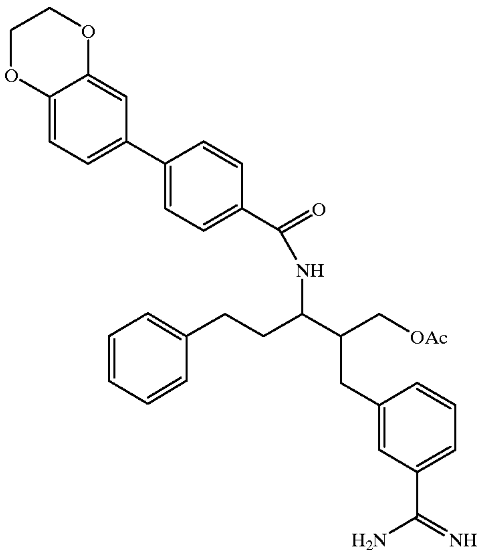
Compound 161
