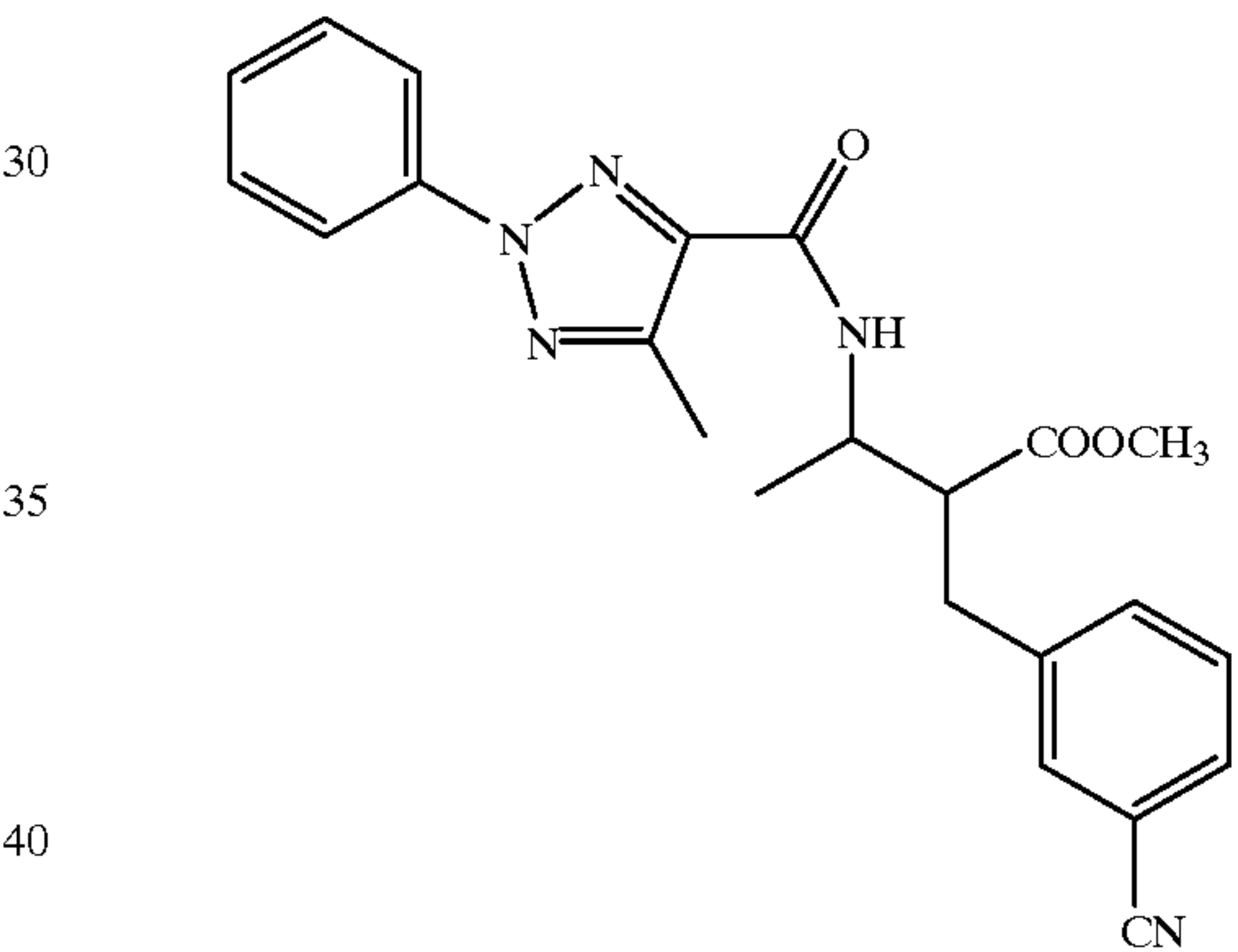
Compound 257
