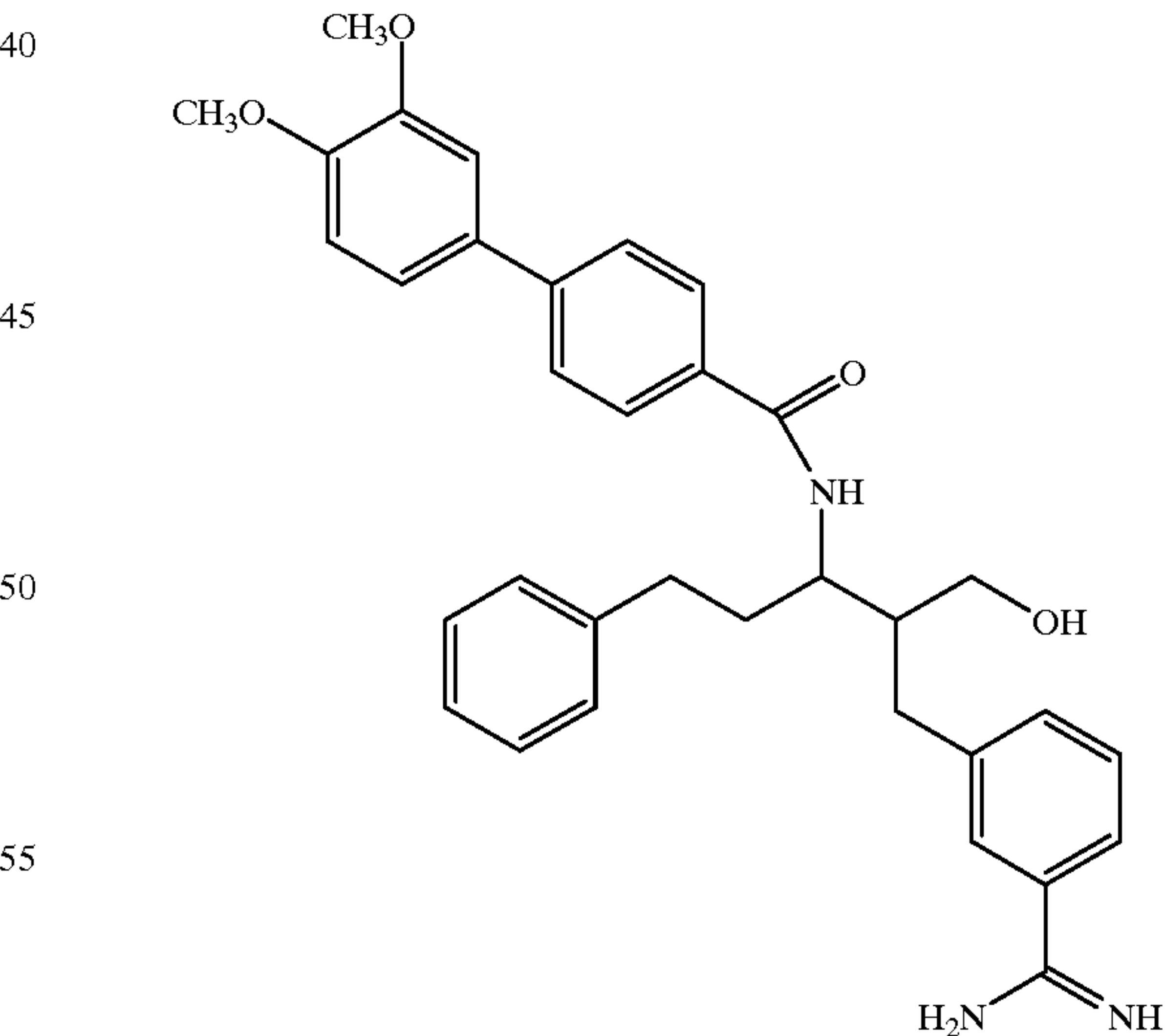
Compound 168
