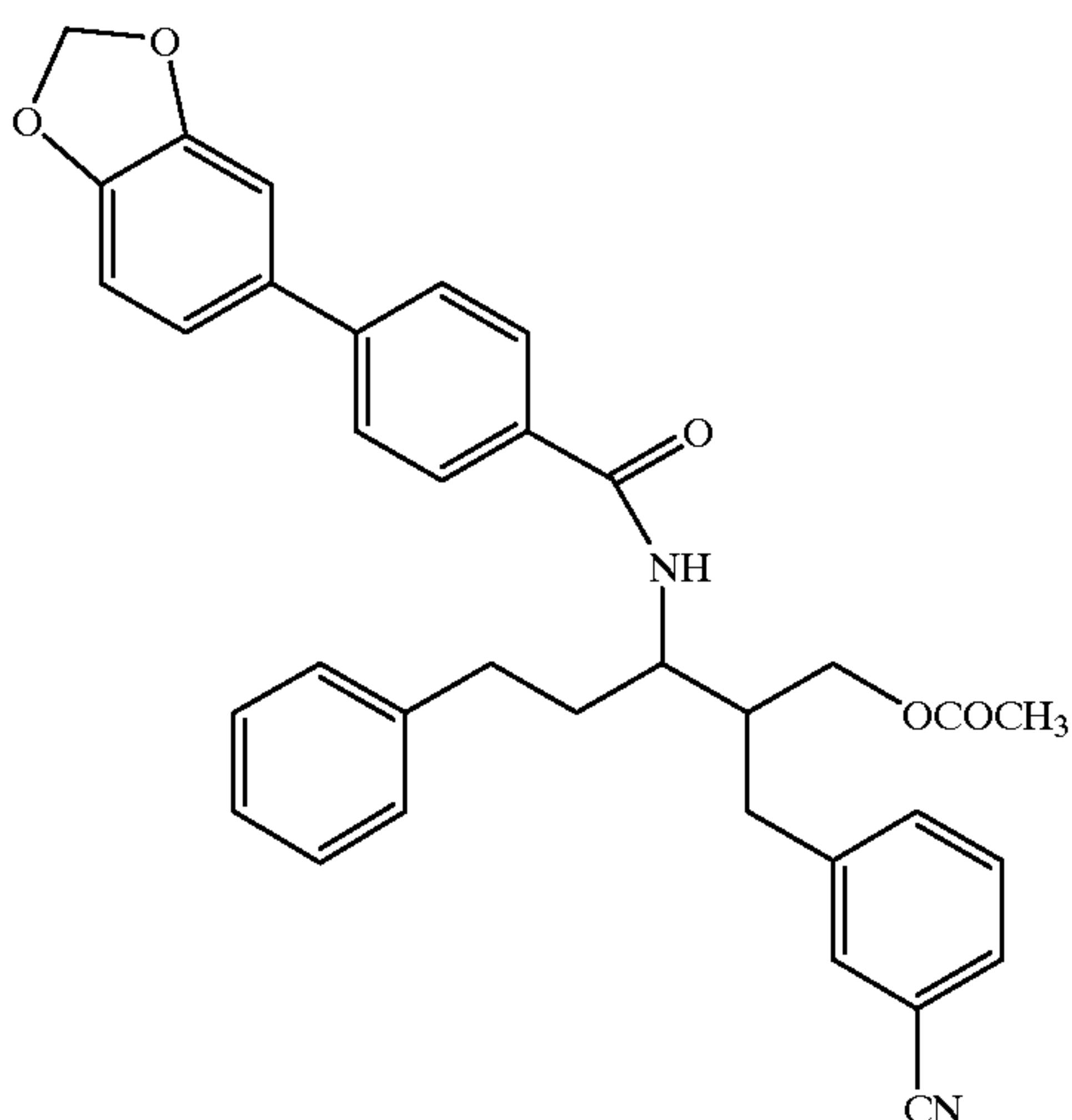
Compound 152
