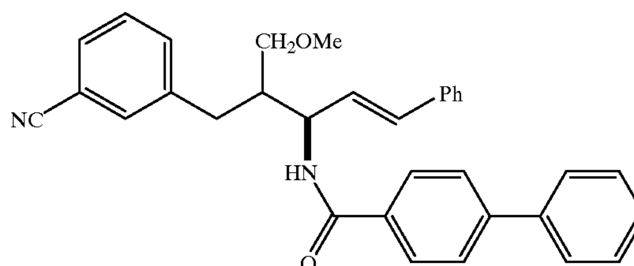
Compound 43
