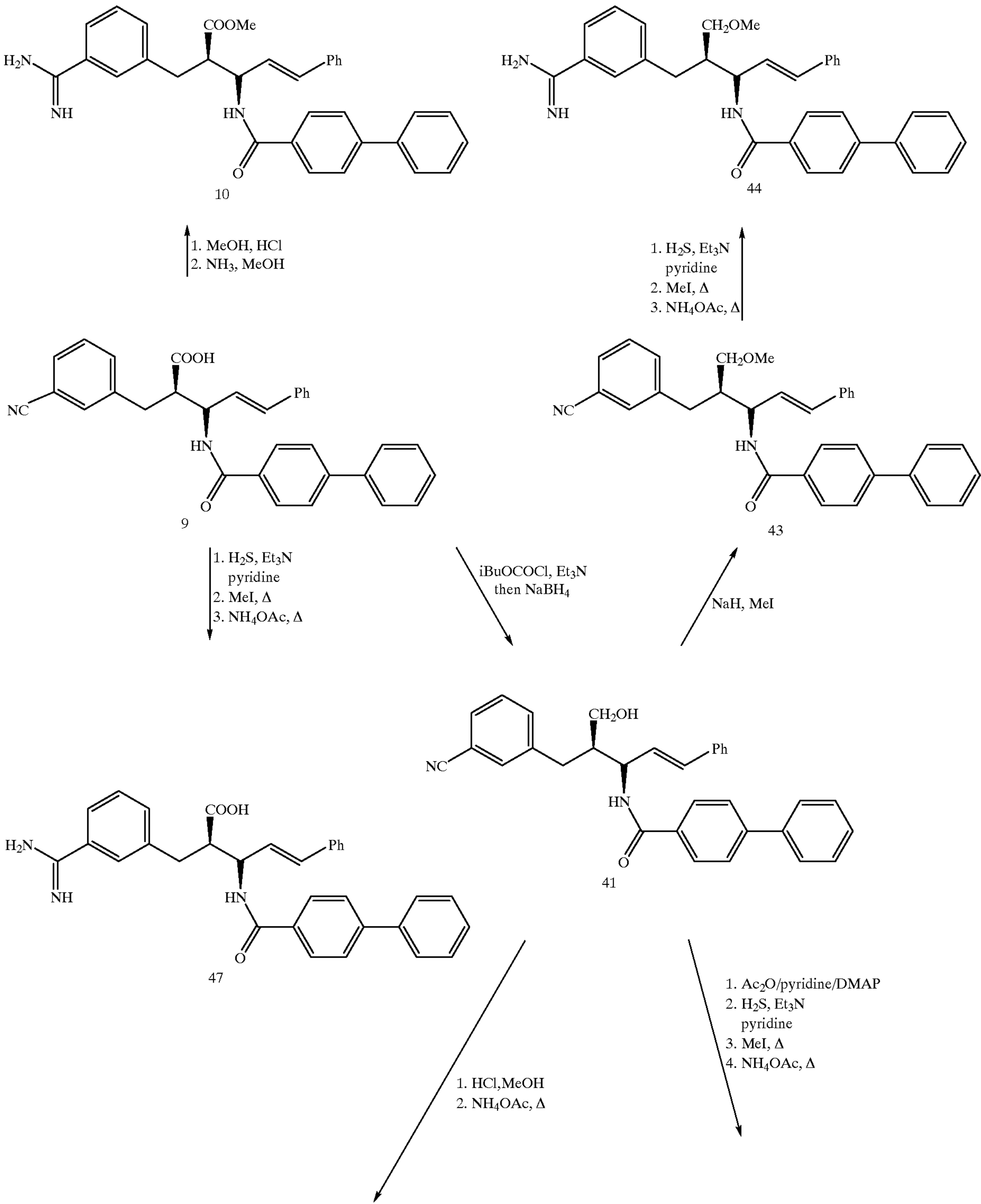
SCHEME C
