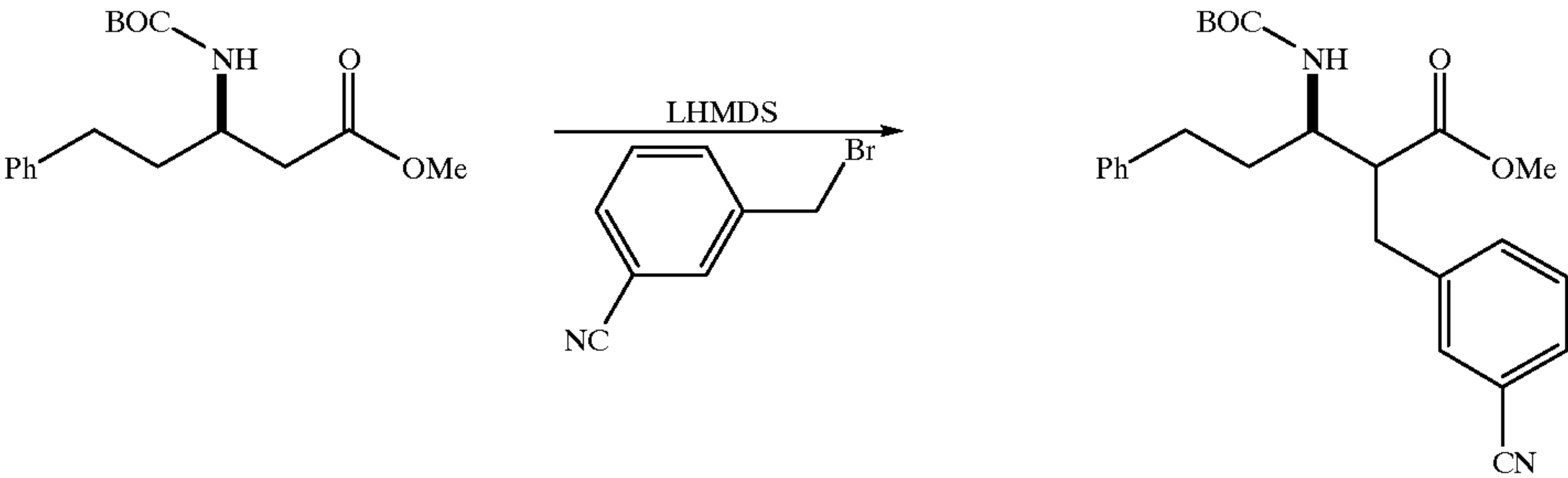
SCHEME F
