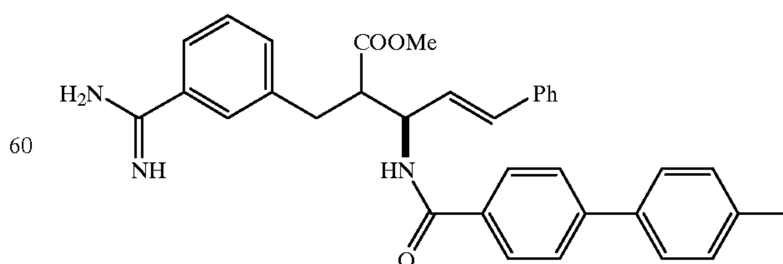
Compound 29
