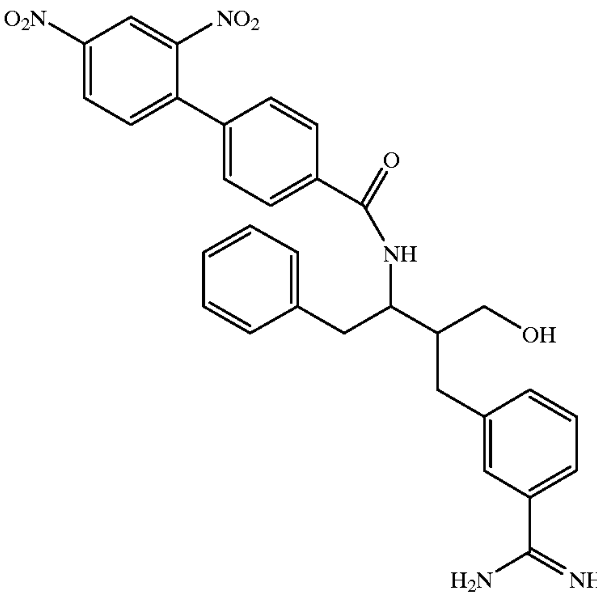
Compound 176
