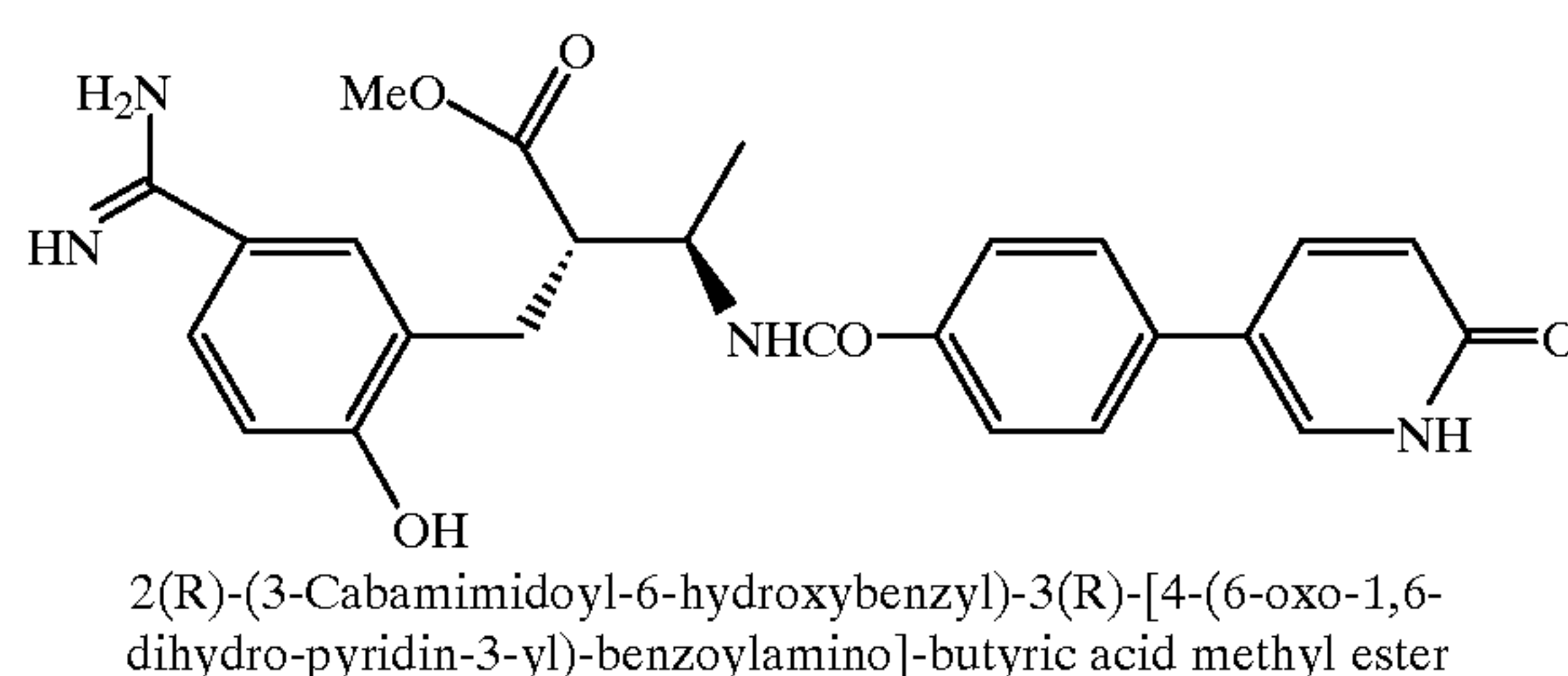
Compound 346
