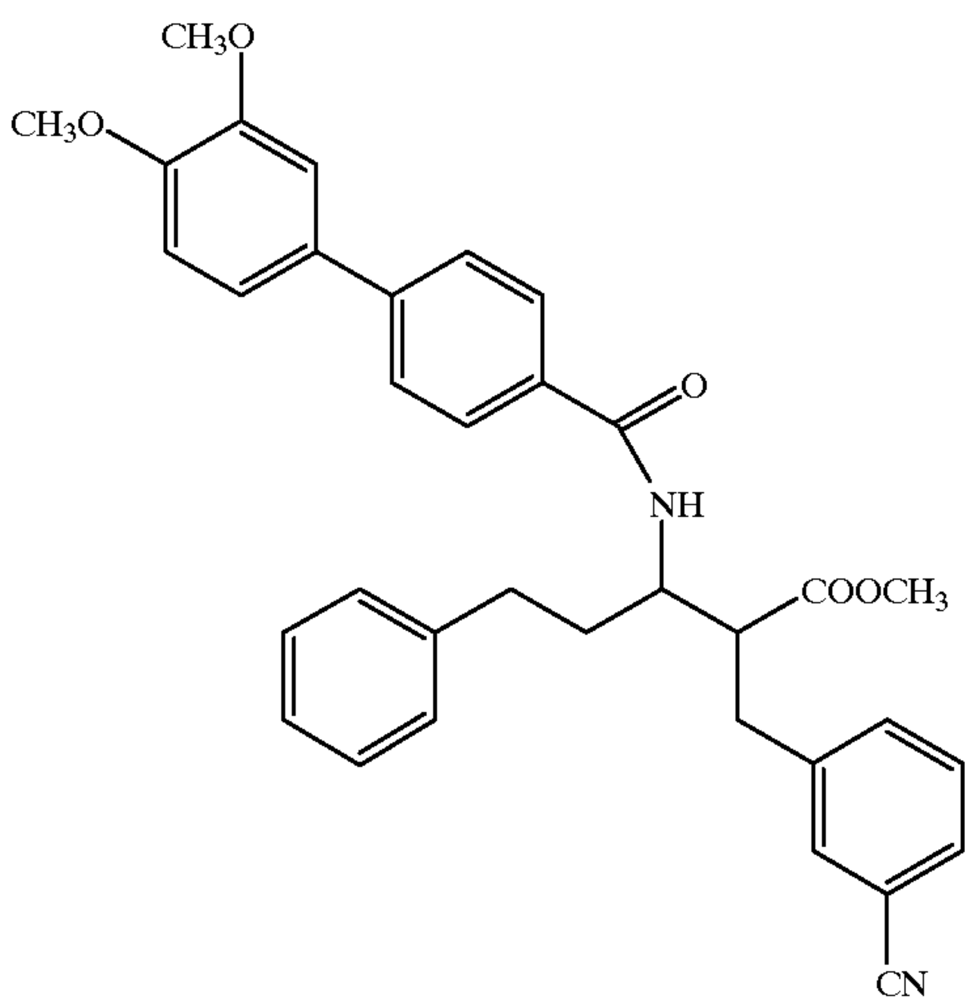
Compound 113
