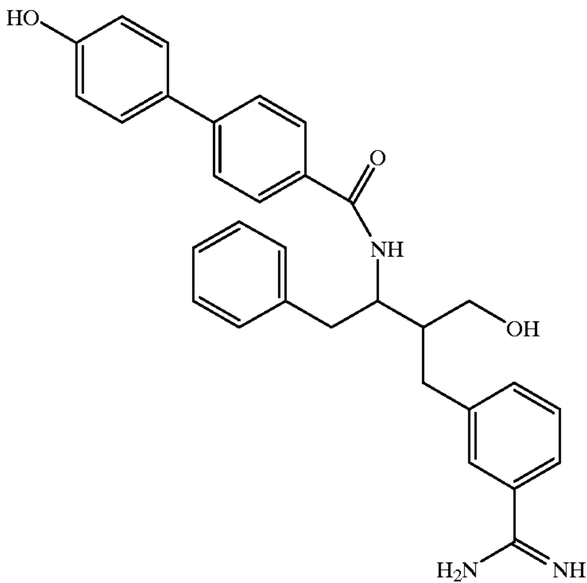
Compound 175
