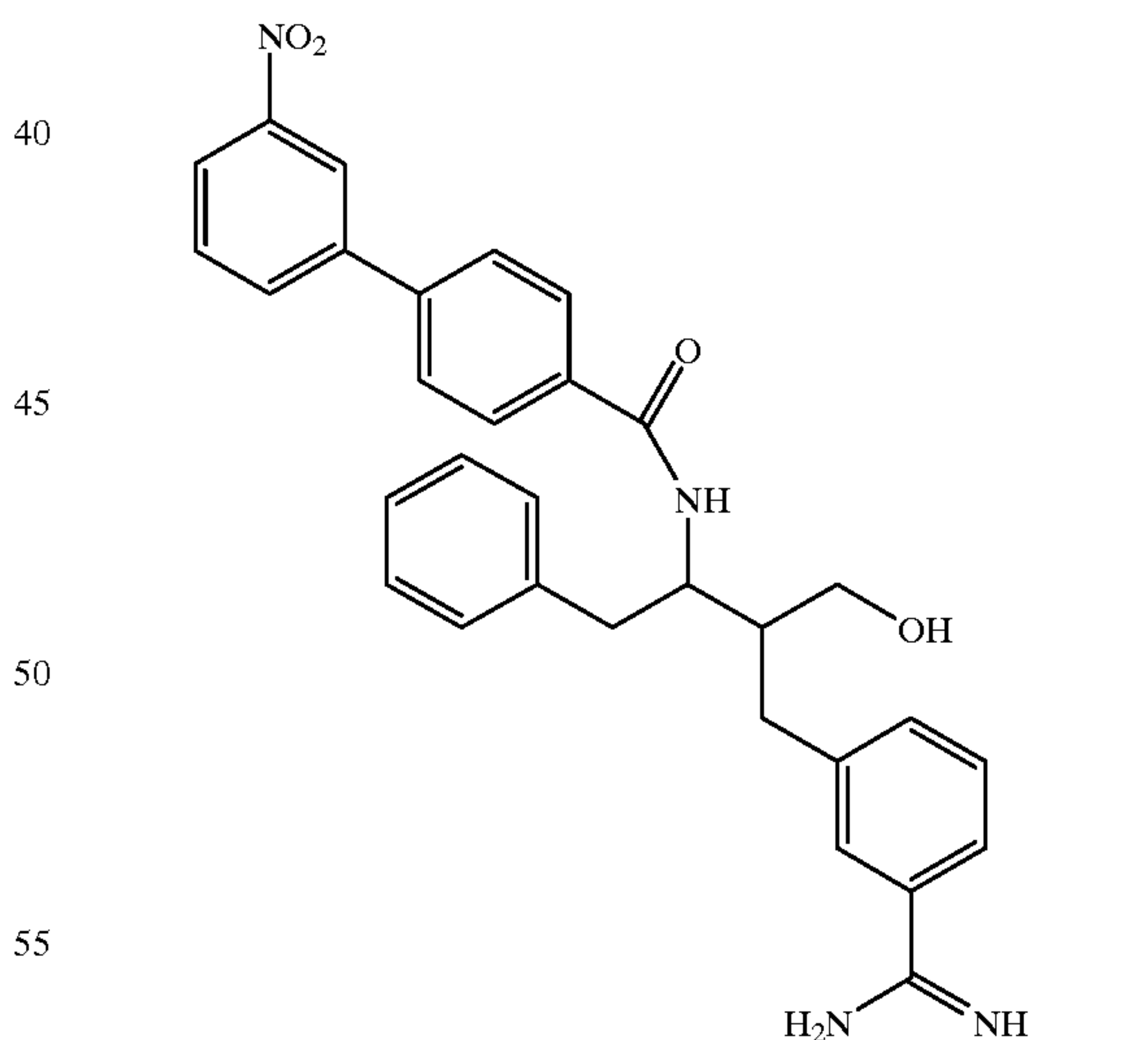
Compound 180
