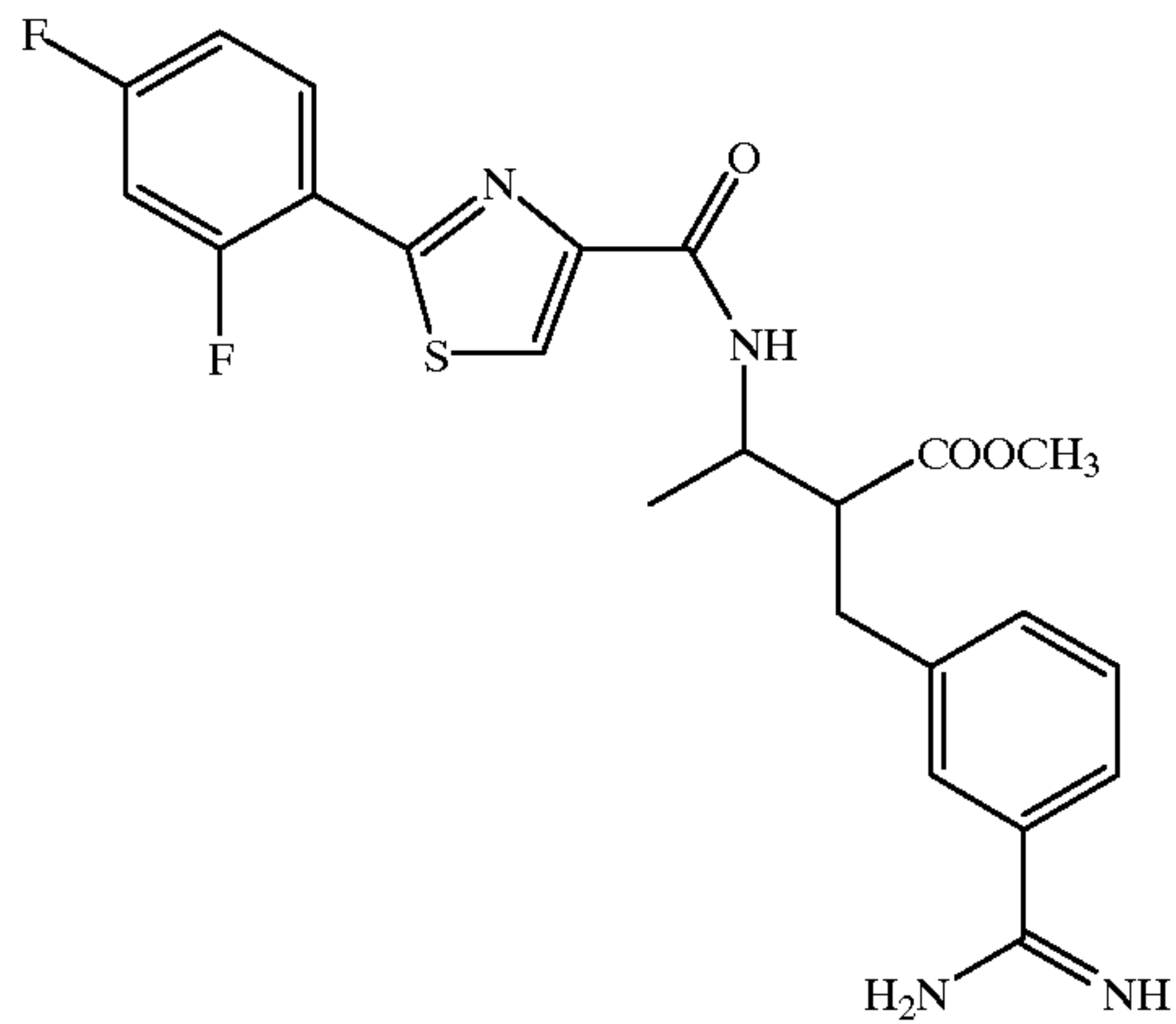
Compound 292
