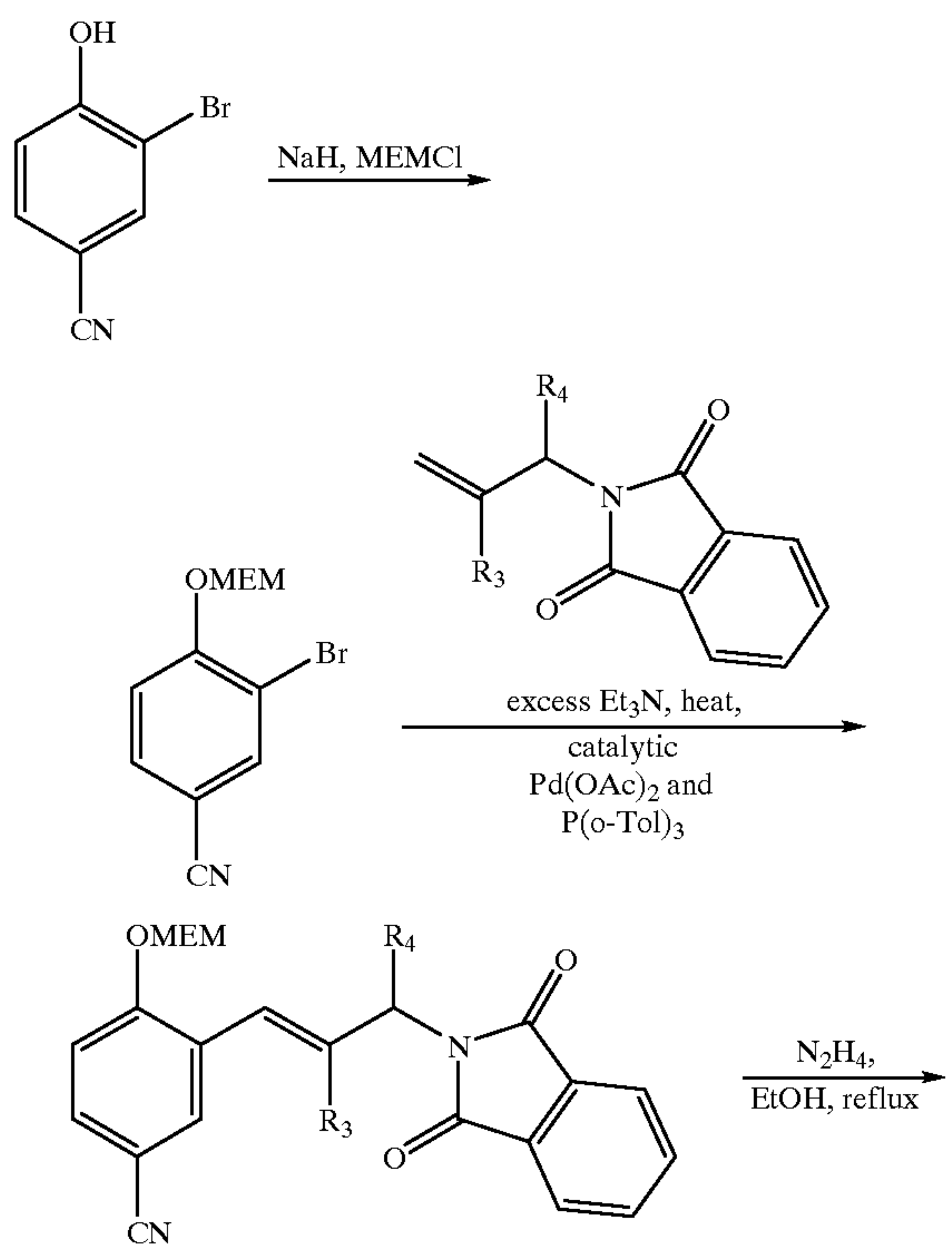
Scheme I
