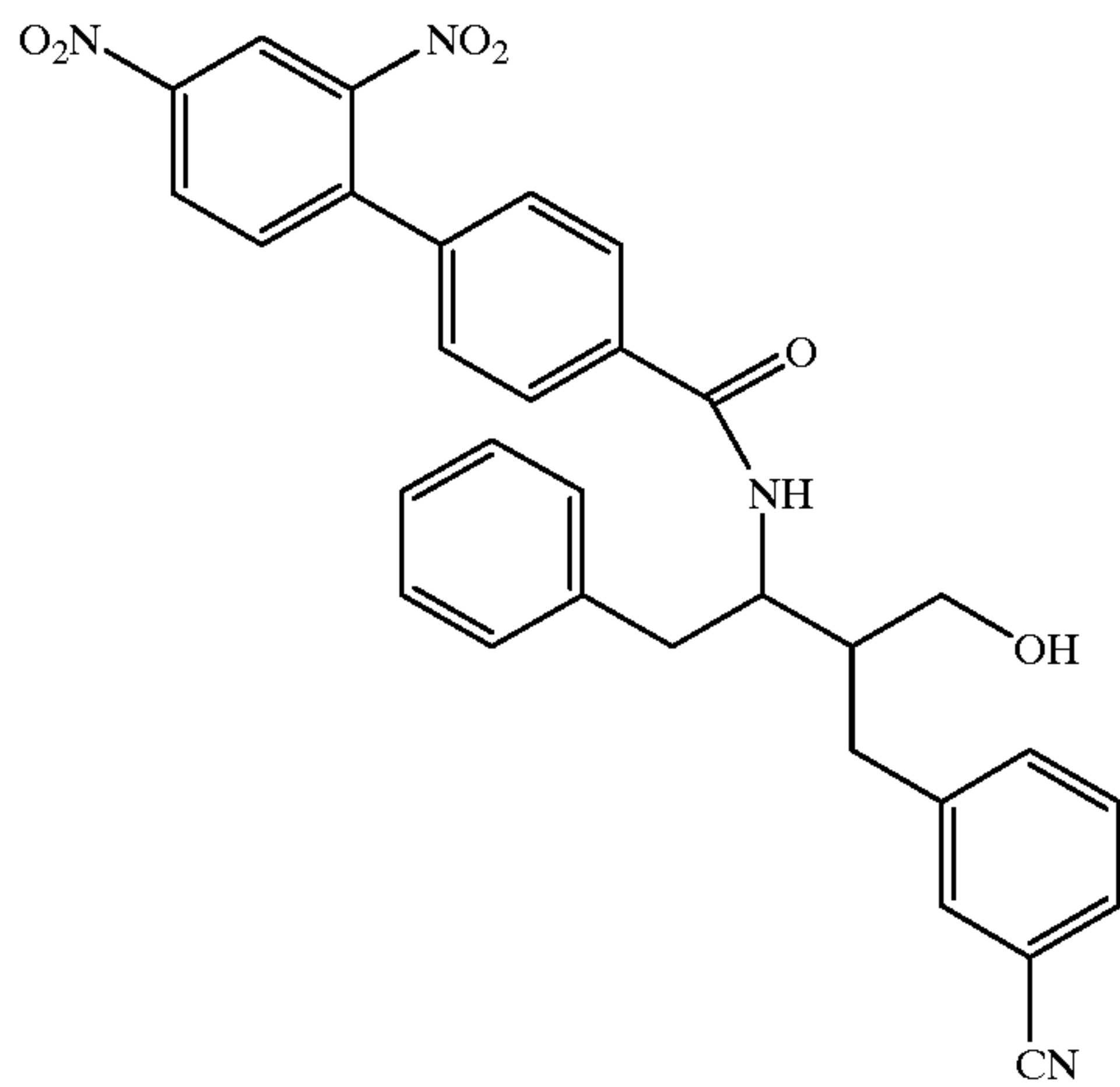
Compound 141
