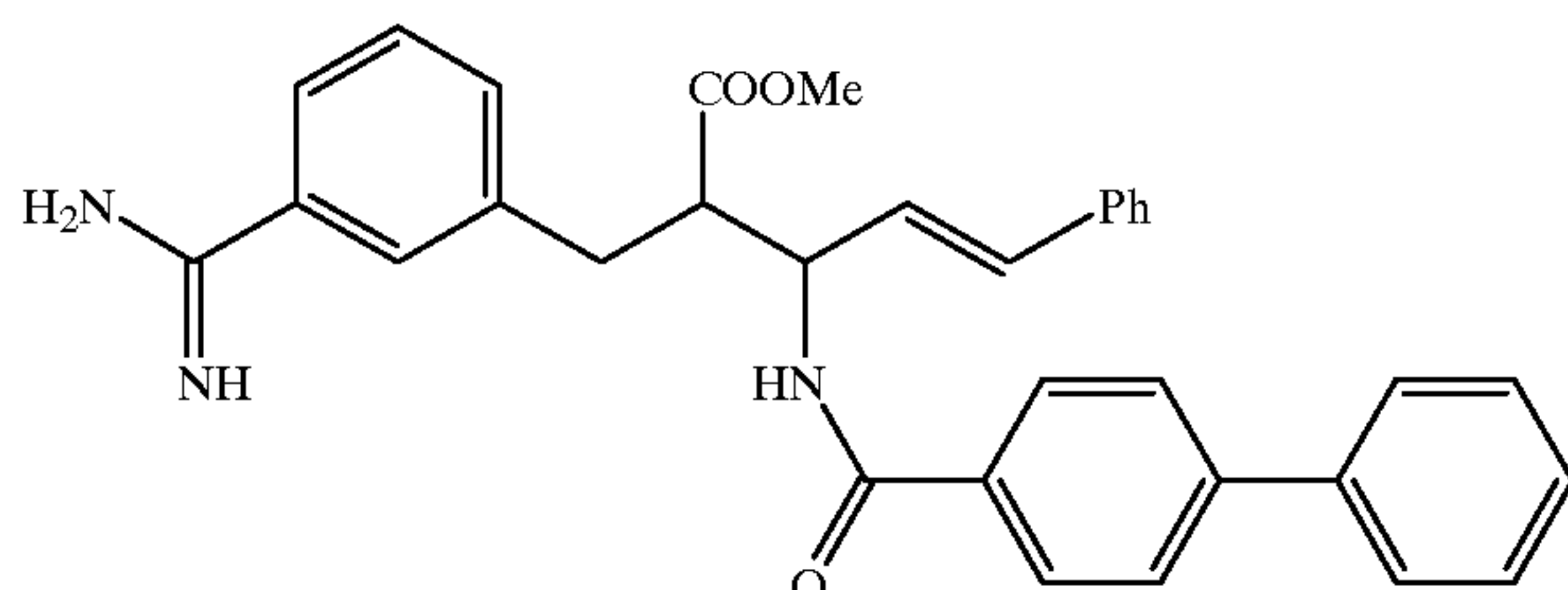
Compound 10
