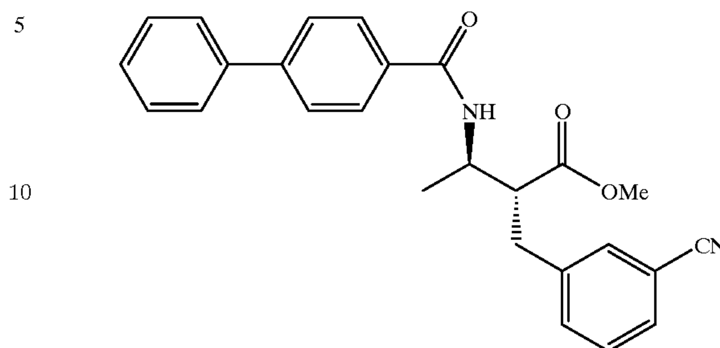
Compound 203
