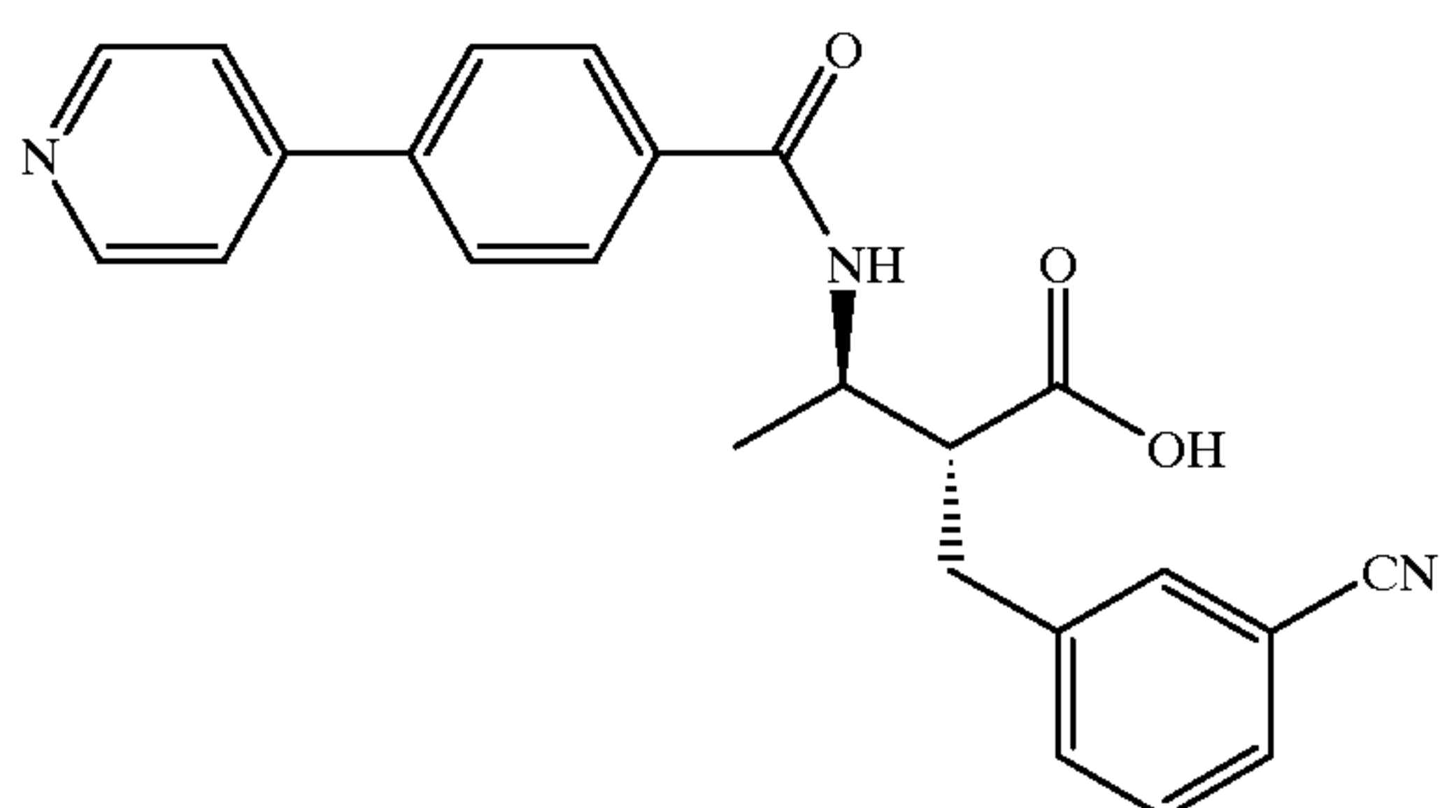
Compound 219
