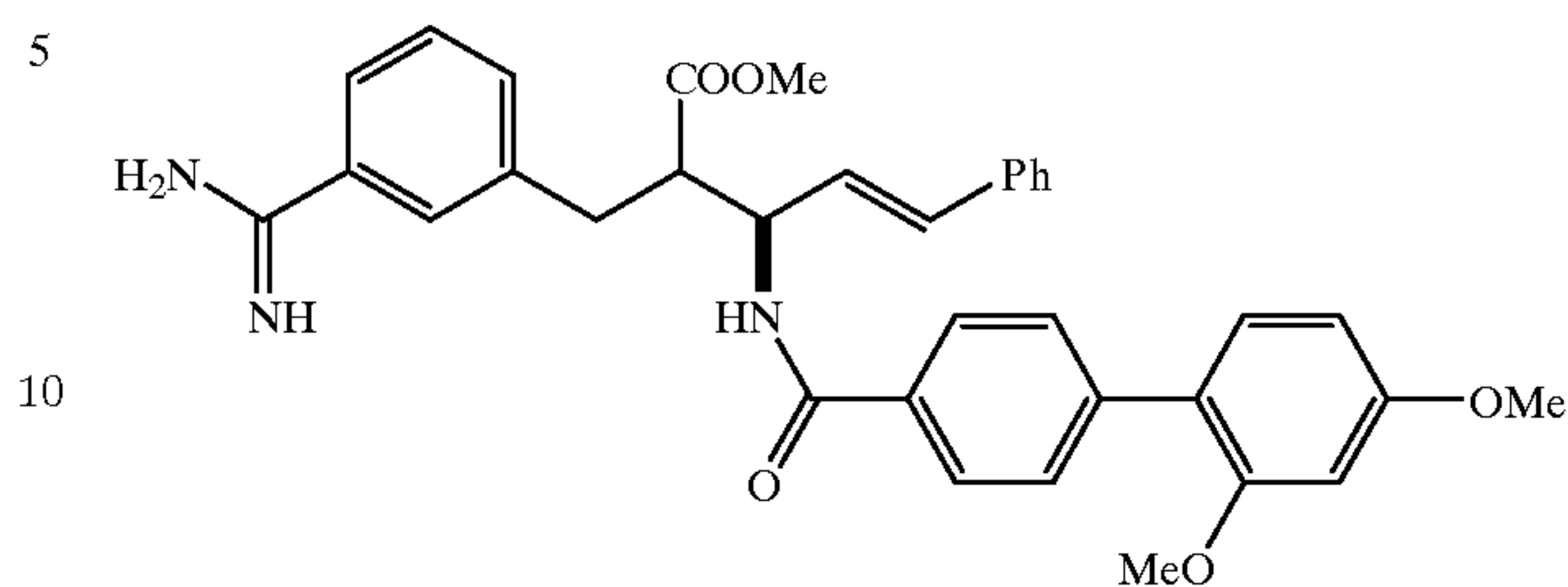
Compound 27
