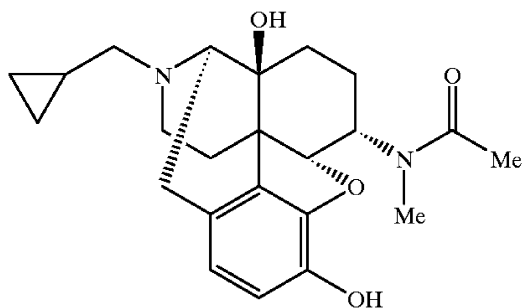
Compound 25
