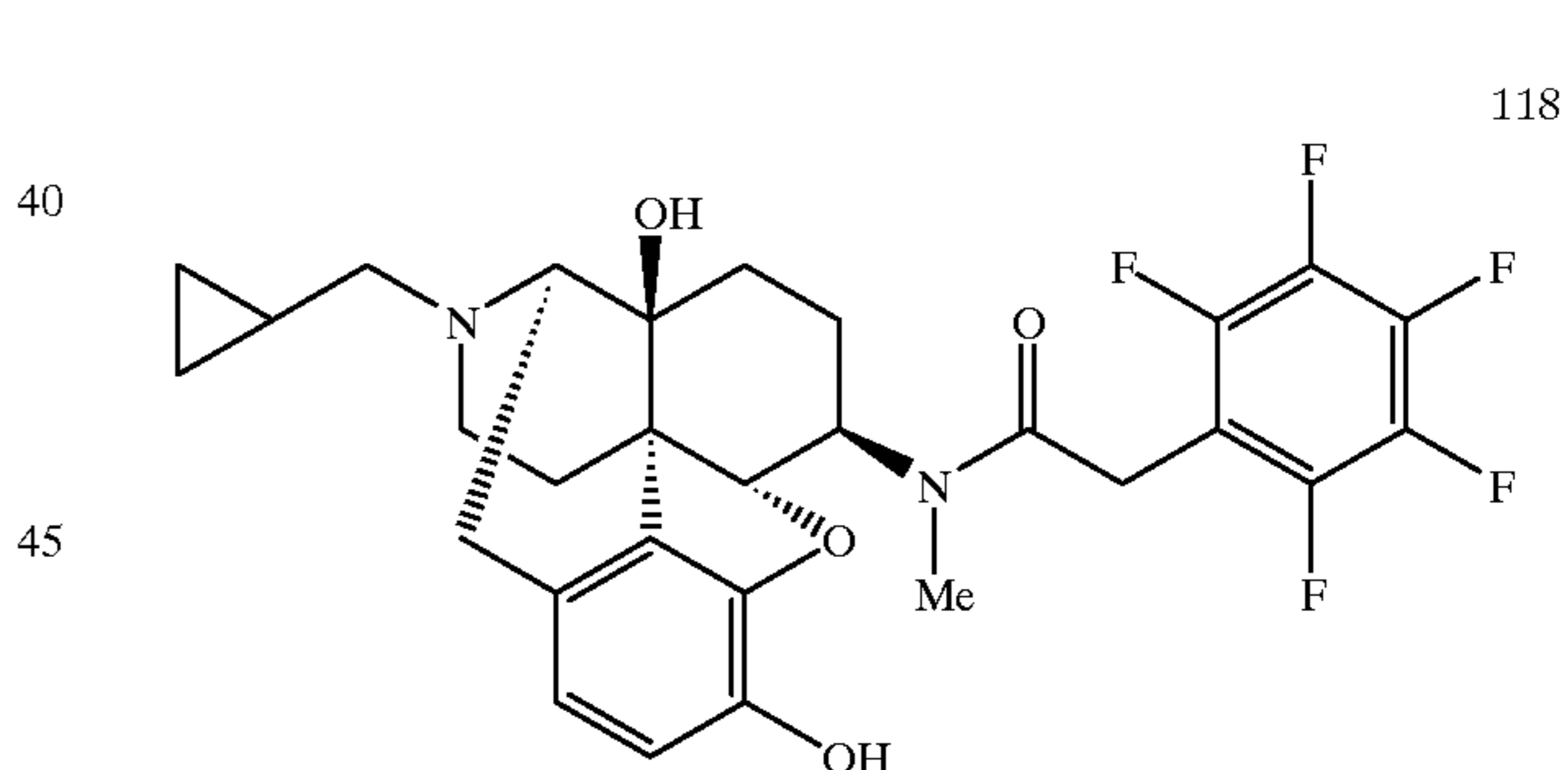
Compound 118
