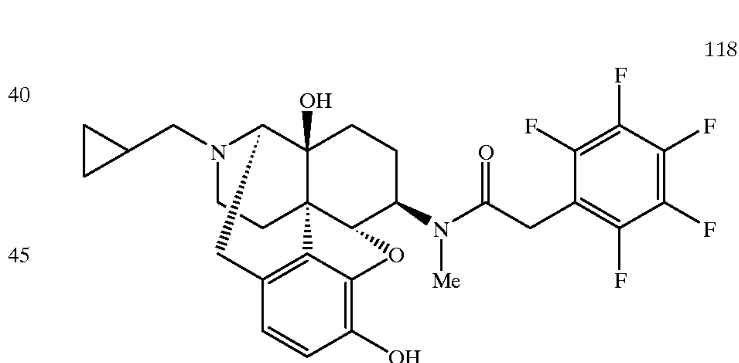
Compound 118
