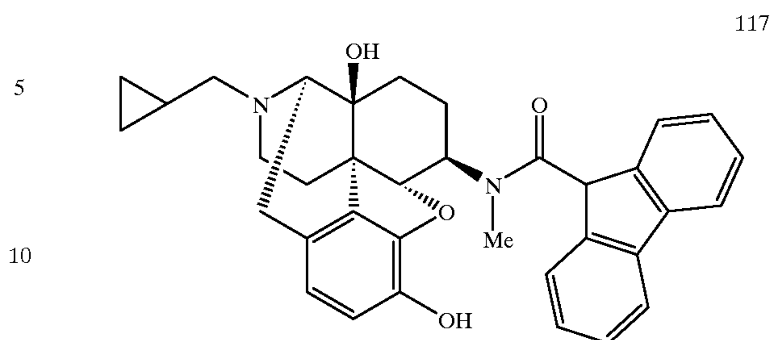
Compound 117
