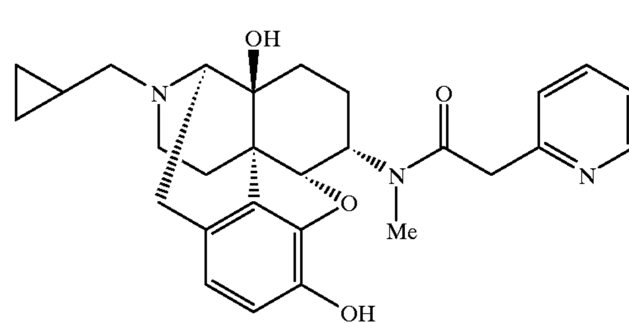
Compound 92
