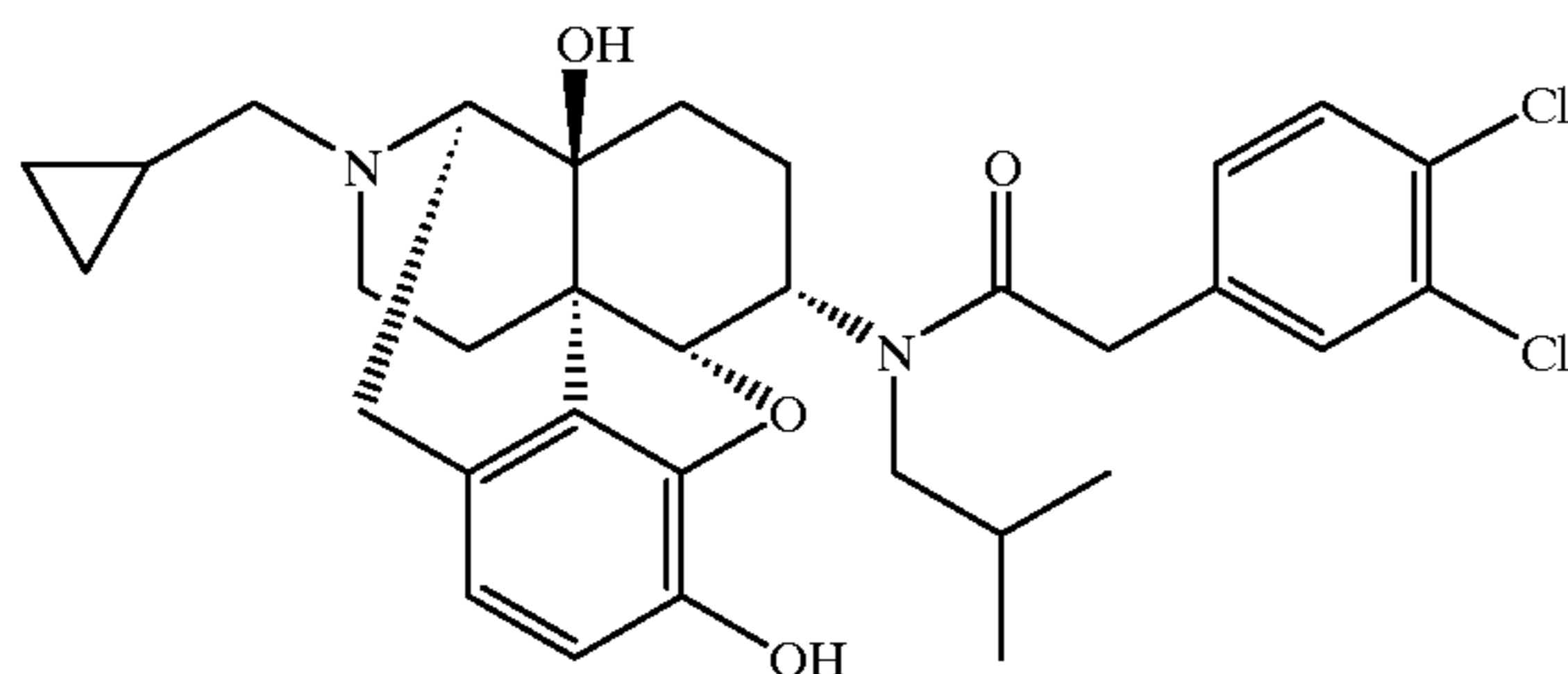
Compound 51
