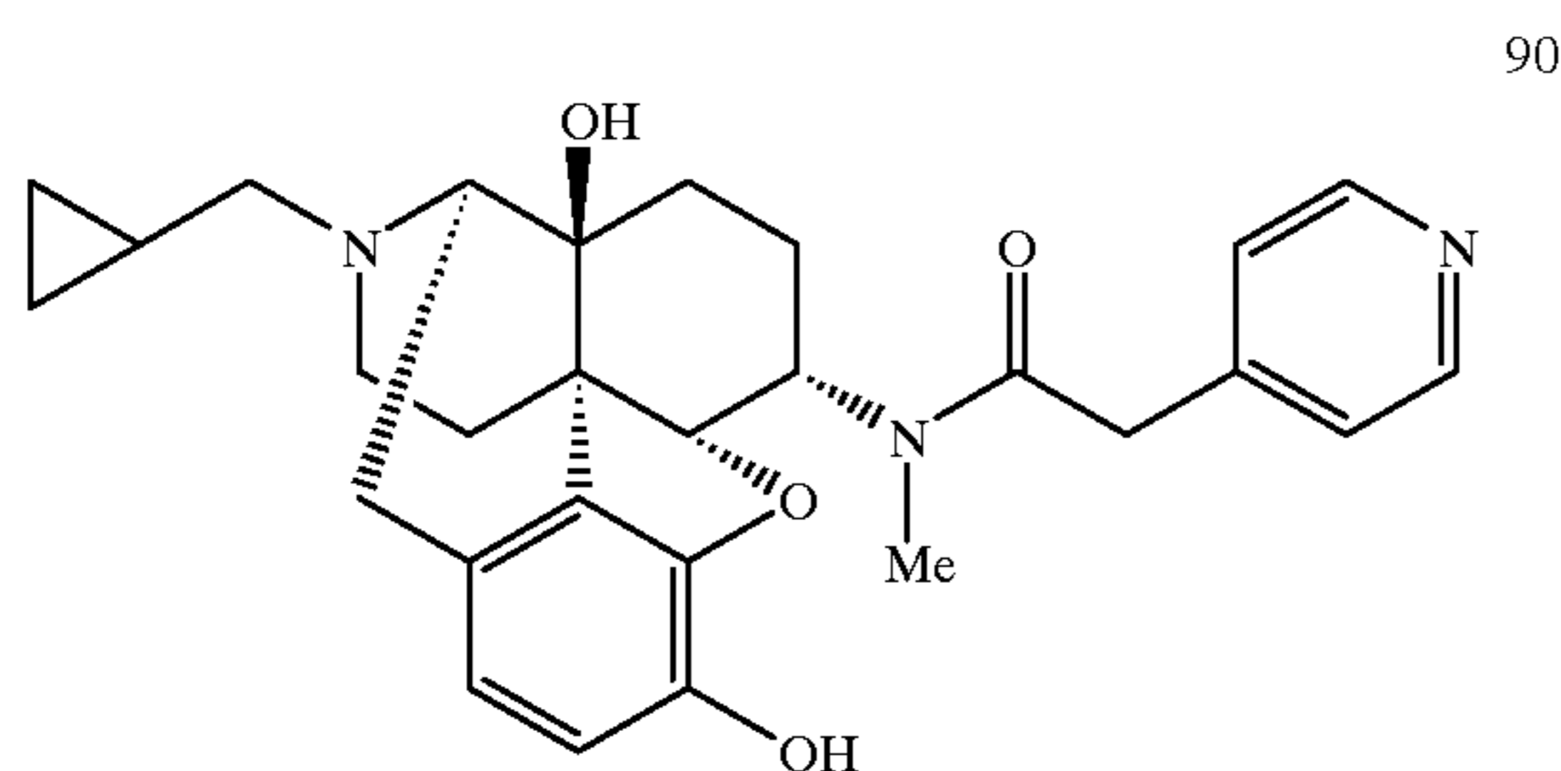
Compound 90
