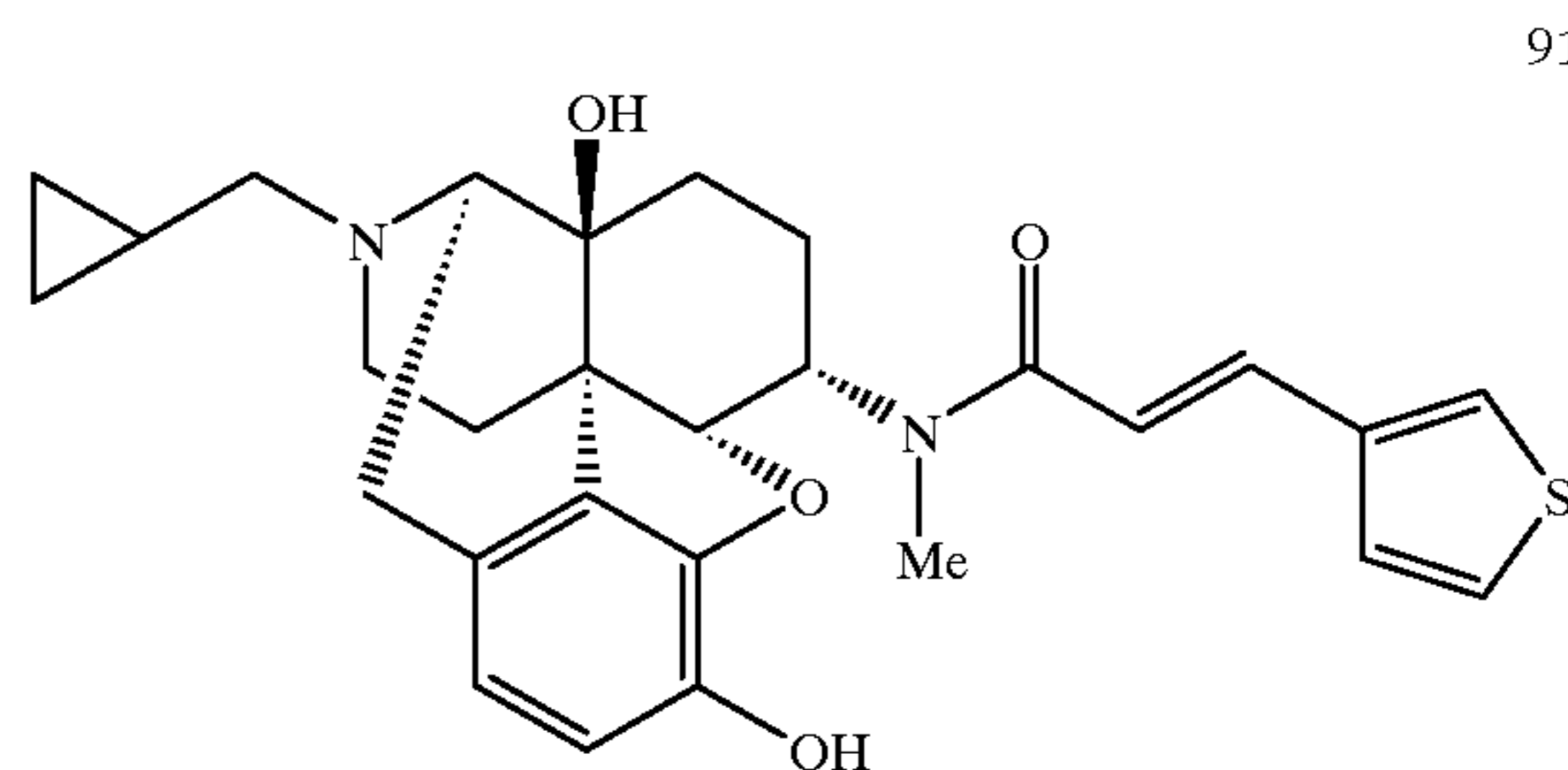
Compound 91
