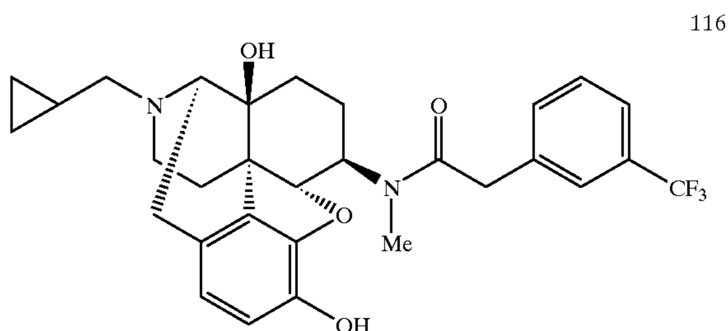
Compound 116
