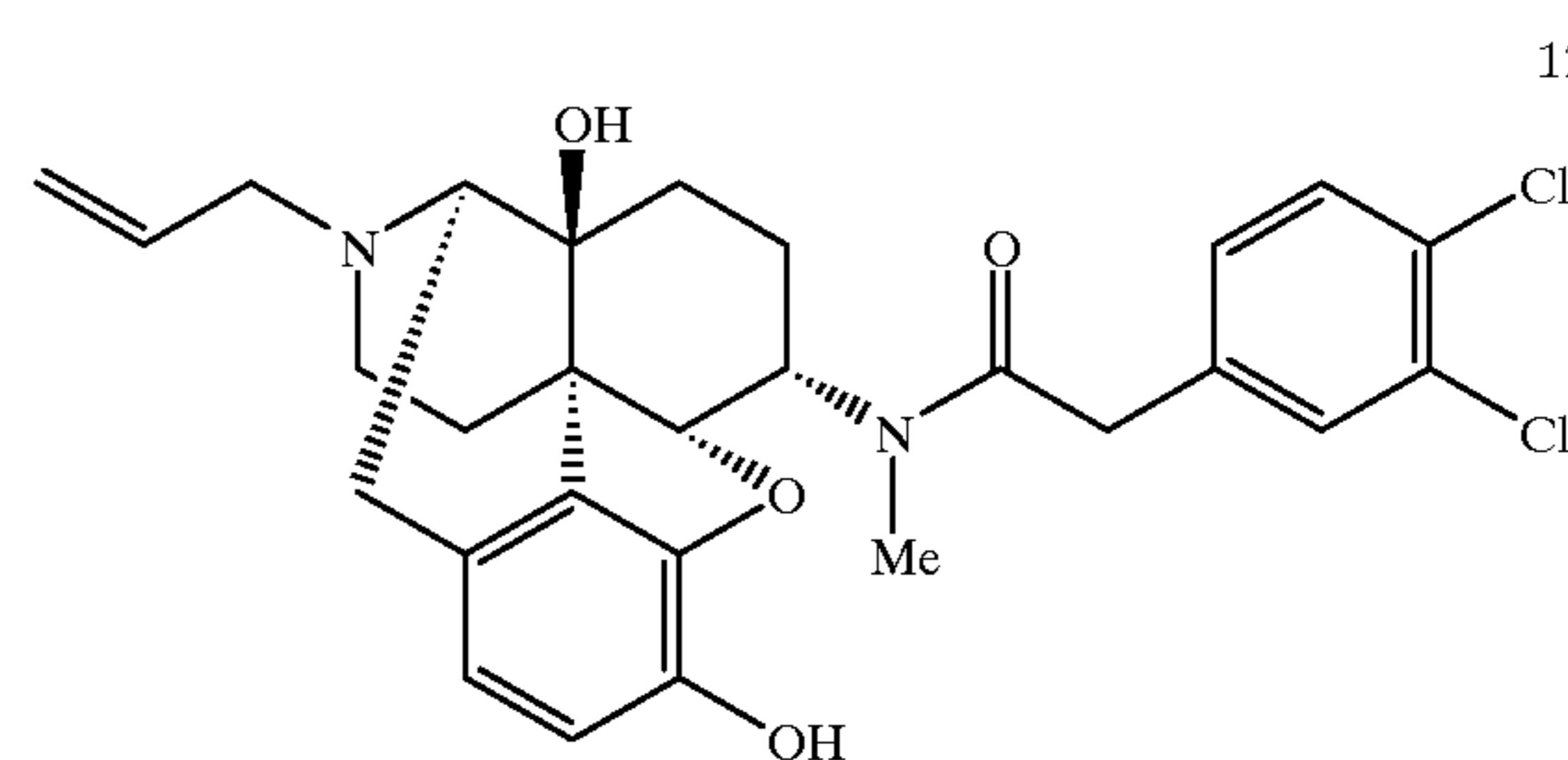
Compound 122
