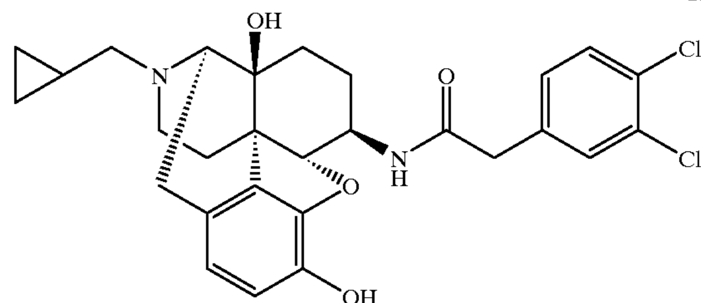
Compound 121
