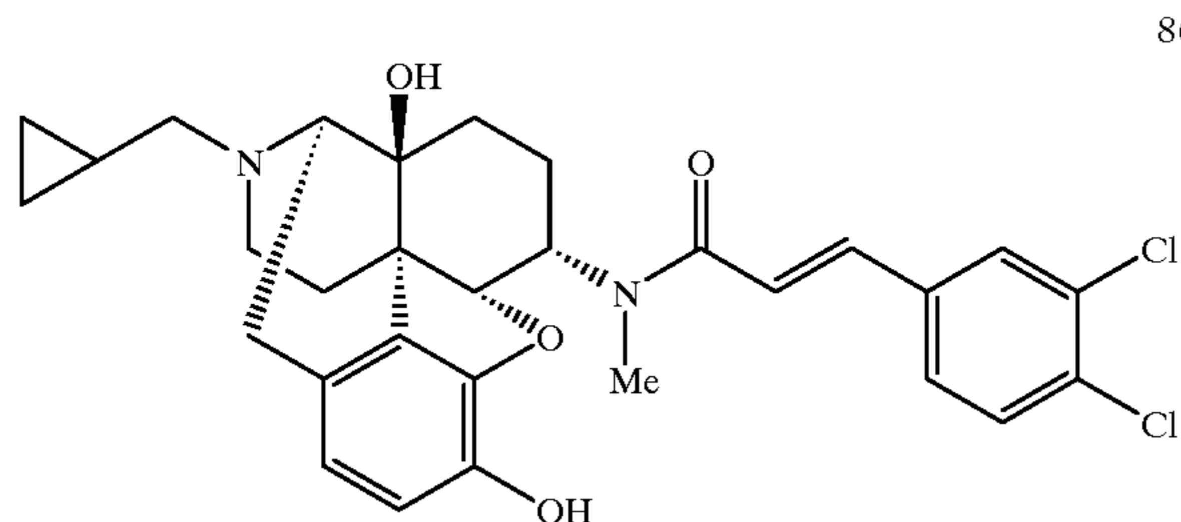
Compound 86
