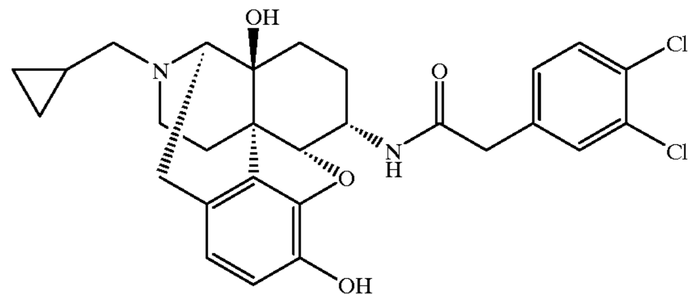
Compound 52
