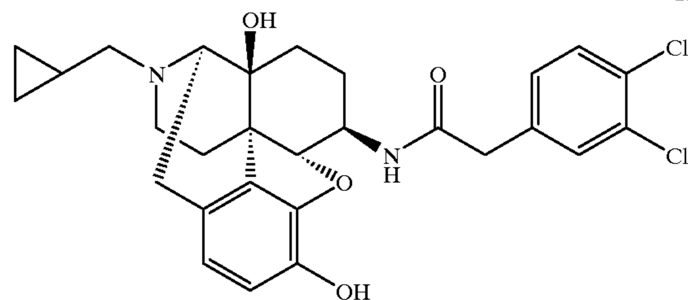
Compound 121
