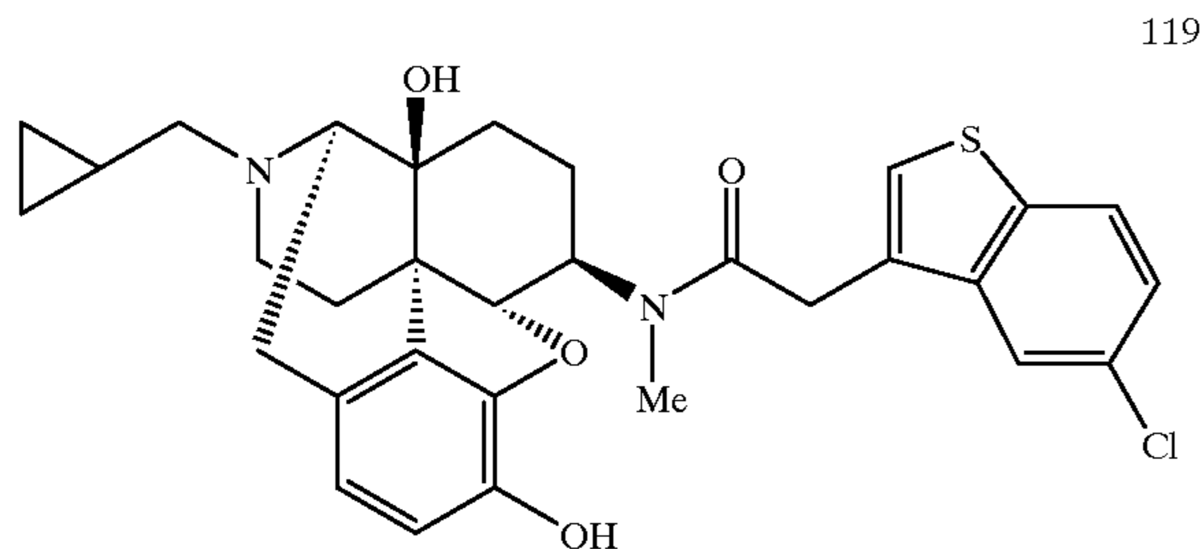
Compound 119
