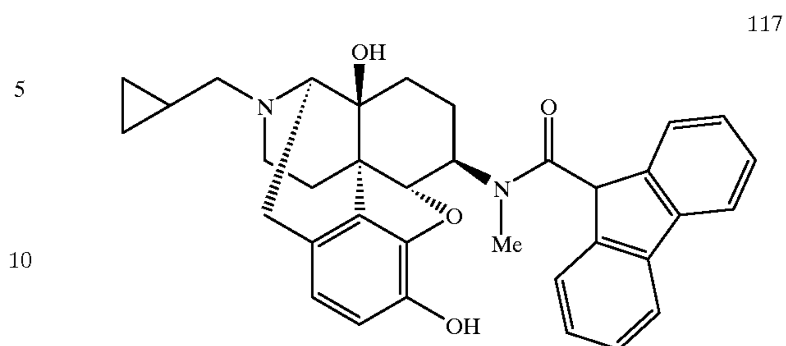
Compound 117
