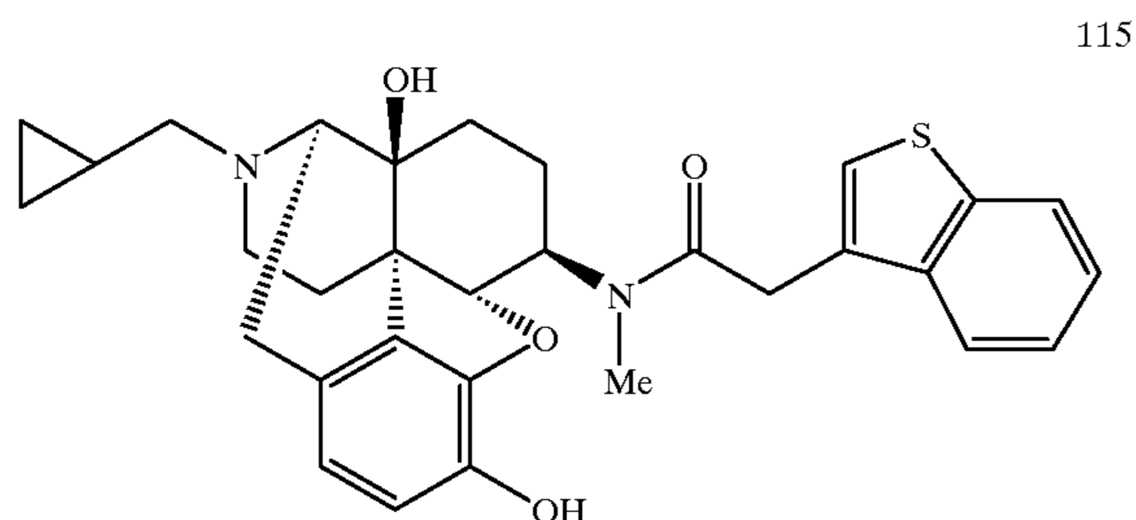
Compound 115
