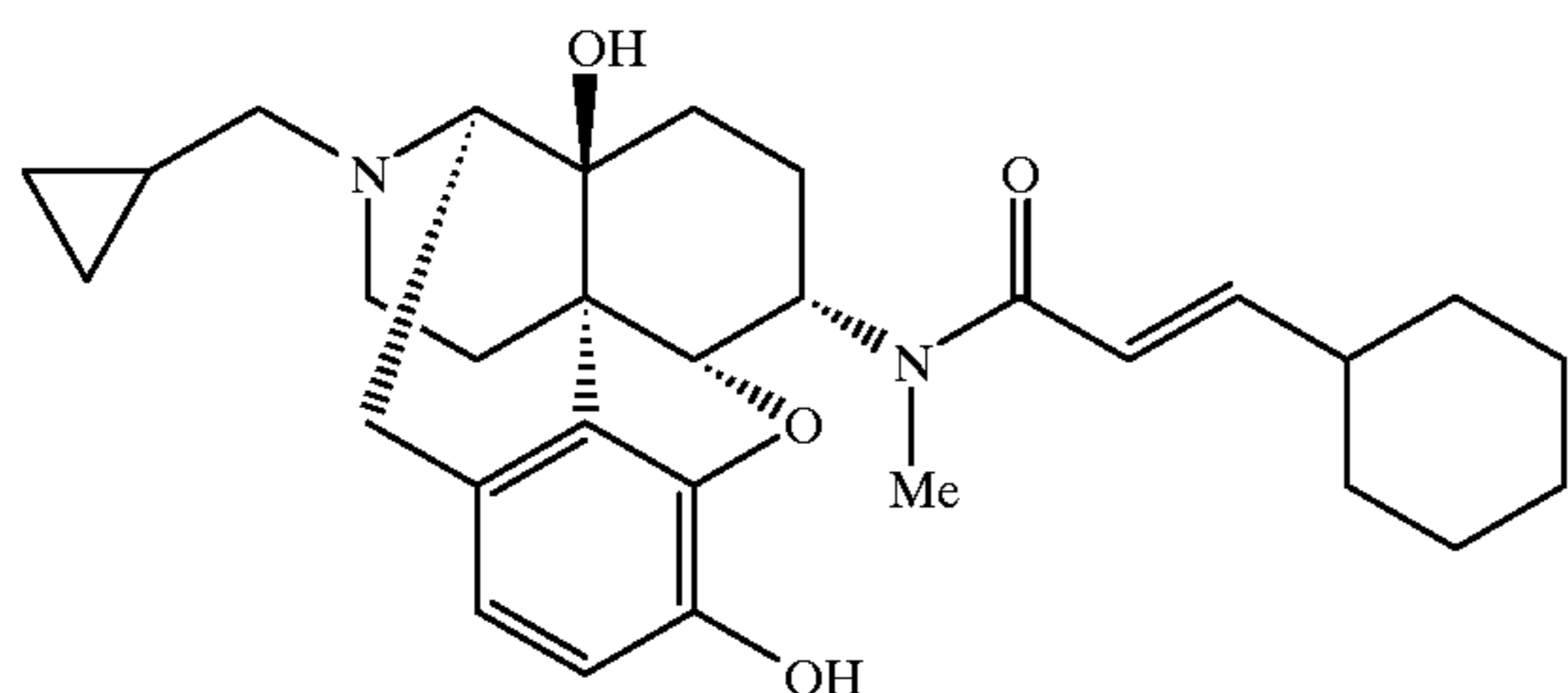
Compound 50
