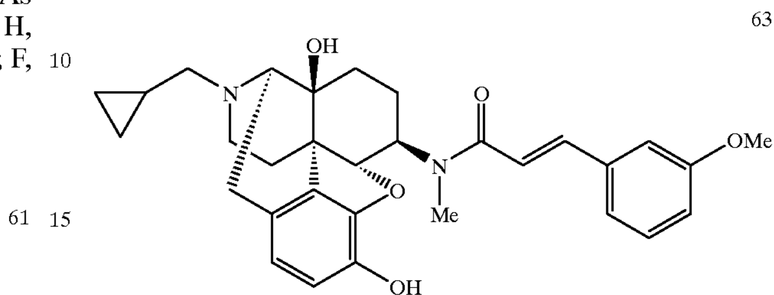
Compound 63
