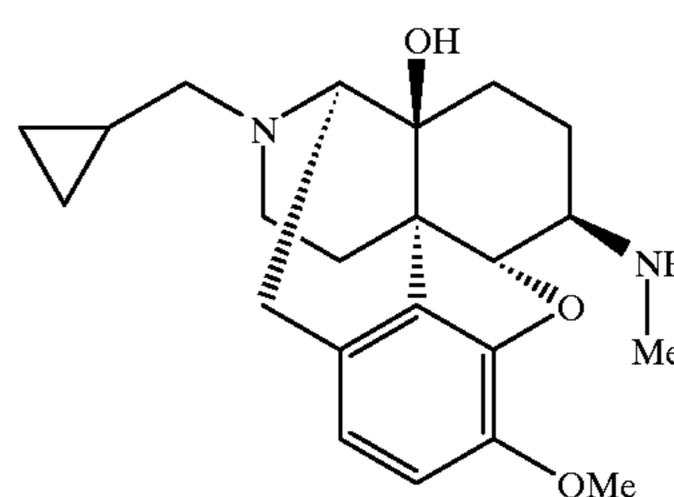
Compound 15
