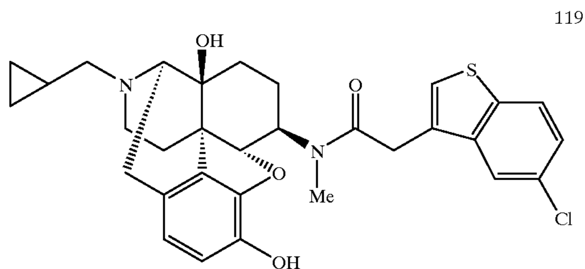
Compound 119
