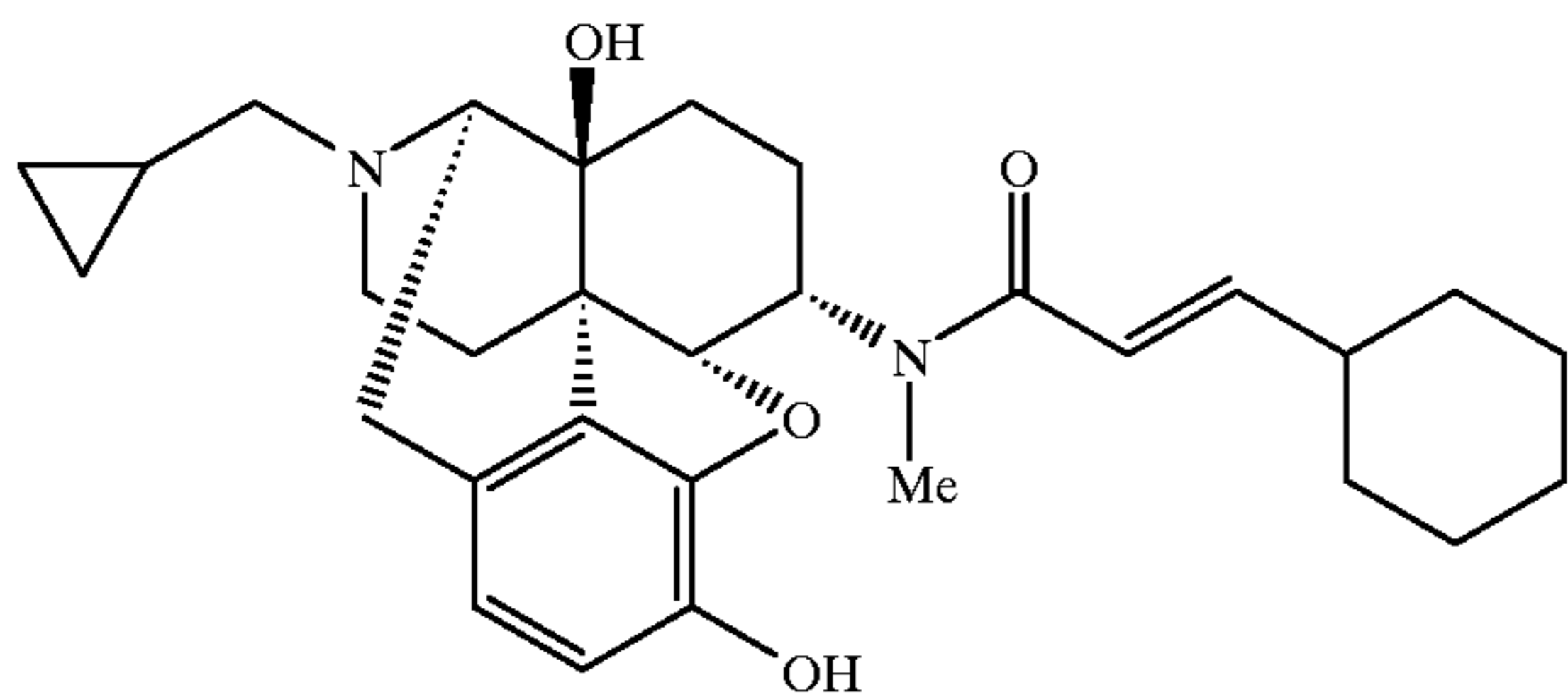
Compound 50
