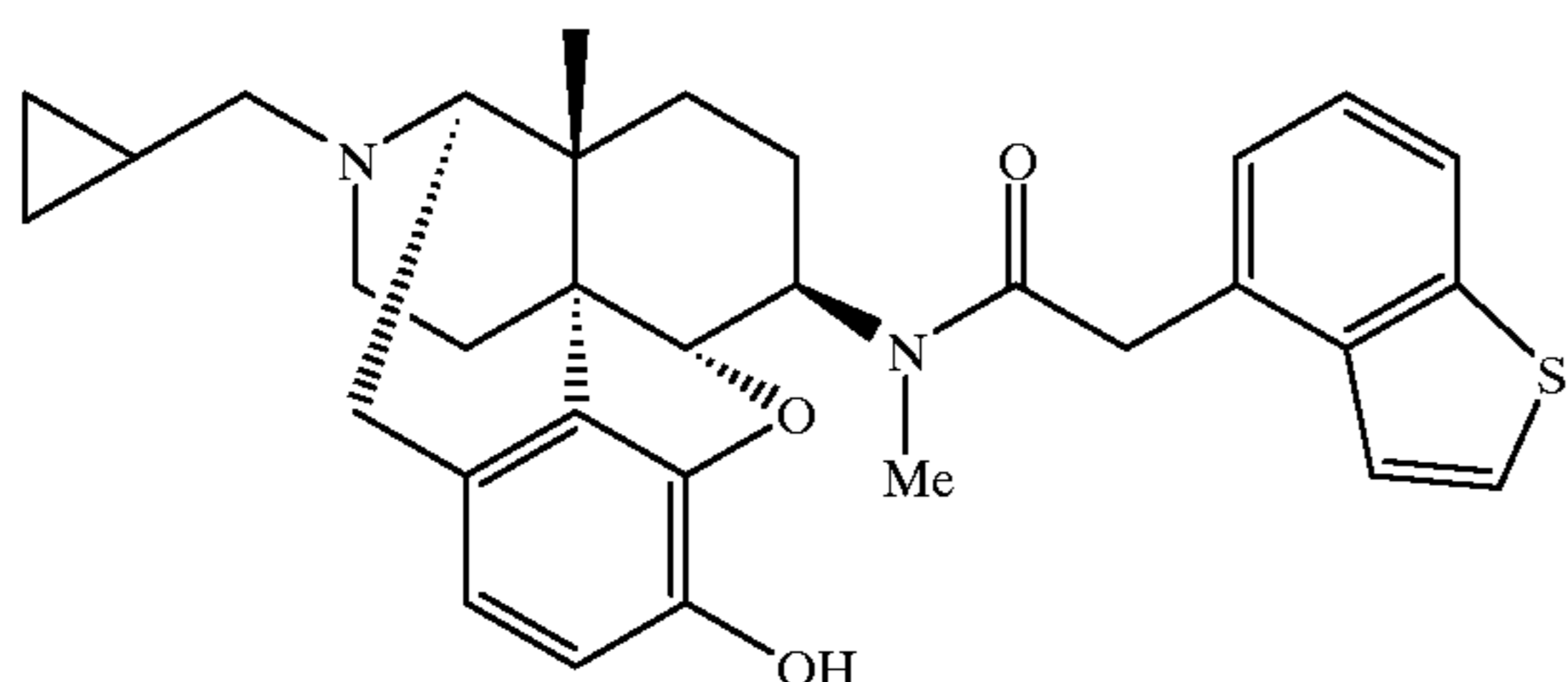
Compound 120
