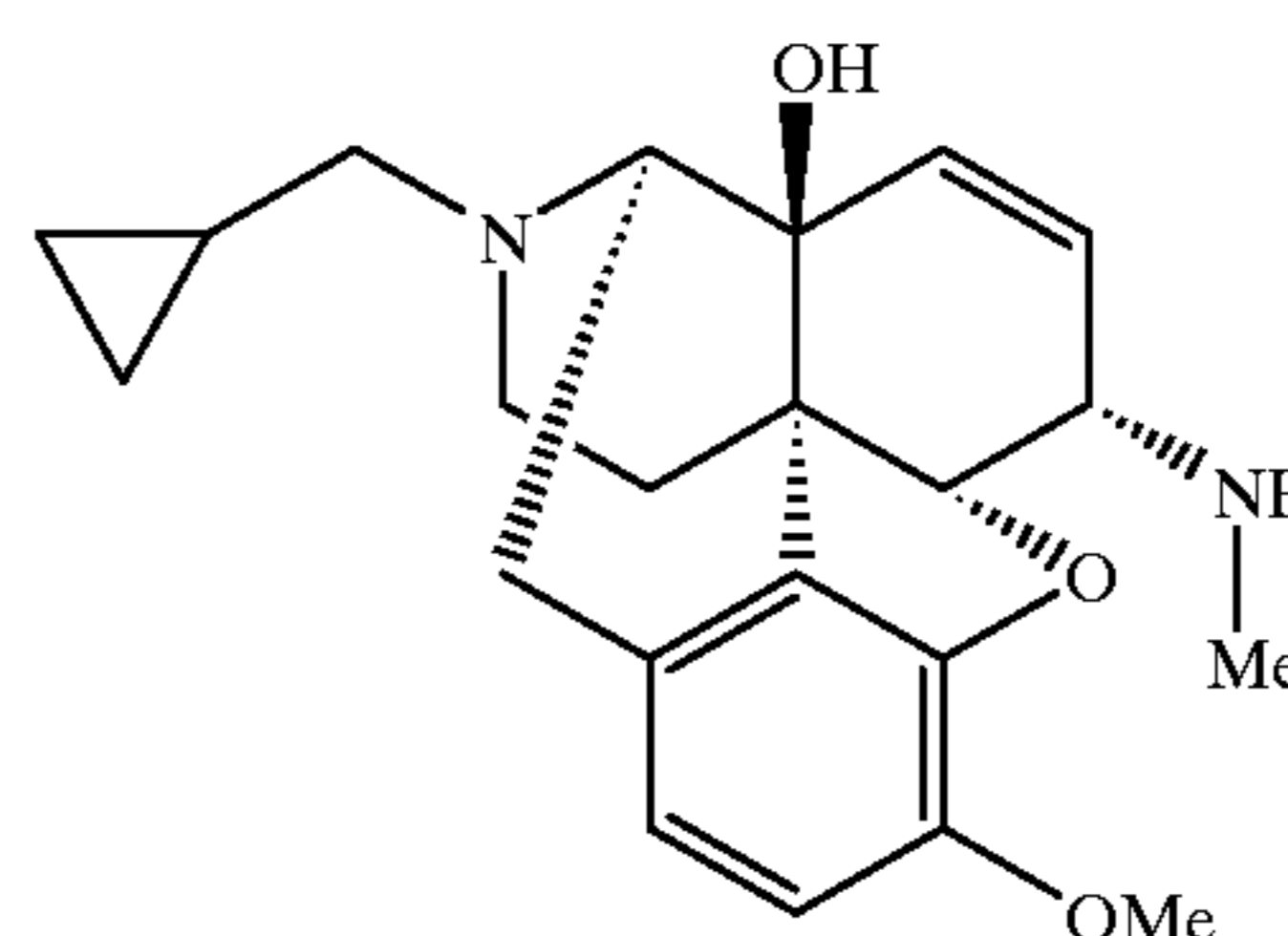
Compound 14
