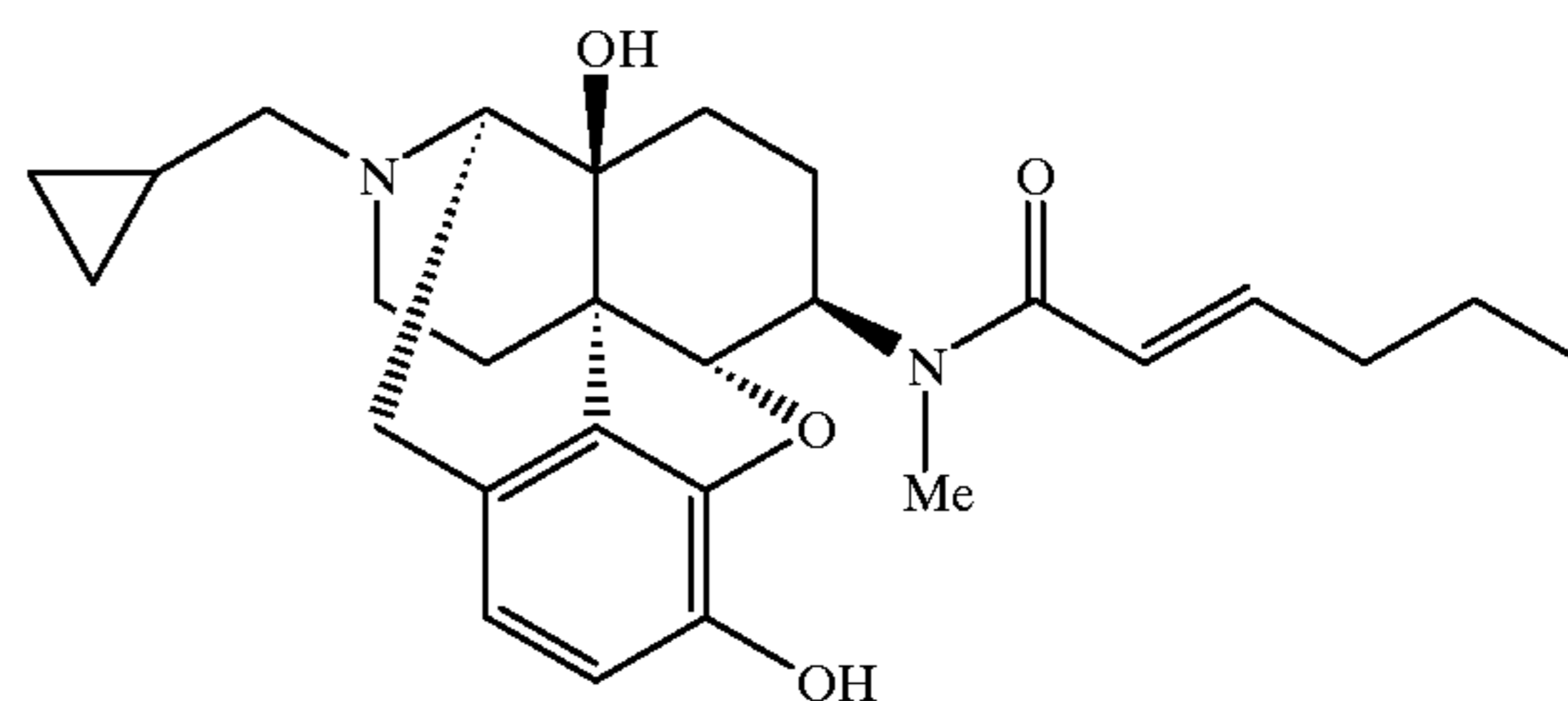
Compound 100
