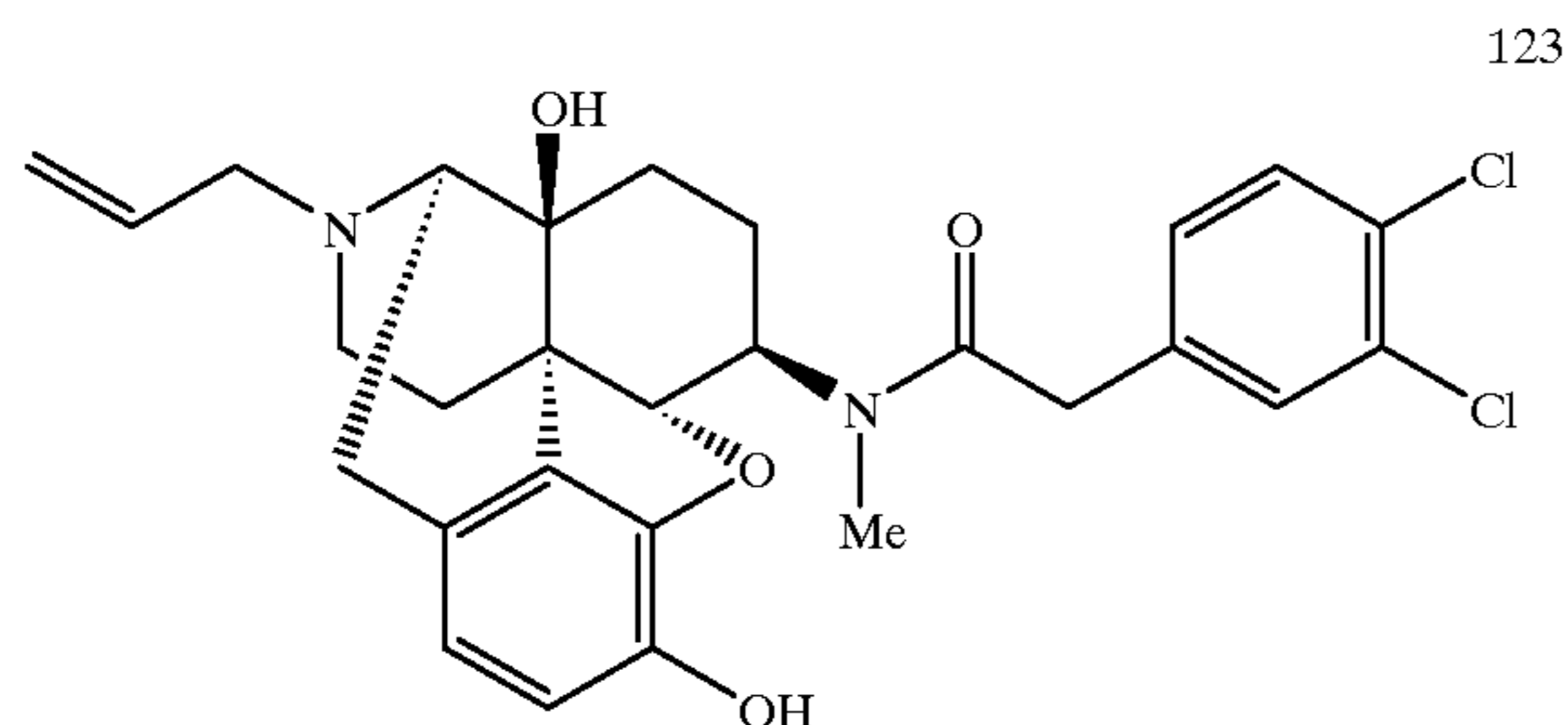
Compound 123
