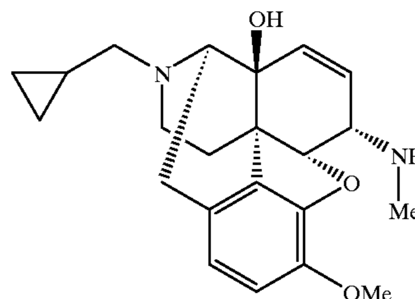
Compound 14
