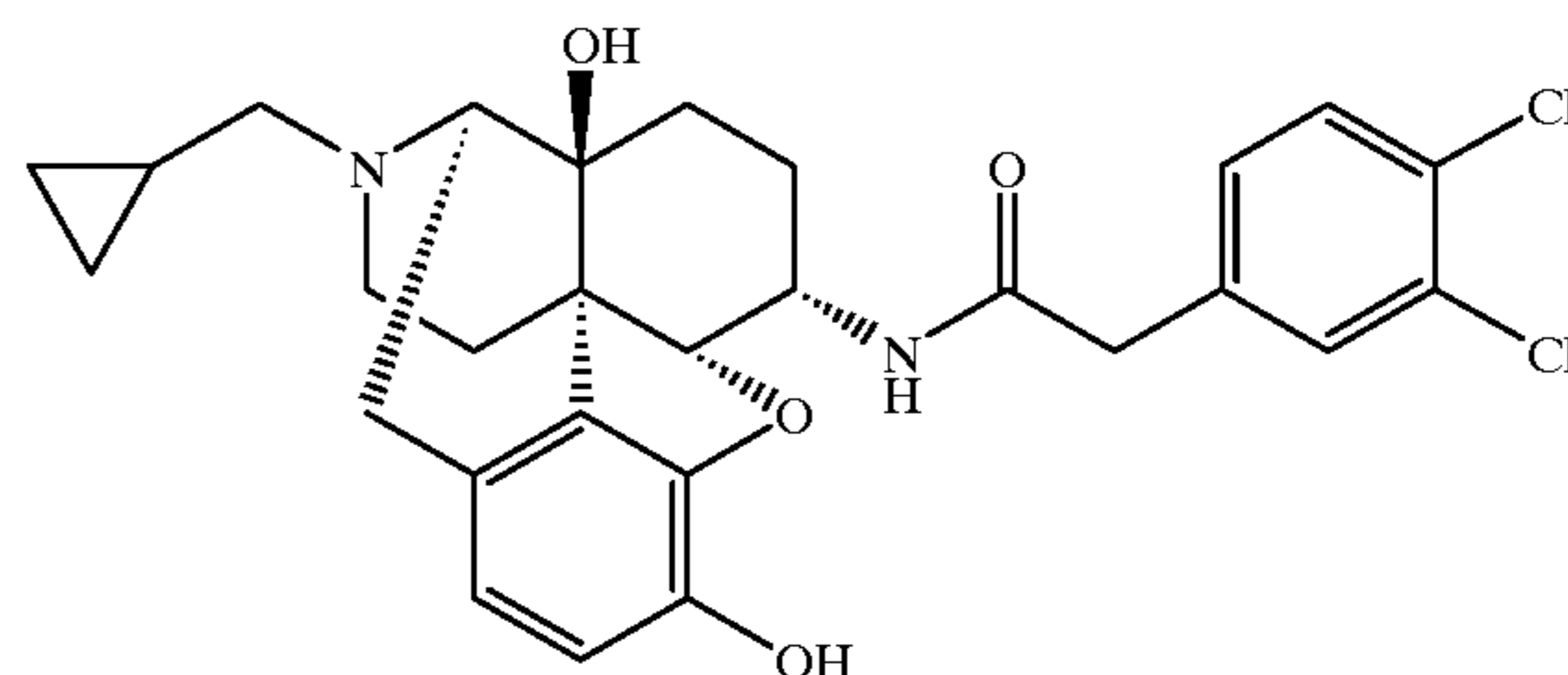
Compound 52
