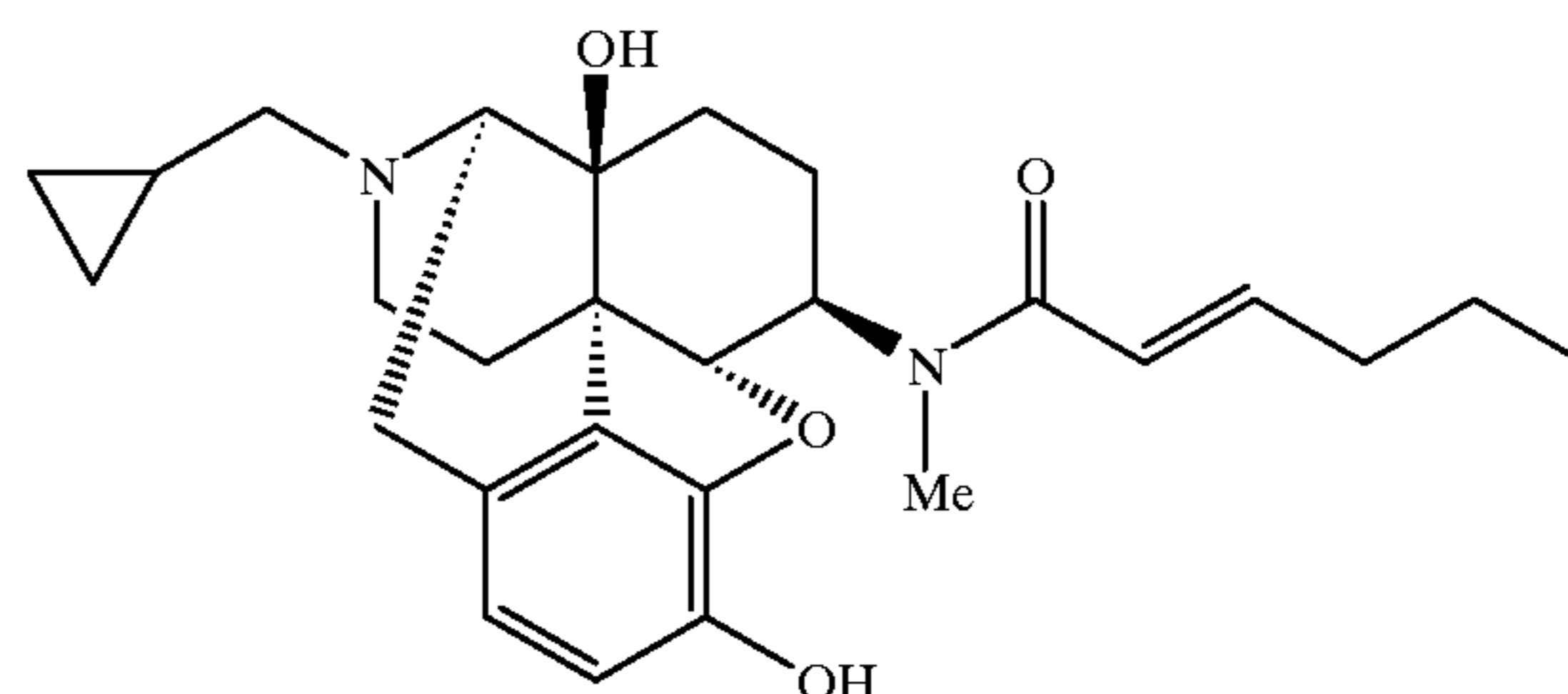
Compound 100
