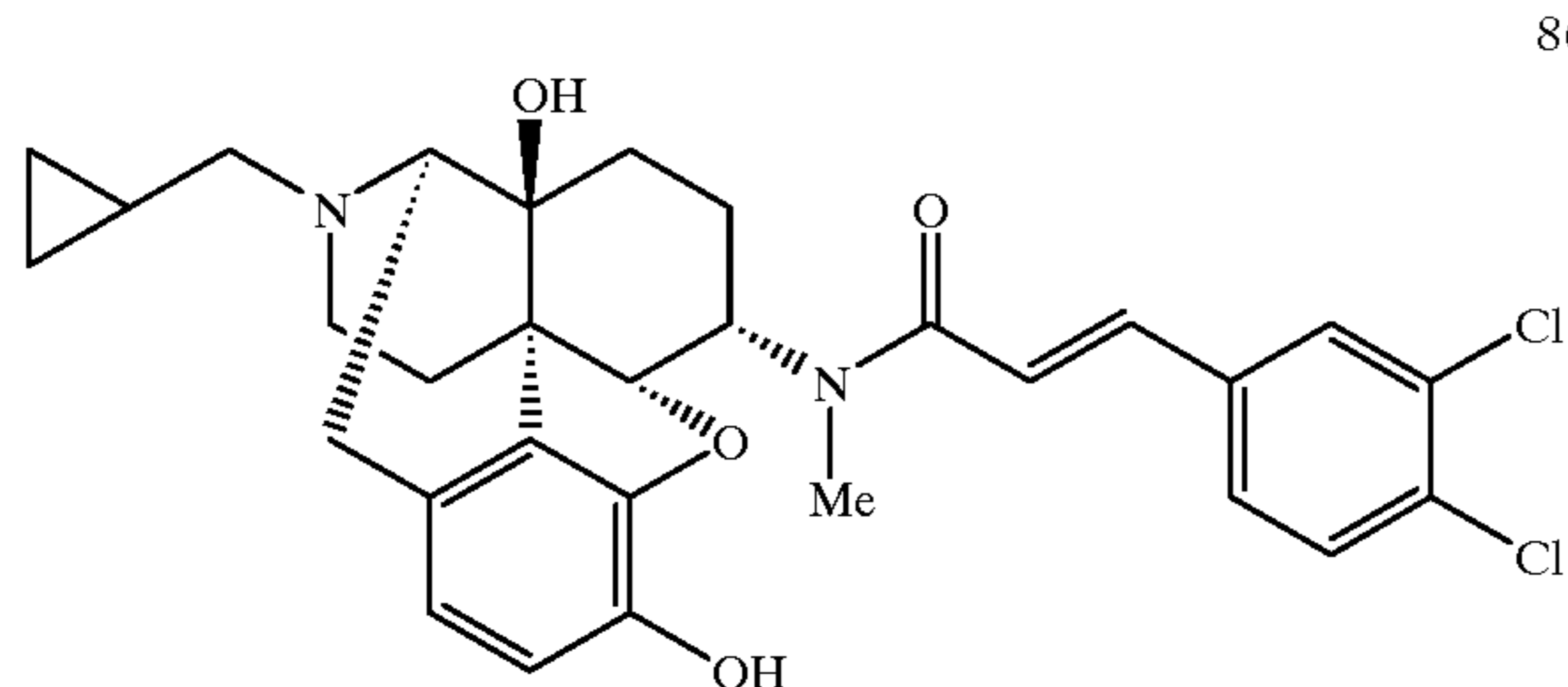
Compound 86
