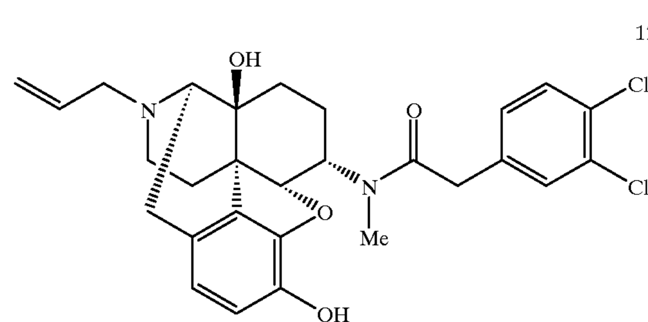
Compound 122
