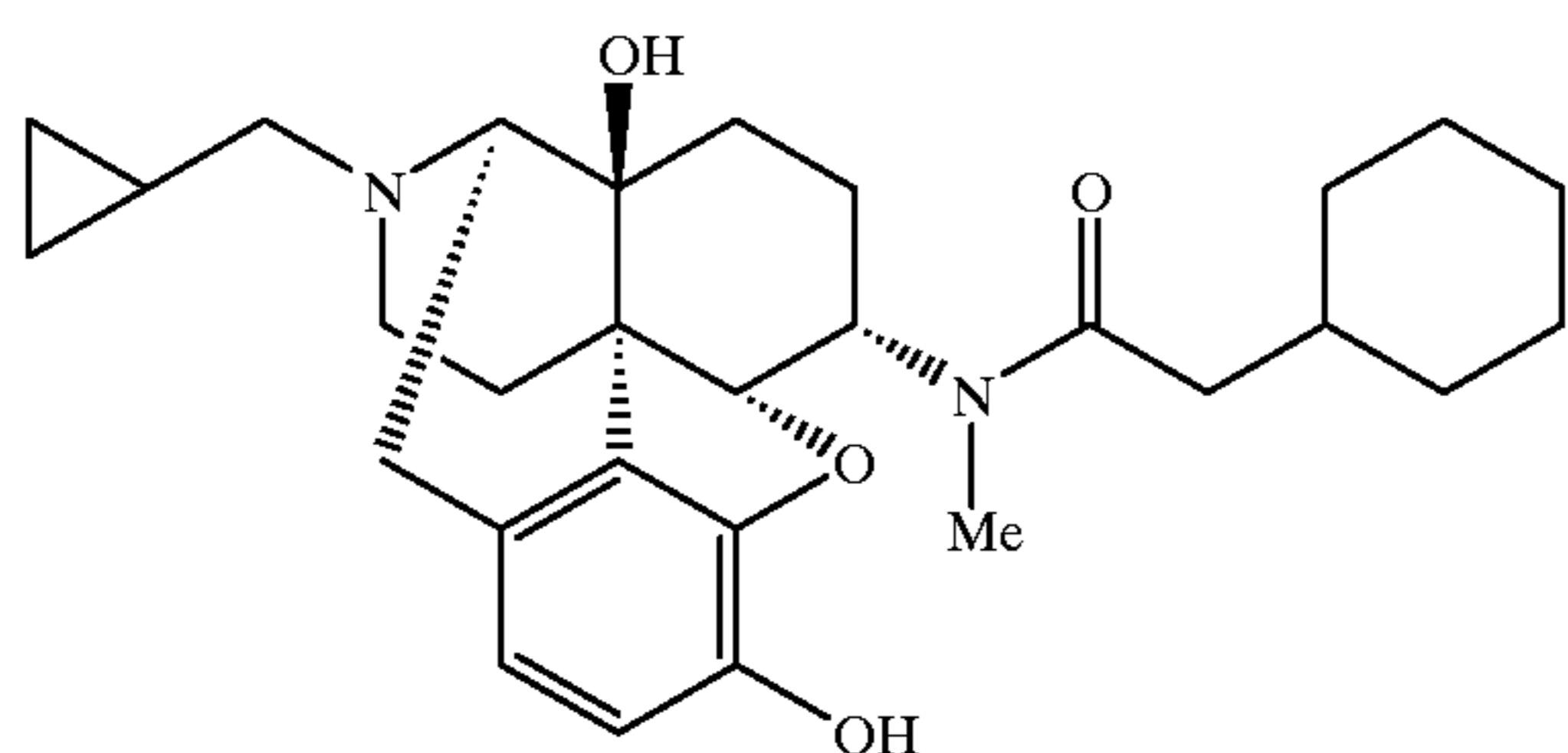
Compound 85
