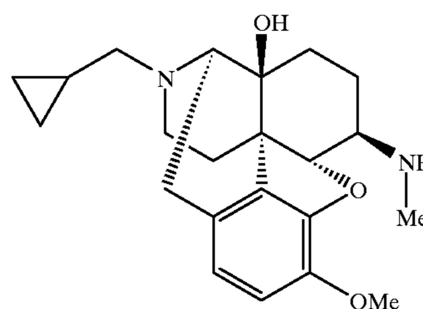
Compound 15
