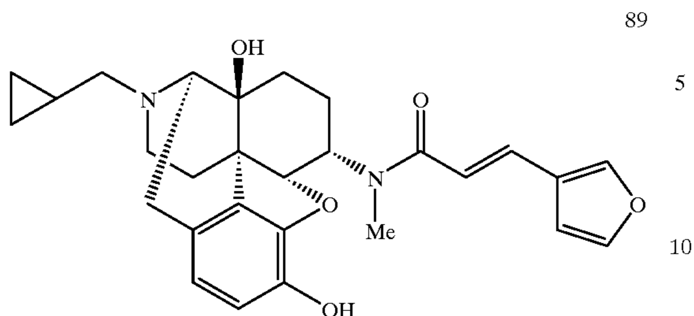
Compound 89
