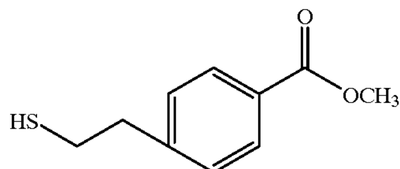
10c) Methyl 4-(2-thioethyl)benzoate
