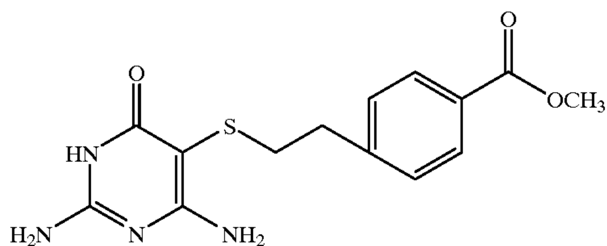
10d) Methyl 4-(2-[(2,6-diamino-4(3H)-oxypyrimidin-5-yl)thio]ethyl)benzoate
