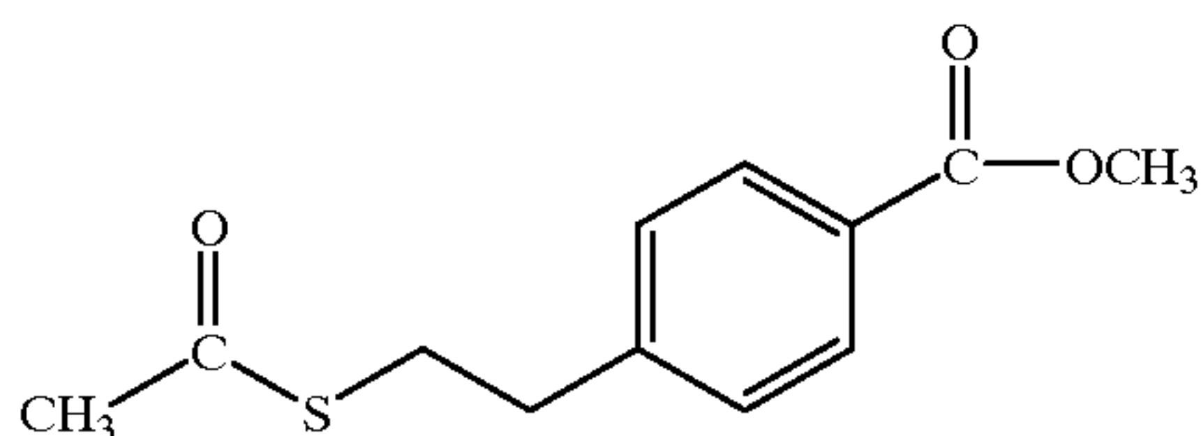
10b) Methyl 4-[2-(acetylthio)ethyl]benzoate
