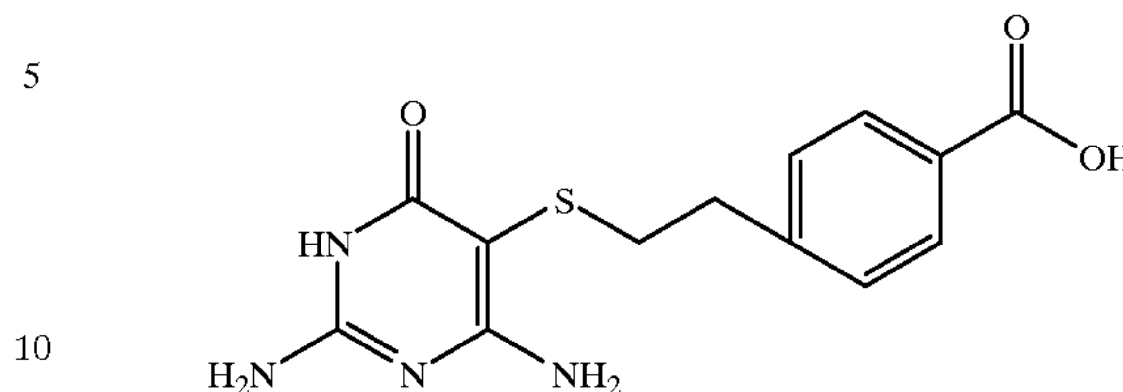
10e) 4-(2-[(2,6-Diamino-4(3H)-oxypyrimidin-5-yl)thio]ethyl)benzoic acid
