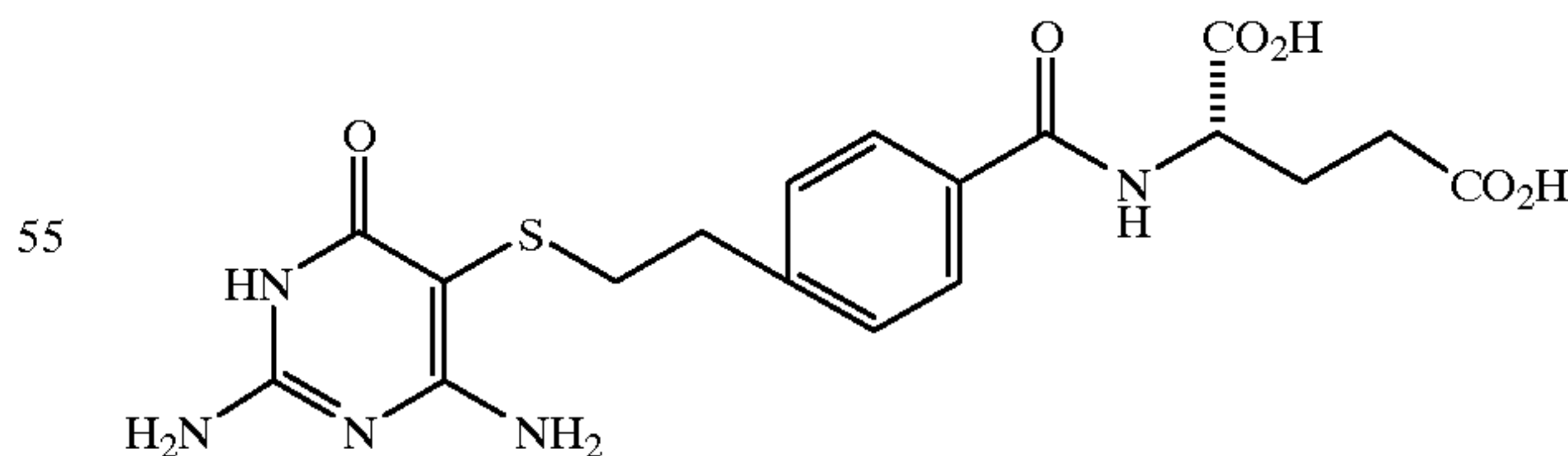
10g N-(4-[2-[(2,6-diamino-4(3H)-oxypyrimidin-5-yl)thio]ethyl]benzoyl)-L-glutamic acid
