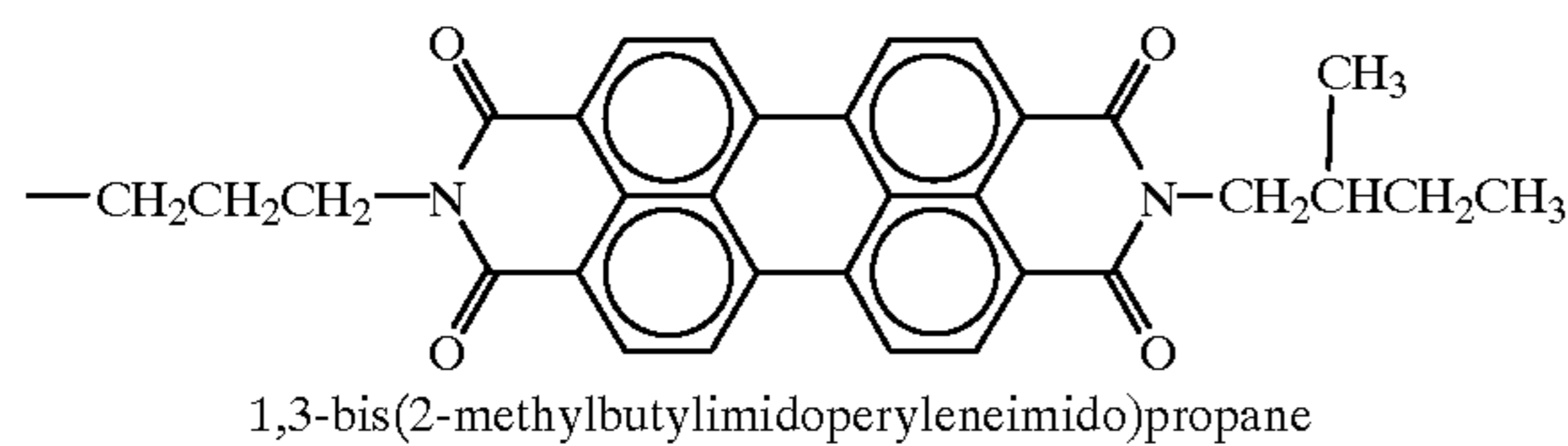
Formula C
