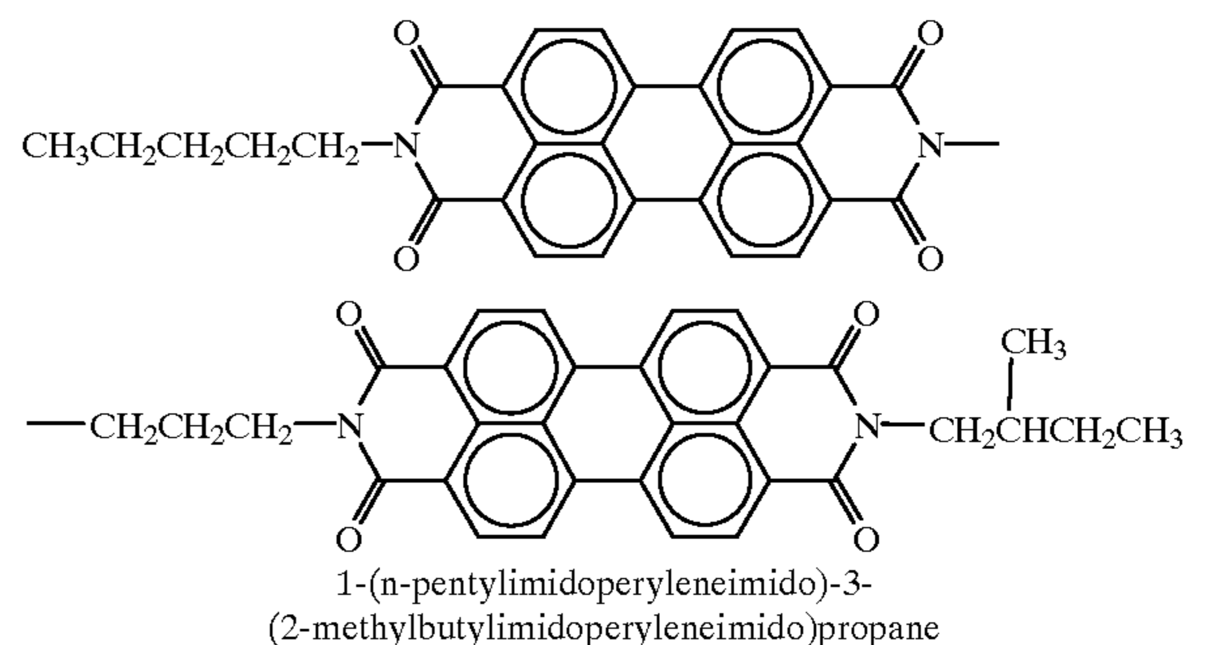
Formula C
