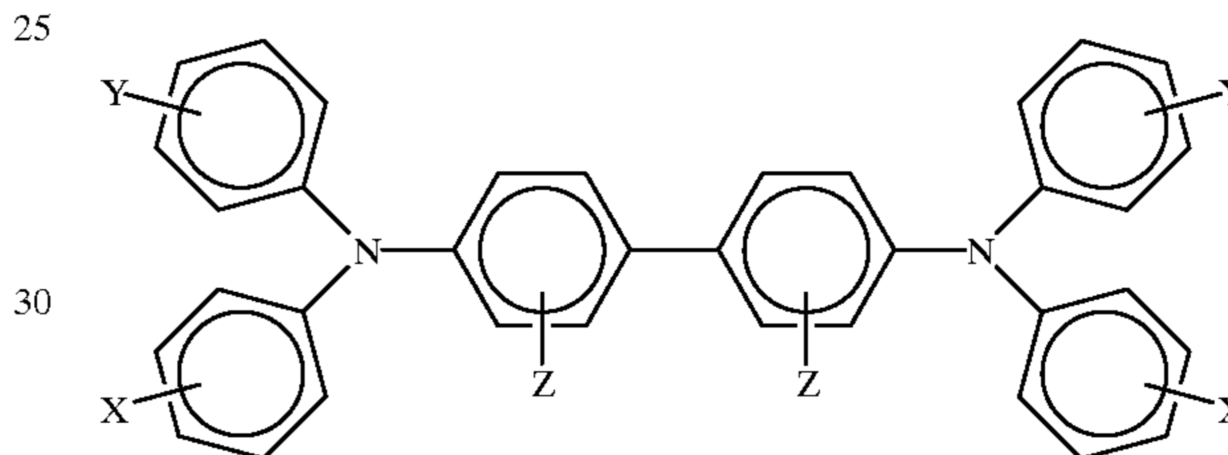
Formula B
