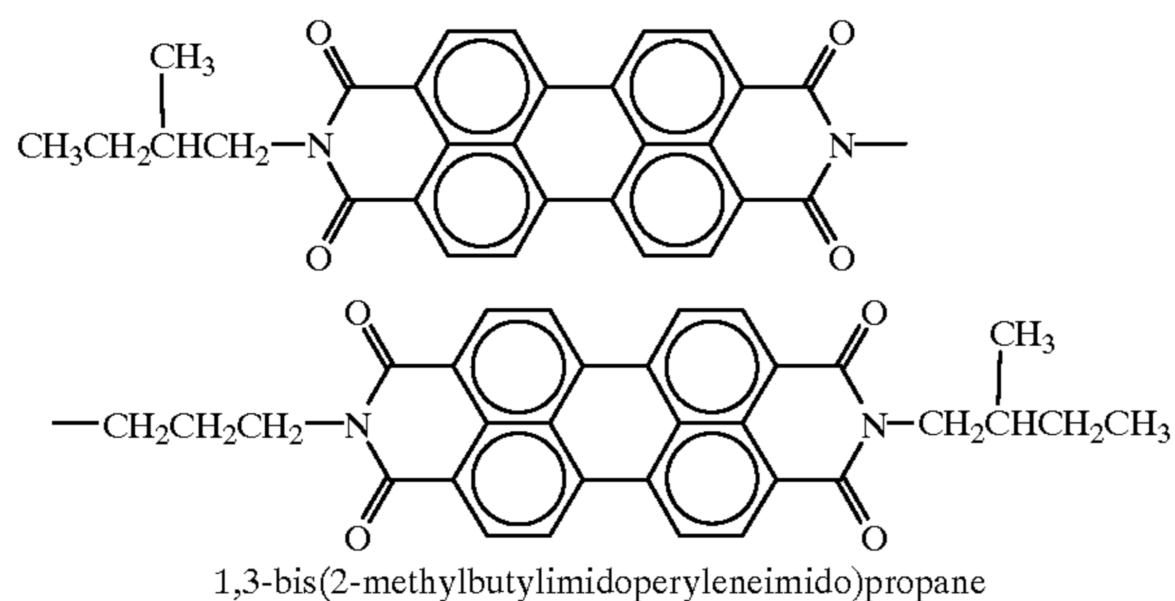
FORMULA B
