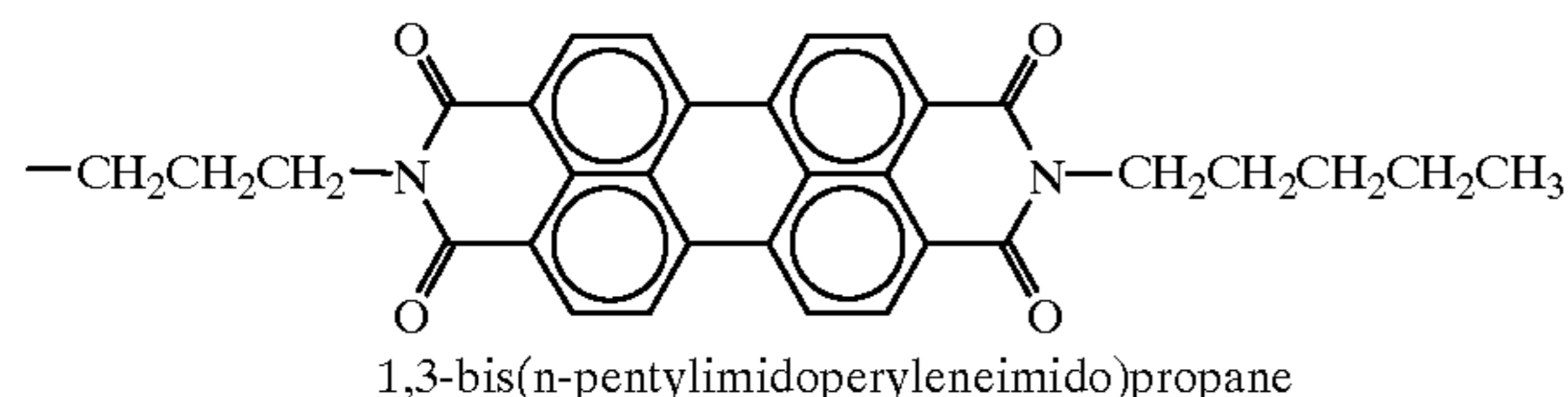
Formula B
