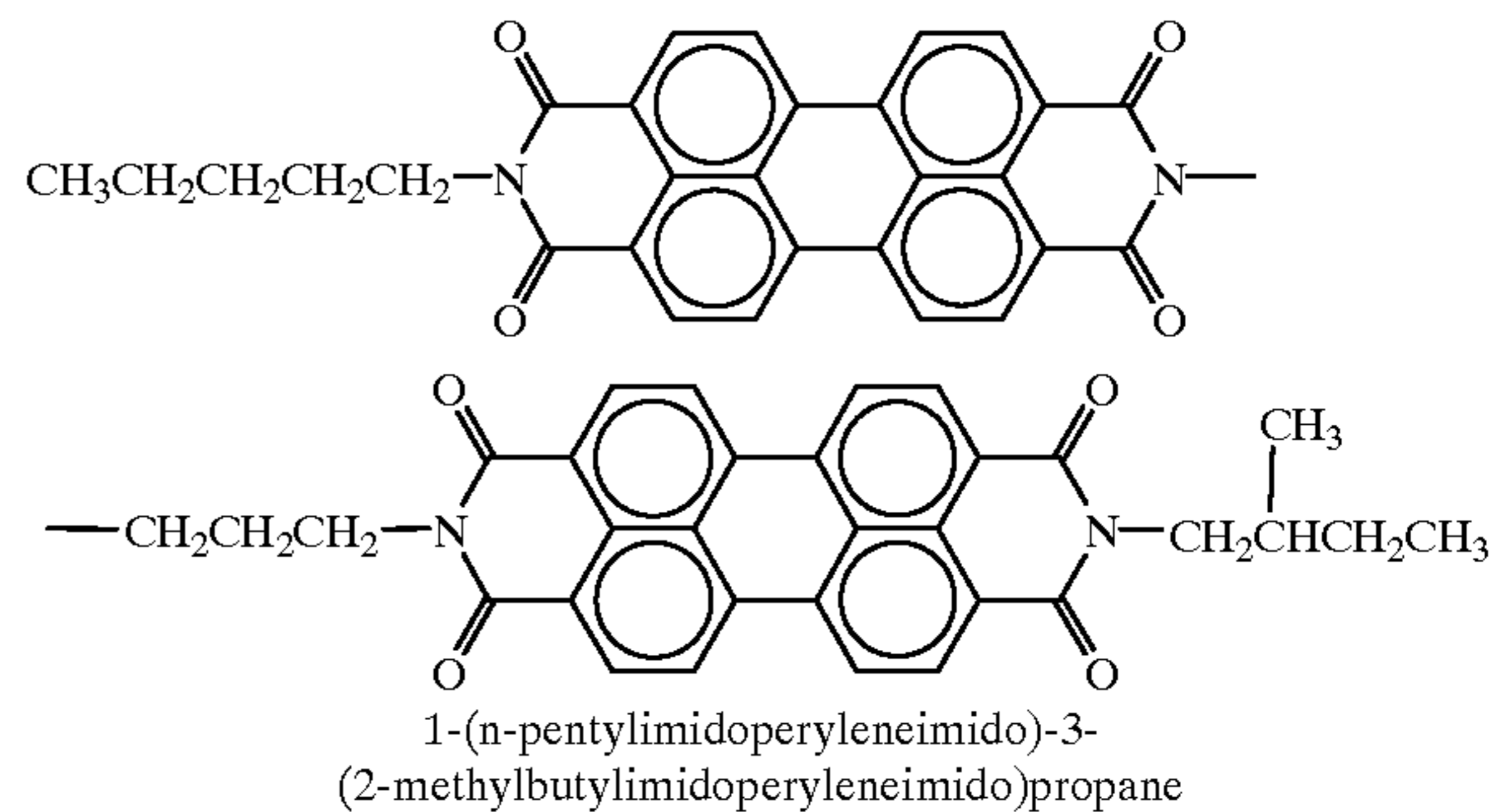
FORMULA C
