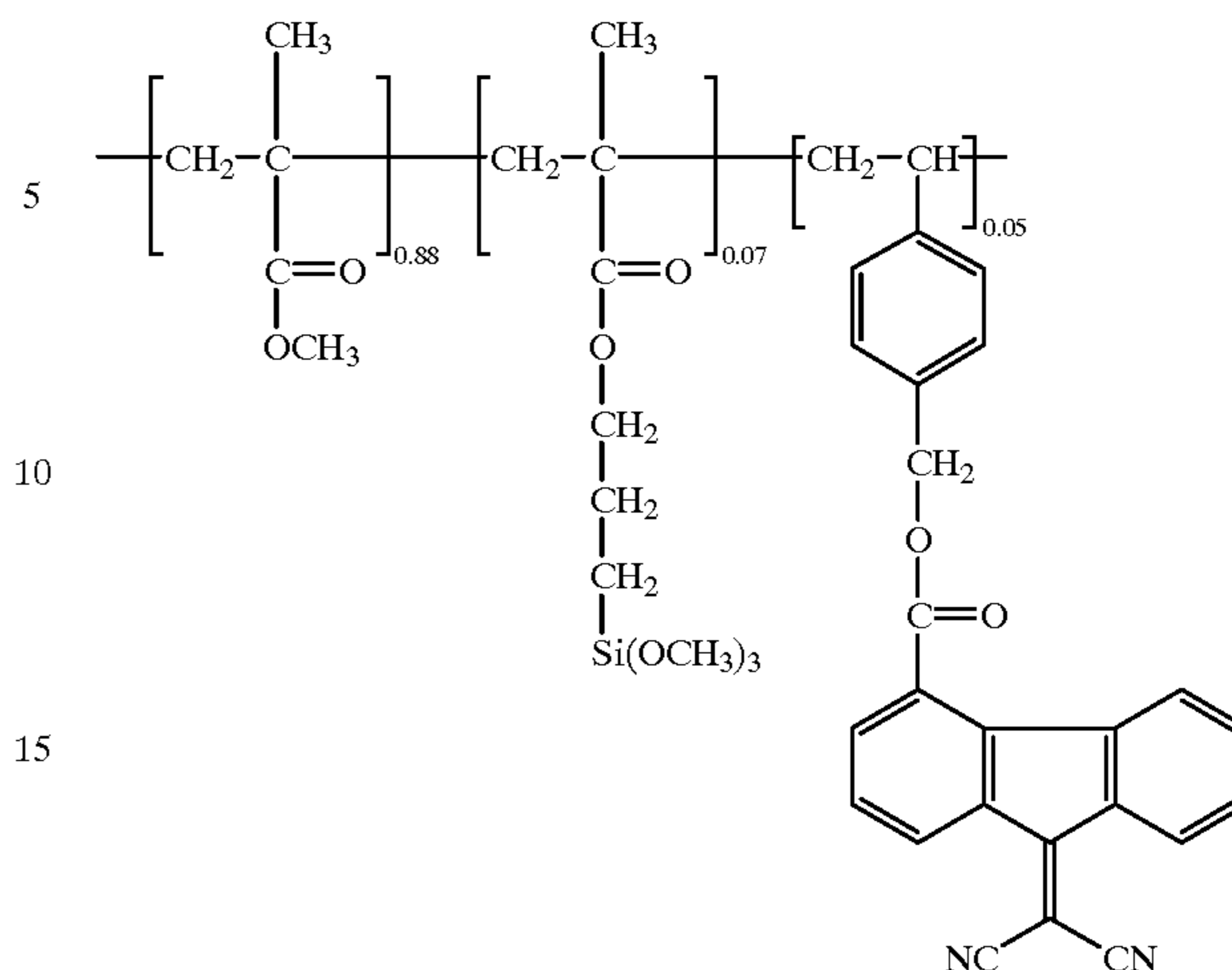
Formula A
