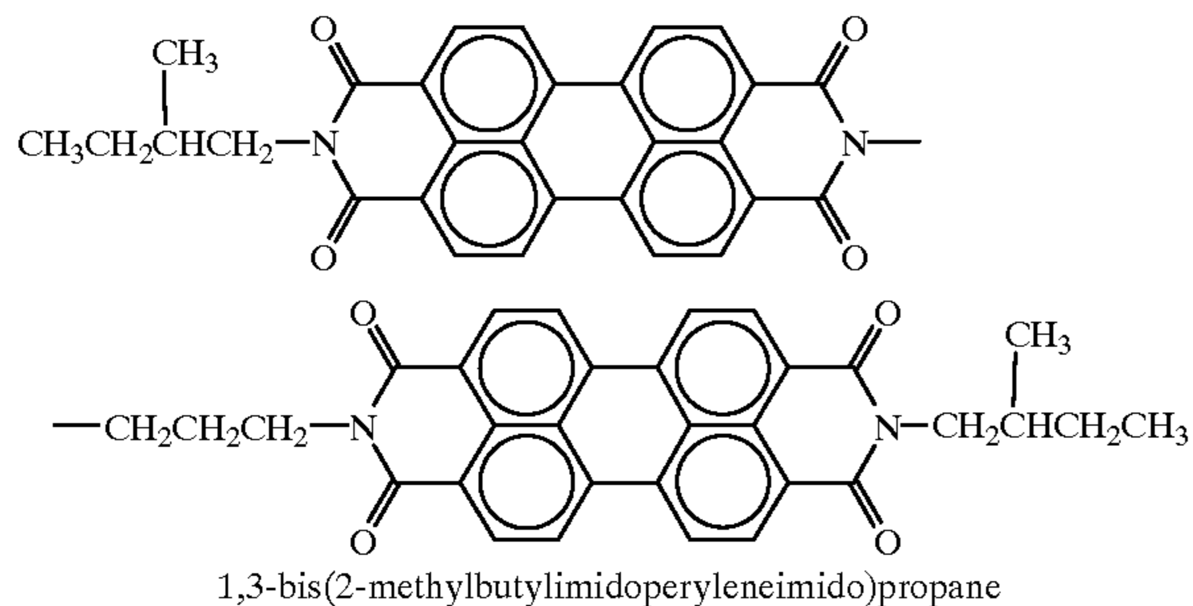
FORMULA B
