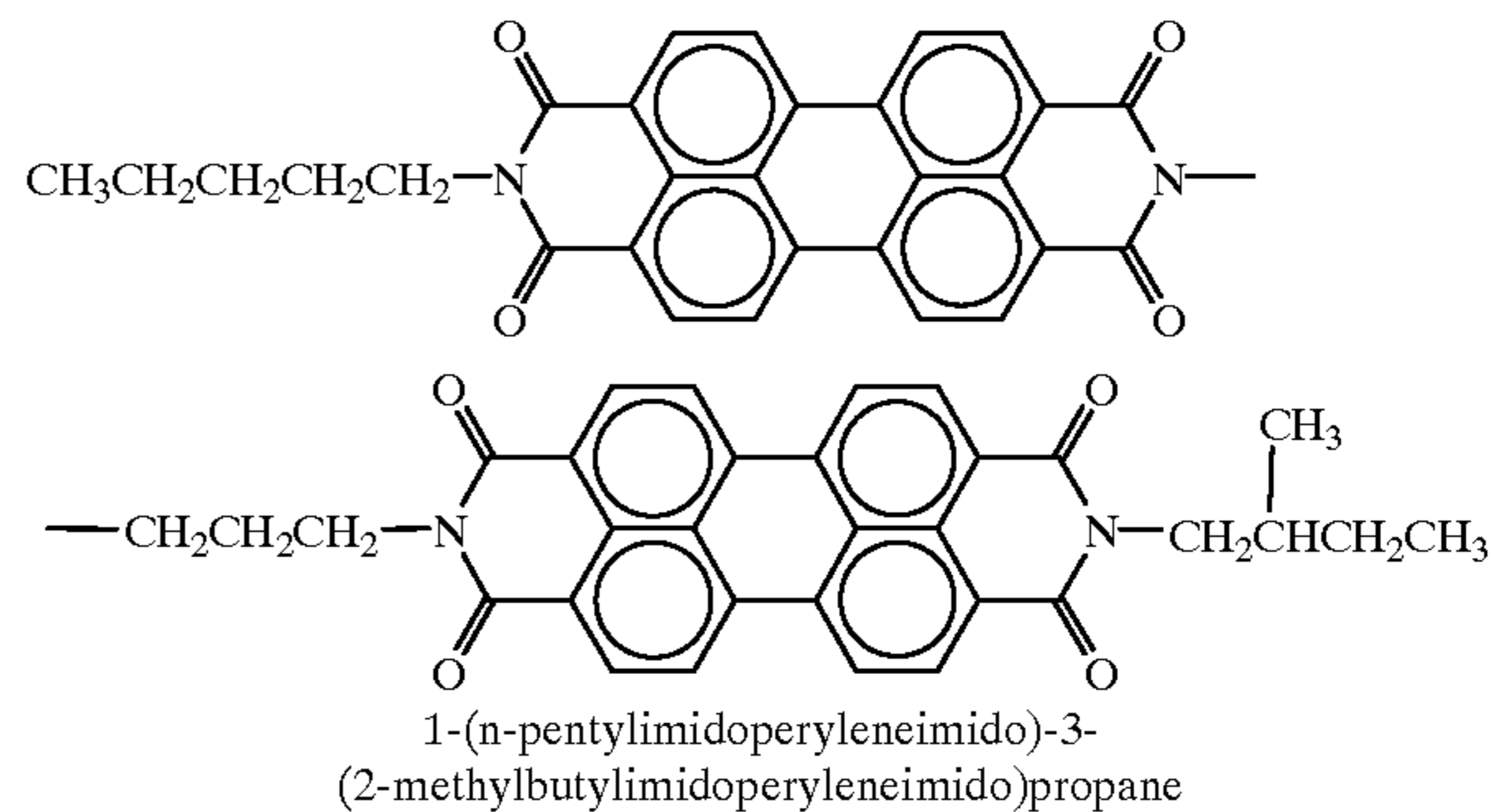
FORMULA C
