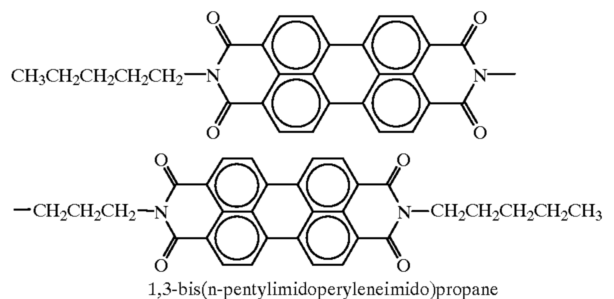
Formula B
