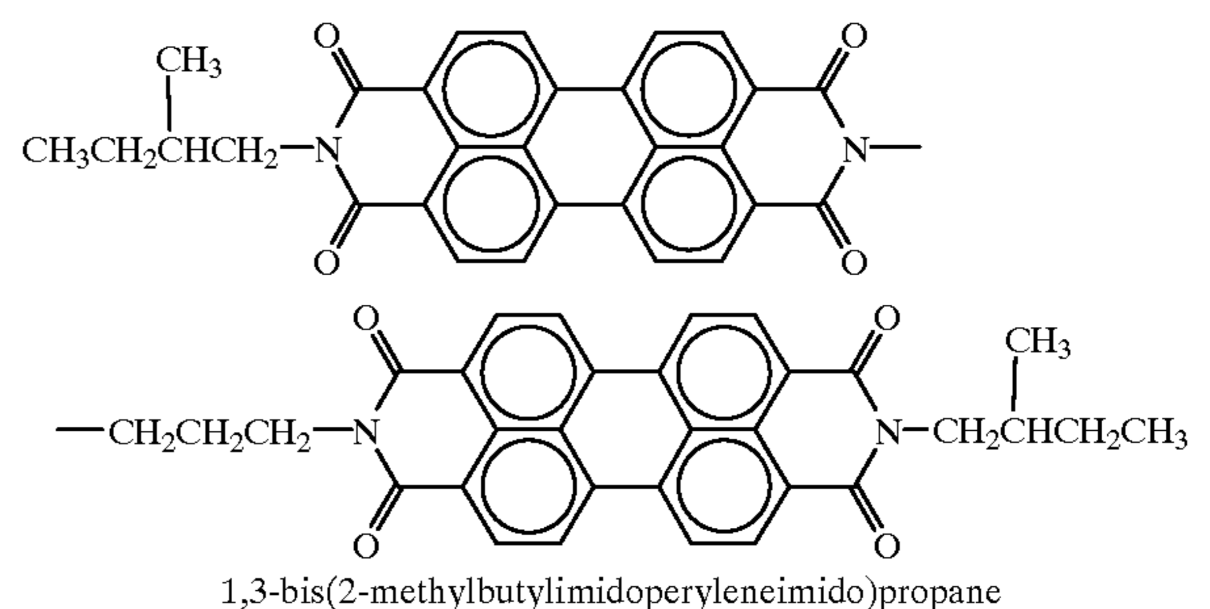
Formula C
