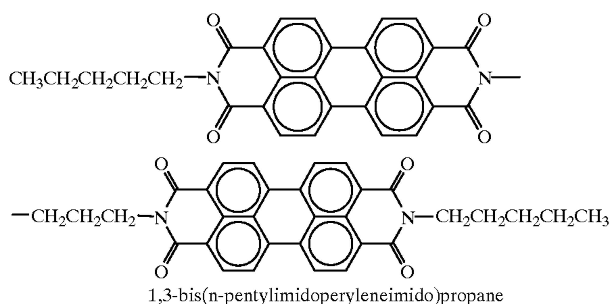
FORMULA B
