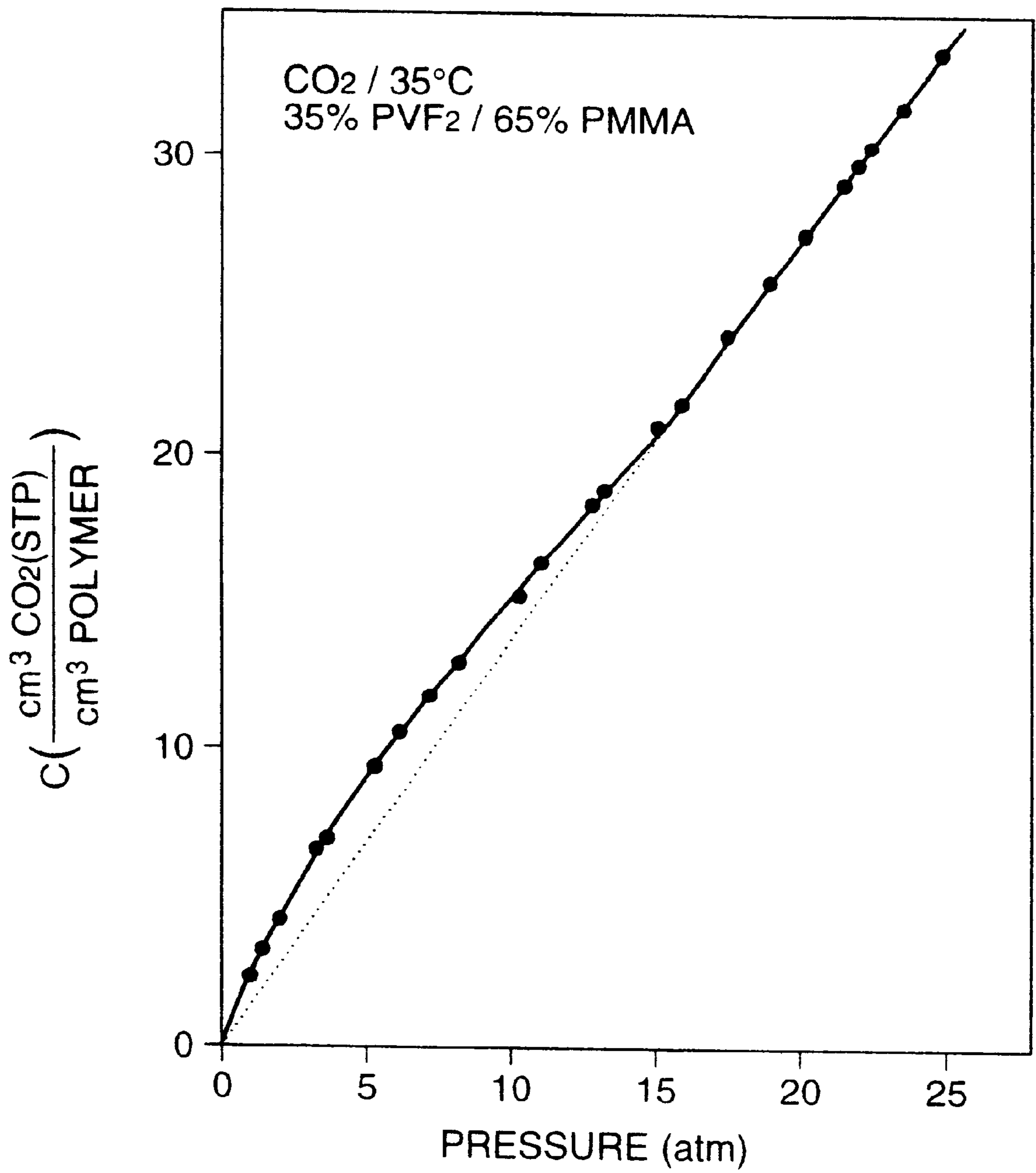
SOLUBILITY OF CARBON DIOXIDE IN PMMA/PVF 2 POLYMER ALLOY
