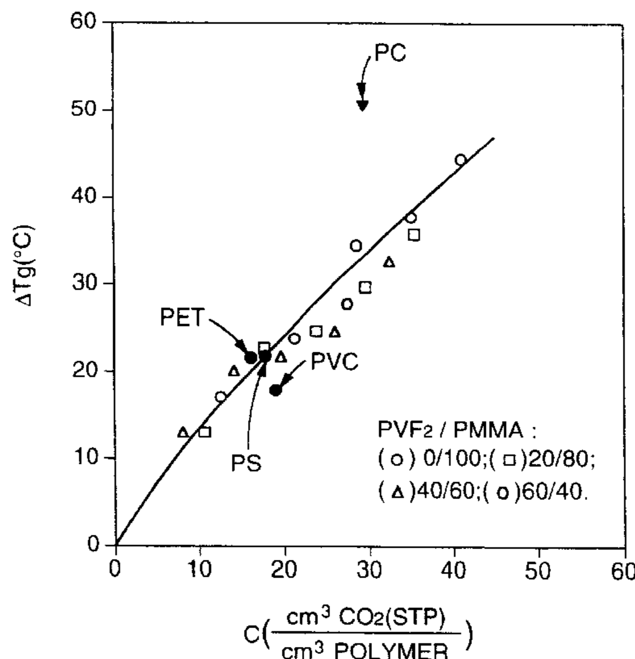
REDUCTION OF T g OF THE SYNTHETIC RESINS DUE TO DISSOLUTION OF CARBON DIOXIDE IN EACH RESIN
