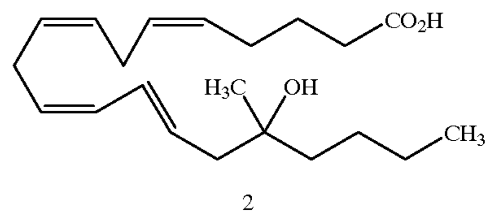
(5Z,8Z,11Z,13E)-(16RS)-16-Hydroxy-16-methyleicosa-5,8,11,13-tetraenoic acid (2)
