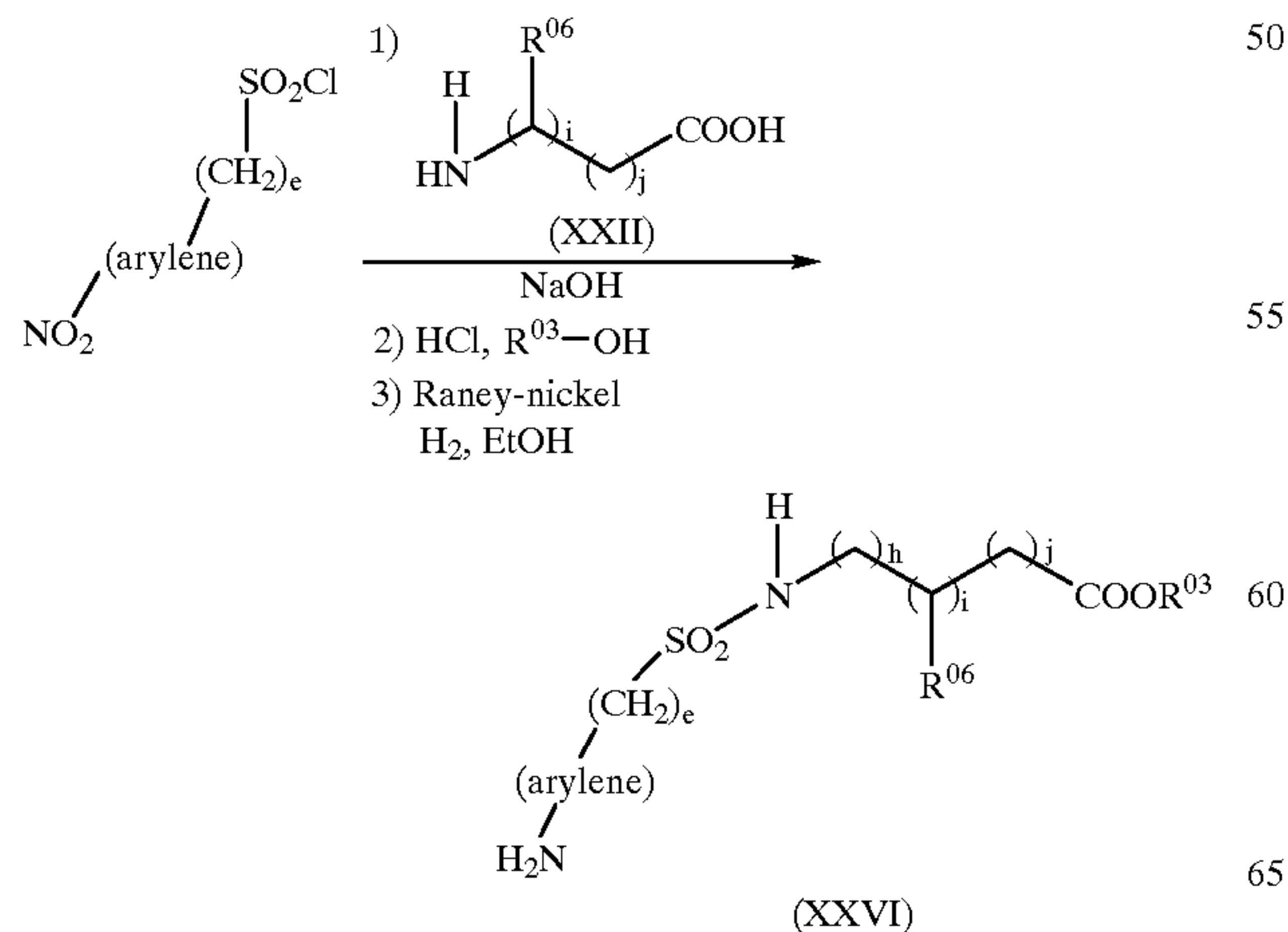
Scheme 5b
