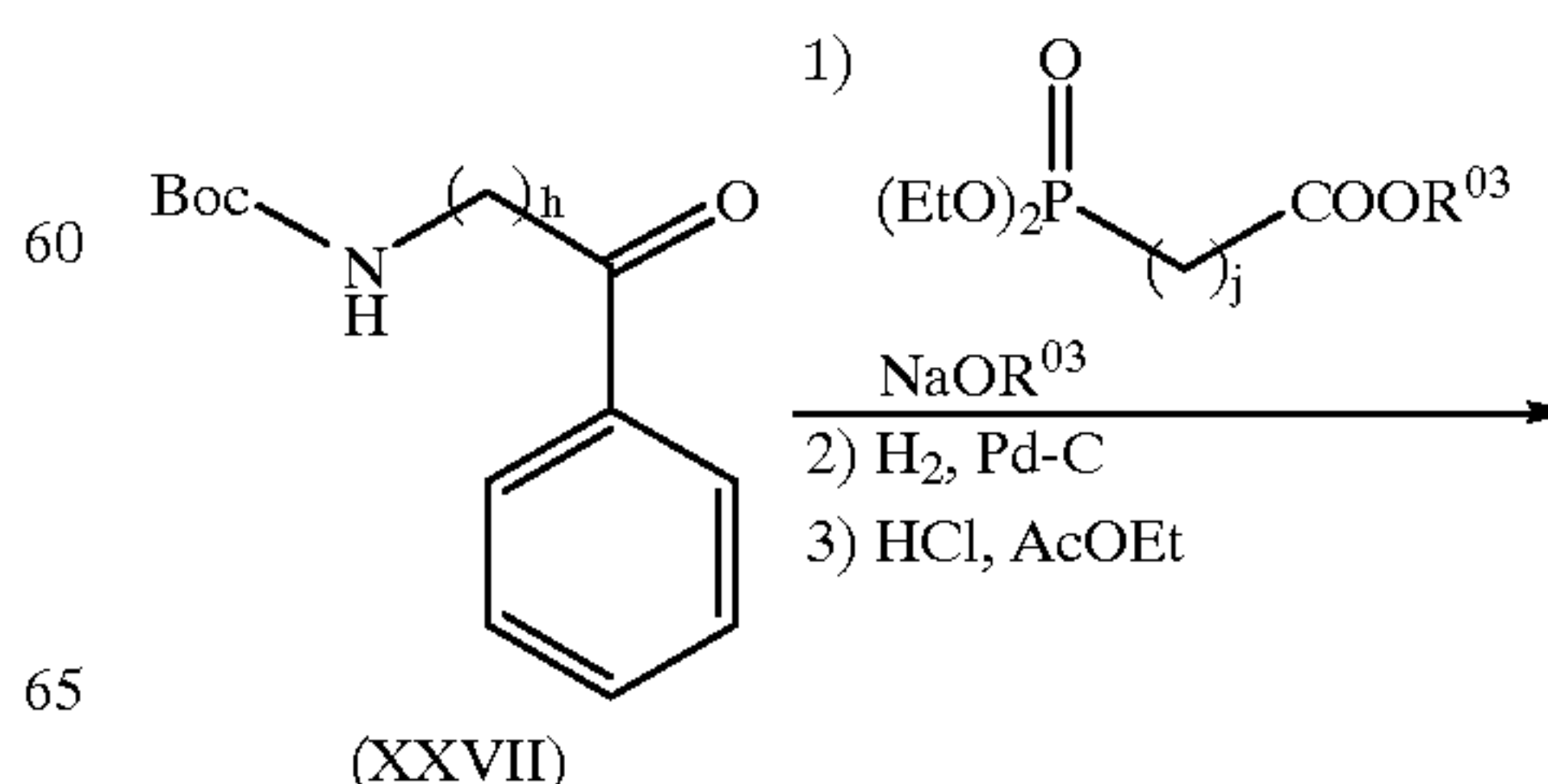
Scheme 9
