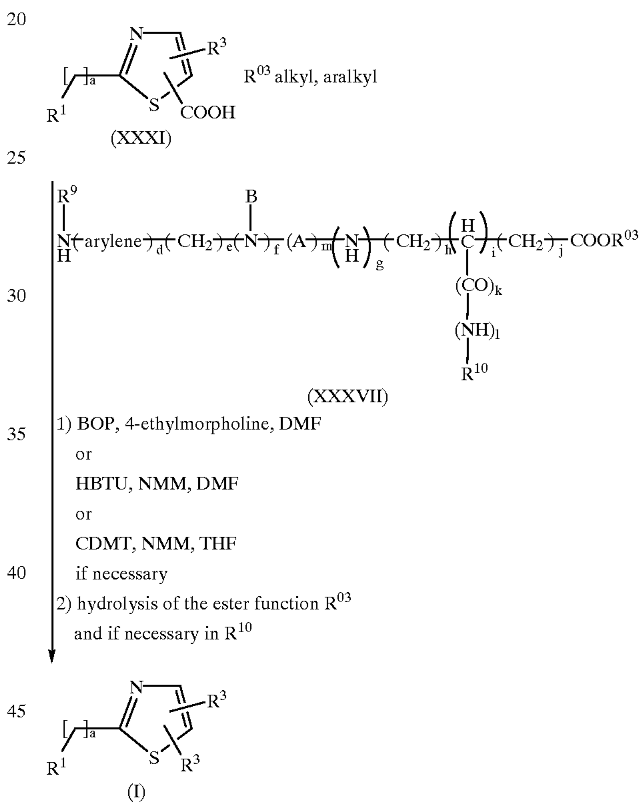
Scheme 2
