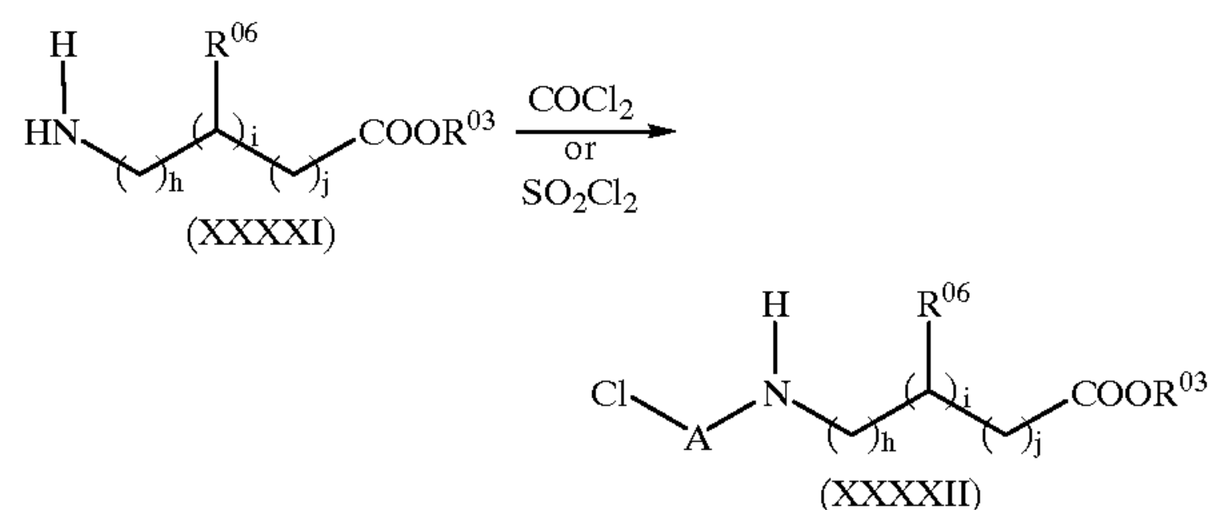
Scheme 6b
