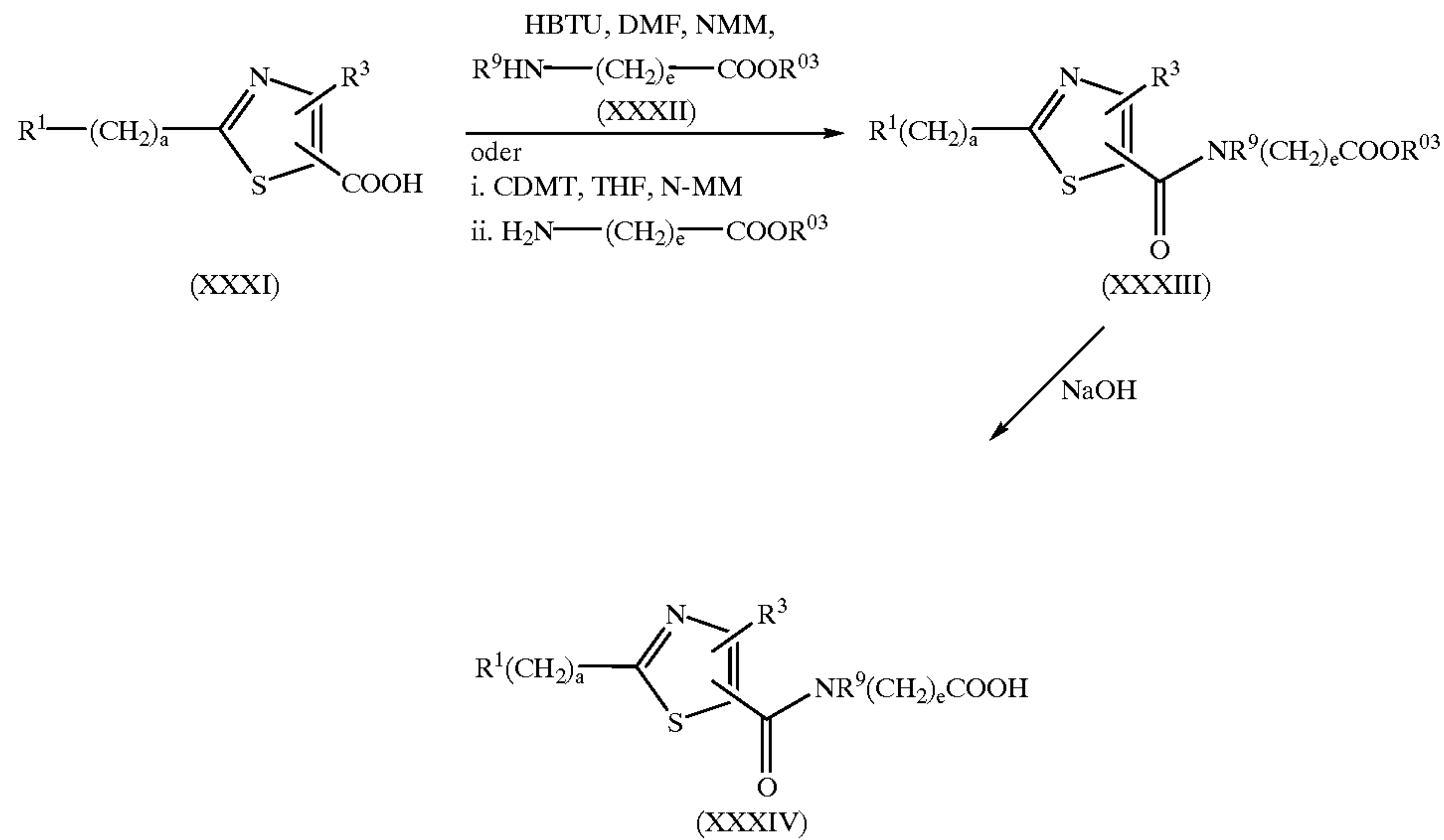
Scheme 3
