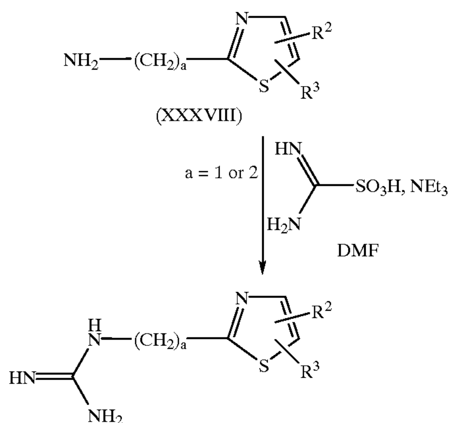
Scheme 10
