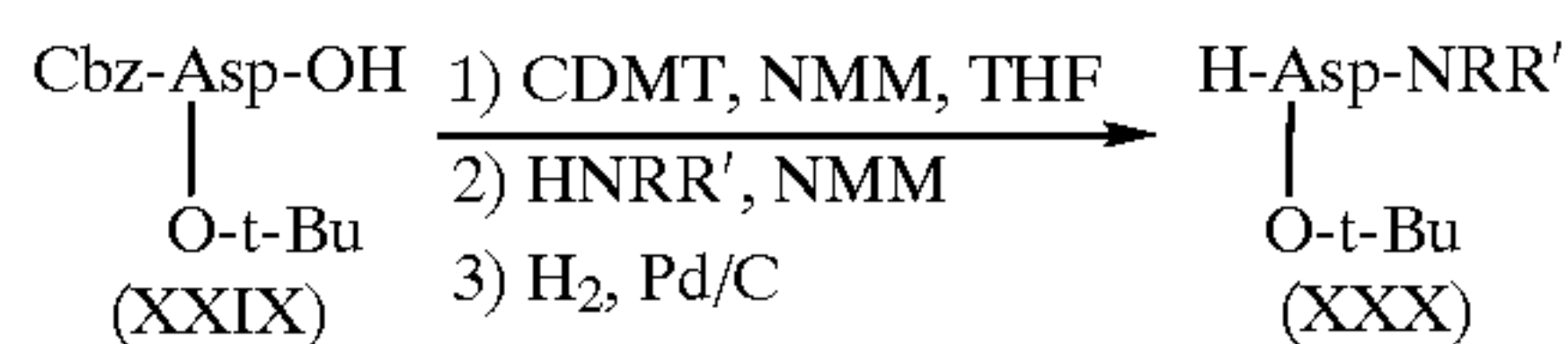
Scheme 6a
