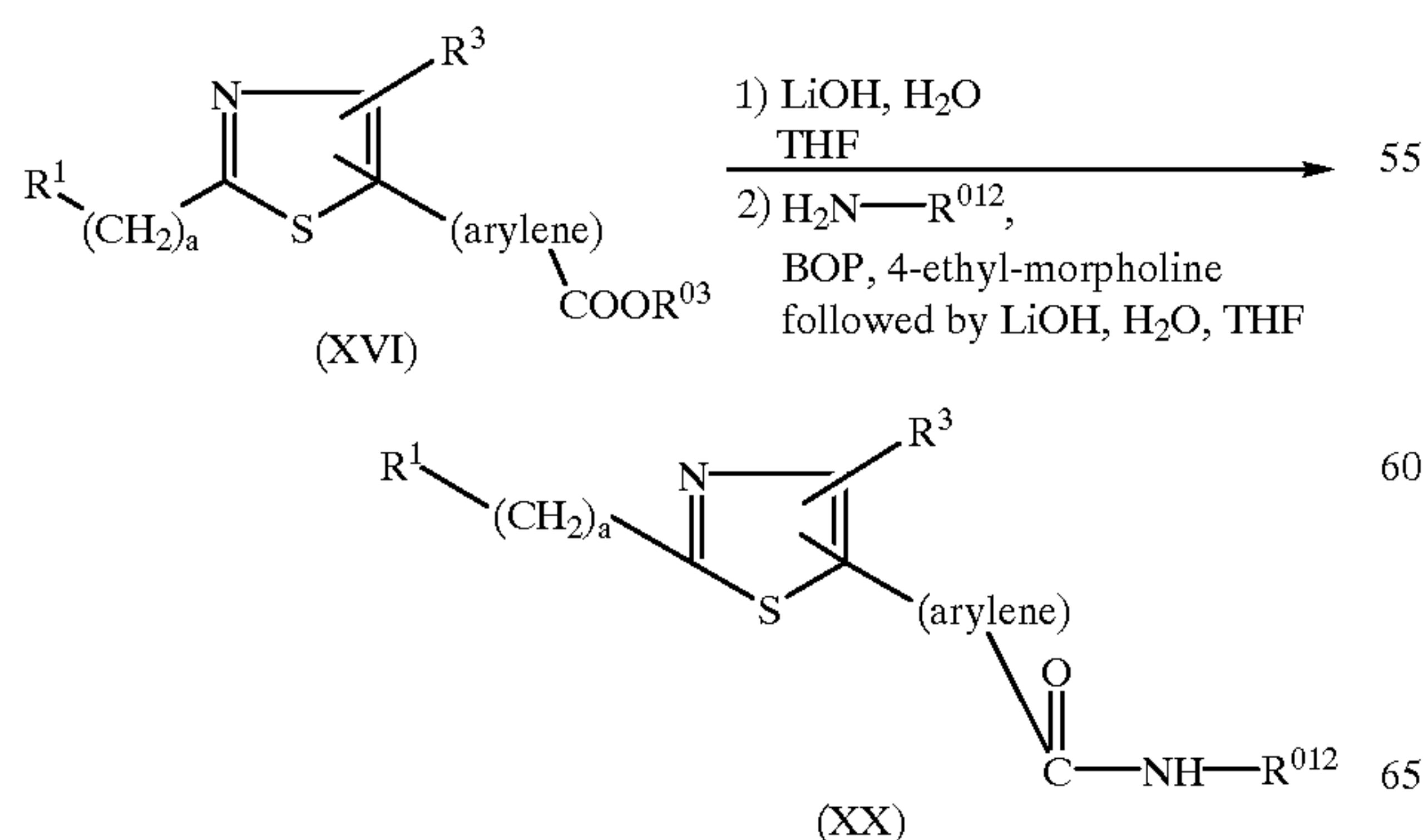
Scheme 8
