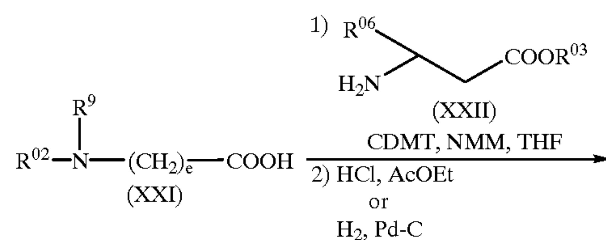
Scheme 4
