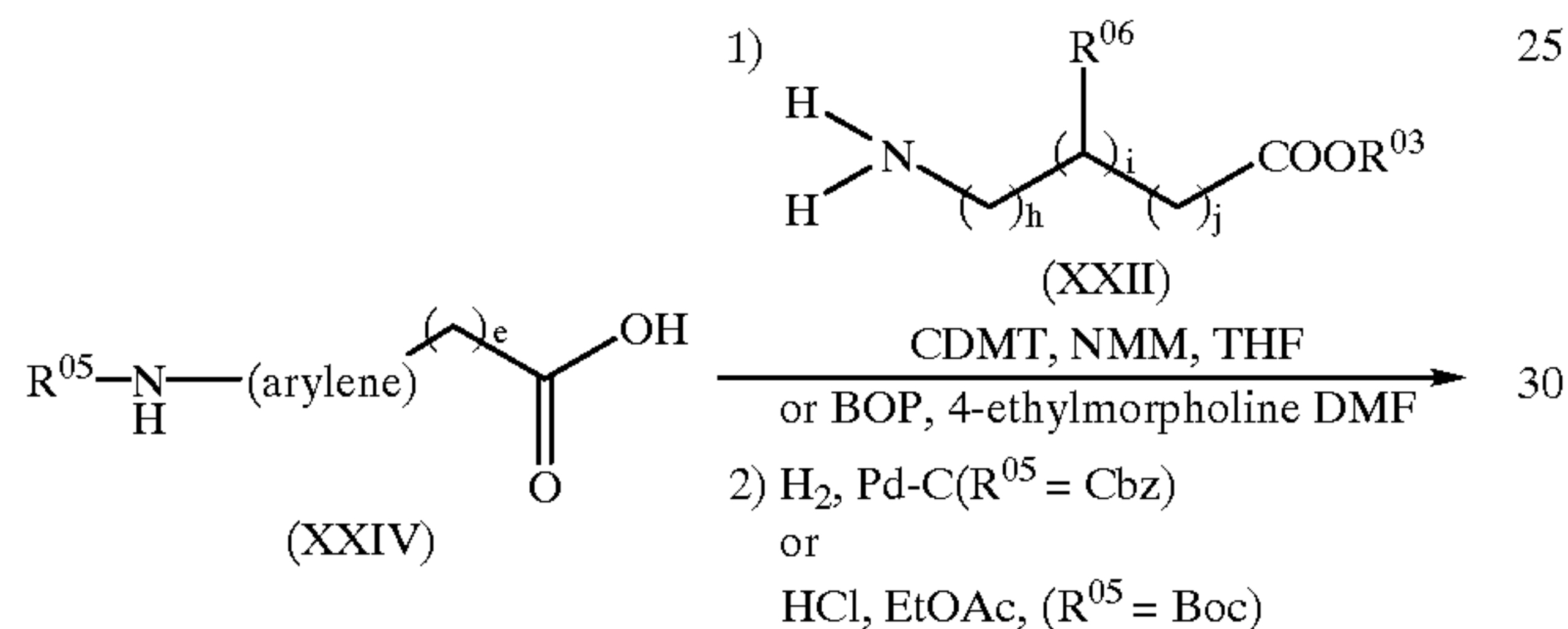
Scheme 5a
