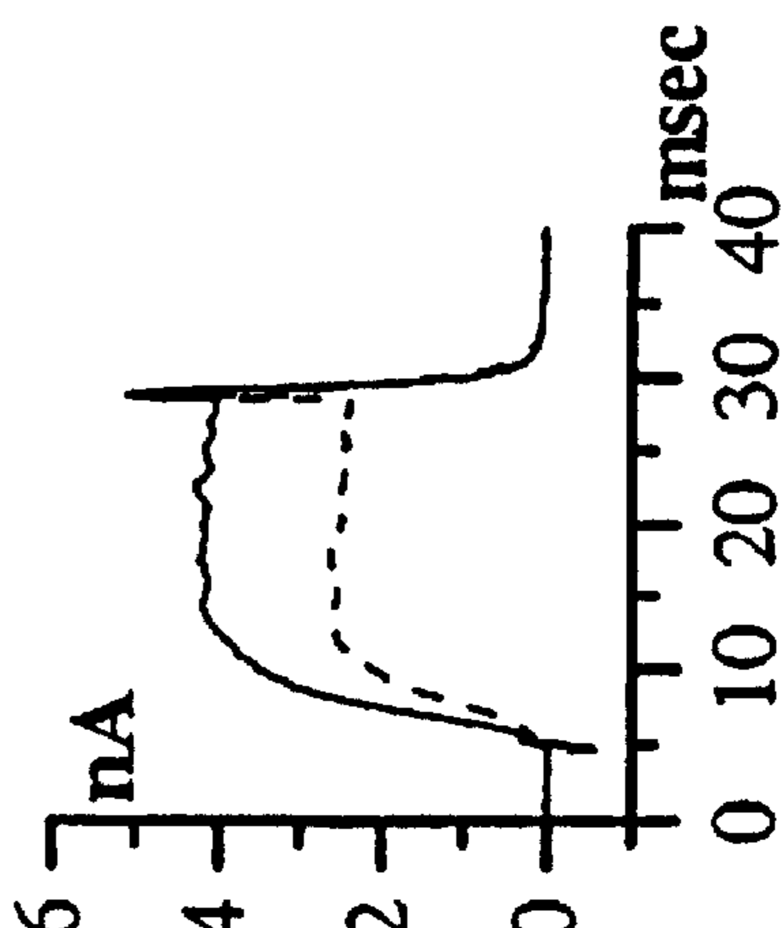
FIG. 3d Flouride
