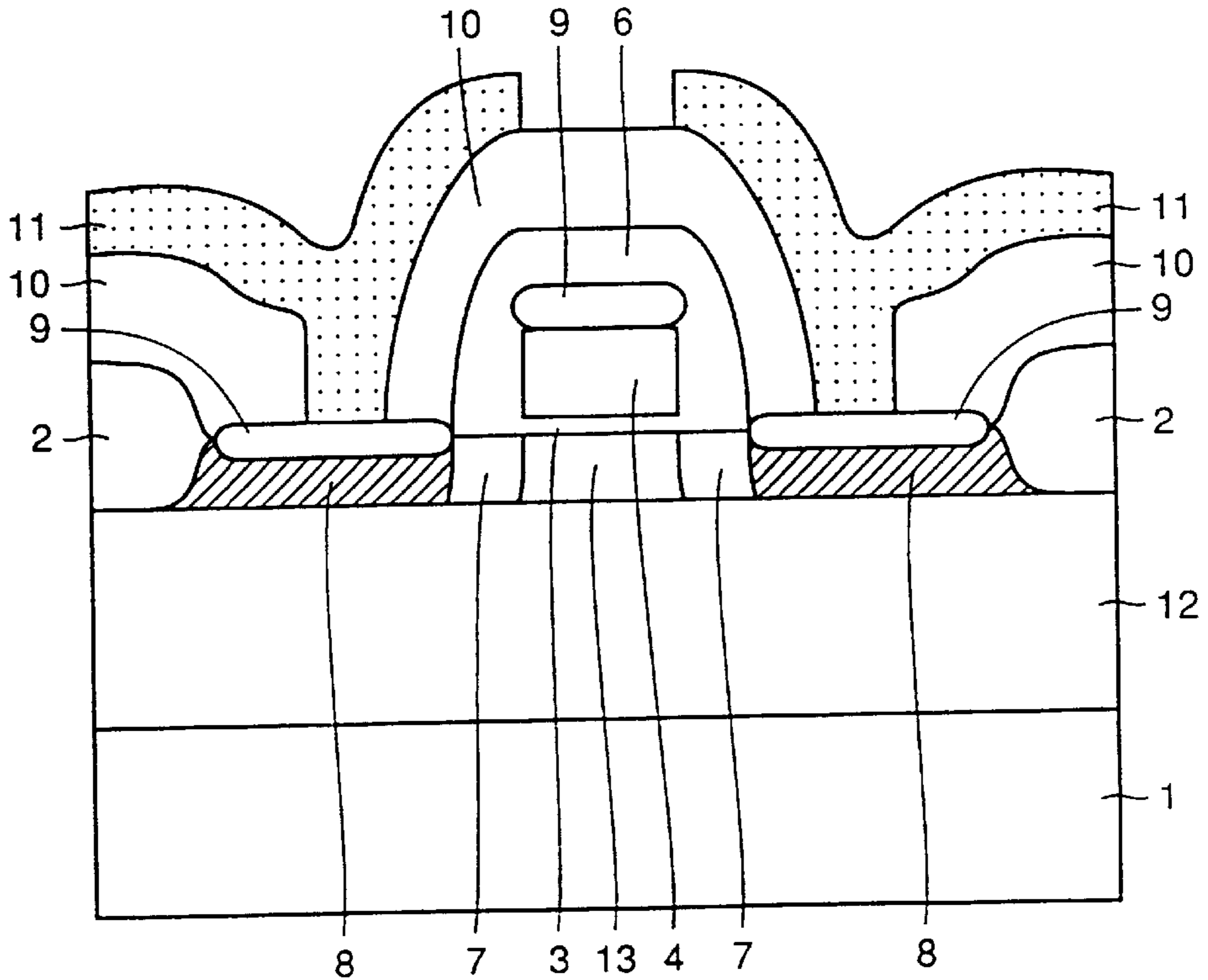
FIG.37 PRIOR ART
