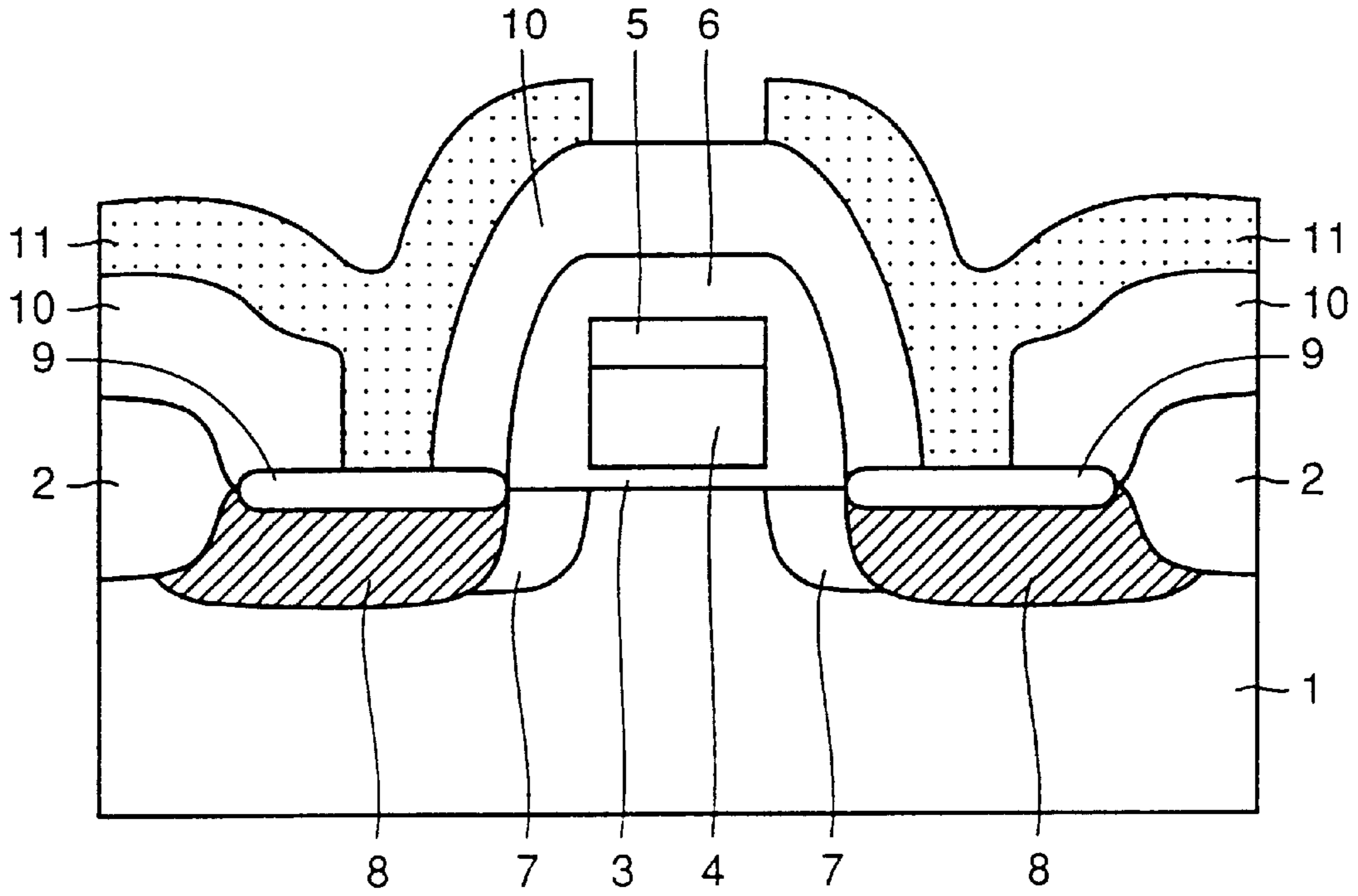
FIG.34 PRIOR ART
