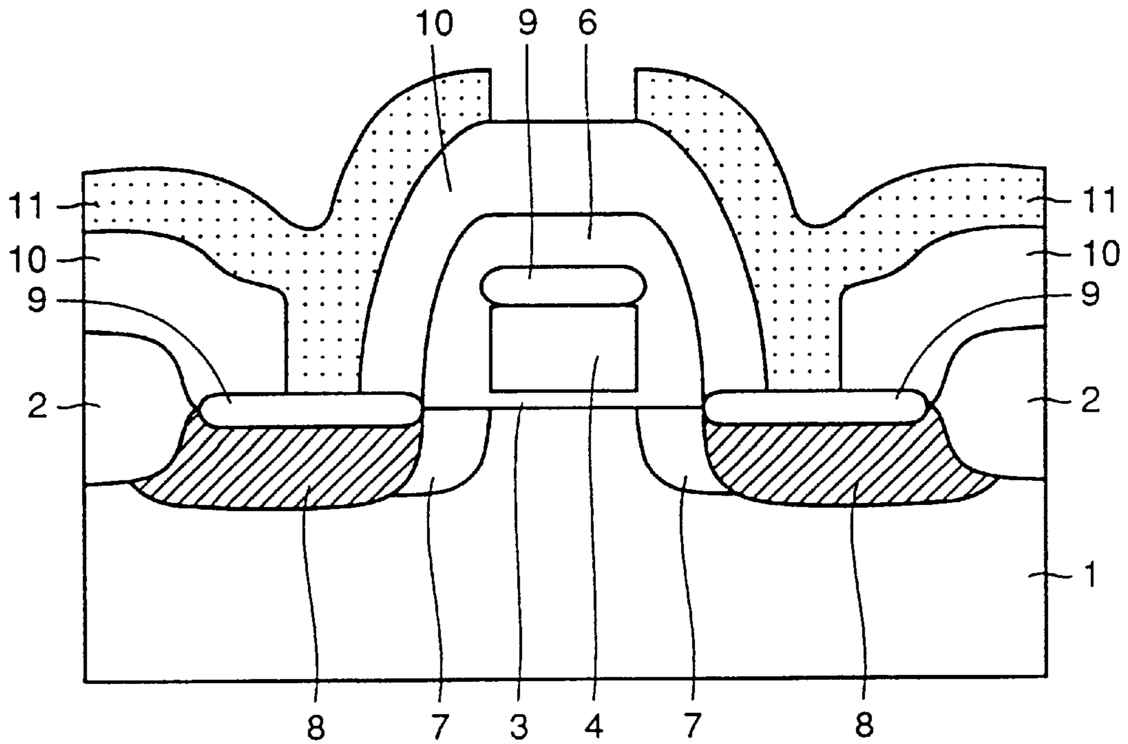
FIG.35 PRIOR ART
