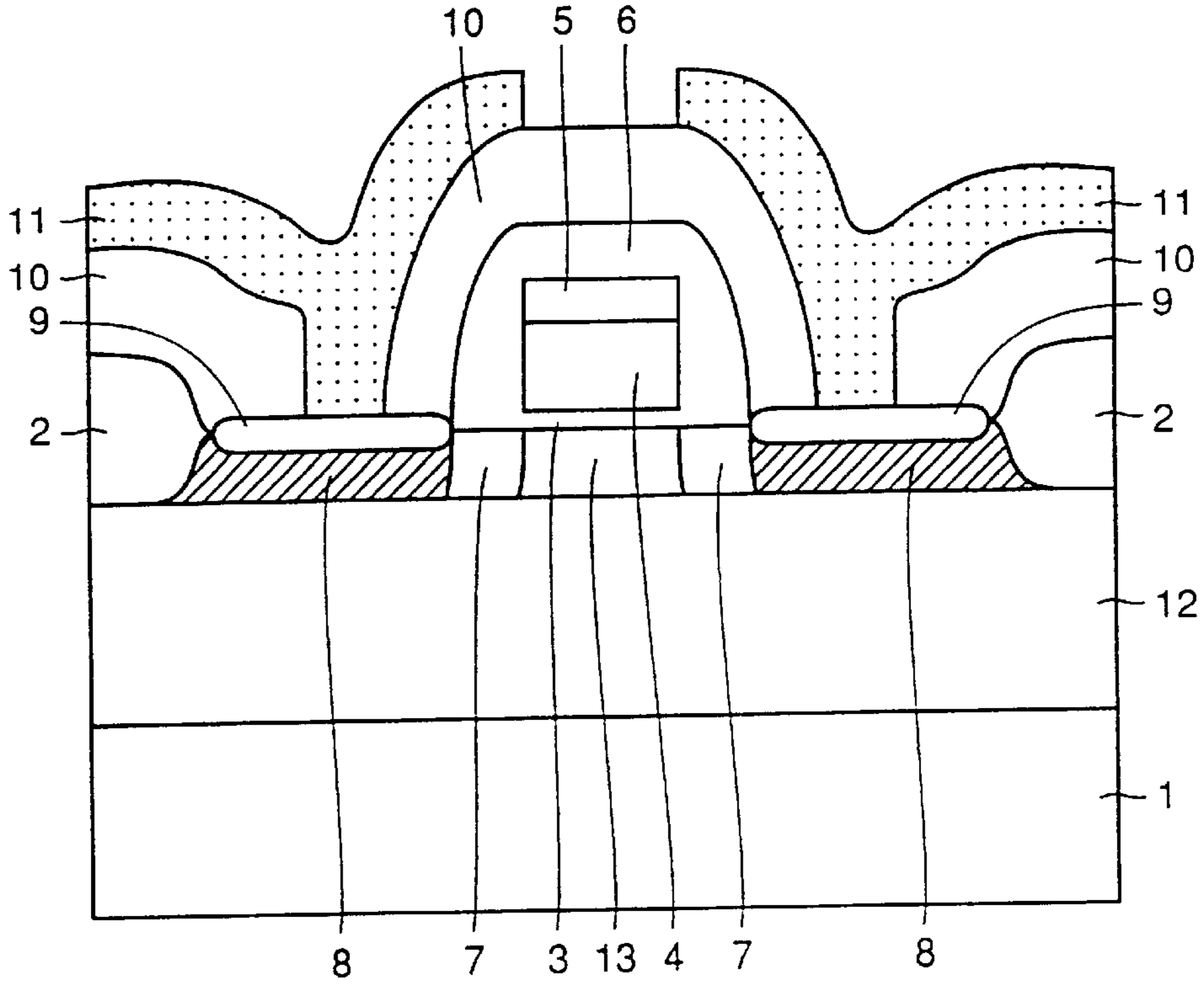
FIG.36 PRIOR ART
