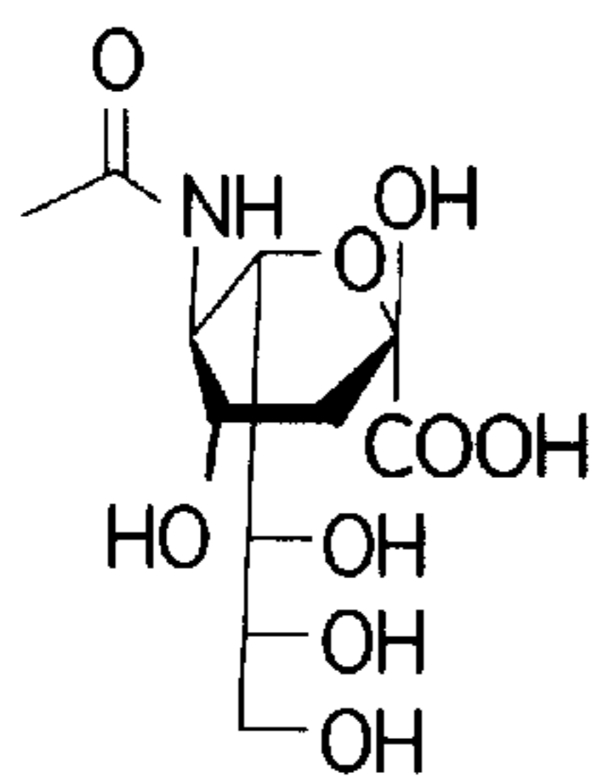
N-ACetylNEURAMINIC ACID
