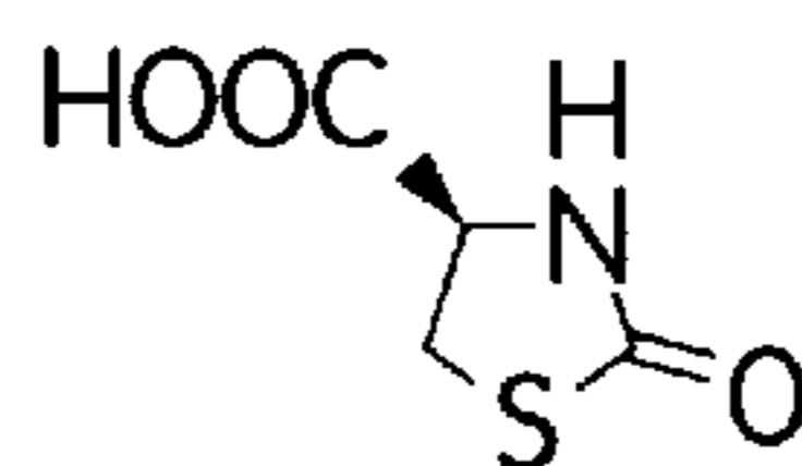
(-)-2-OXO-4-THIAZOLIDINE-CARBOXYLIC ACID
