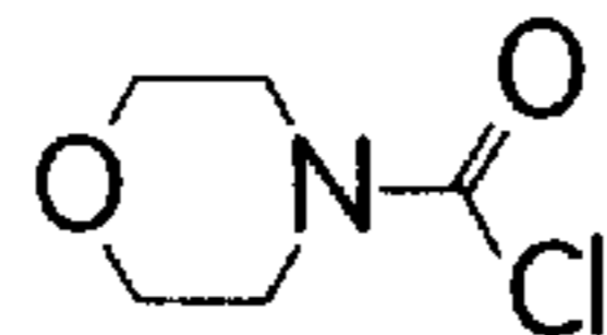
4-MORPHOLINECARBONYL CHLORIDE
