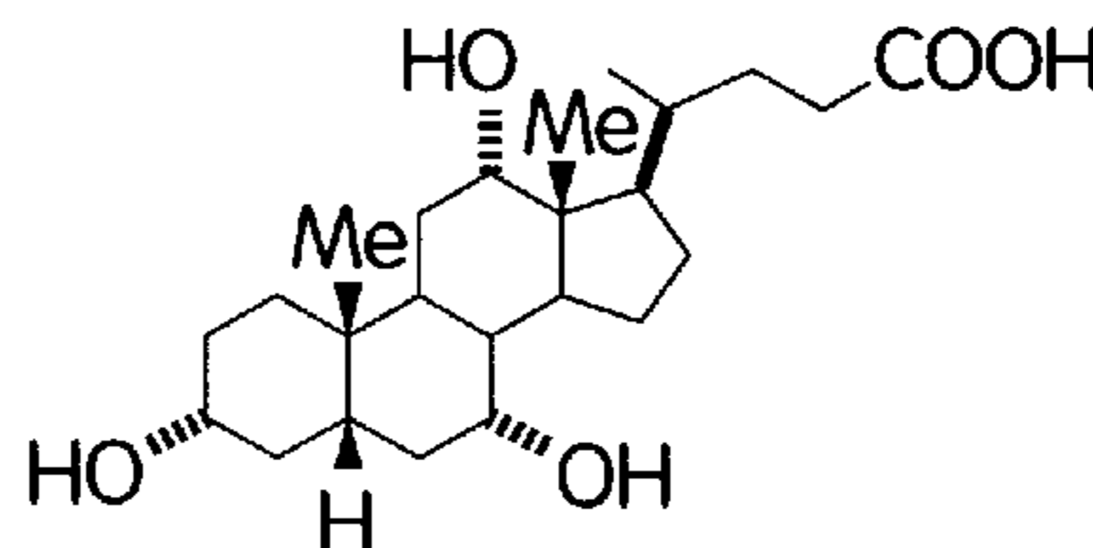
CHOLIC ACID
