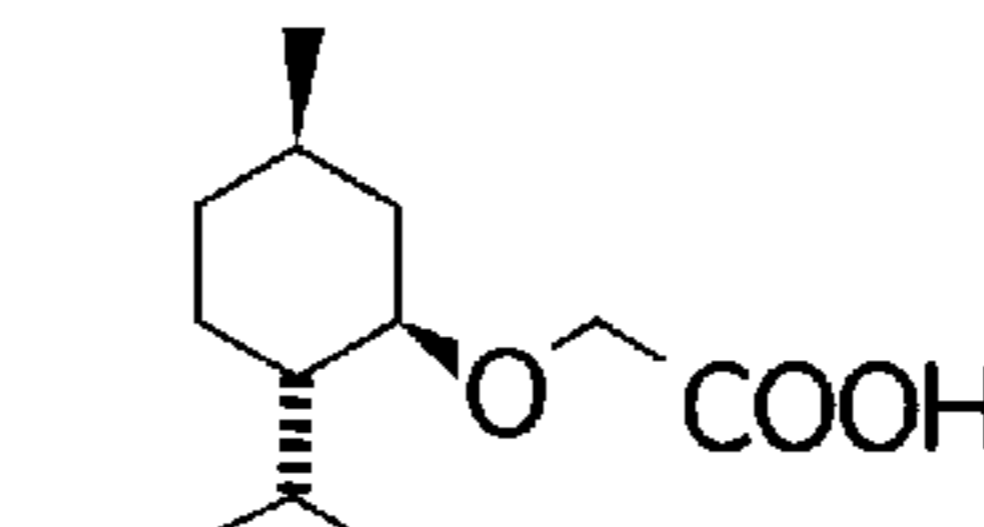
(-)-MENTHOXYACETIC ACID
