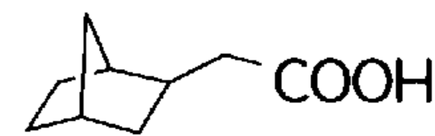
2-NORBORNANEACETIC ACID
