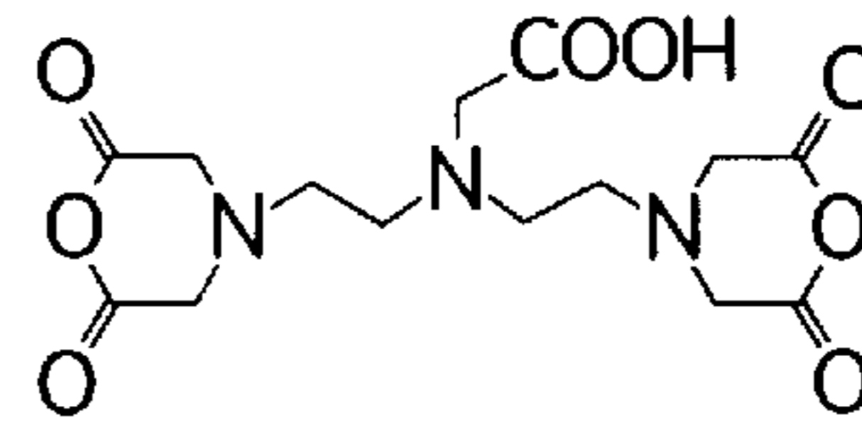
DIETHYLENTRIAMINEPENTAACETIC DIANHYDRIDE
