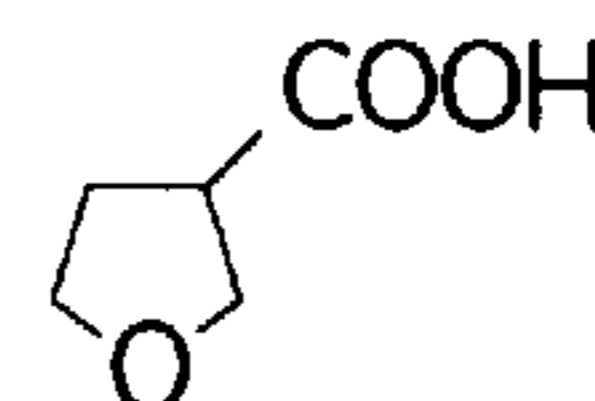
TETRAHYDRO-3-FUROIC ACID
