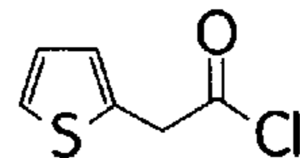
2-THIOPHENEACETYL CHLORIDE
