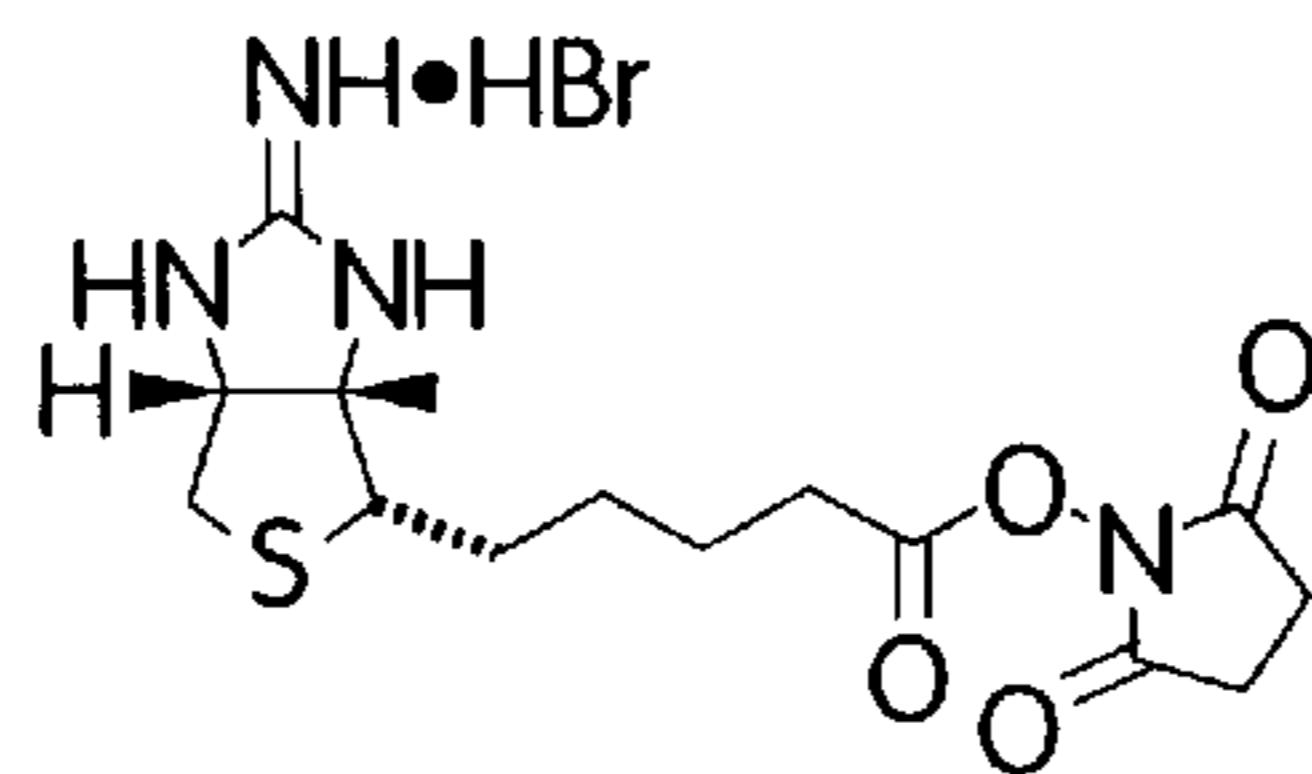
2-IMINOBIOTIN-NHS ESTER
