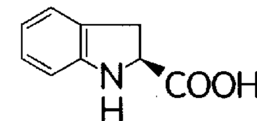
(S)-(-)-INDOLINE-2-CARBOXYLIC ACID
