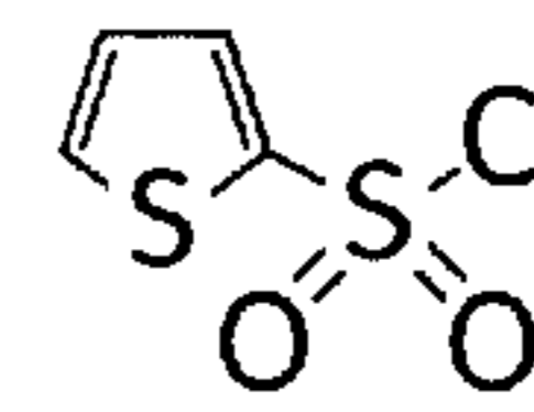
2-THIOPHENESULFONYL CHLORIDE
