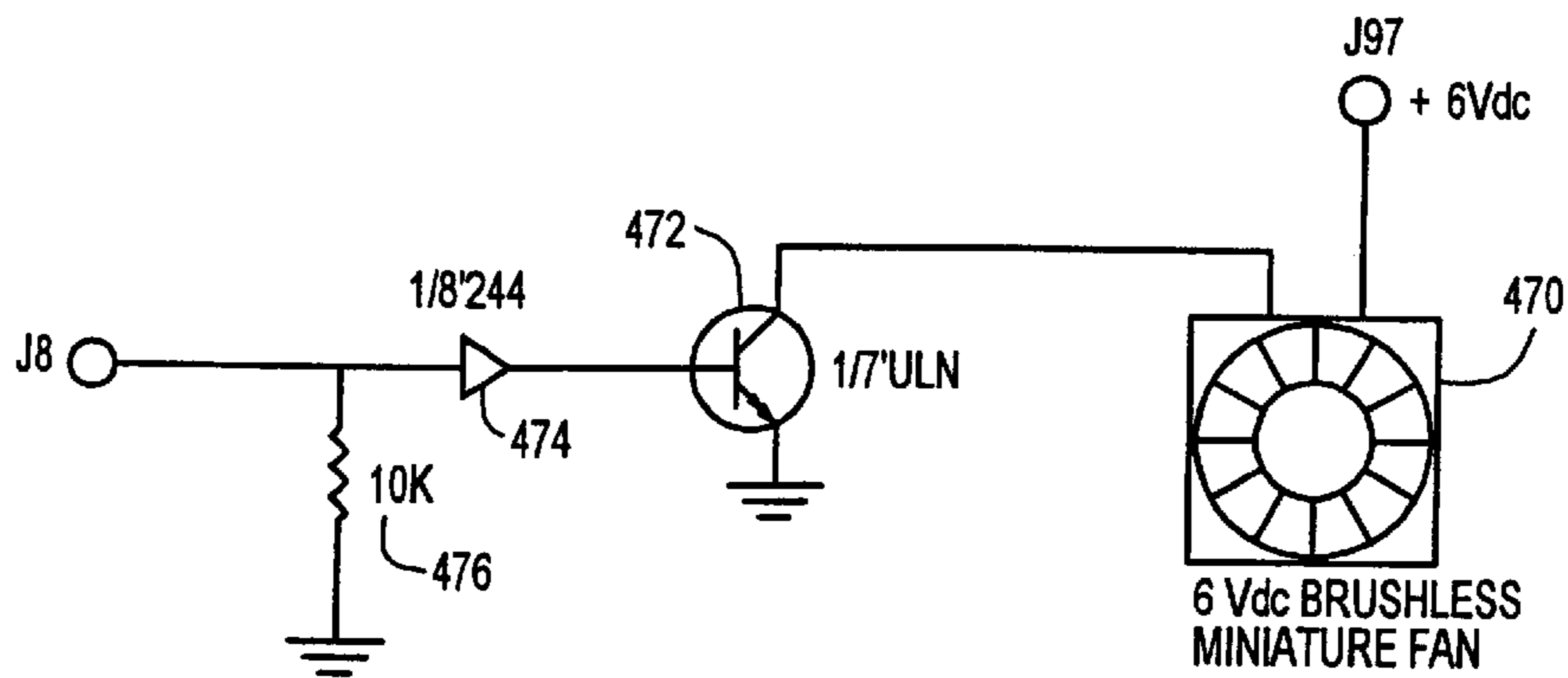
FIG. 36 SCAVENGING SYSTEM 468
