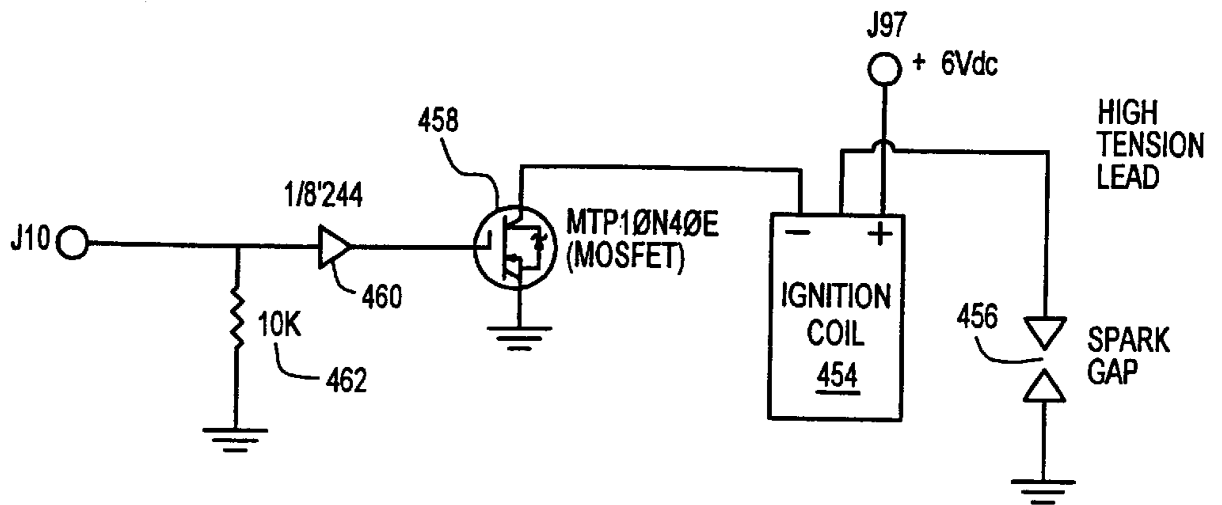
FIG. 35 IGNITION SYSTEM 452
