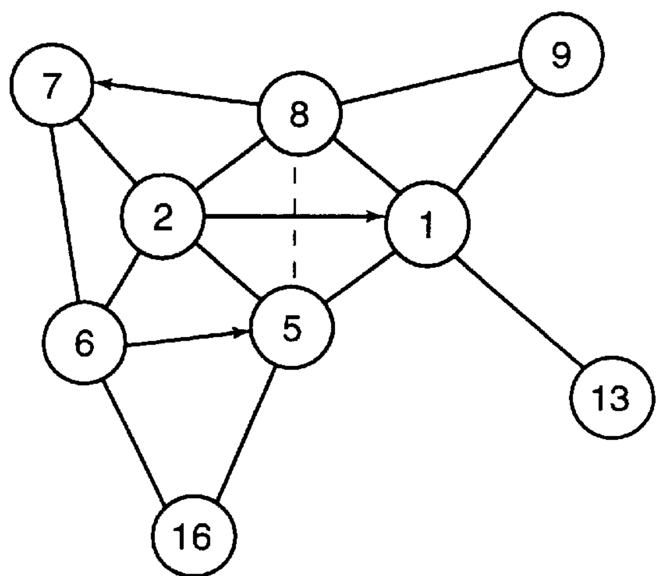
LINK ACTIVATION
