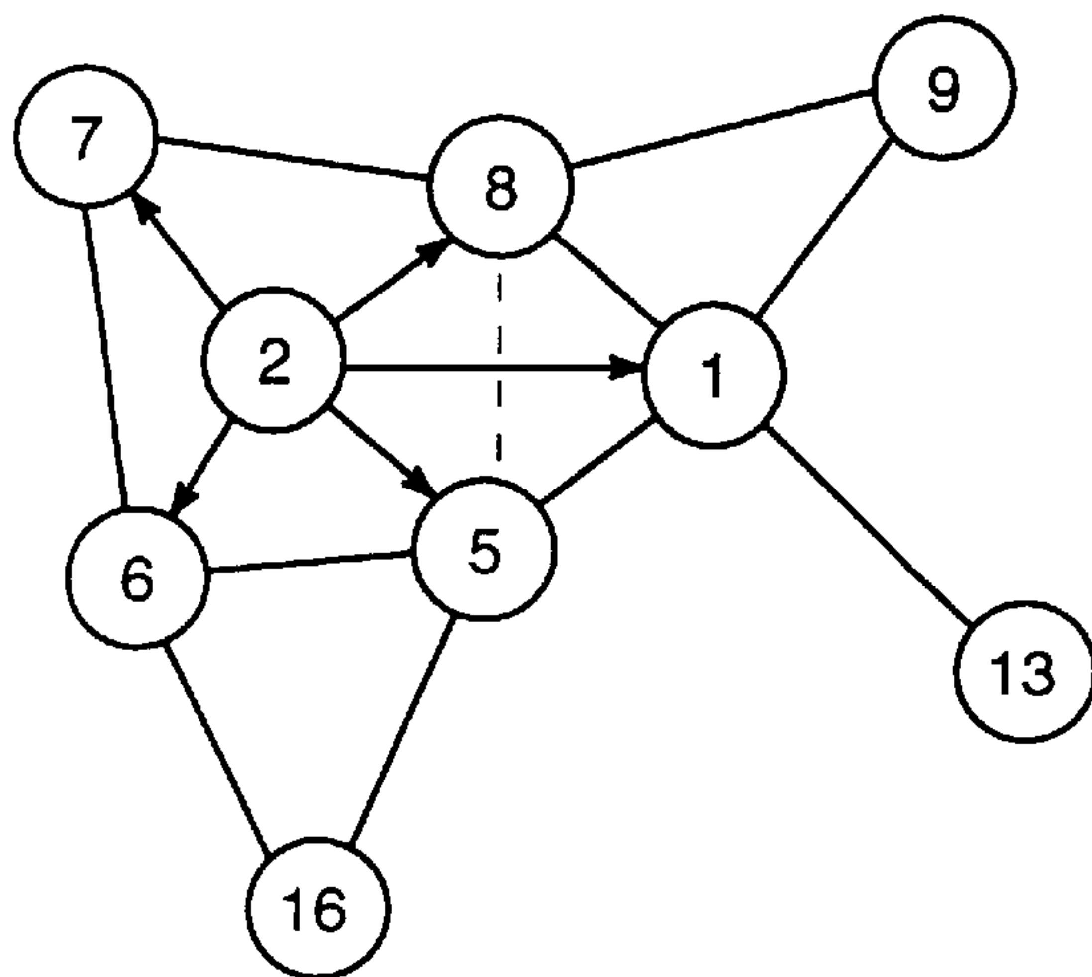
NODE ACTIVATION
