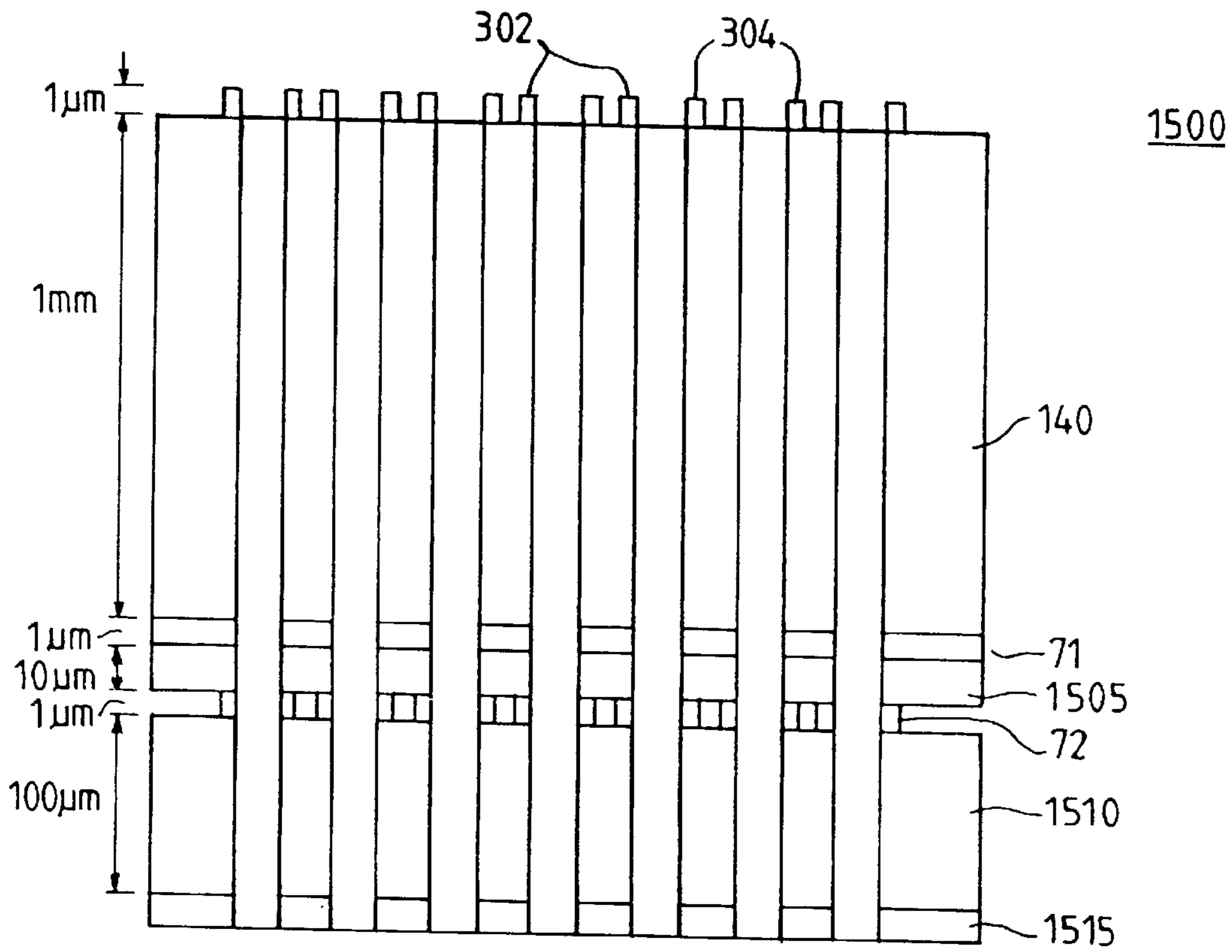
FIG. 14 PRIOR ART
