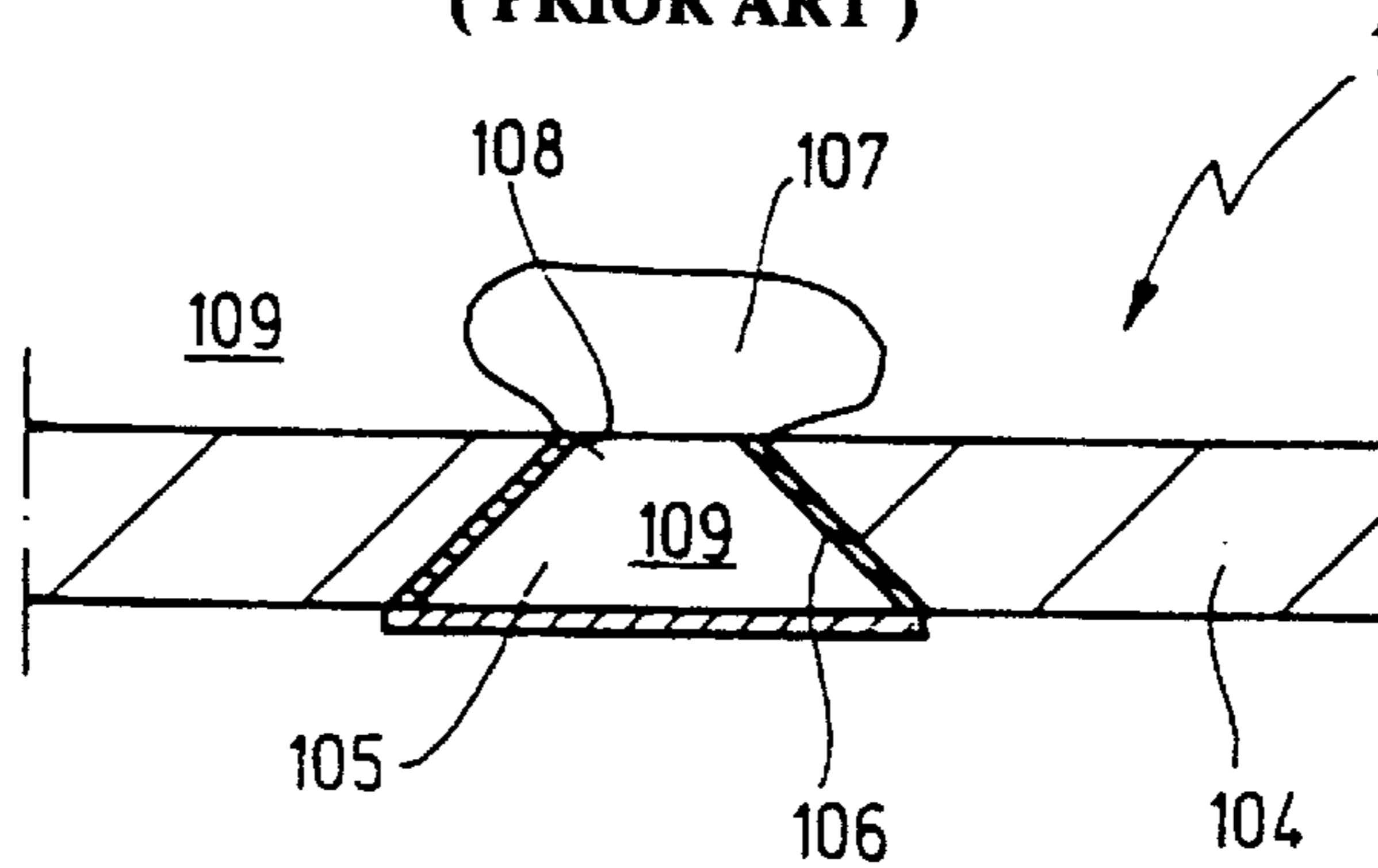
Fig. 2 (PRIOR ART)
