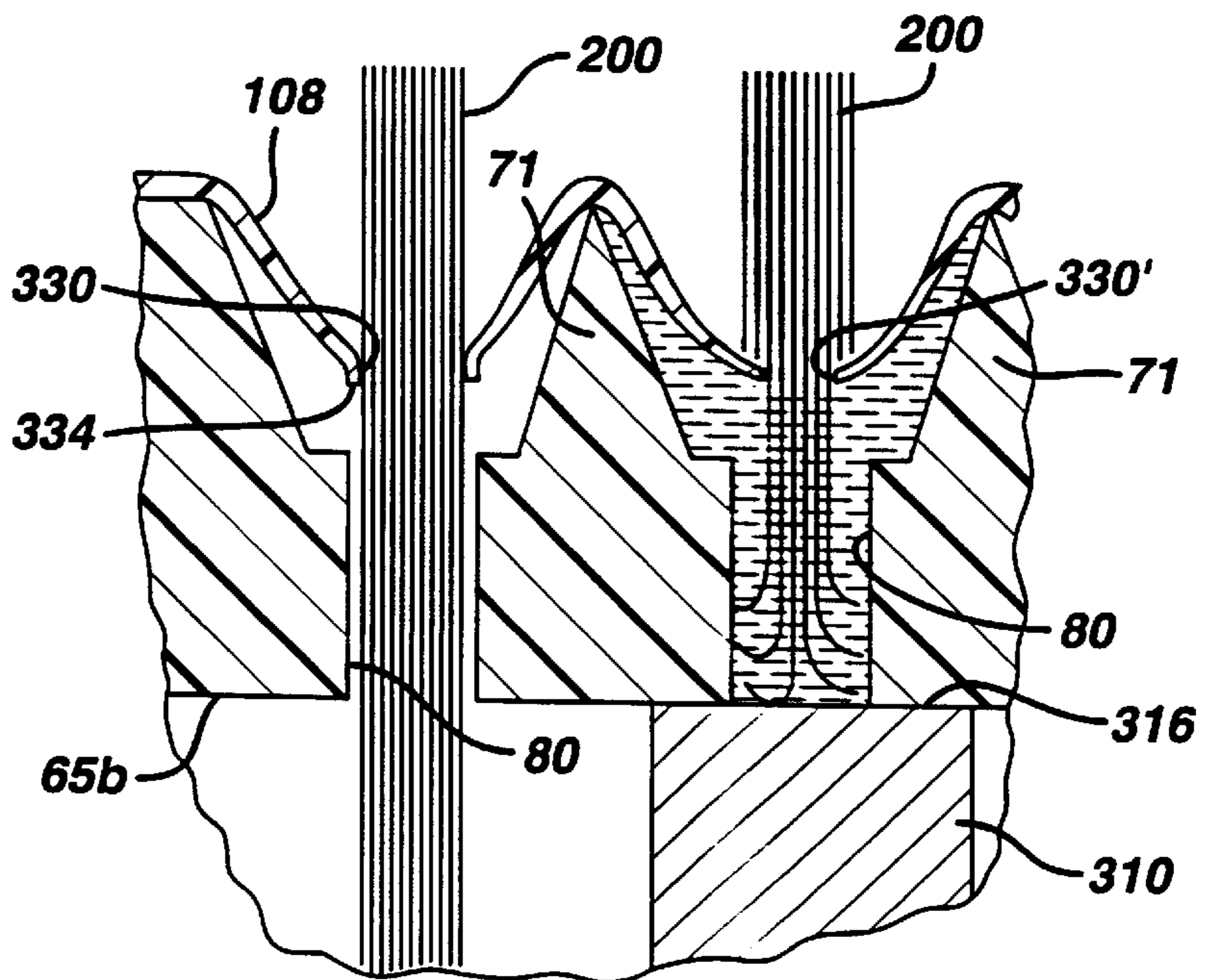
FIG. 5 PRIOR ART
