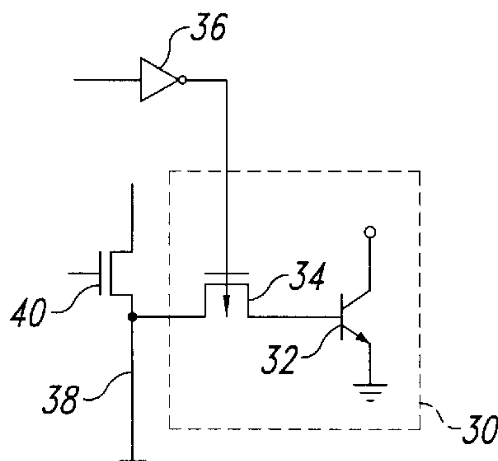
Fig. 2 (Prior Art)
